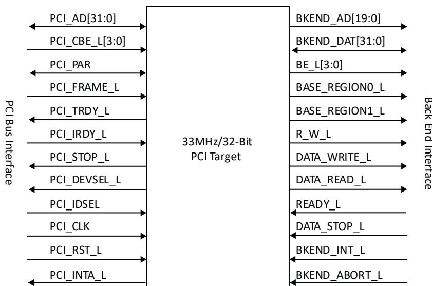
Figure 3.1. PCI Target I/O Interface
