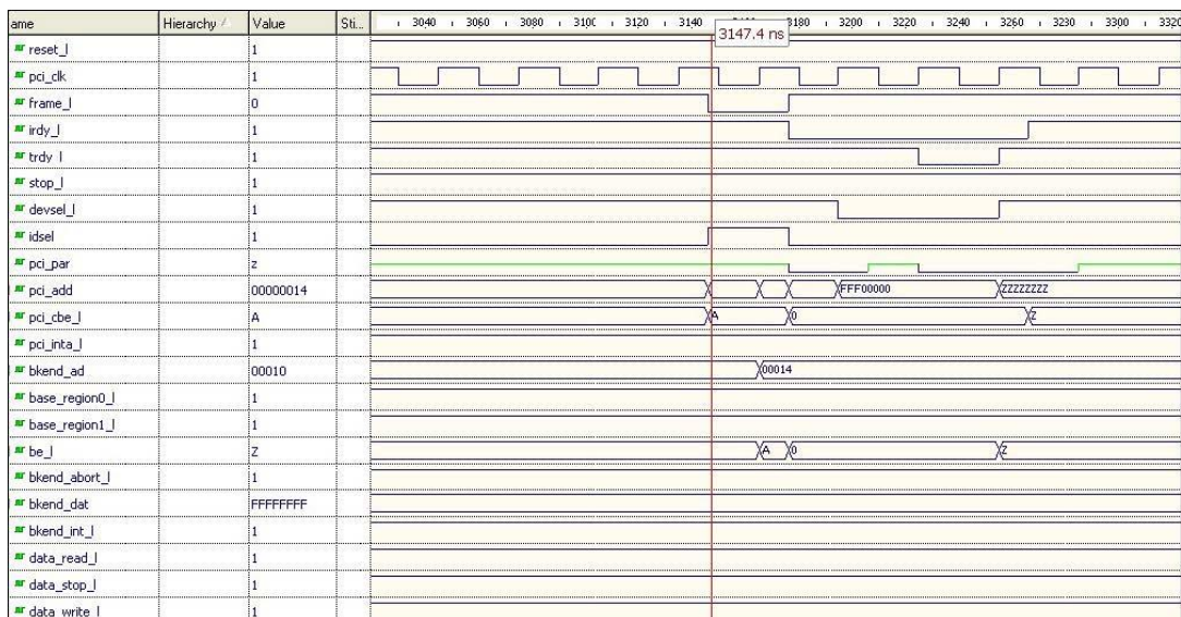
Figure 6.2. 33 MHz, 32-Bit PCI Target – Configuration Read
