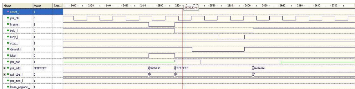
Figure 6.1. 33 MHz, 32-Bit PCI Target – Configuration Write
