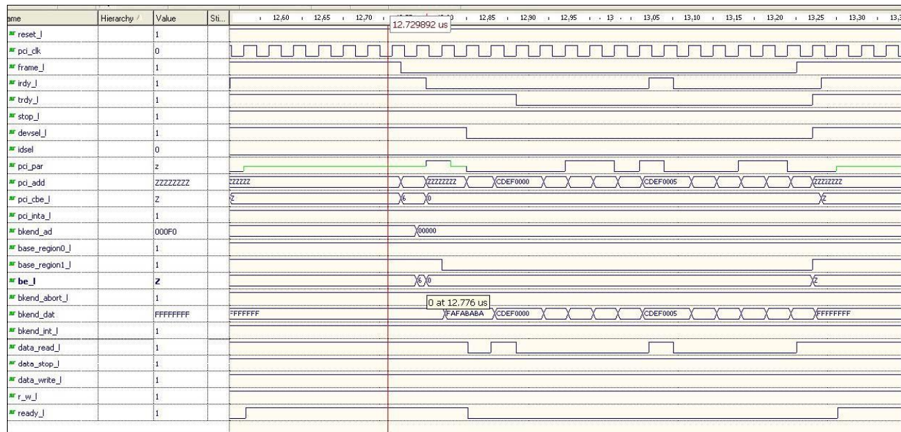
Figure 6.6. 33 MHz, 32-Bit PCI Target – Burst Read
