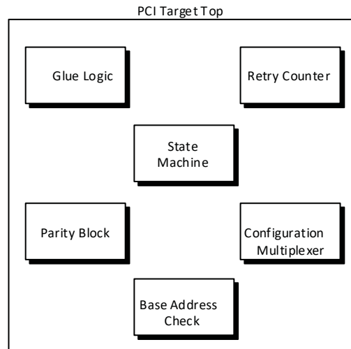
Figure 4.1. The 33 MHz, 32-Bit PCI Target Block Diagram
