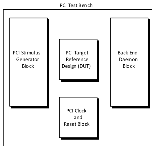
Figure 5.1. 33 MHz, 32-Bit PCI Target Test Suite
