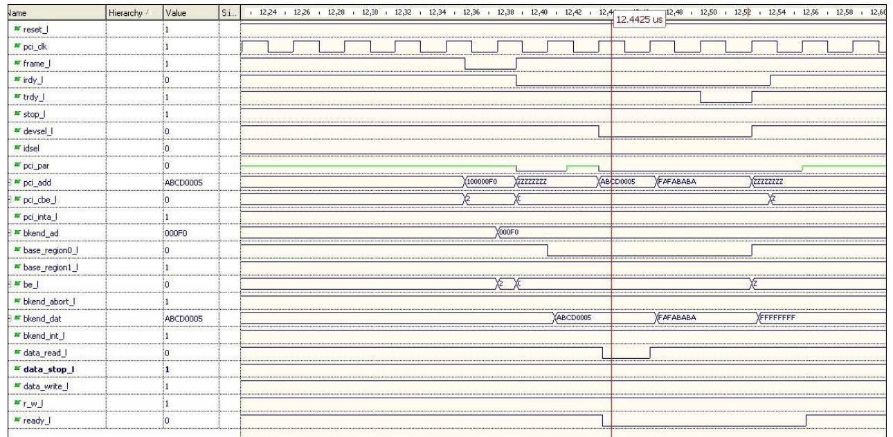
Figure 6.4. 33 MHz, 32-Bit PCI Target – Single Read
