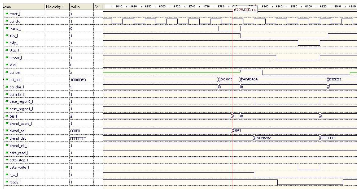
Figure 6.3. 33 MHz, 32-Bit PCI Target – Single Write
