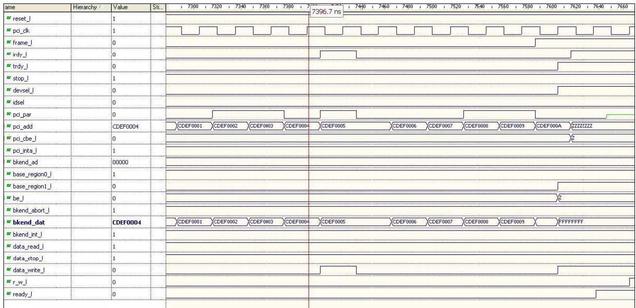
Figure 6.5. 33 MHz, 32-Bit PCI Target – Burst Write
