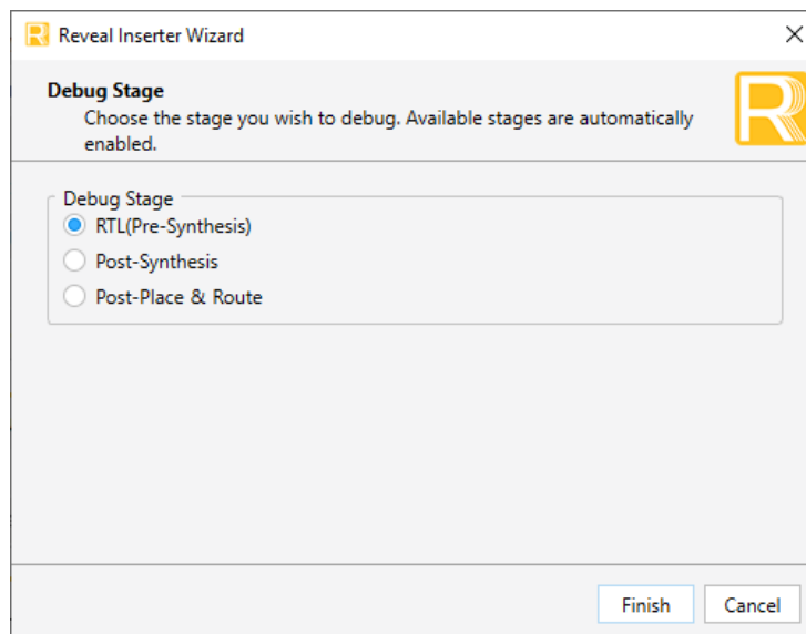
Figure 1: Reveal Inserter Wizard
