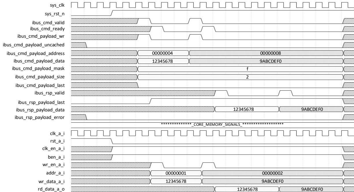
Figure 2.2. Write-Read Operation
