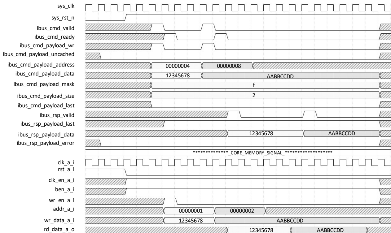
Figure 2.3. Sequential Write/Read
