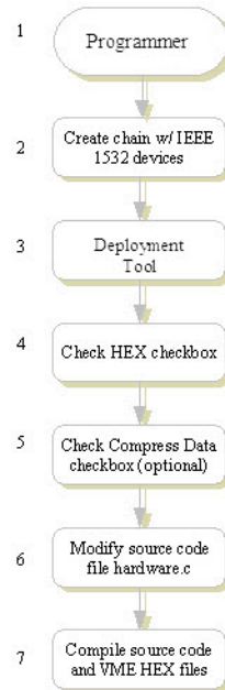
Figure 47: 8051 JTAG Slim VME Embedded User Flow
