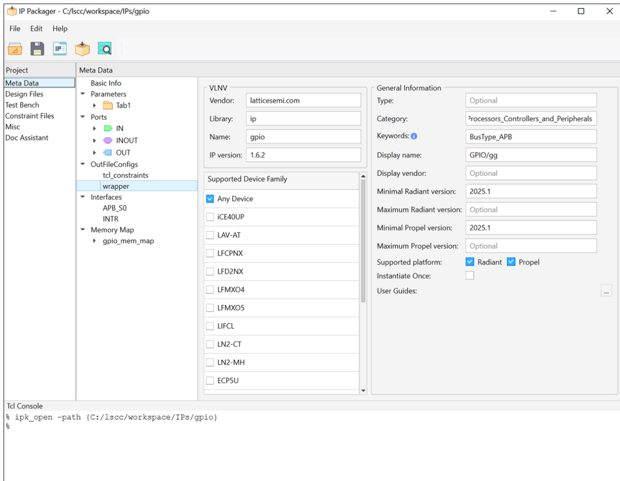
Figure 2.6. IP Packager with IP Project Details
