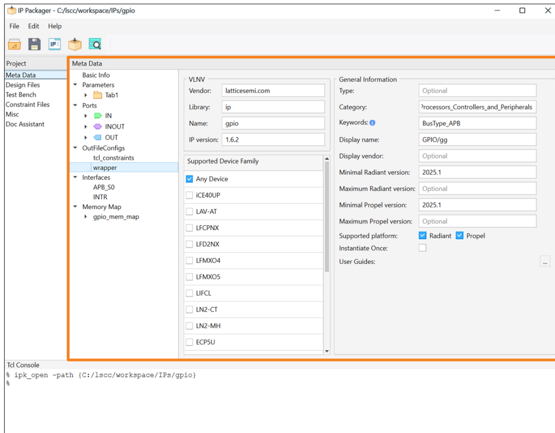
Figure 2.7. IP Packager with Meta Data Details
