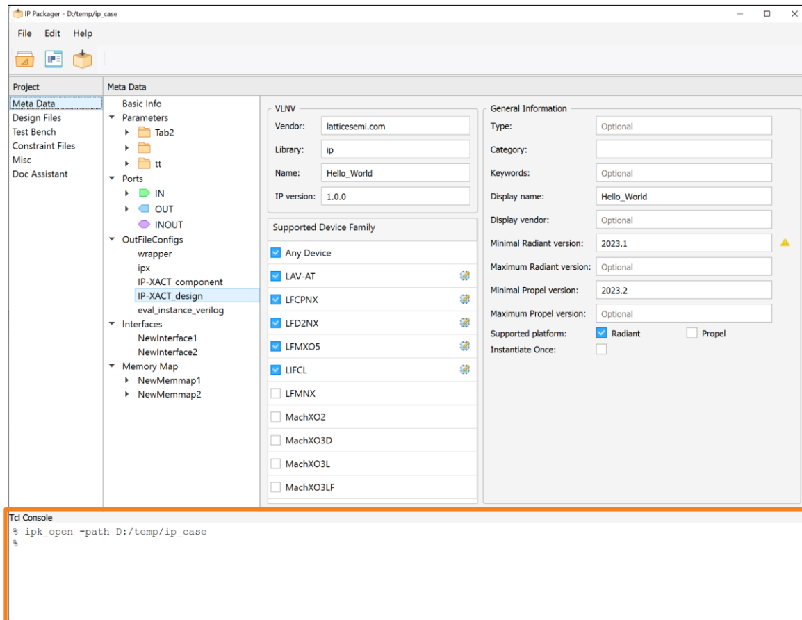
Figure 3.1. Tcl Console
