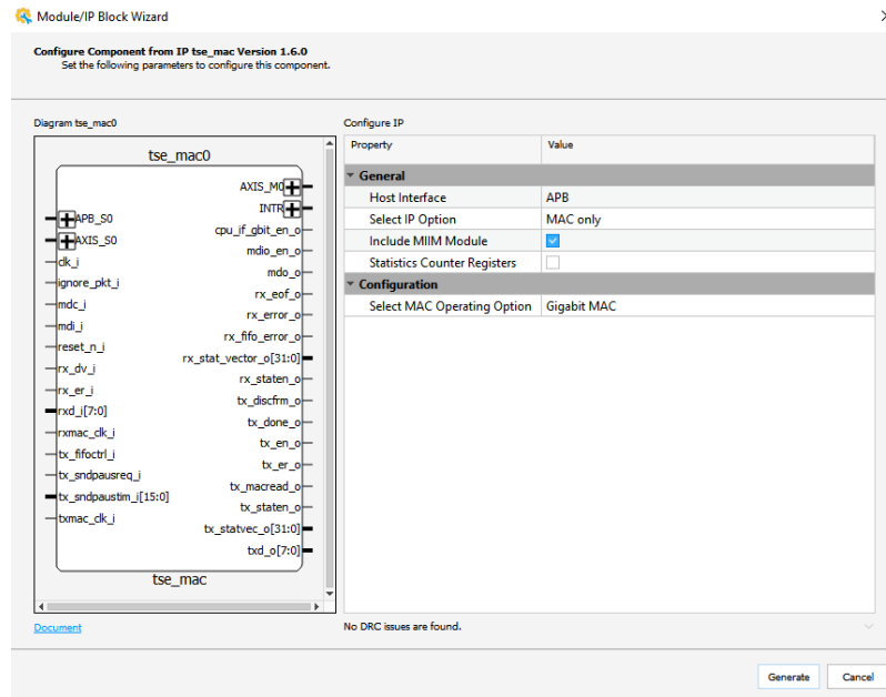
Figure 2.11. TSE MAC Configuration
