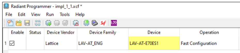
Figure 7.12. Select Device for Programming
