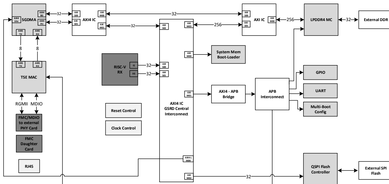
Figure 2.1. GHRD Architecture on Avant-AT-E
