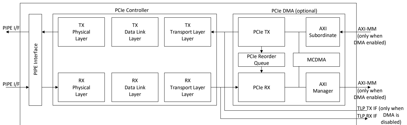
Figure 2.16. PCIe Core
