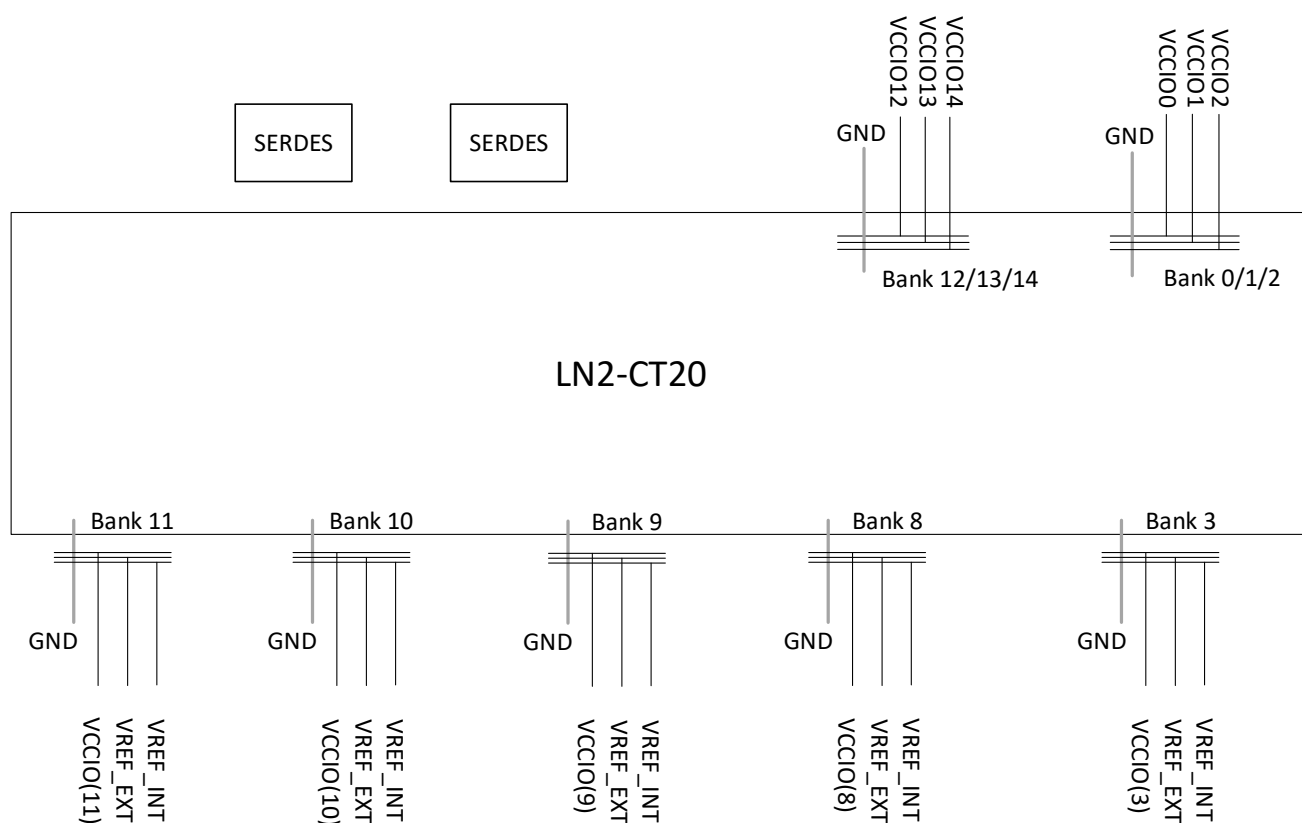
Figure 2.11. sysI/O Banking (LN2-CT20 Device)
