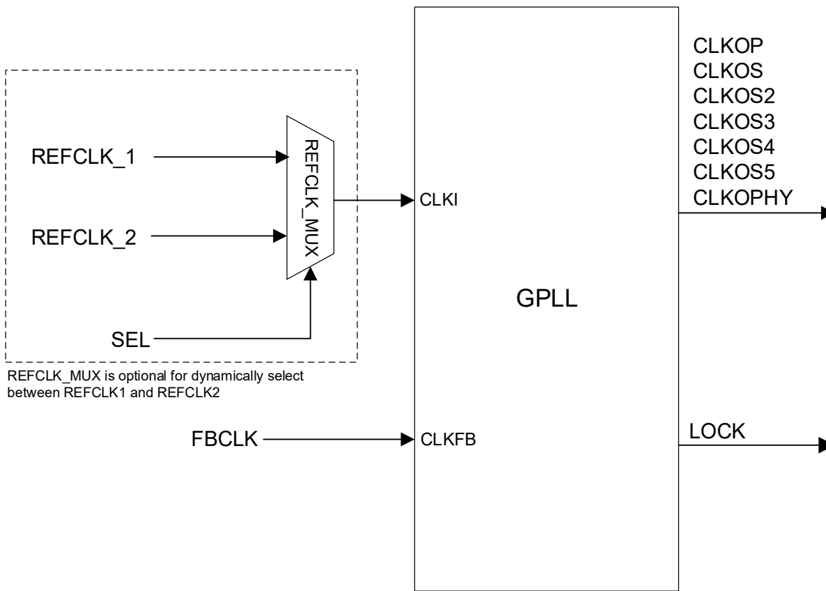
Figure 2.6. Lattice Nexus 2 PLL Block Diagram
