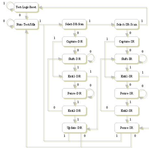
Figure 51: Shift Registers
