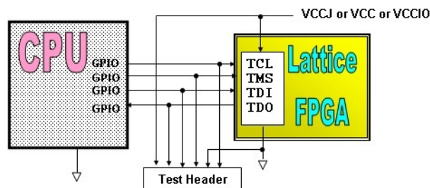
Figure 13: Map Four GPIO Pins from the CPU to the Four JTAG Pins
