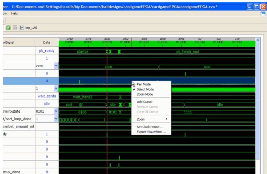
Figure 102: Reveal Analyzer Waveform Cursor Controls
