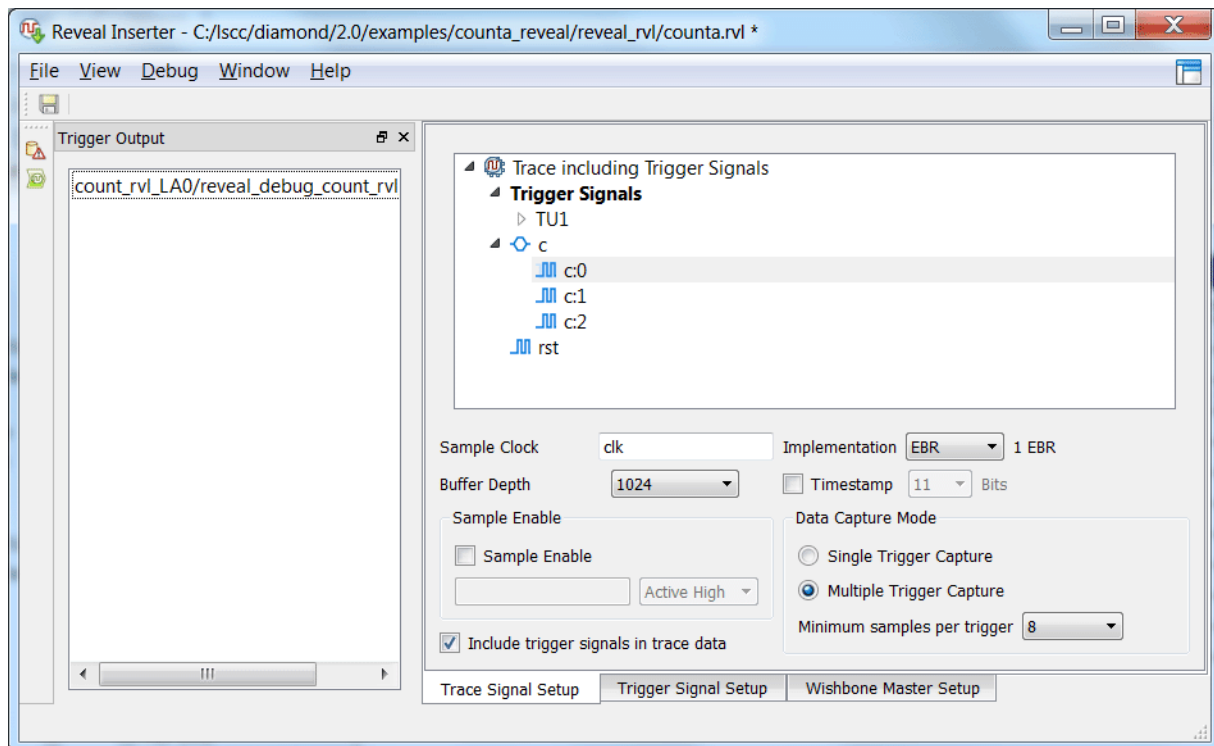
Figure 96: Reveal Inserter Trace Signal Setup
