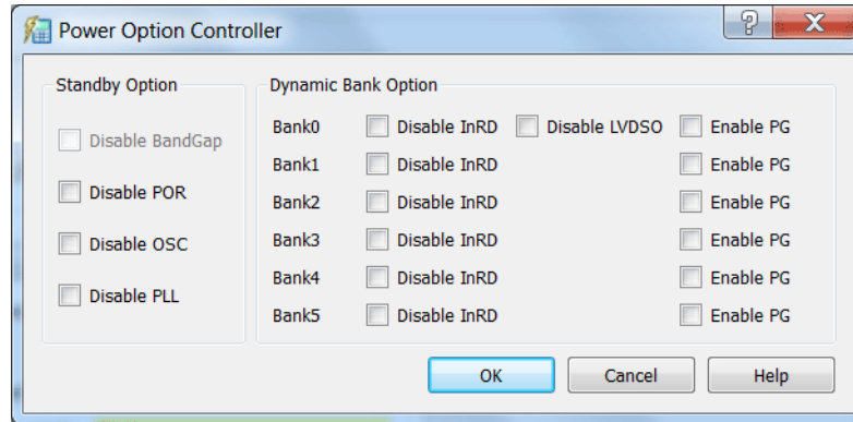
Figure 115: Power Option Controller for MachXO2, MachXO3D, MachXO3L, MachXO3LFP, and Platform Manager 2
