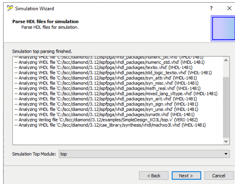
Figure 77: Simulation Top Module
