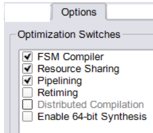
Implementation Options-&gt;Options
