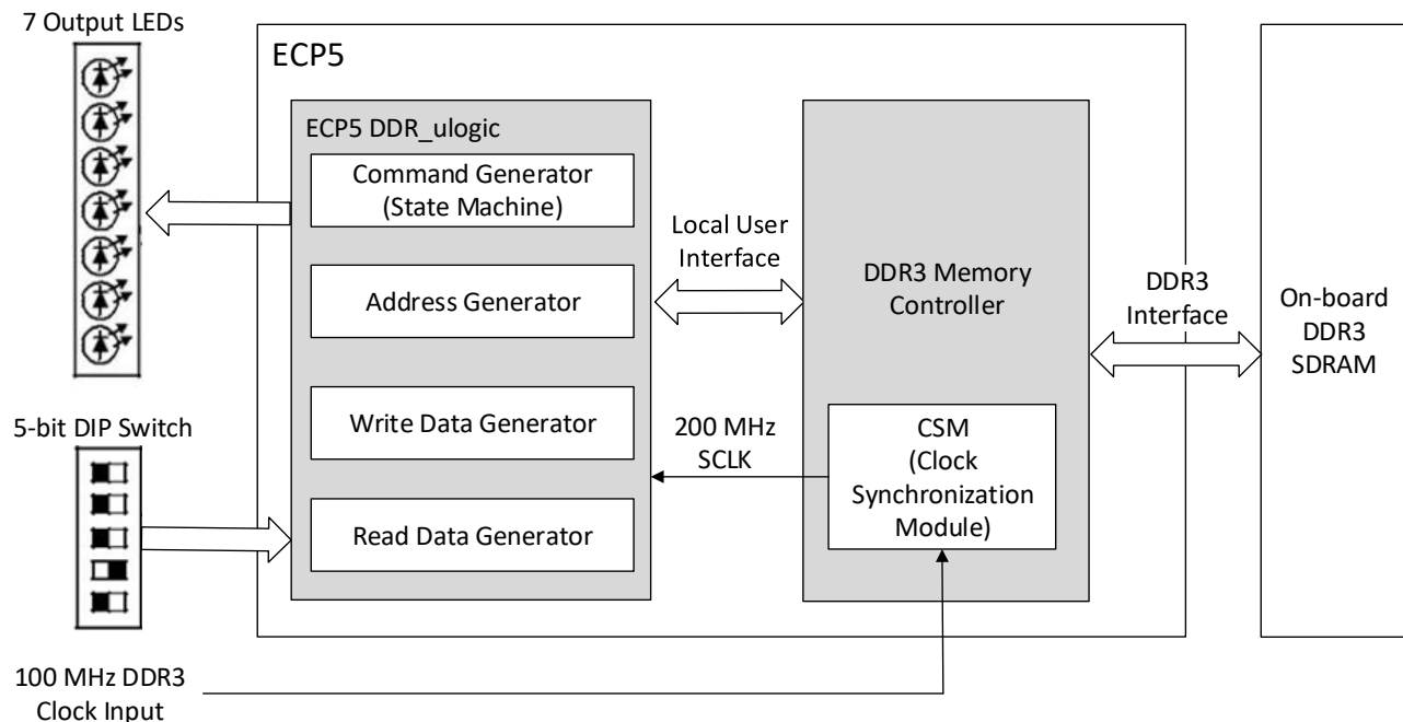
Figure 2.1. DDR3 Demo Block Diagram
