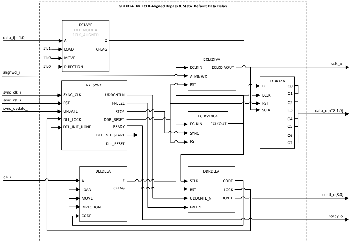
Figure 3.16. GDDR4_RX.ECLK.Aligned (Bypass & Static Default Data Delay)
