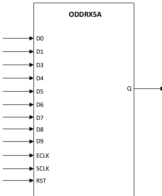
Figure 5.17. ODDRX5A Ports
