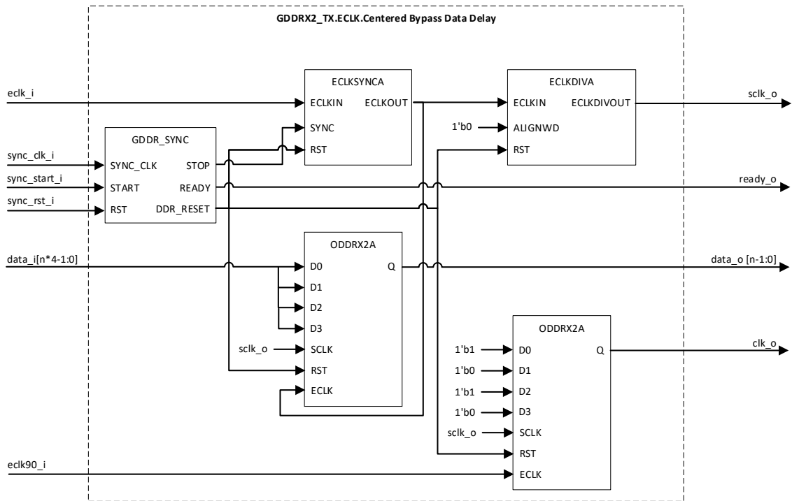
Figure 3.34. GDDR_X2_TX.ECLK.Centered (Bypass Data Delay)
