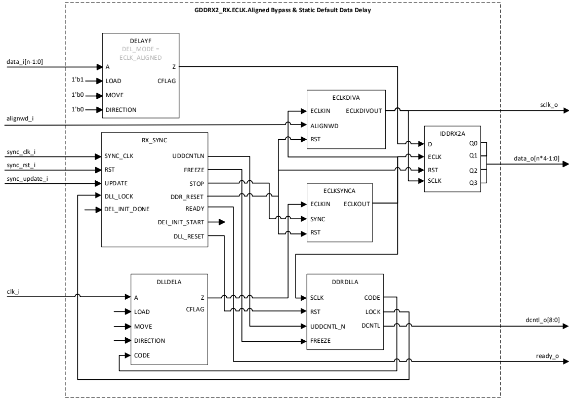
Figure 3.15. GDDR2_RX.ECLK.Aligned (Bypass & Static Default Data Delay)
