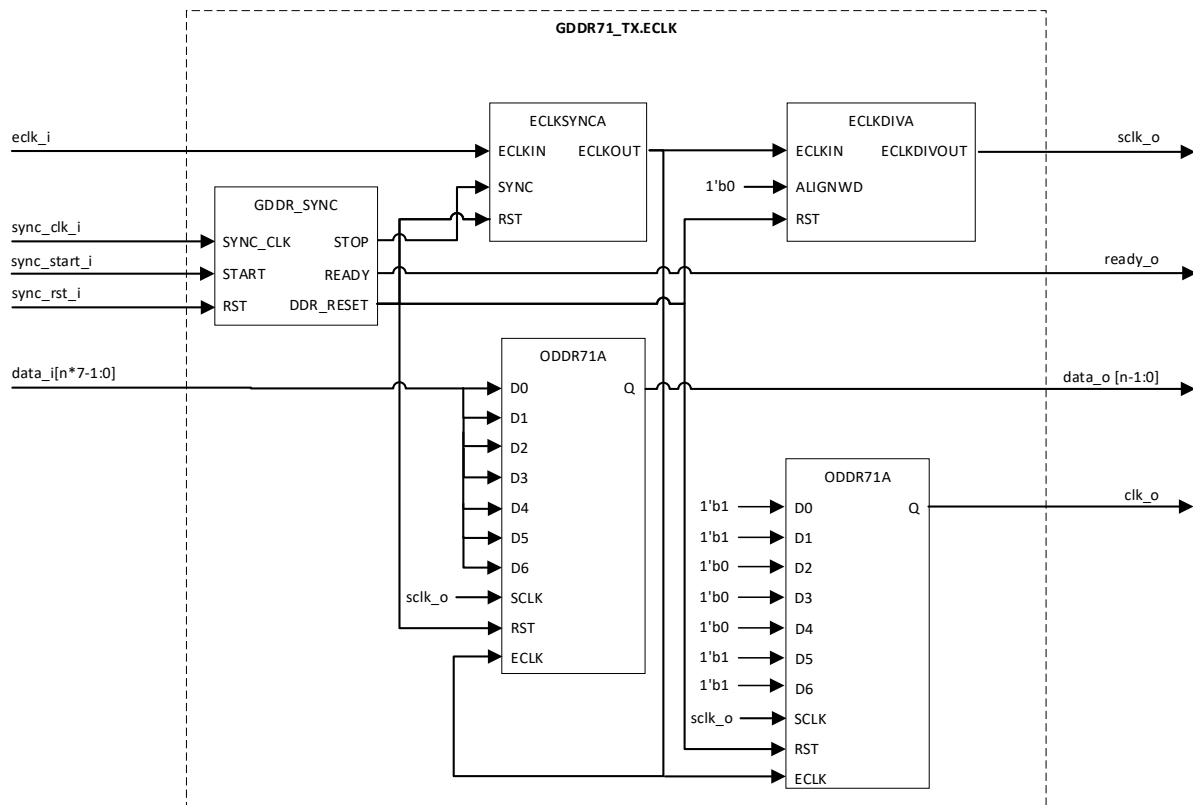
Figure 3.52. GDDR71_TX.ECLK
