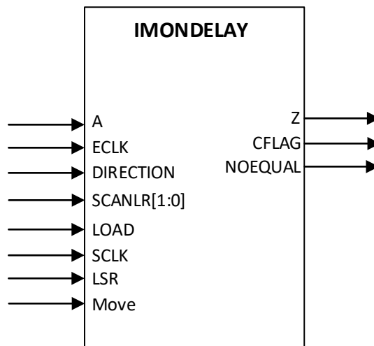
Figure 5.6. IMONDELAY Ports
