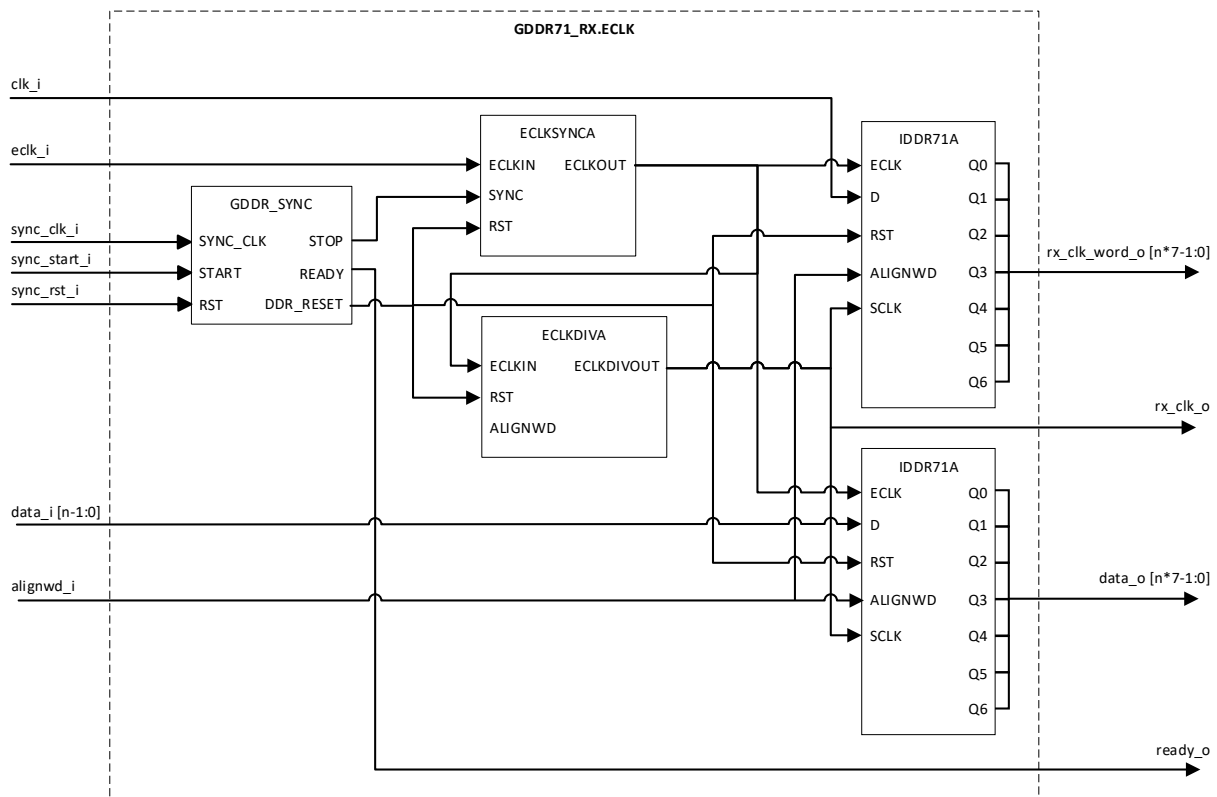
Figure 3.21. GDDR71_RX.ECLK
