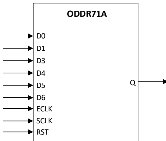
Figure 5.18. ODDR71A Ports
