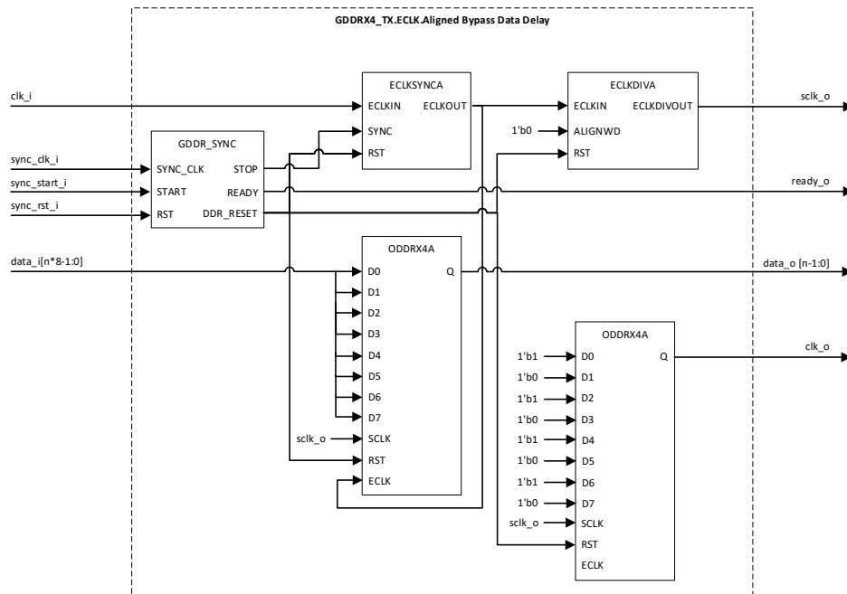
Figure 3.44. GDDR4_TX.ECLK.Aligned (Bypass Data Delay)
