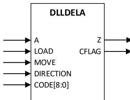
Figure 5.2. DLLDELA Ports
