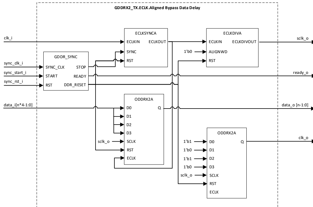
Figure 3.43. GDDR2_TX.ECLK.Aligned (Bypass Data Delay)
