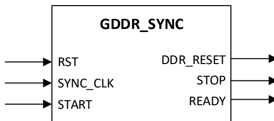
Figure 6.2. GDDR_SYNC Ports
