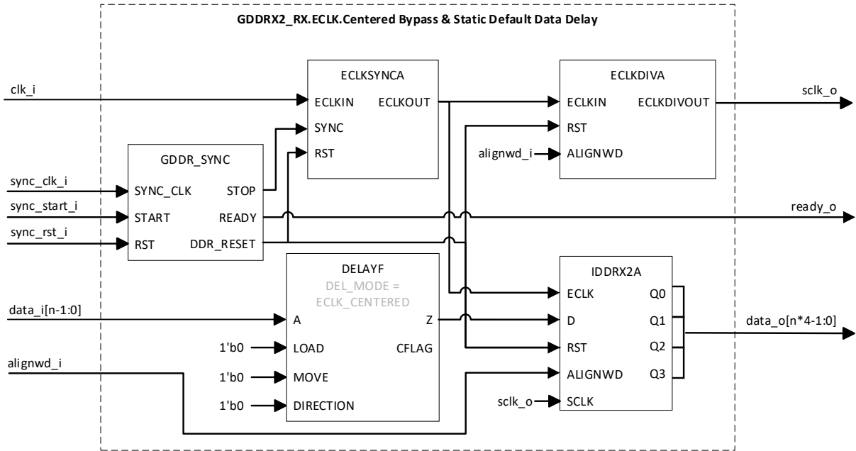
Figure 3.9. GDDR2_RX.ECLK.Centered (Bypass & Static Default Data Delay)
