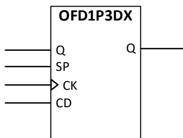
Figure 5.13. OFD1P3DX Ports
