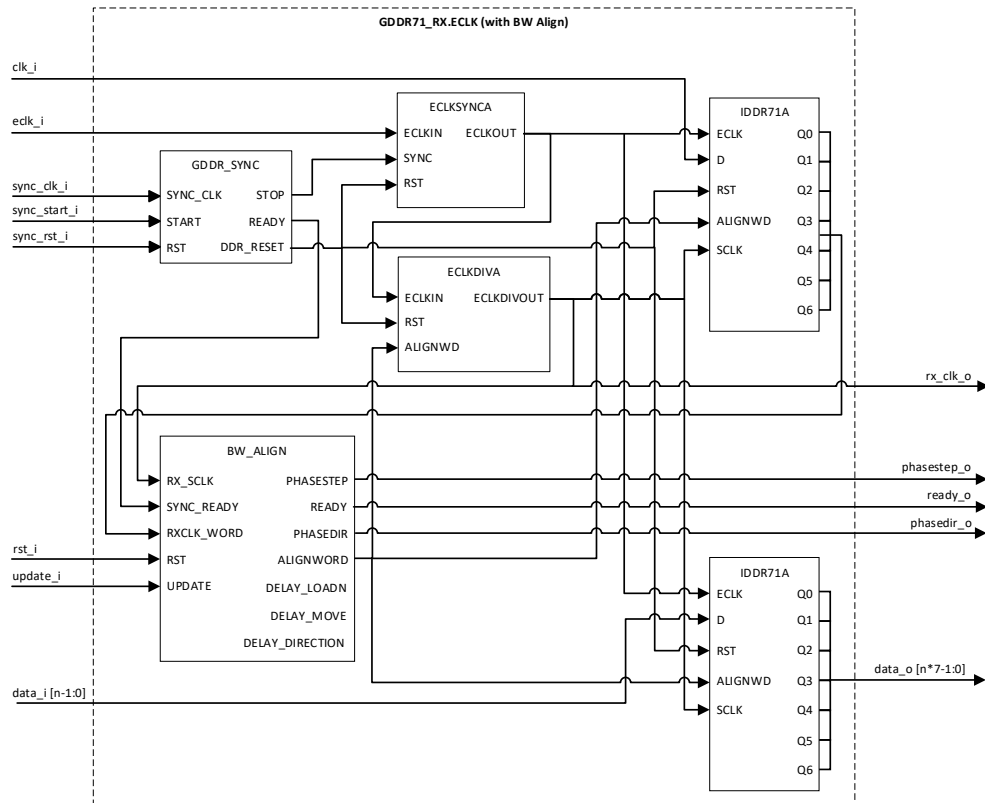
Figure 3.22. GDDR71_RX.ECLK (with Bit and Word Alignment)
