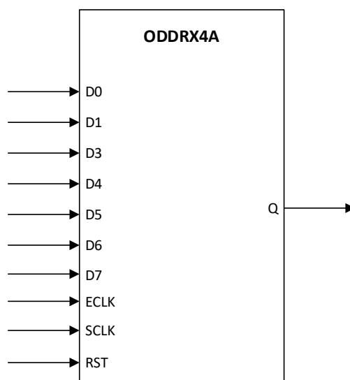
Figure 5.16. ODDRX4A Ports
