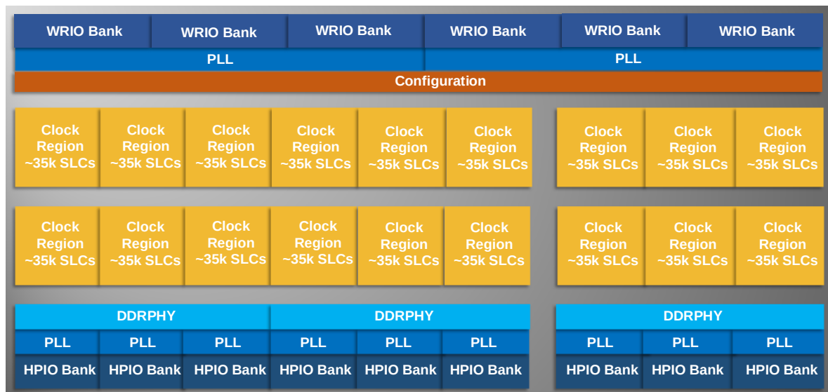
Figure 2.1. High-level Device Floorplan (LAV-AT-E70)
