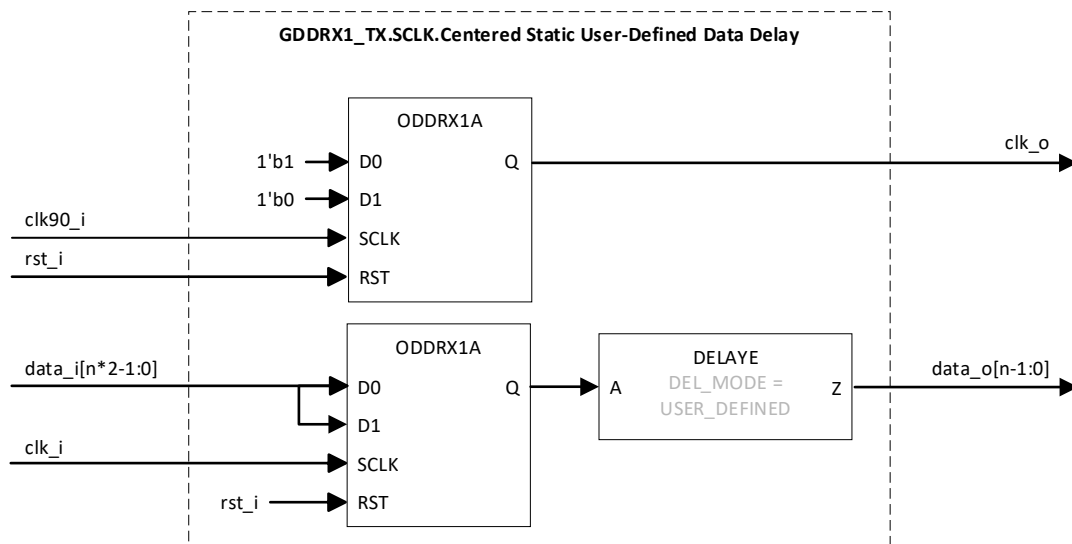
Figure 3.29. GDDR1_TX.SCLK.Centered (Static User-Defined Data Delay)
