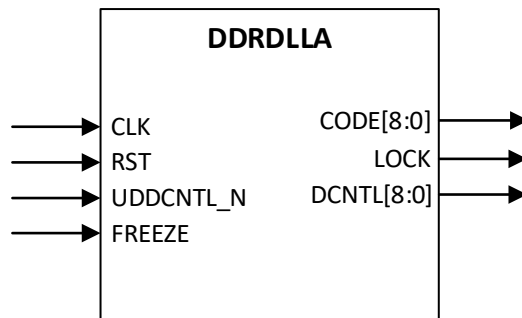
Figure 5.1. DDRDLLA Ports
