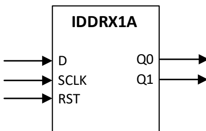
Figure 5.8. IDDRX1A Ports
