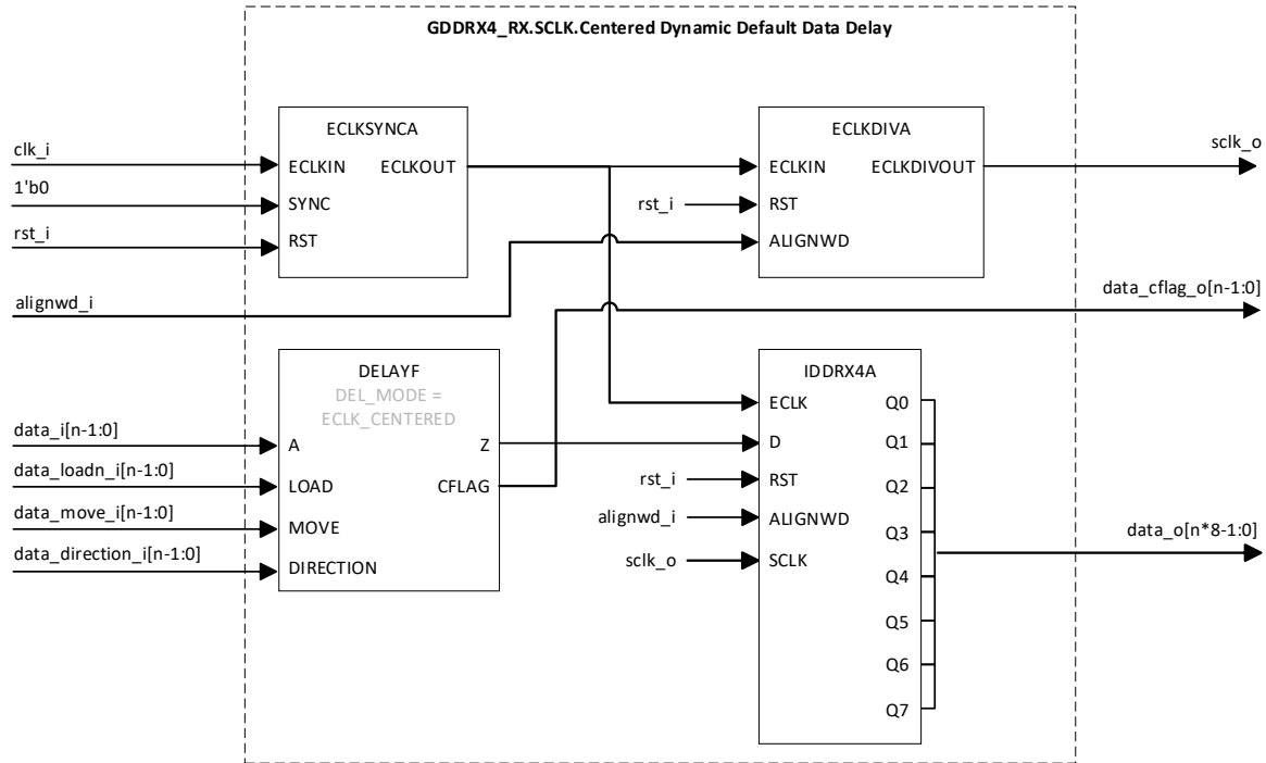
Figure 3.13. GDDR4_RX.ECLK.Centered (Dynamic Default Data Delay)
