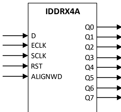
Figure 5.10. IDDRX4A Ports
