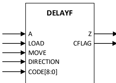
Figure 5.5. DELAYF Ports
