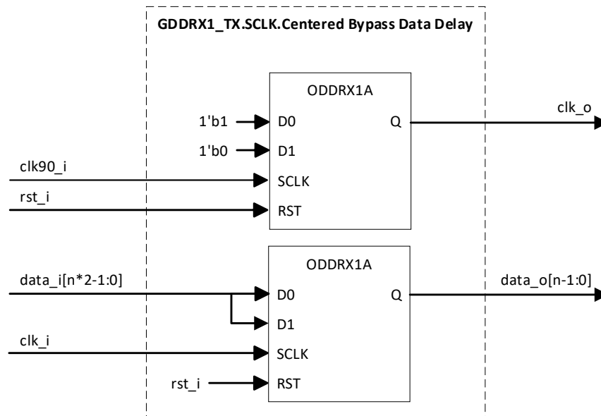
Figure 3.28. GDDR1_TX.SCLK.Centered (Bypass Data Delay)
