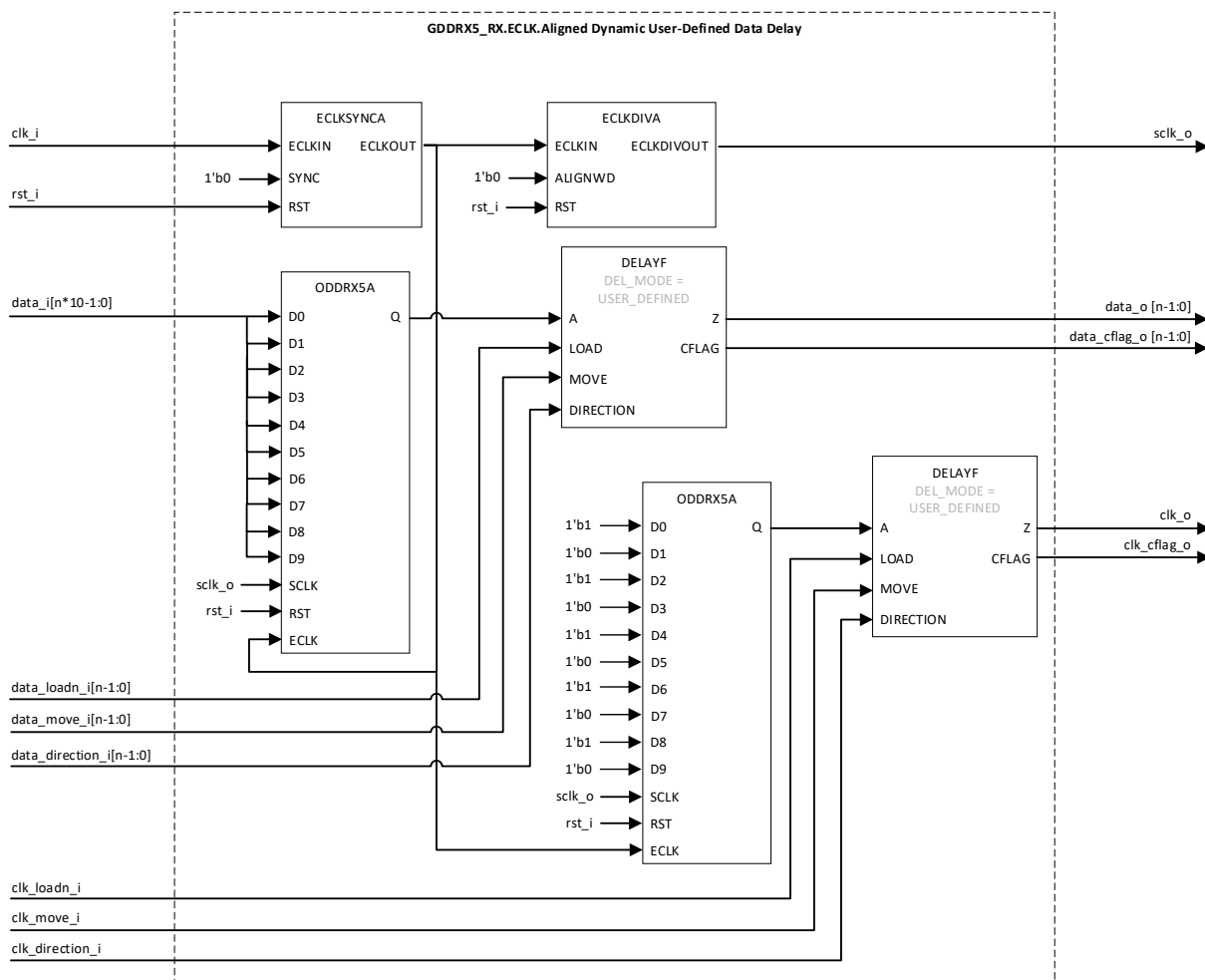
Figure 3.51. GDDR5_TX.ECLK.Aligned (Dynamic User-Defined Data Delay)
