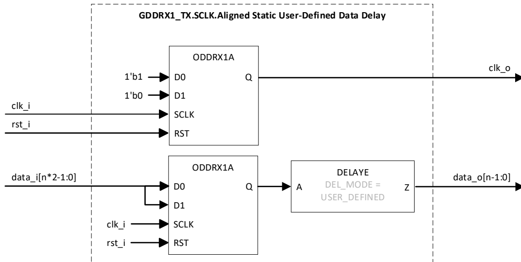
Figure 3.32. GDDRX1_TX.SCLK.Aligned (Static User-Defined Data Delay)
