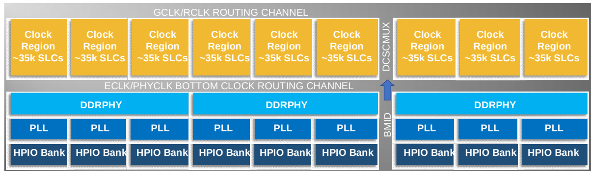
Figure 2.2. High-Level View of Clock Networks (LAV-AT-E/G/X70)
