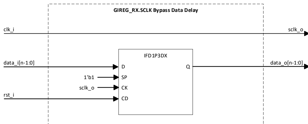
Figure 3.1. GIREG_RX.SCLK (Bypass Data Delay)
