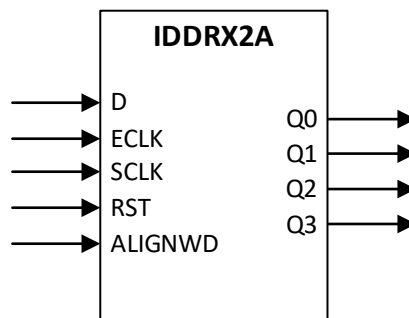
Figure 5.9. IDDRX2A Ports
