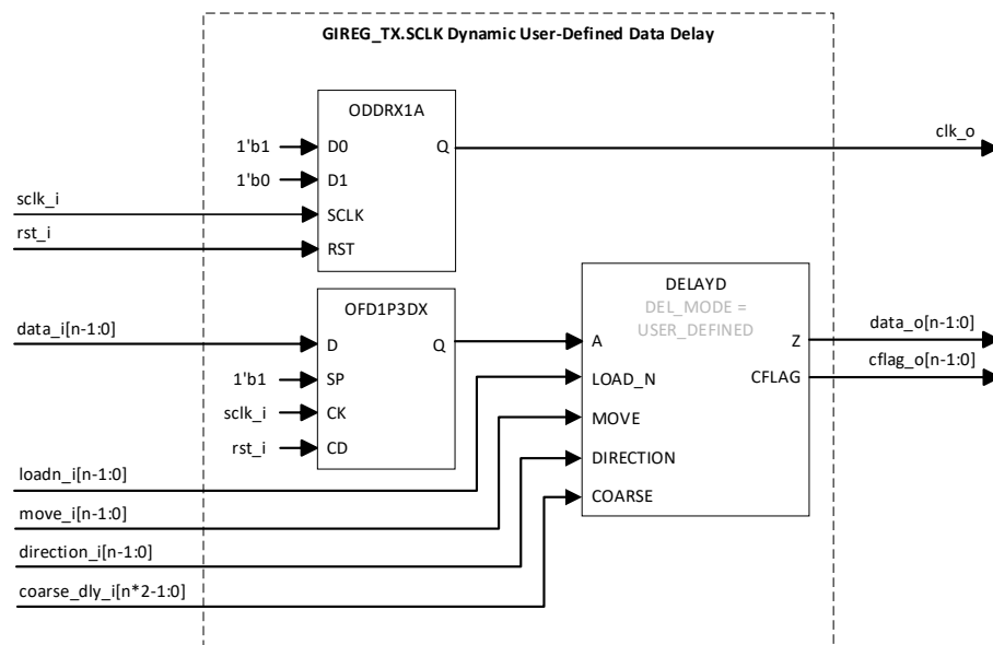
Figure 3.27. GIREG_TX.SCLK (Dynamic User-Defined Data Delay)
