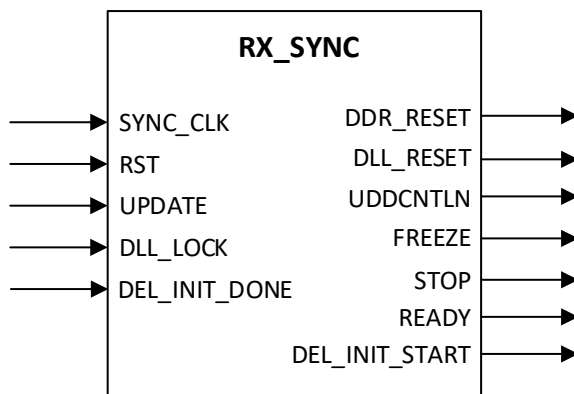
Figure 6.1. RX_SYNC Ports
