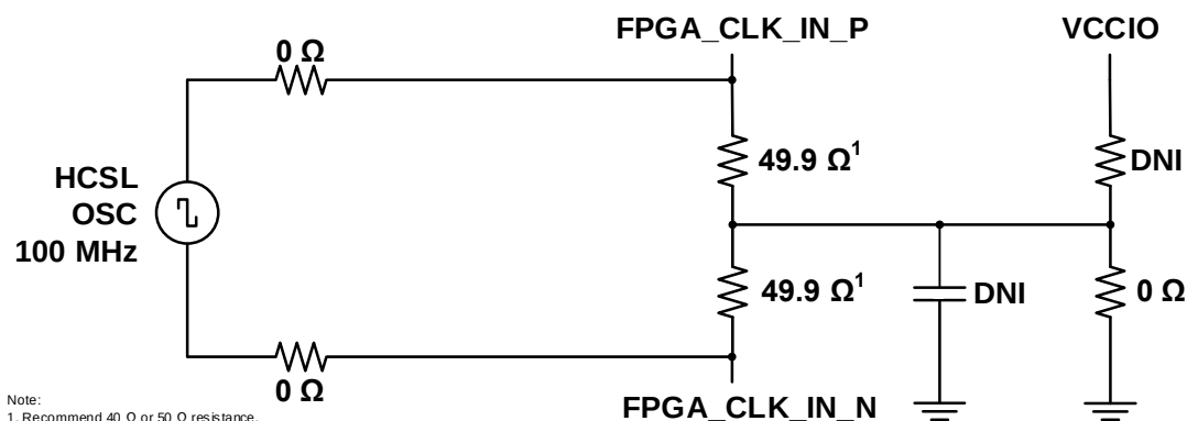
Figure 4.4. HSCL Oscillator on LVDS PCB Footprint
