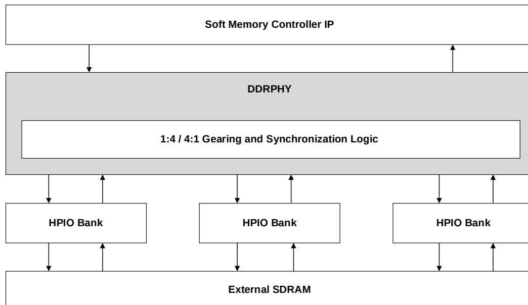
Figure 2.3. Lattice Avant DDRPHY Block Diagram
