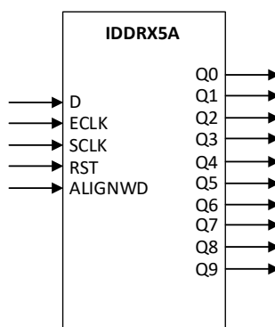
Figure 5.11. IDDRX5A Ports
