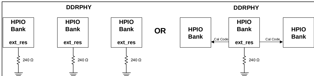
Figure 4.8. External Reference Resistor for SSTL (DDR3L)
