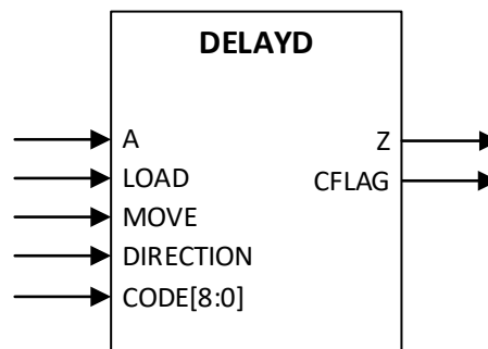
Figure 5.3. DELAYD Ports
