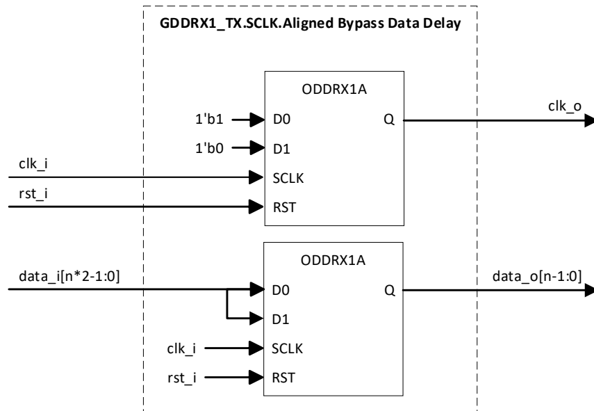
Figure 3.31. GDDRX1_TX.SCLK.Aligned (Bypass Data Delay)
