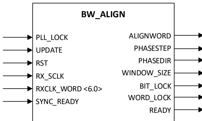
Figure 6.3. BW_ALIGN Ports
