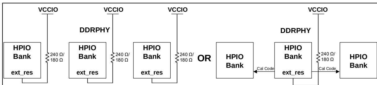
Figure 4.12. External Reference Resistor for LVSTL_I/LVSTL_II (LPDDR4)
