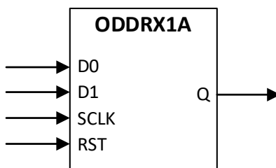
Figure 5.14. ODDRX1A Ports
