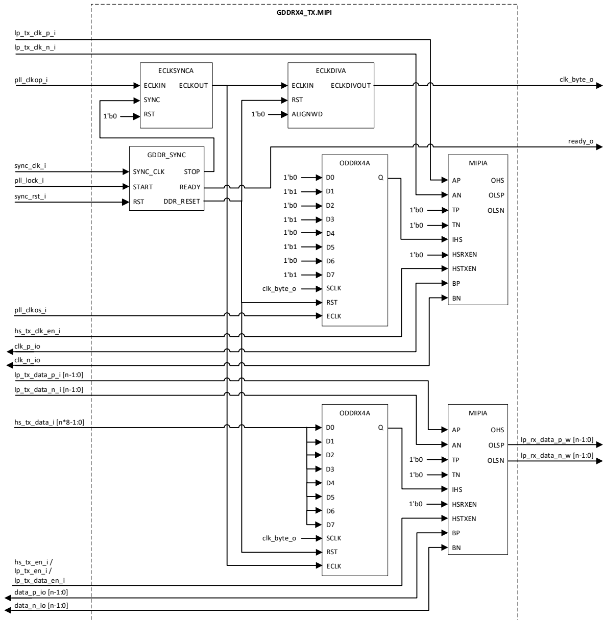
Figure 3.53. GDDR4_TX.MIPI
