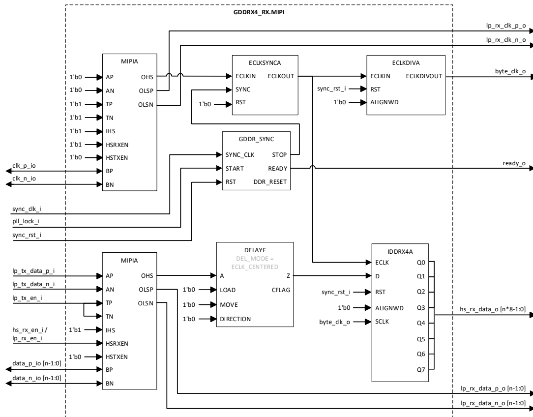
Figure 3.24. GDDR4_RX.MIPI
