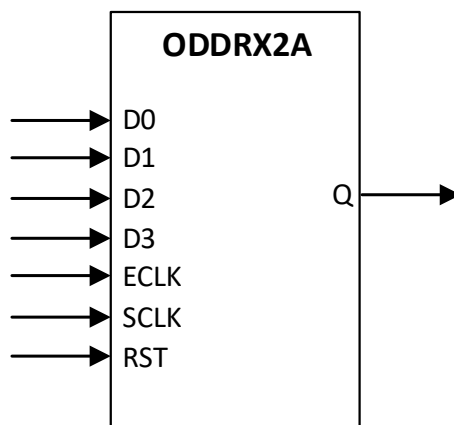
Figure 5.15. ODDRX2A Ports
