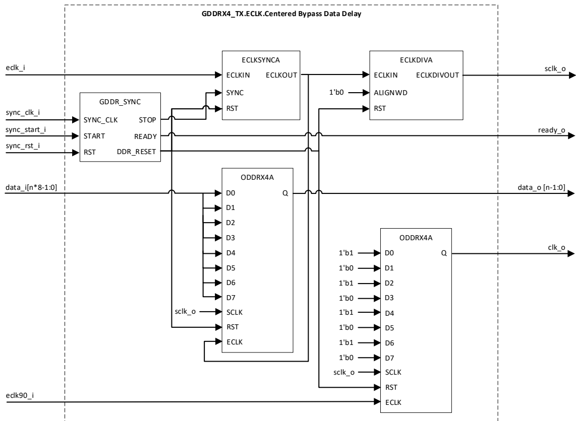
Figure 3.35. GDDR_X4_TX.ECLK.Centered (Bypass Data Delay)
