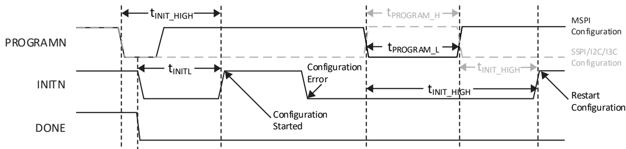
Figure 3.22. Slave SPI/I²C/I³C Wake-Up Timing
