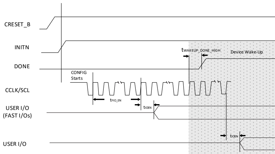
Figure 3.22. Slave SPI/I²C/I³C Wake-Up Timing
