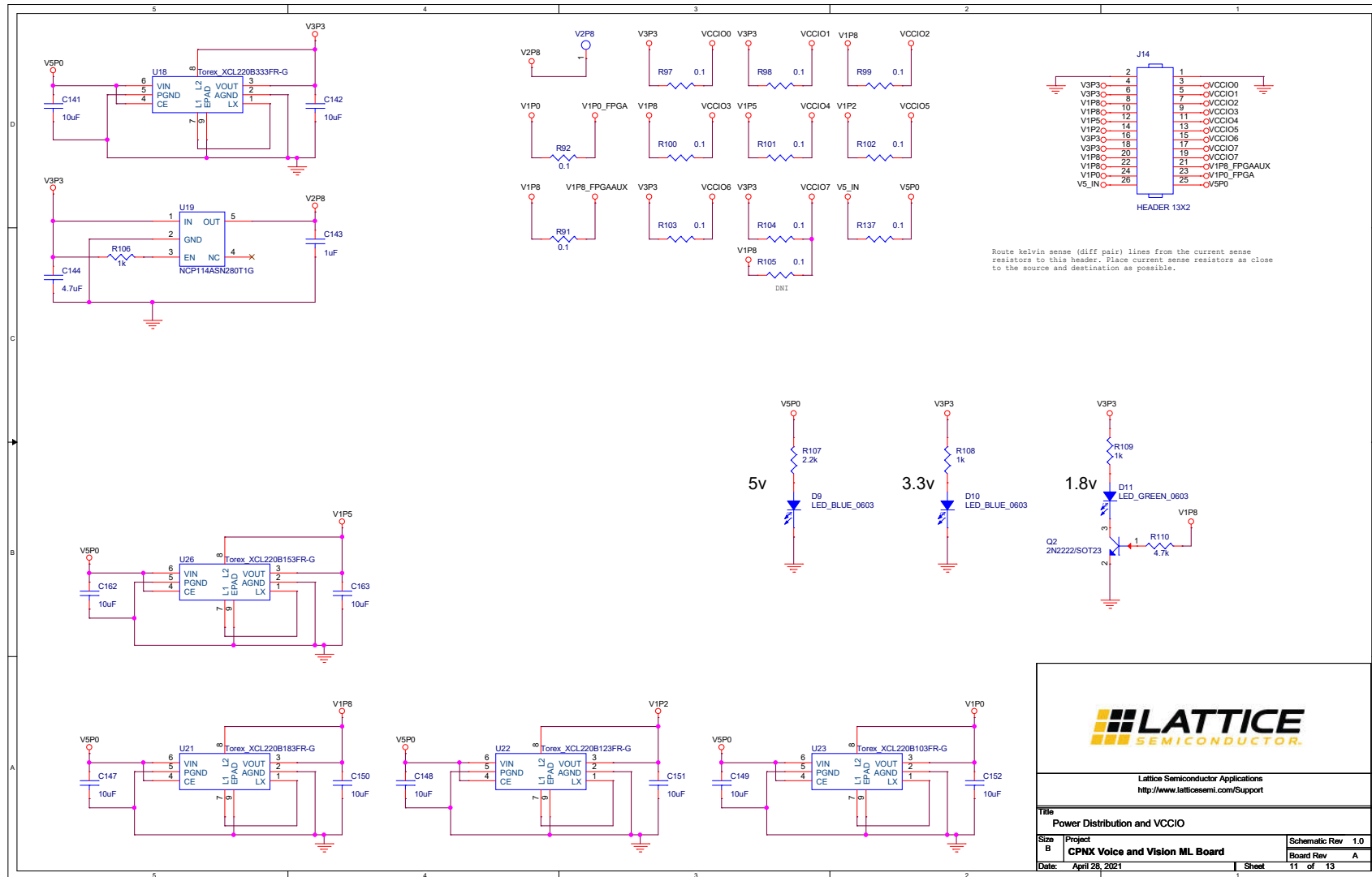
Figure A.11. Power Distribution and VCCIO
