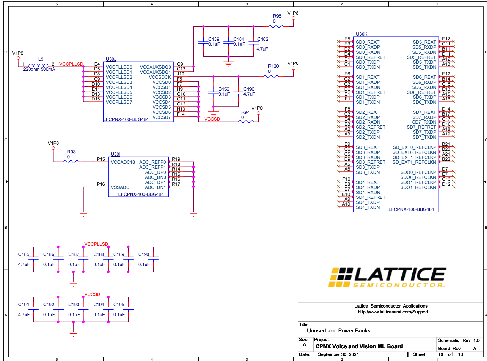
Figure A.10. Unused and Power Banks
