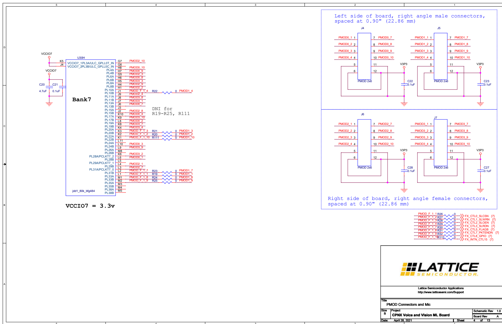
Figure A.4. PMOD Connectors and Mic
