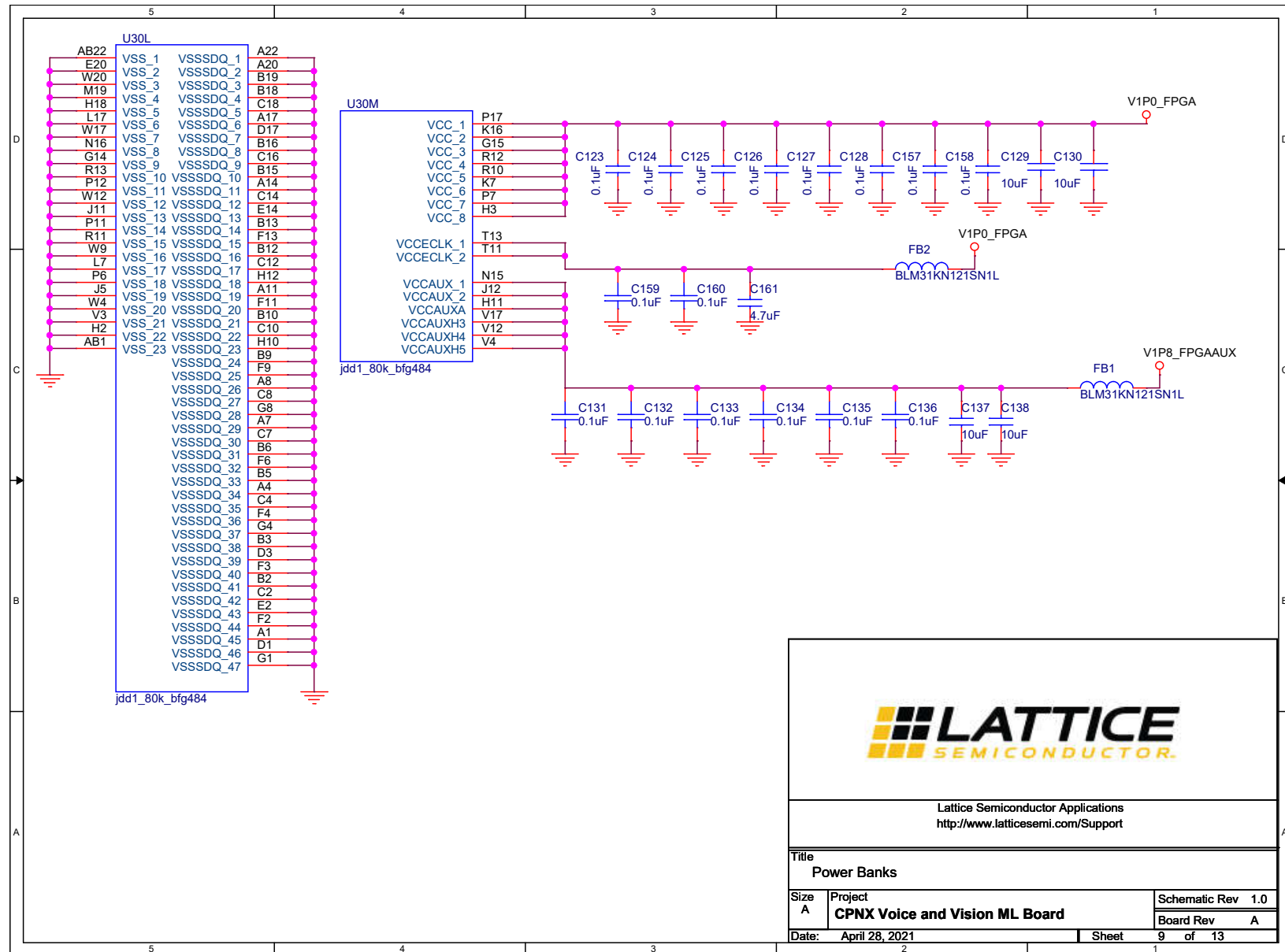
Figure A.9. Power Banks
