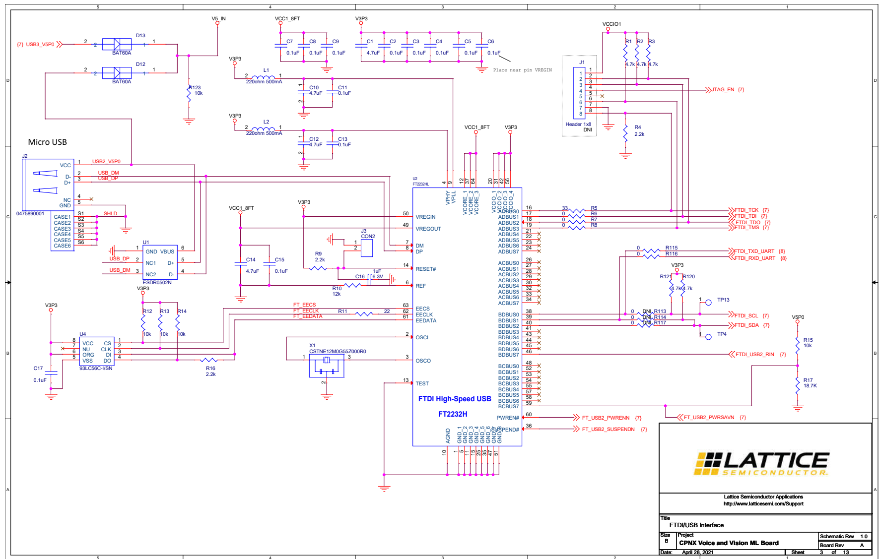
Figure A.3. FTDI/USB Interface
