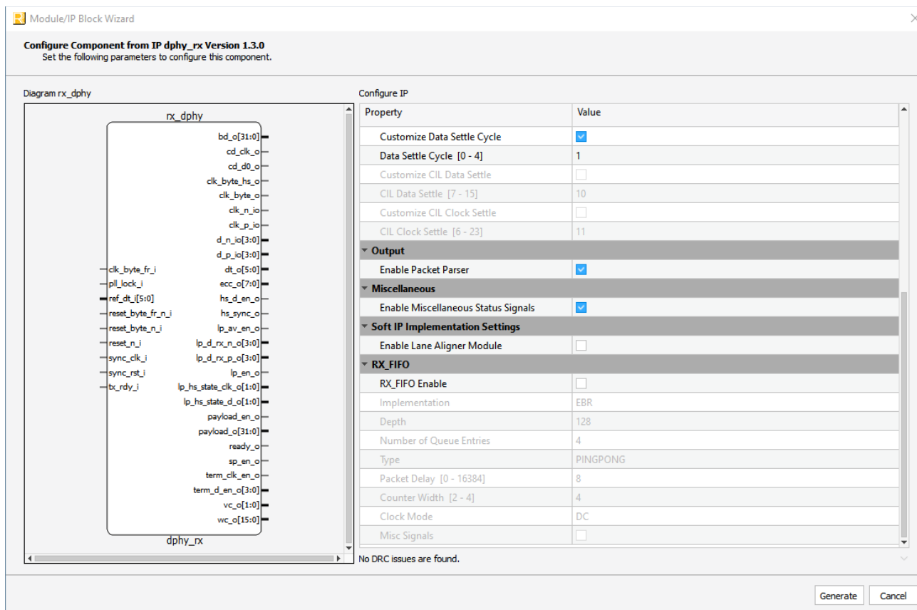
Figure 3.2. rx_dphy IP Creation 2 in Lattice Radiant Software
