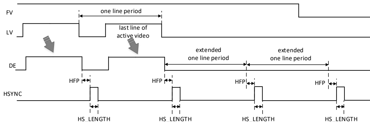
Figure 3.8. HSYNC Generation
