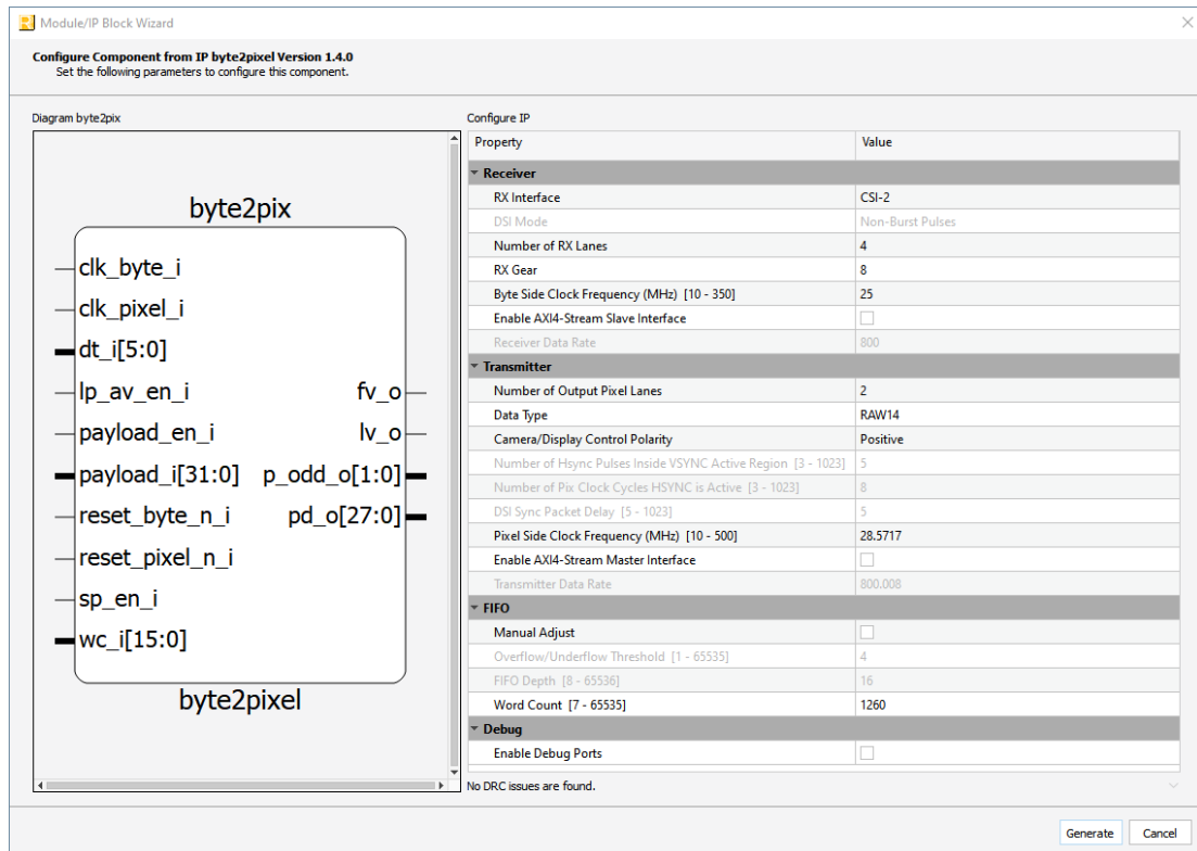
Figure 3.3. byte2pixel IP Creation in Lattice Radiant
