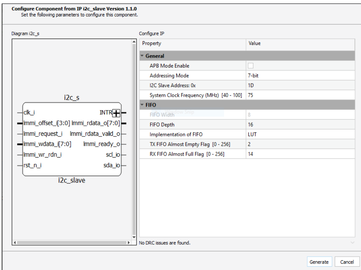
Figure 3.17. I 2 C IP Creation in Lattice Radiant
