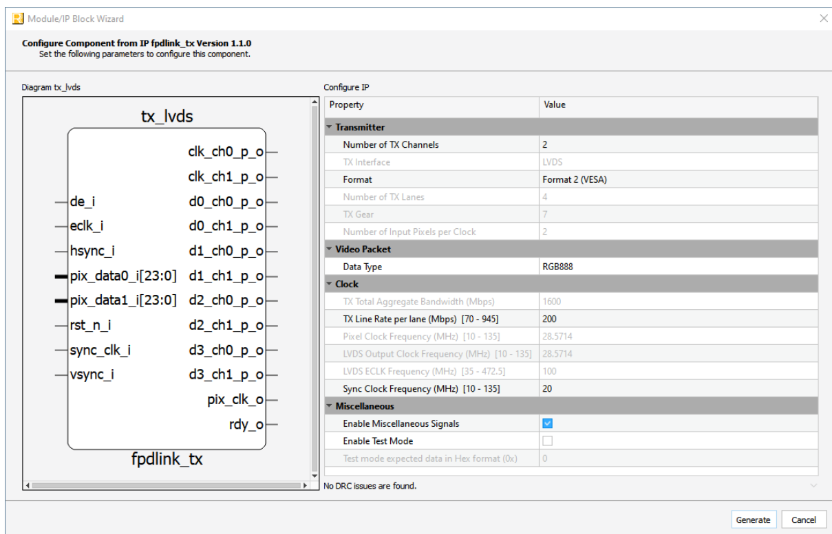
Figure 3.12. tx_dphy IP Creation in Lattice Radiant
