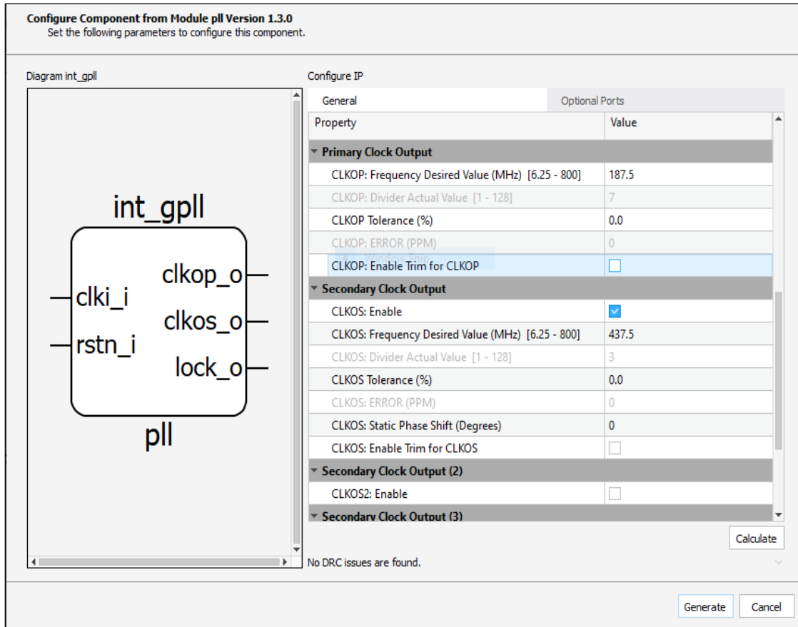
Figure 3.16. GPLL IP Creation 2 in Lattice Radiant
