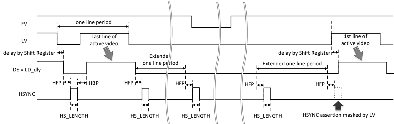
Figure 3.9. HSYNC Masked by LV
