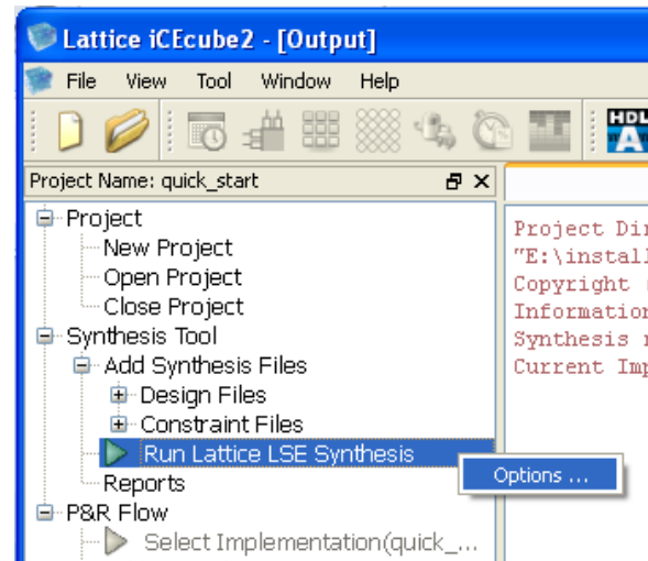
Figure 3-6 : Open LSE Tool Options Dialog Box
