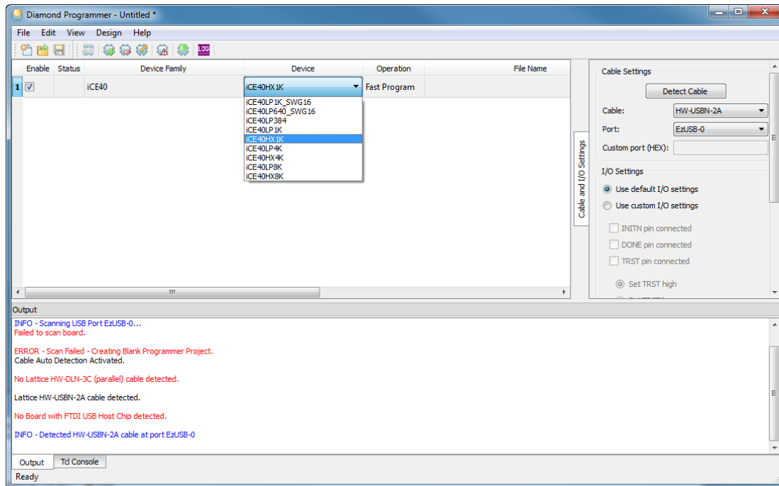
Figure 2-23 : Choosing iCE40HX1K Device
