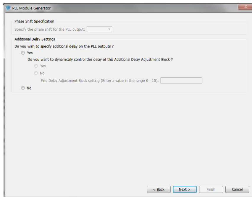
Figure 3-18: iCE40 PLL - Additional Delay and Phase Shift Options
