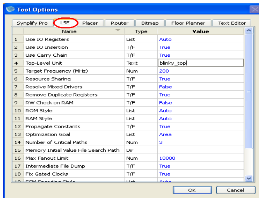
Figure 3-7 : LSE Tool Options
