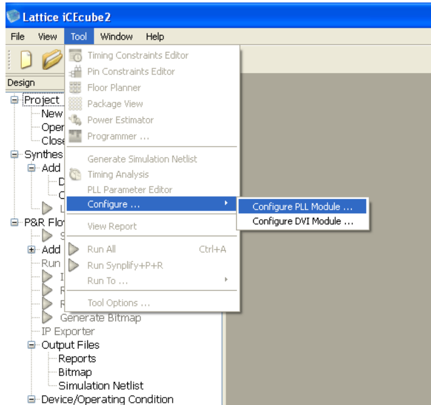
Figure 3-12: Launching the PLL Module Generator
