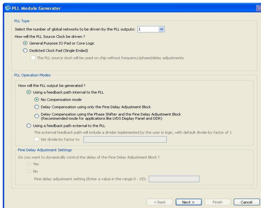
Figure 3-17: iCE40 PLL - Selecting PLL Type and Operation Modes
