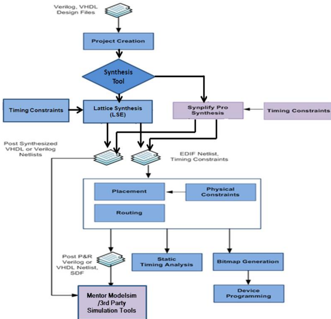
Figure 1-1: The iECube2 Design Flow
