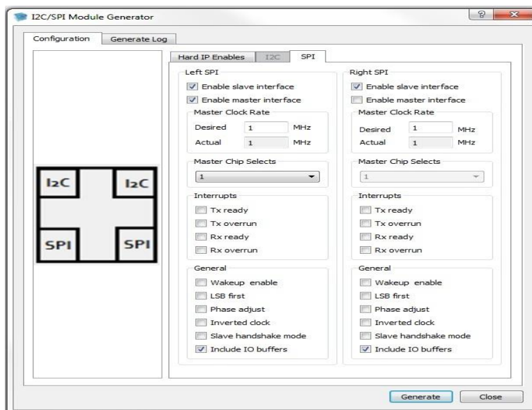
Figure 3-26: Configure Left/Right SPI hard IP.
