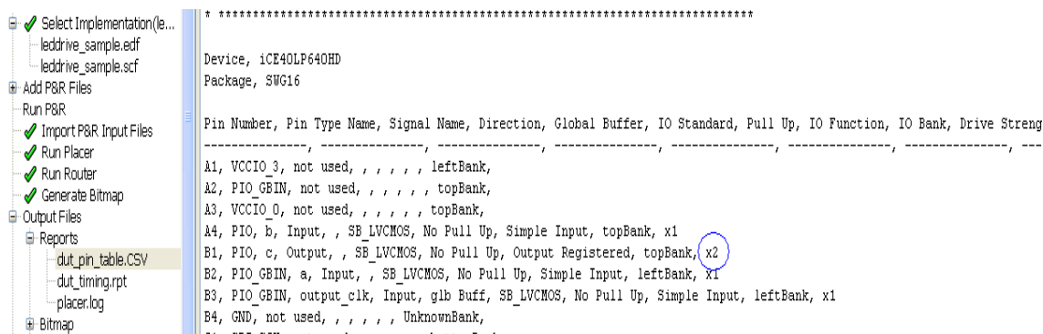
Figure 11-1 : Drive Strength Display in Pin Table CSV File.
