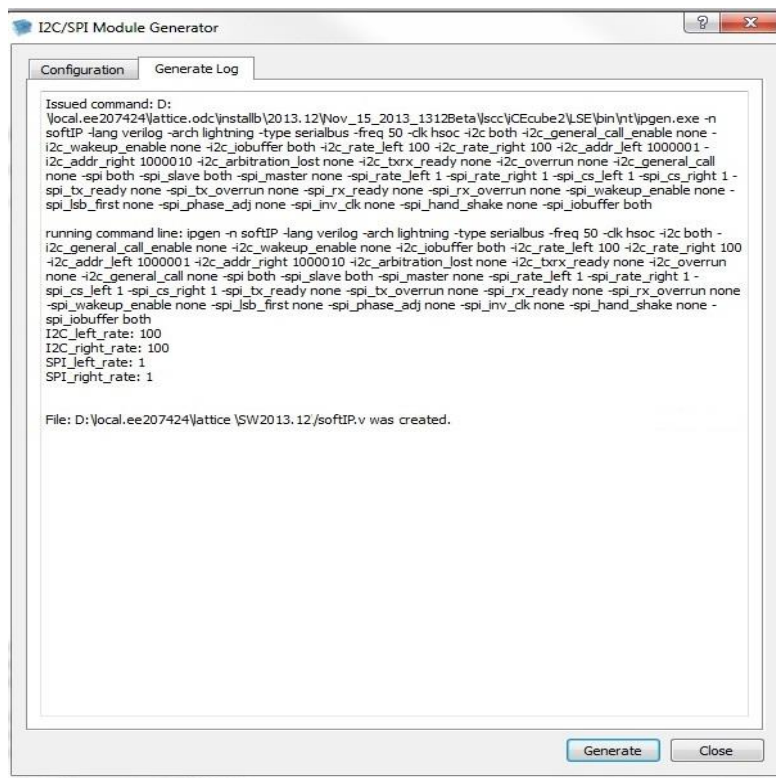
Figure 3-27: I2C/SPI soft IP module generation.
