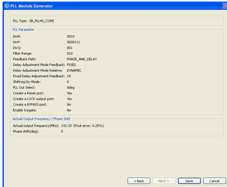
Figure 3-20 : PLL Summary
