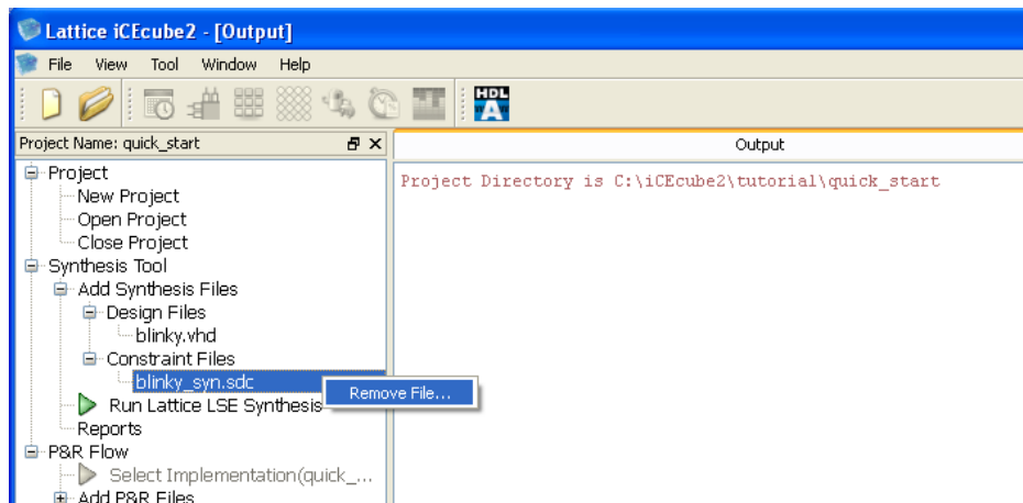
Figure 3-3 : Removing Files from the Design Project
