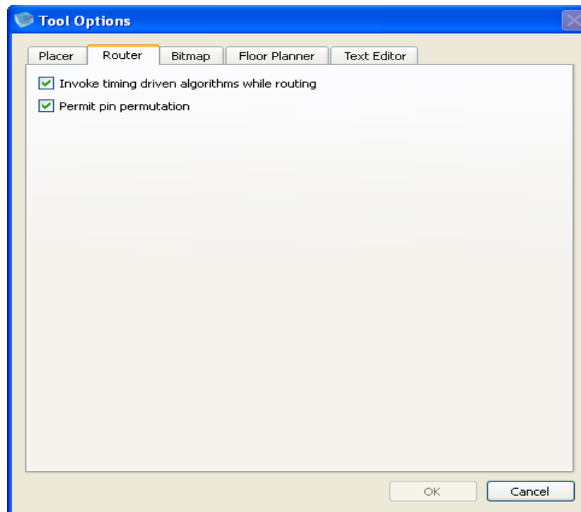
Figure 5-2 : Router Options
