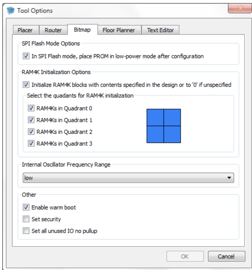
Figure 5-20 : Bitmap Options
