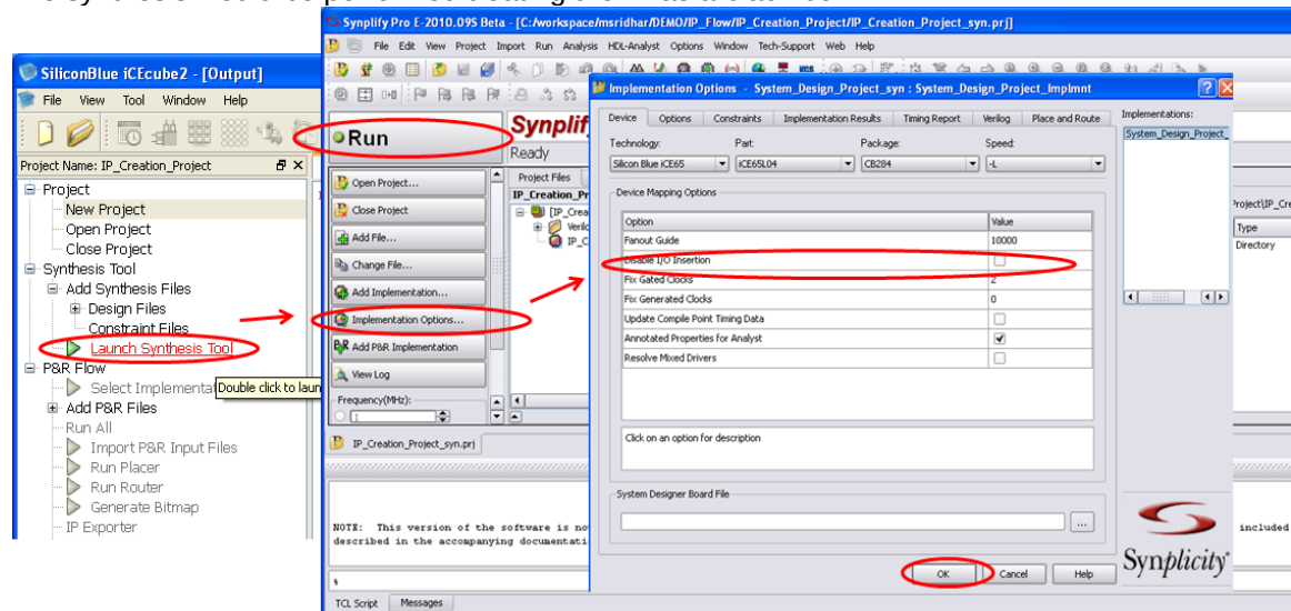
Figure 8-9 Run Synthesis
