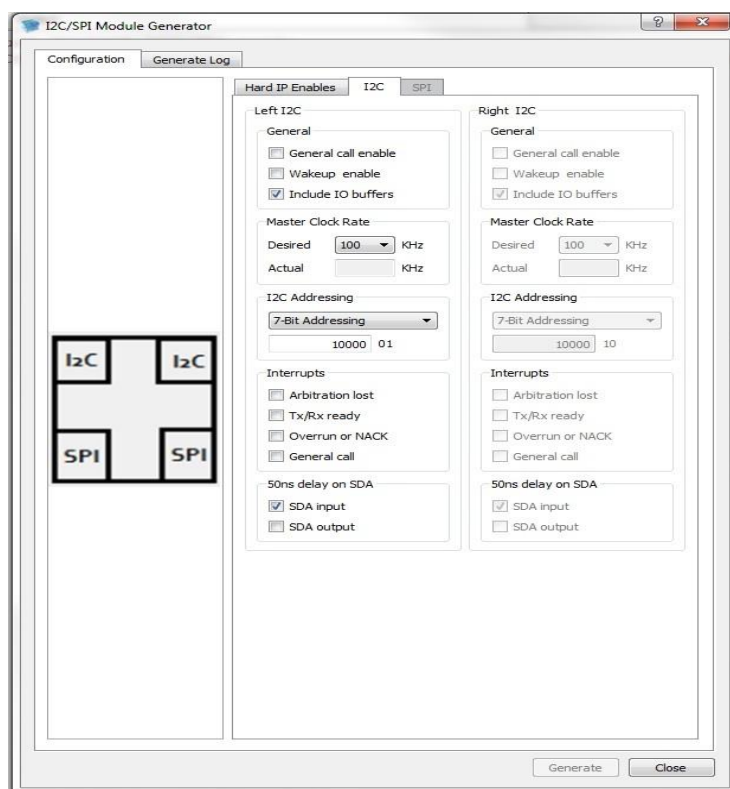
Figure 3-25: Configure Left/Right I2C hard IP.
