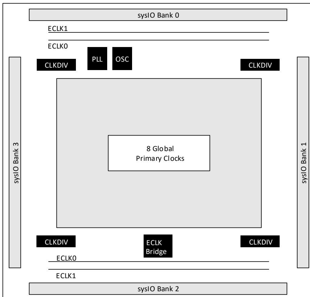
Figure 3.1. Mach-NX Clocking Structure
