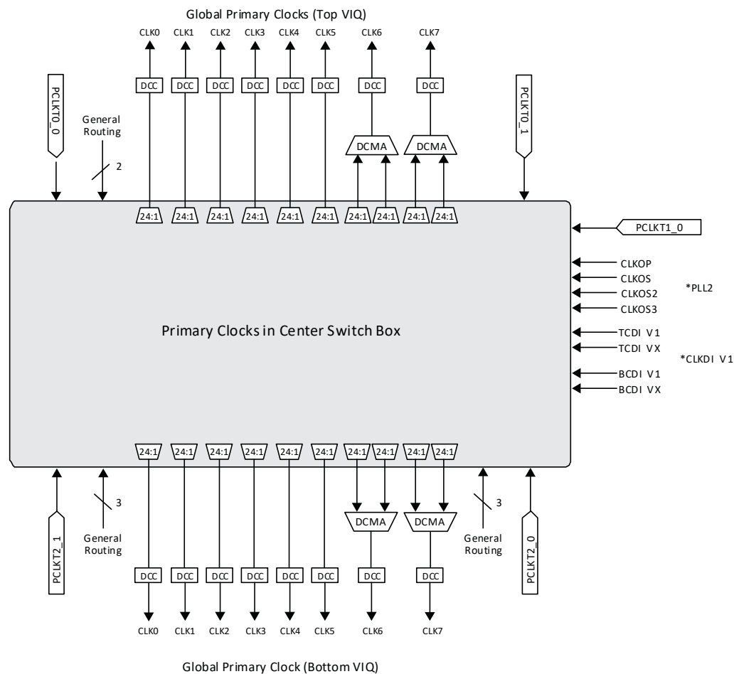
Figure A.1. Mach-NX Primary Clock Sources and Distribution
