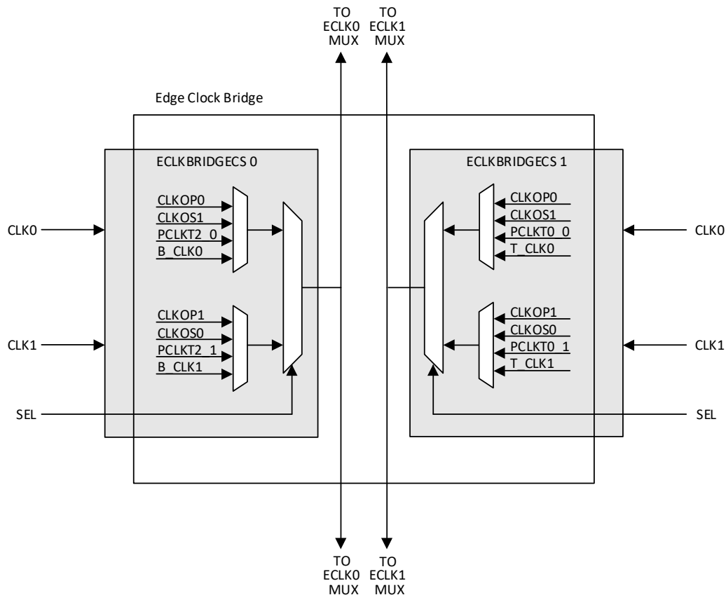
Figure B.2. Mach-NX Edge Clock Bridge Sources and Connectivity
