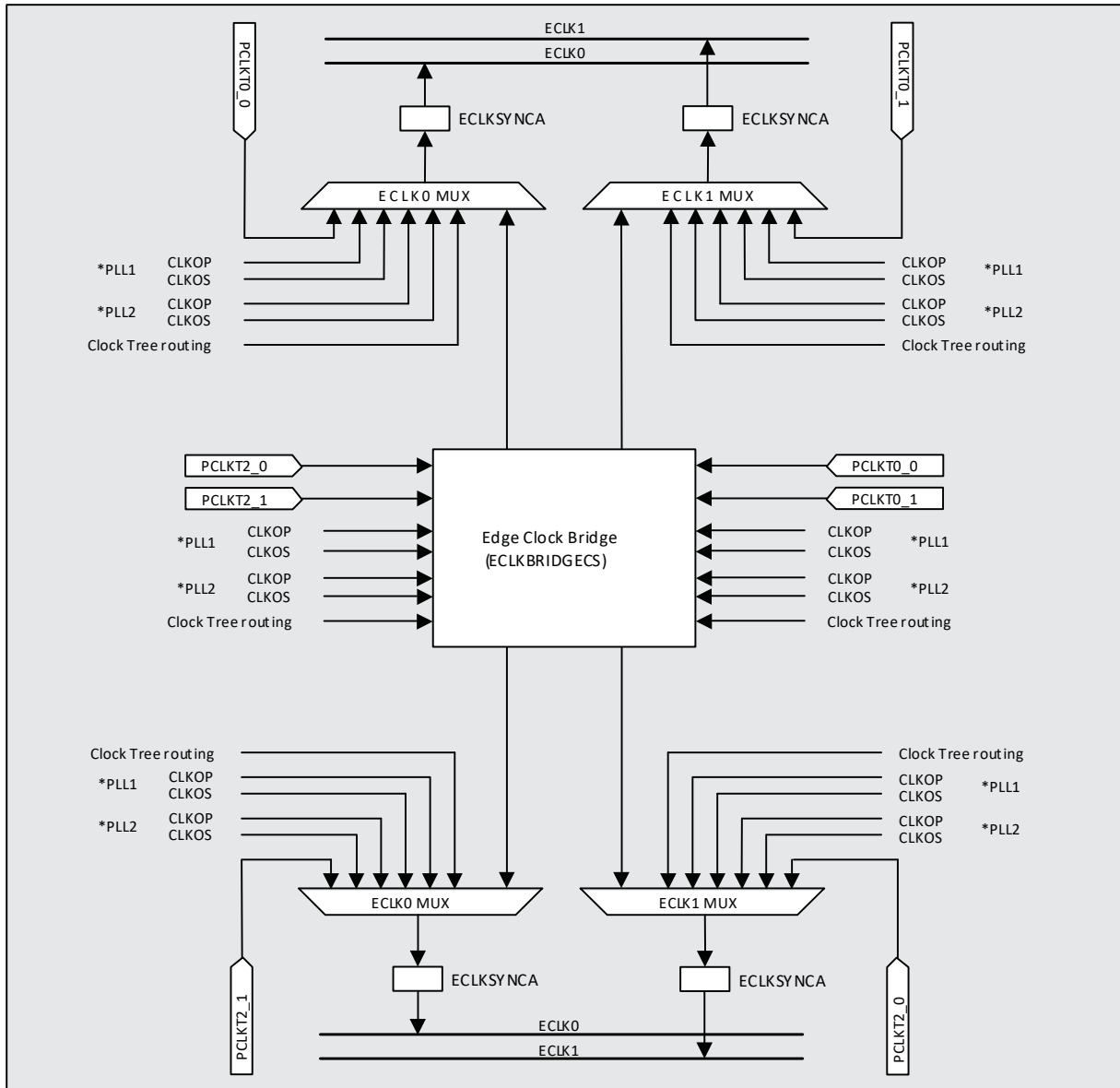
Figure B.1. Mach-NX Edge Clock Sources and Connectivity
