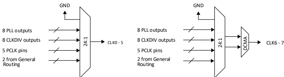
Figure A.2. Mach-NX Primary Clock Muxes
