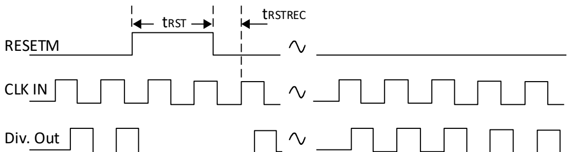
Figure 10.2. RST and RESETM Timing Diagram
