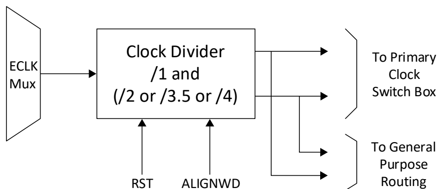
Figure 9.1. Mach-NX Clock Divider
