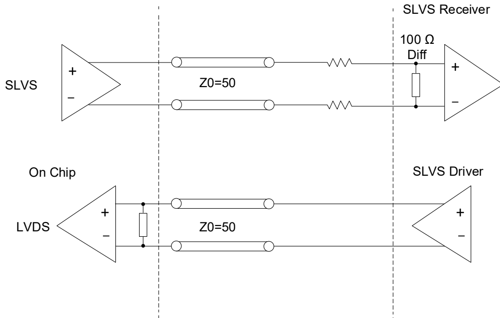
Figure 4.5. SLVS Interface
