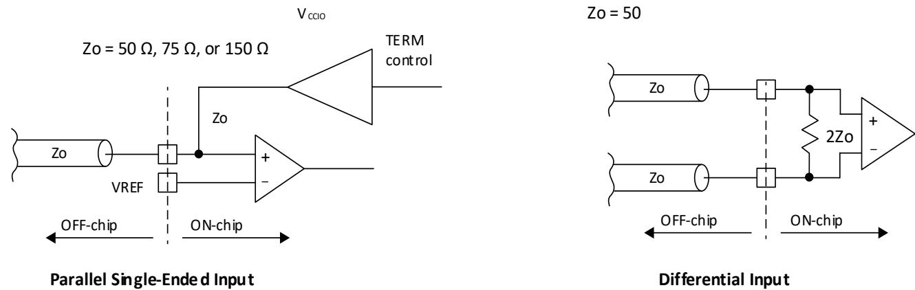
Figure 3.1. On-chip Termination
