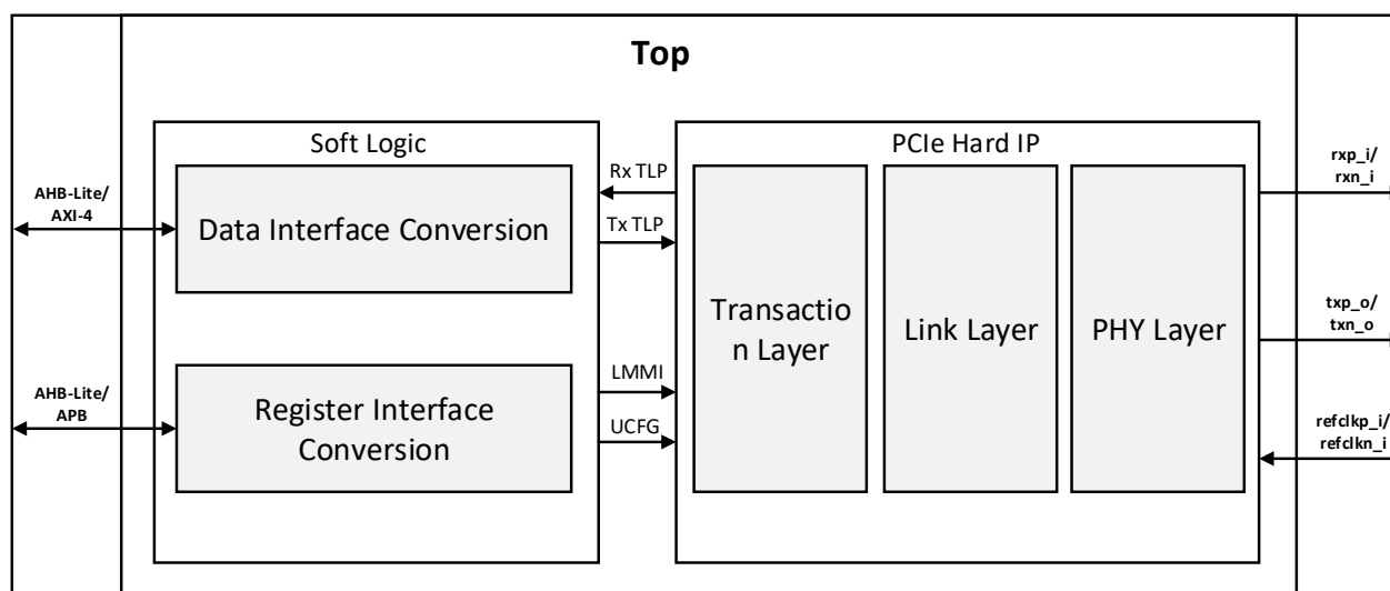
Figure 2.35. PCIe Soft IP Wrapper
