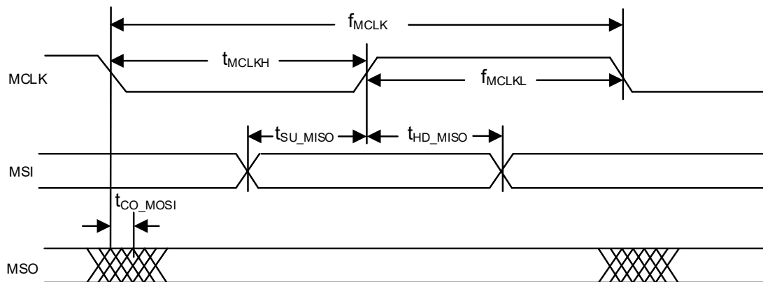
Figure 3.19. Master SPI Configuration Timing
