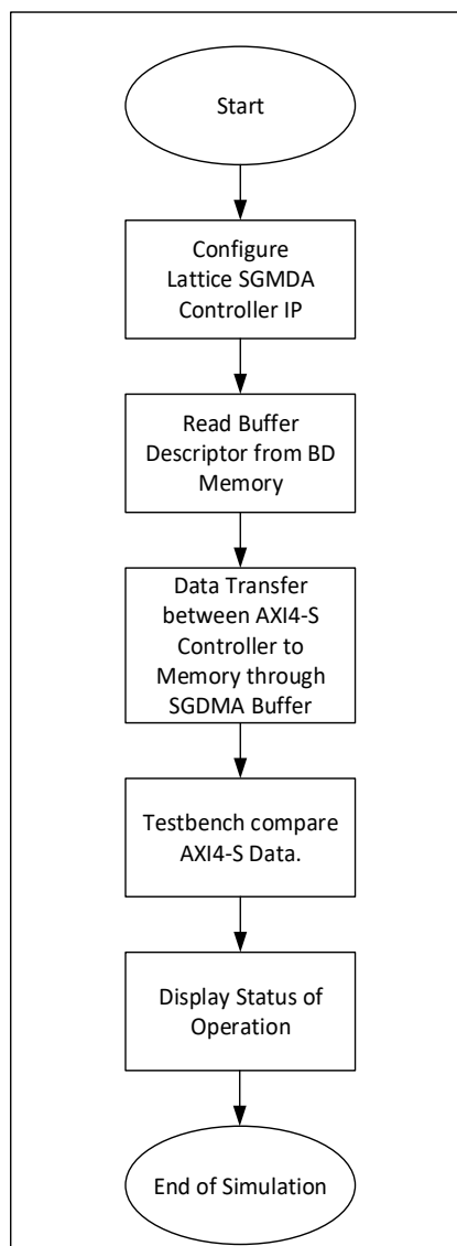
Figure 6.9. SGDMA Controller Example Design Simulation Flow
