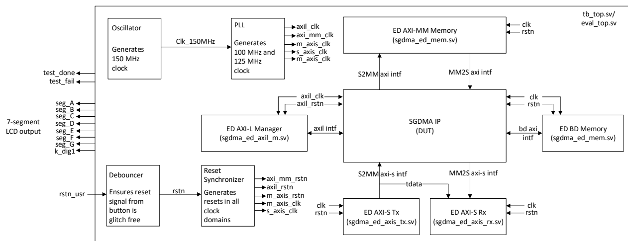
Figure 6.3. SGDMA Controller Example Design Block Diagram with Separate AXI-S Transmitter and Receiver Clock Domains Enabled and AXI-4Lite CSR Access Interface Selected
