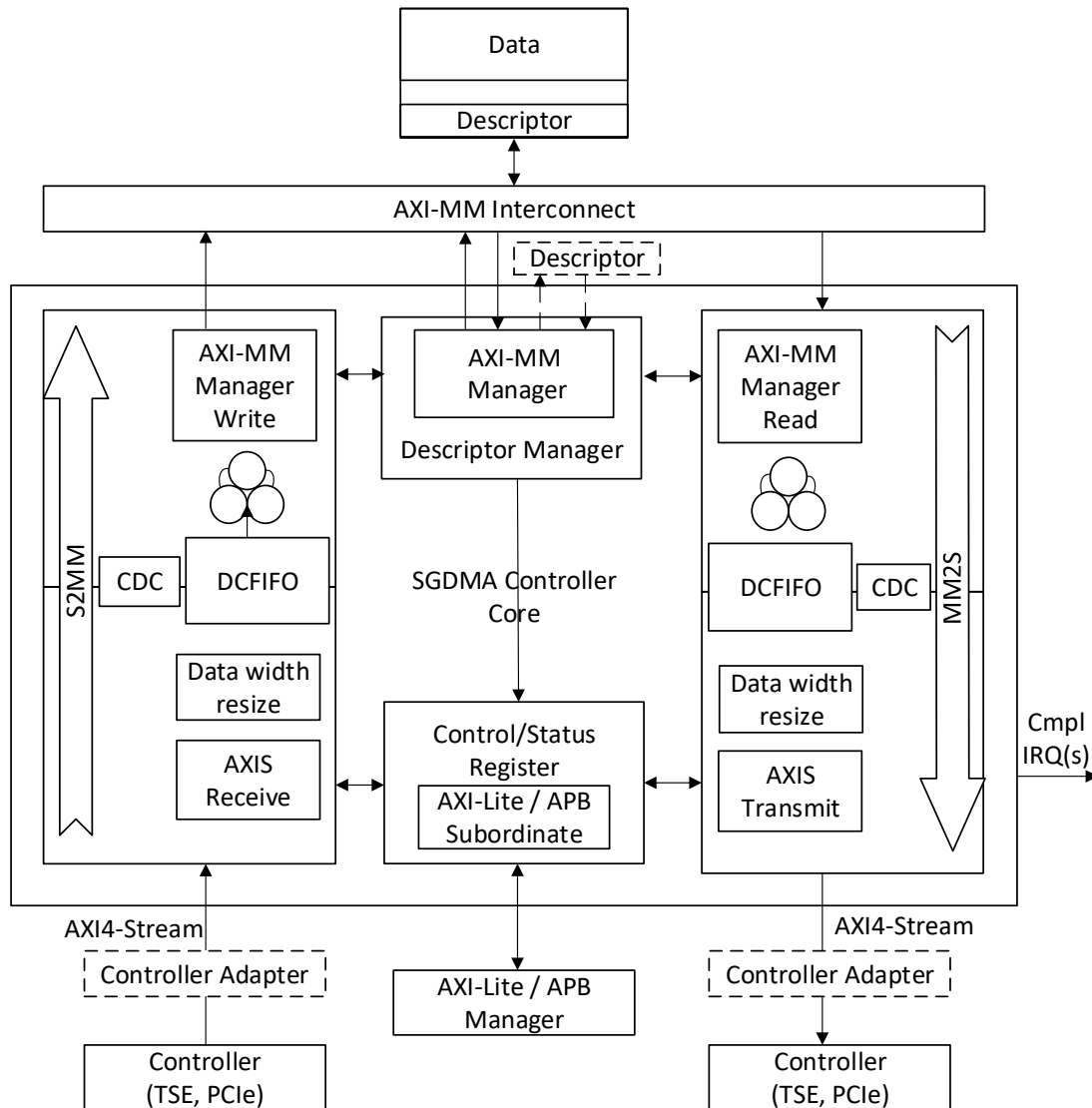
Figure 2.2. SGDMA Controller Core Block Diagram with Separate Clock Domains for AXI-S Transmitter and Receiver Enabled
