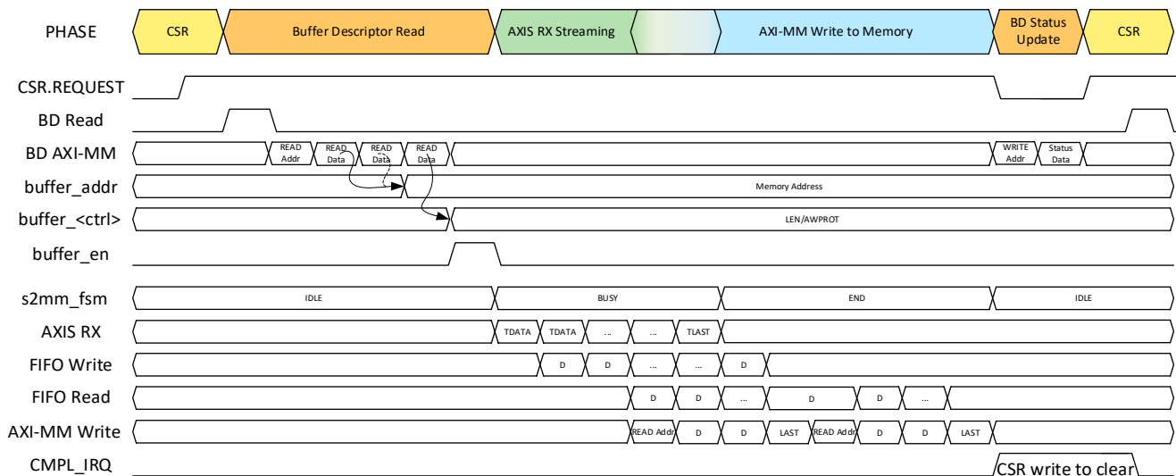
Figure 2.5 SGDMA Controller IP S2MM Operation Phase
