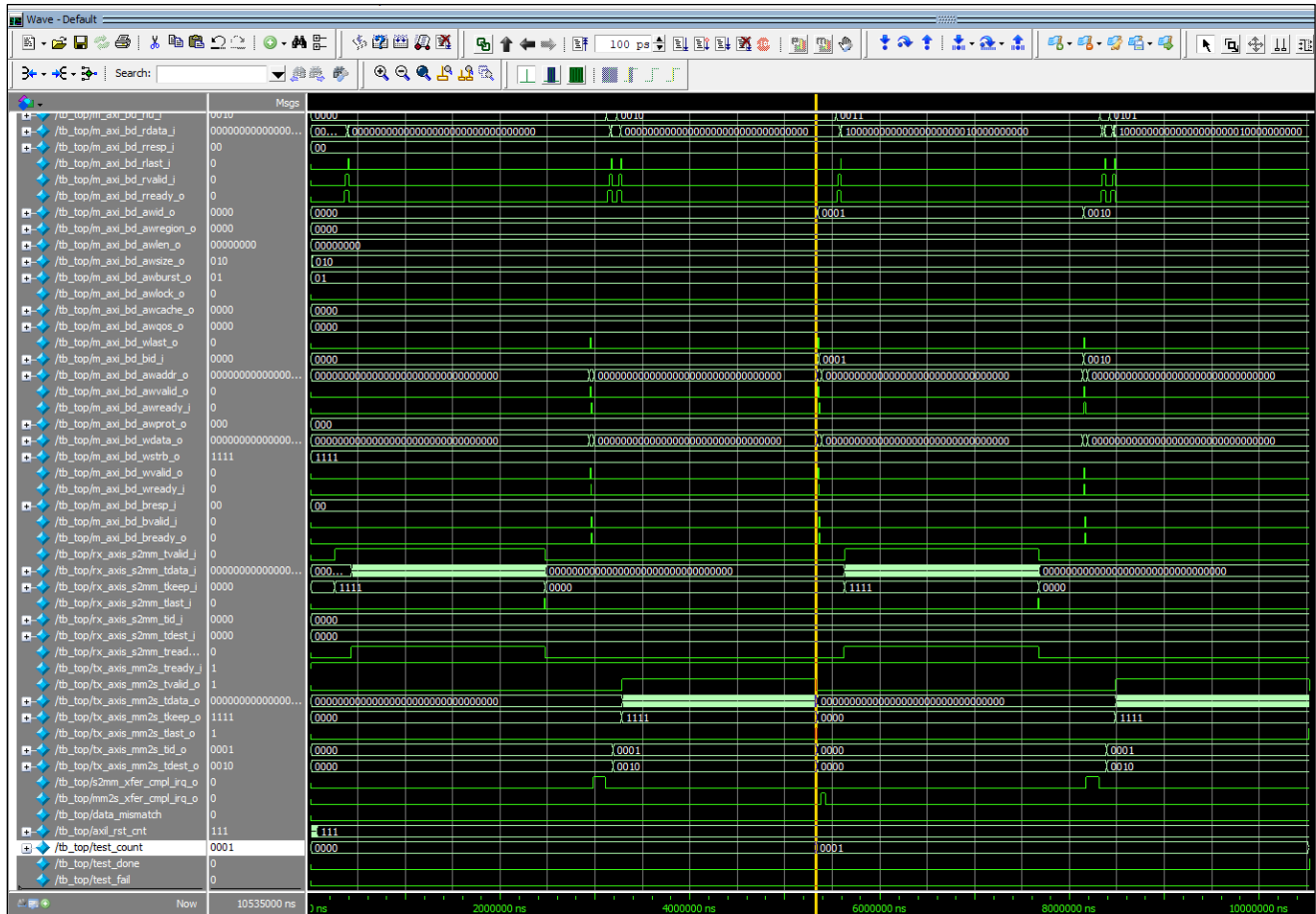
Figure 7.12 Passing Simulation Waveform
