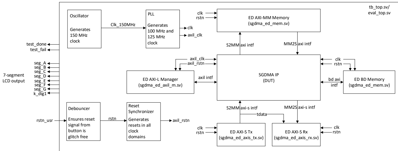
Figure 6.1. SGDMA Controller Example Design Block Diagram with Separate AXI-S Transmitter and Receiver Clock Domains Disabled and AXI-4Lite CSR Access Interface Selected
