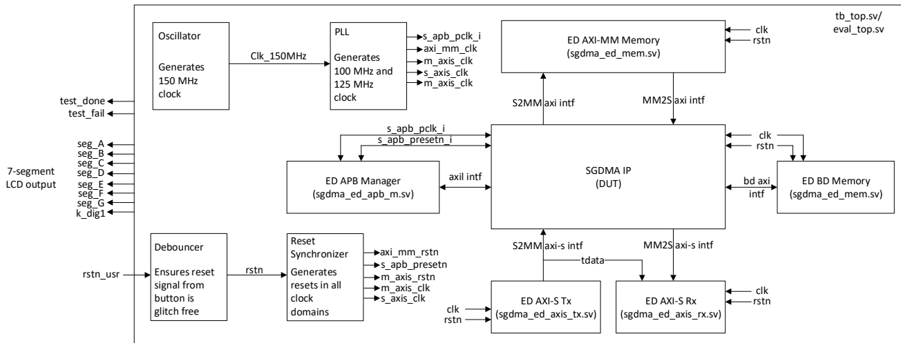
Figure 6.4. SGDMA Controller Example Design Block Diagram with Separate AXI-S Transmitter and Receiver Clock Domains Enabled and APB CSR Access Interface Selected
