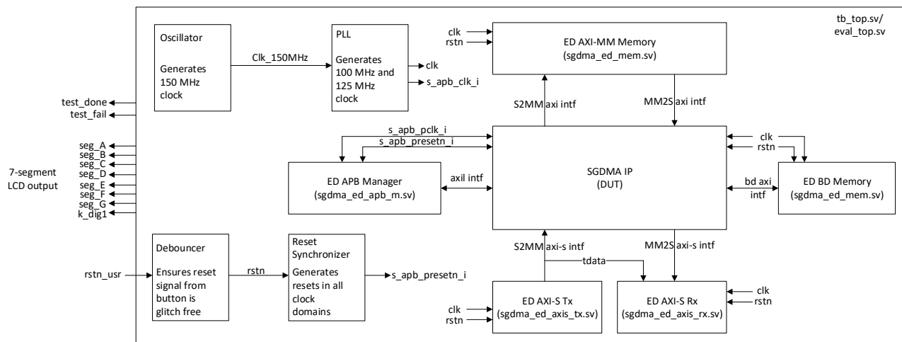
Figure 6.2. SGDMA Controller Example Design Block Diagram with Separate AXI-S Transmitter and Receiver Clock Domains Disabled and APB CSR Access Interface Selected
