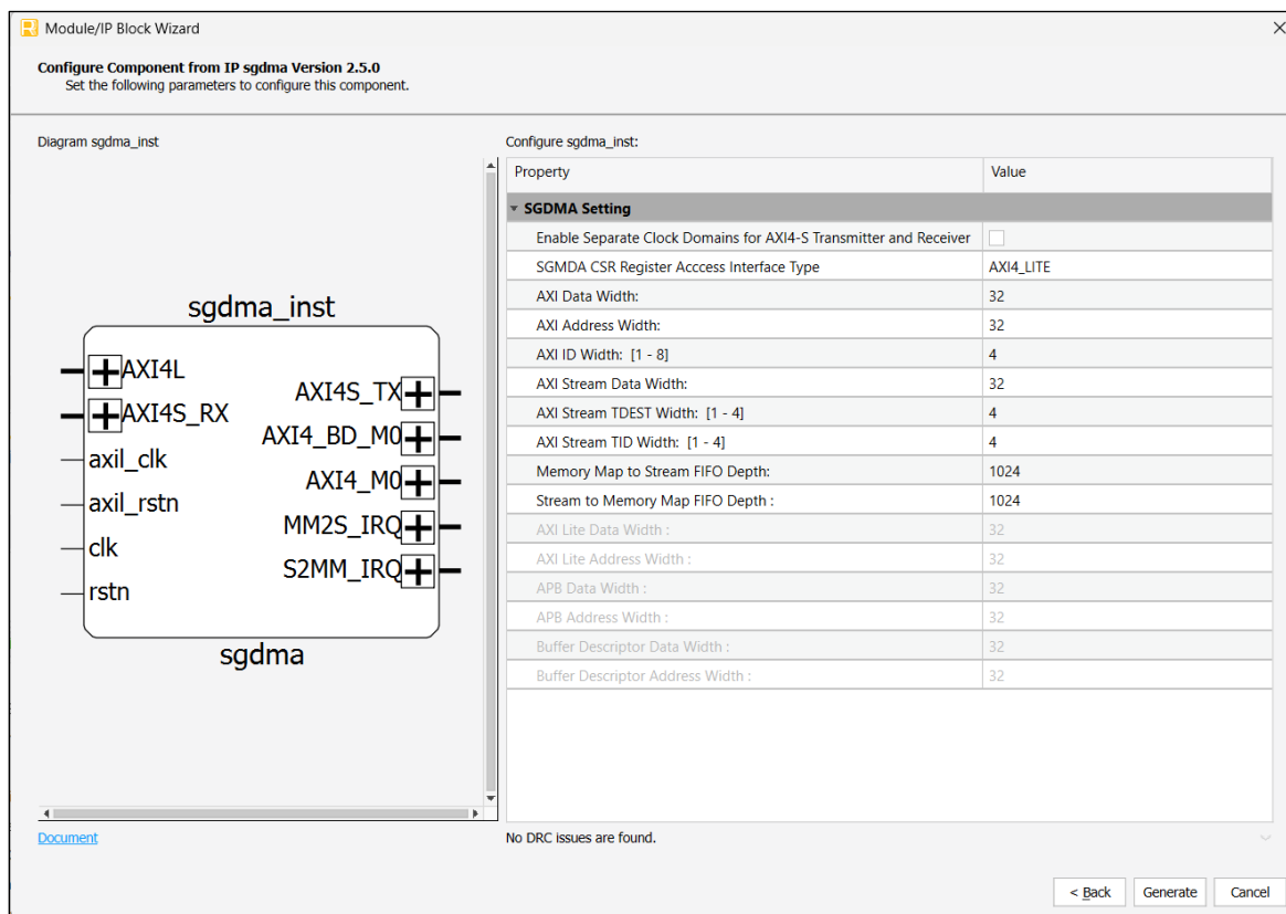
Figure 3.1. SGDMA Controller IP User Interface
