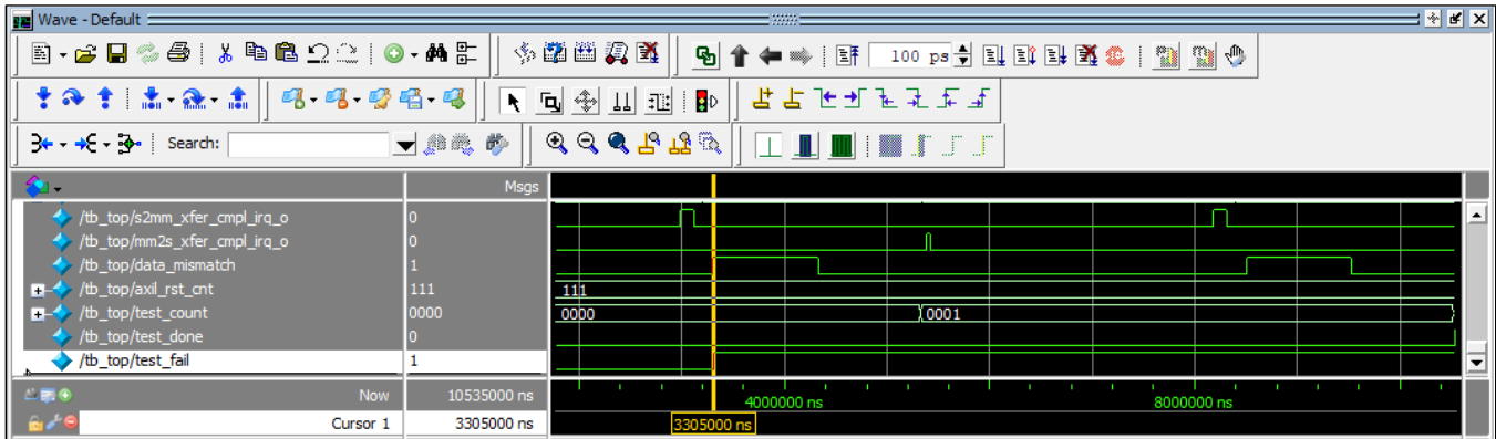
Figure 7.14. Failing Simulation Waveform
