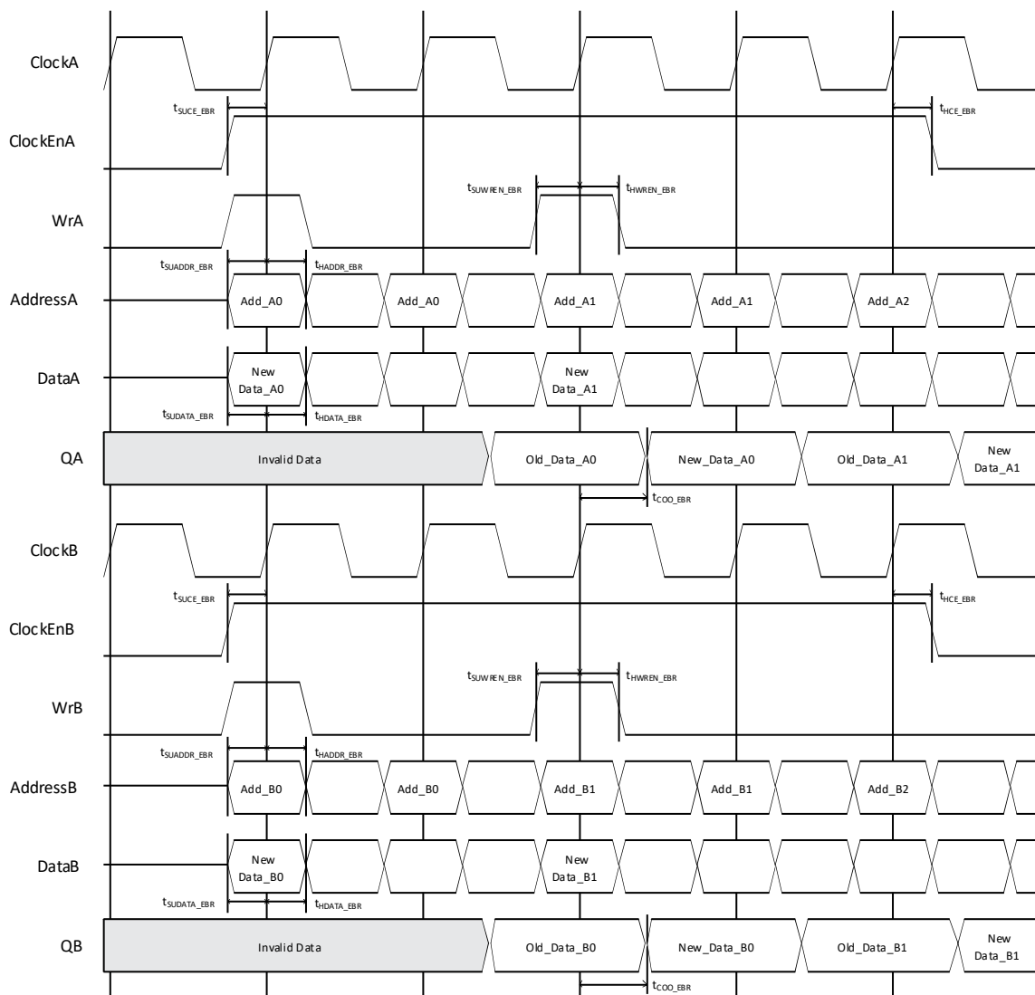
Figure 4.12. True Dual Port RAM Timing Waveform – READ BEFORE WRITE Mode, with Output Registers
