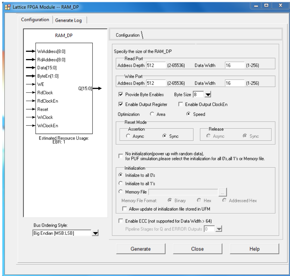
Figure 3.3. Example Generating Pseudo Dual Port RAM (RAM_DP) Module Customization (Mach-NX)
