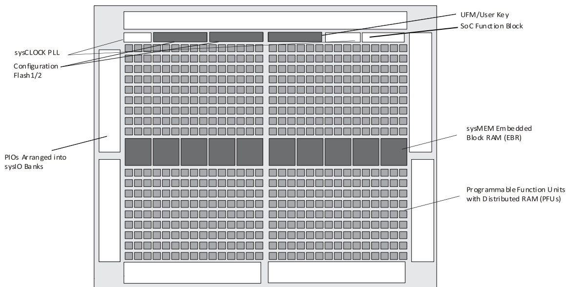
Figure 2.1. Top View of the Mach-NX Device
