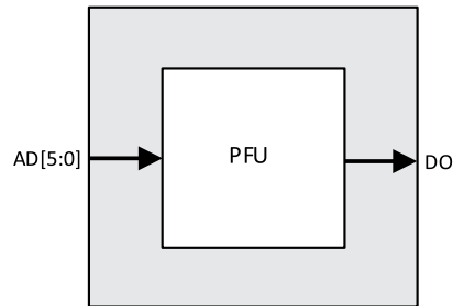
Figure 5.9. Distributed_ROM Primitive (ROM64X1A)
