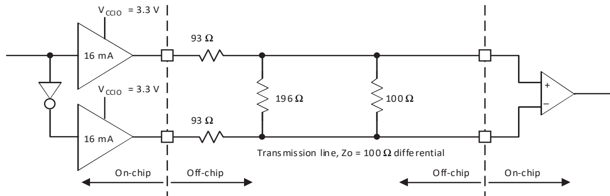
Figure 3.3. Differential LVPECL
