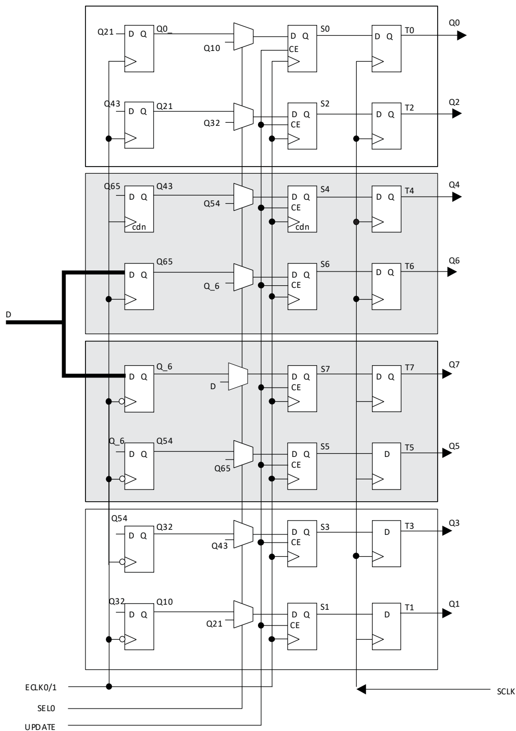
Figure 2.12. Input Gearbox
