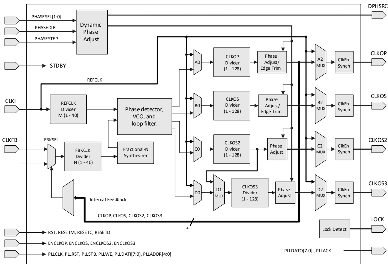
Figure 2.6. PLL Diagram
