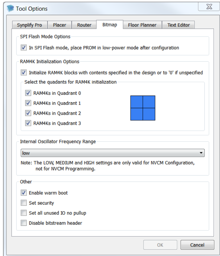
Figure 1: Bitstream Options in iCEcube2
