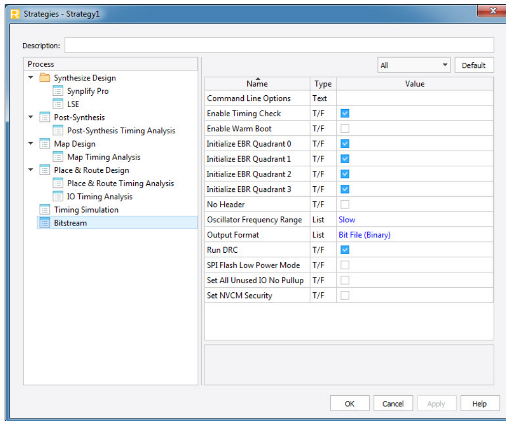
Figure 2: Bitstream Options in Radiant Software
