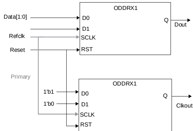
Figure 5.20. GDDR1_TX.SCLK.Aligned Interface
