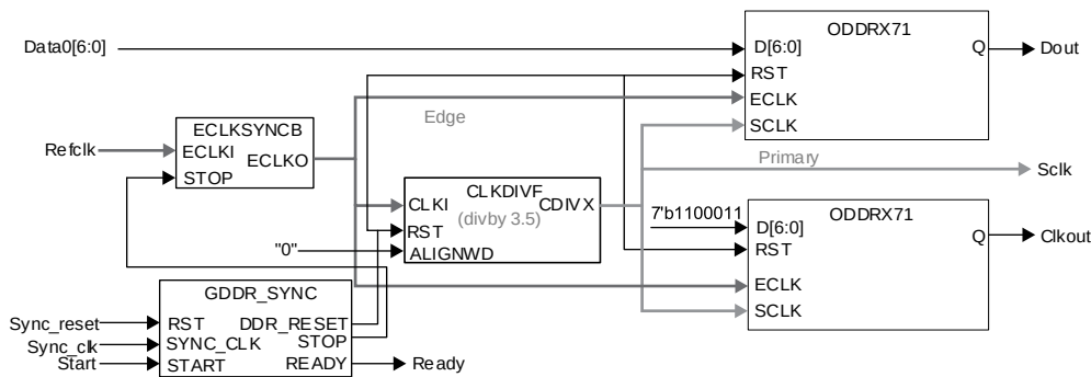
Figure 5.28. GDDR71_TX.ECLK Interface
