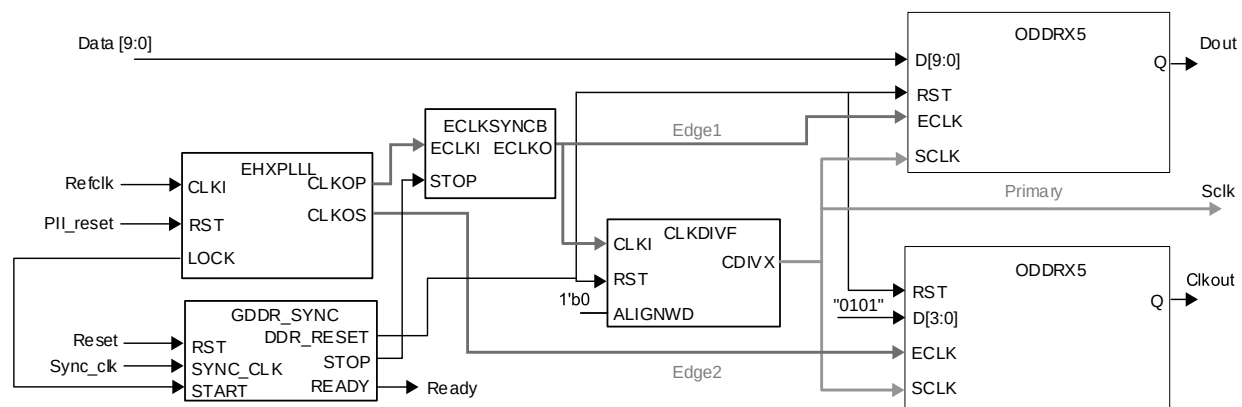
Figure 5.27. GDDR5_TX.ECLK.Centered Interface
