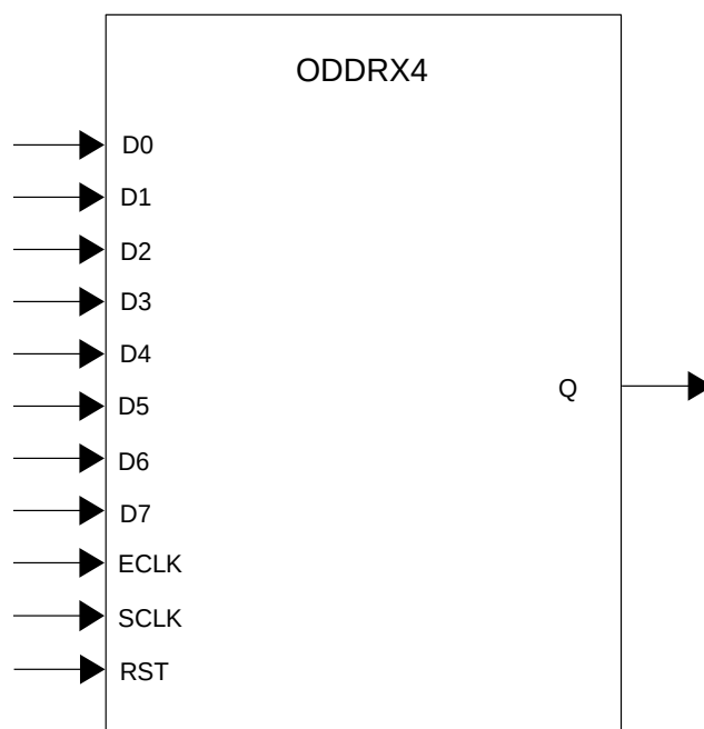
Figure 8.12. ODDRX4 Primitive
