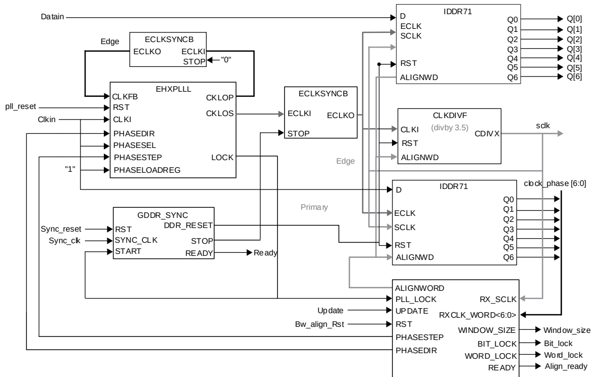
Figure 5.17. GDDR71_RX.ECLK Interface
