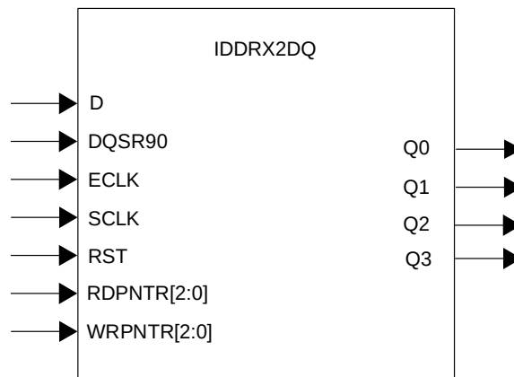
Figure 8.15. IDDRX2DQ Primitive
