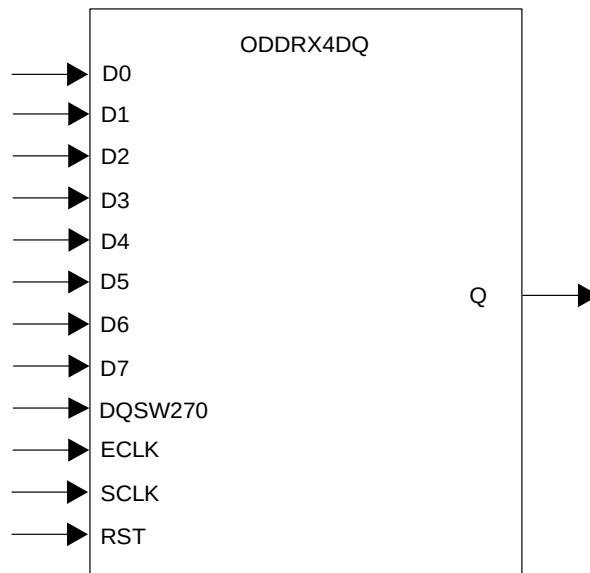
Figure 8.18. ODDRX4DQ Primitive
