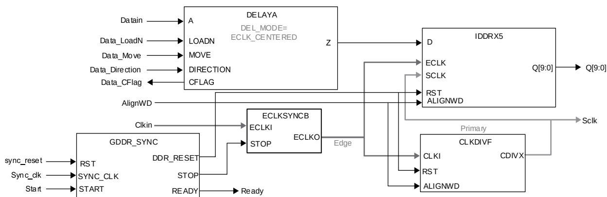
Figure 5.14. GDDR5_RX.ECLK.Centered Interface (Dynamic Data Delay)
