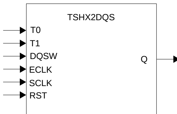
Figure 8.23. TSHX2DQS Primitive
