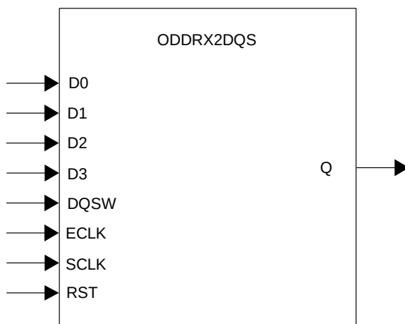
Figure 8.19. ODDR2DQS Primitive
