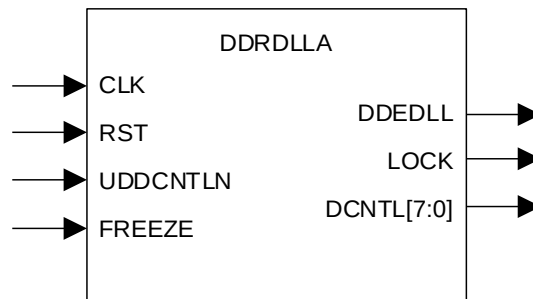
Figure 8.3. DDRDLLA Primitive
