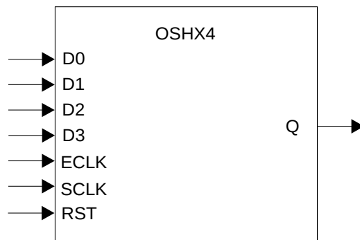
Figure 8.26. OSHX4 Primitive
