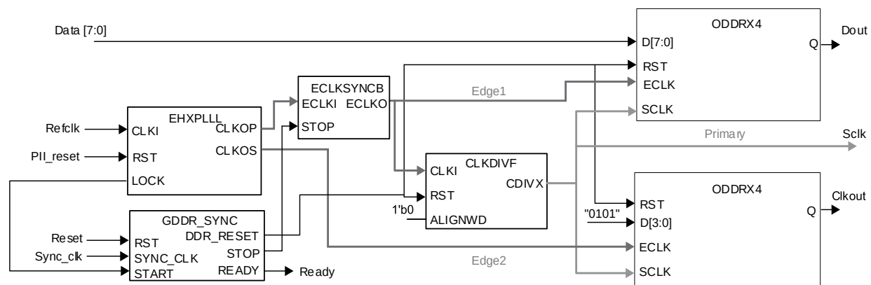
Figure 5.25. GDDR4_TX.ECLK.Centered Interface
