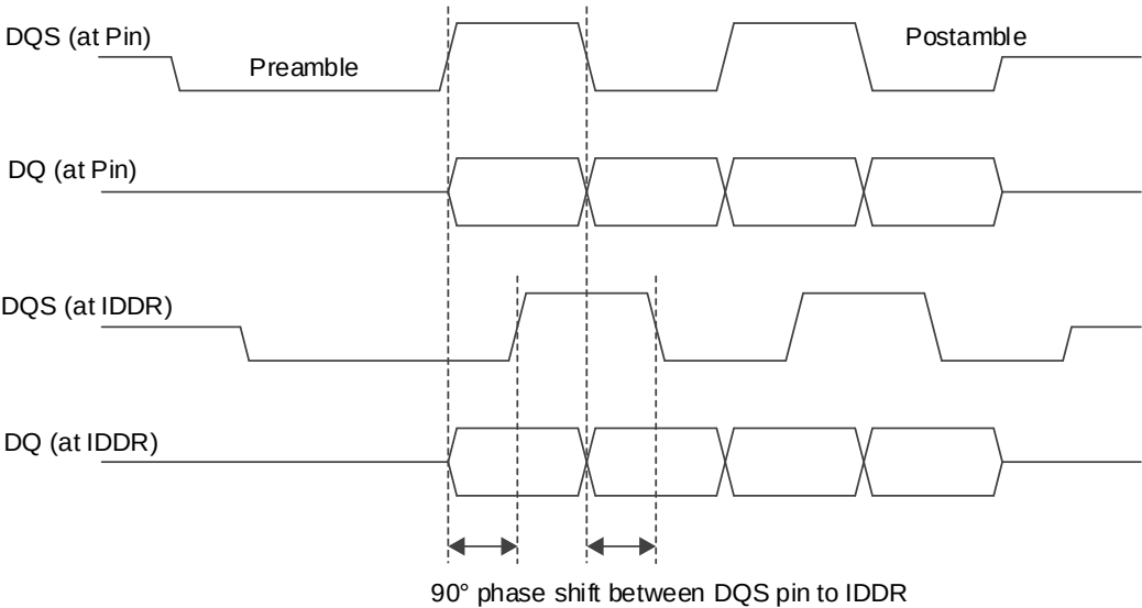
Figure 6.3. DQ-DQS During Read
