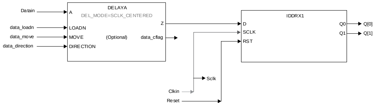
Figure 5.2. GDDR_X1_RX.SCLK.Centered Interface (Dynamic Data delay)
