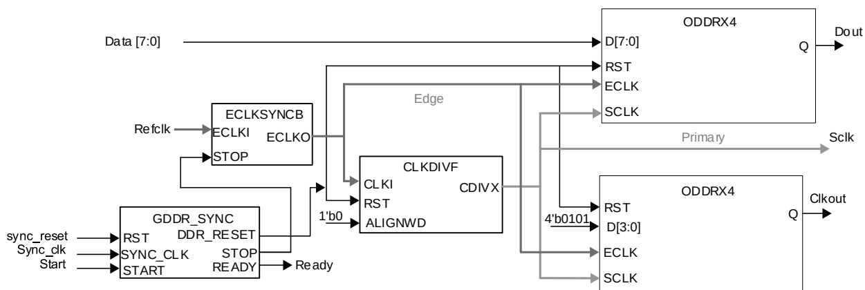
Figure 5.24. GDDR4_TX.ECLK.Aligned Interface
