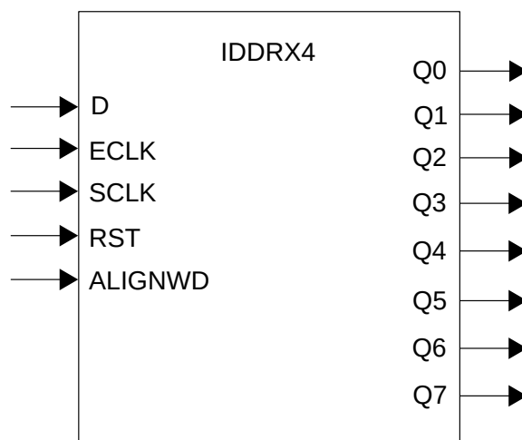
Figure 8.7. IDDRX4 Primitive
