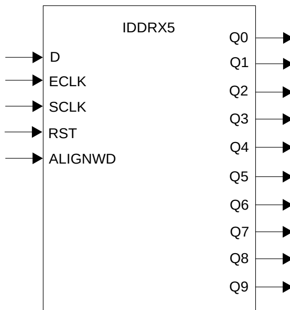
Figure 8.8. IDDRX5 Primitive
