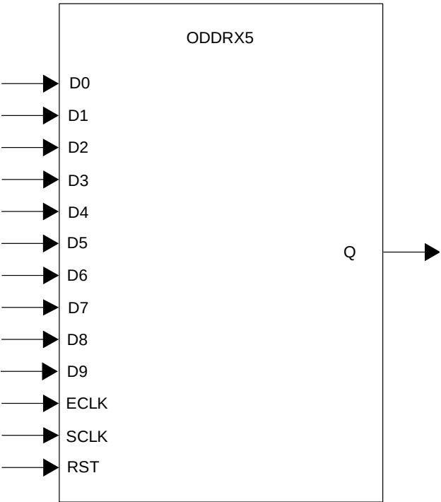
Figure 8.13. ODDR5 Primitive
