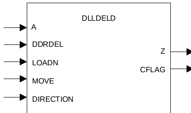
Figure 8.4. DLLDELD Primitive
