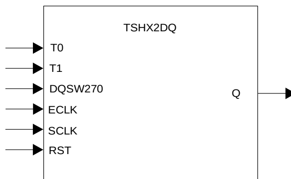
Figure 8.21. TSHX2DQ Primitive
