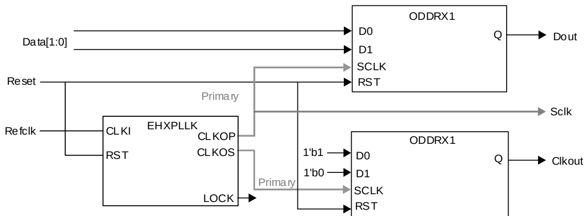
Figure 5.21. GDDR1_TX.SCLK.Centered Interface
