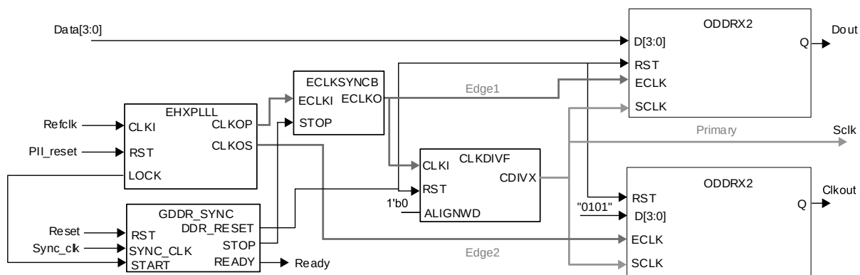
Figure 5.23. GDDR2_TX.ECLK.Centered Interface
