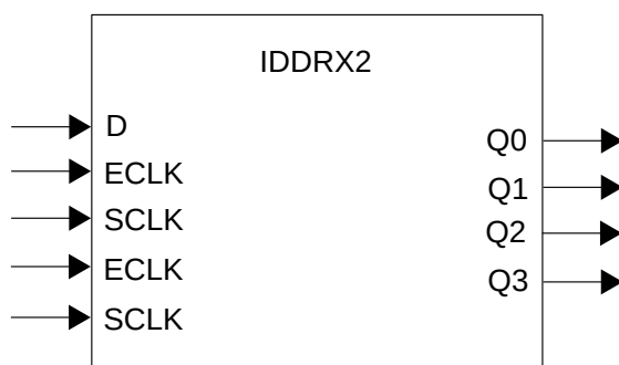
Figure 8.6. IDDRX2 Primitive
