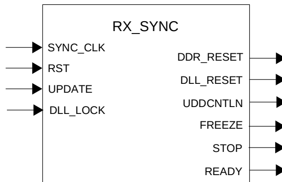
Figure 9.2. RX_SYNC Ports
