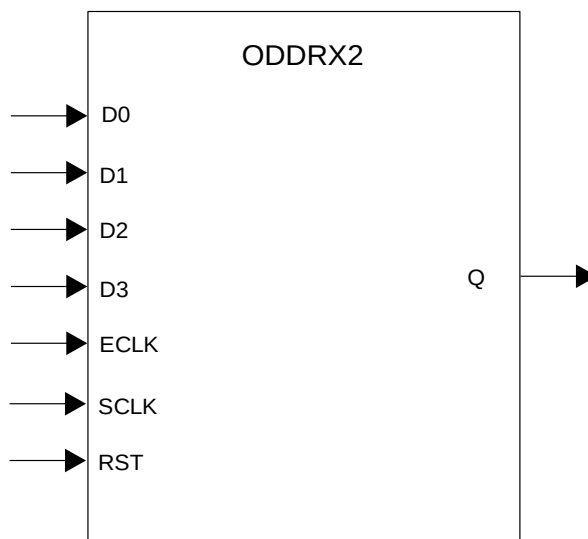
Figure 8.11. ODDR2
