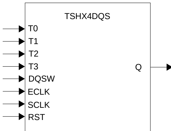
Figure 8.24. TSHX4DQS Primitive
