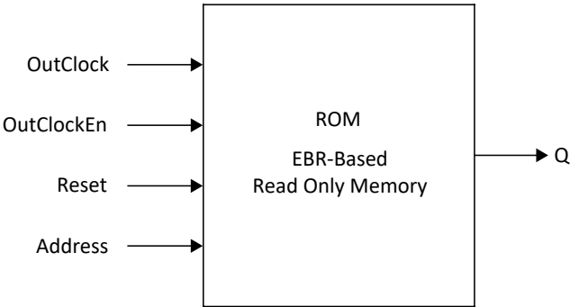
Figure 4.20. ROM – Read Only Memory Module Generated by Clarity Designer
