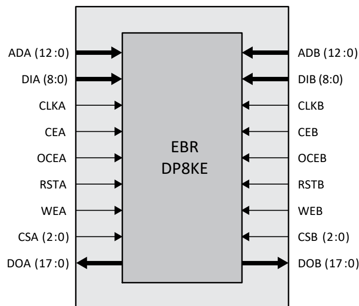
Figure 4.9. True Dual Port RAM Primitive for CrossLinkPlus Devices
