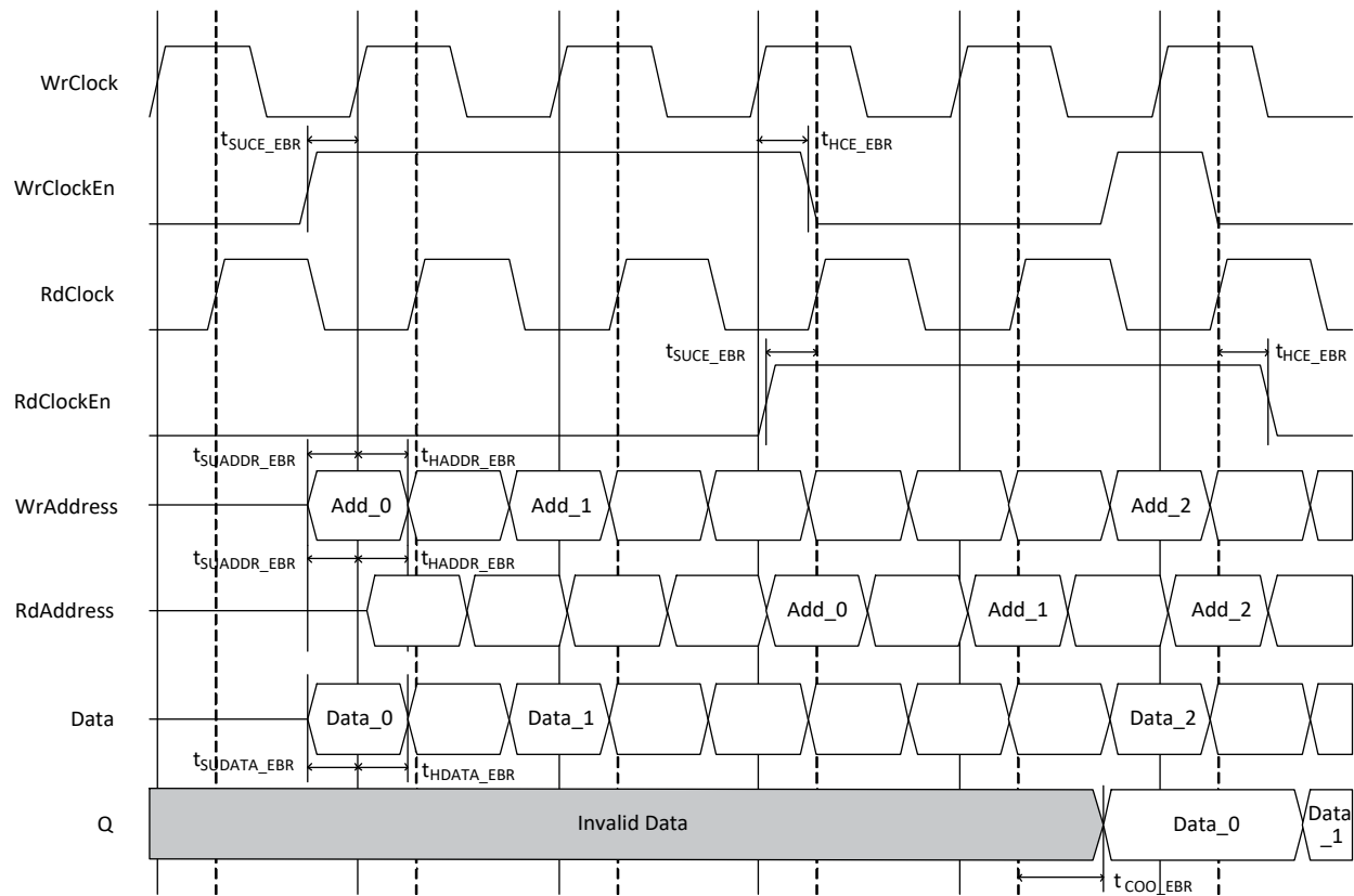
Figure 4.19. Pseudo Dual Port RAM Timing Diagram with Output Registers
