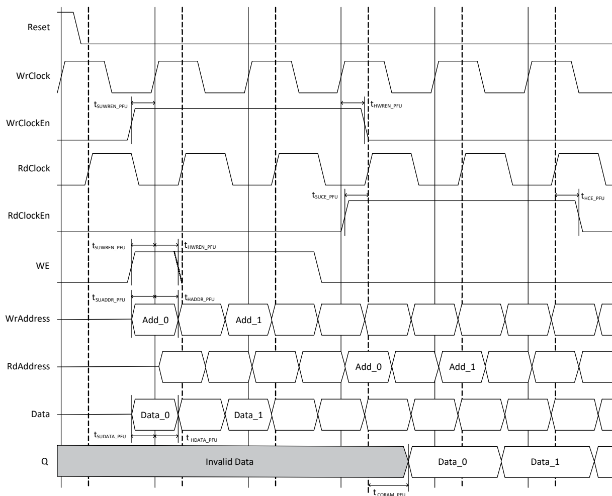
Figure 4.50. PFU-Based Distributed Dual Port RAM Timing Waveform with Output Registers
