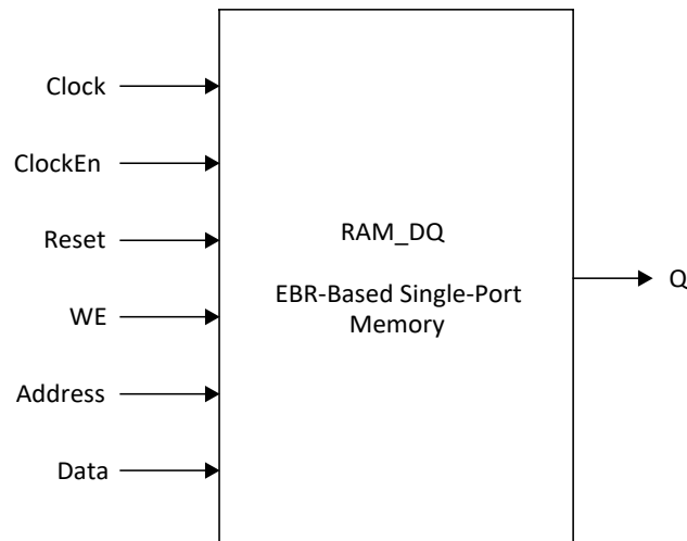
Figure 4.1. Single-Port Memory Module Generated by Clarity Designer
