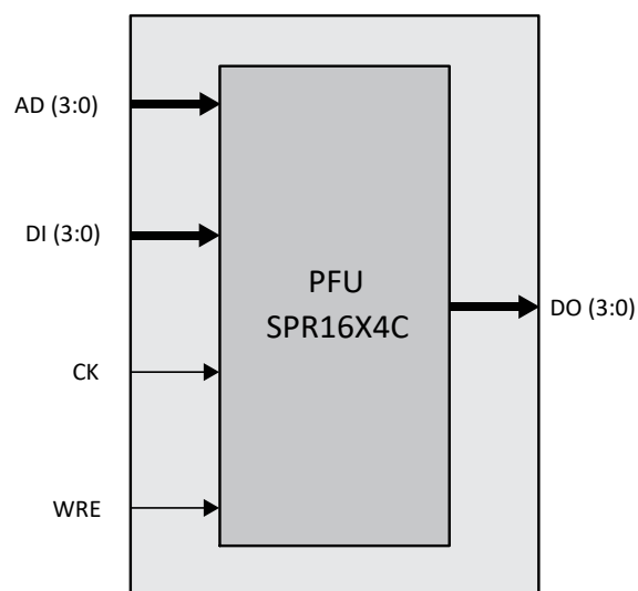
Figure 4.44. Single Port Distributed RAM Primitive for CrossLinkPlus Devices
