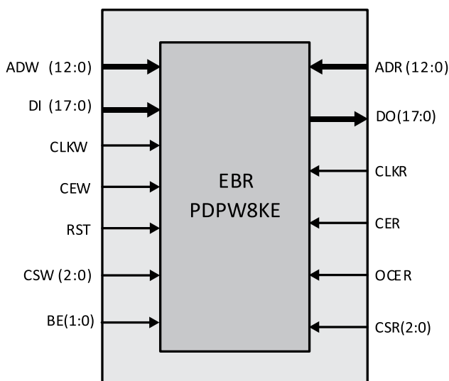
Figure 4.17. Pseudo-Dual Port RAM Primitive for CrossLinkPlus Devices
