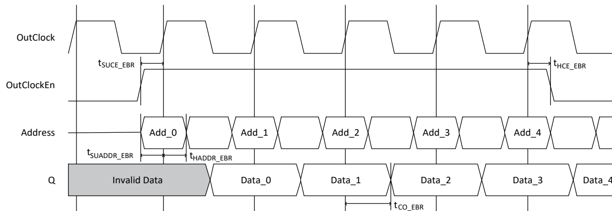
Figure 4.21. ROM Timing Waveform without Output Registers
