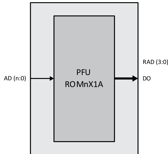
Figure 4.52. Distributed ROM Primitive for CrossLinkPlus Devices
