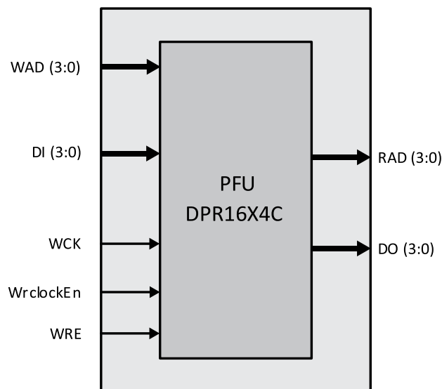
Figure 4.48. Dual Port Distributed RAM Primitive for CrossLinkPlus Devices
