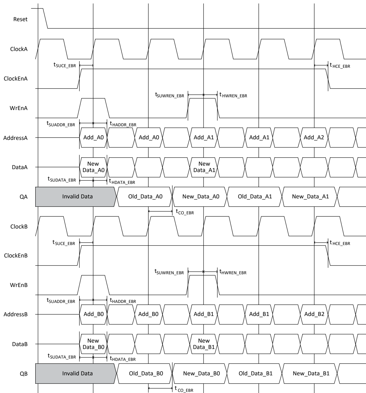
Figure 4.14. True Dual Port RAM Timing Waveform in Read Before Write (READBEFOREWRITE) Mode without Output Registers
