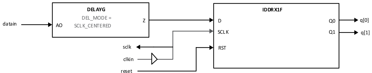
Figure 5.1. GDDR1_RX.SCLK.Centered Interface (Static Delay)
