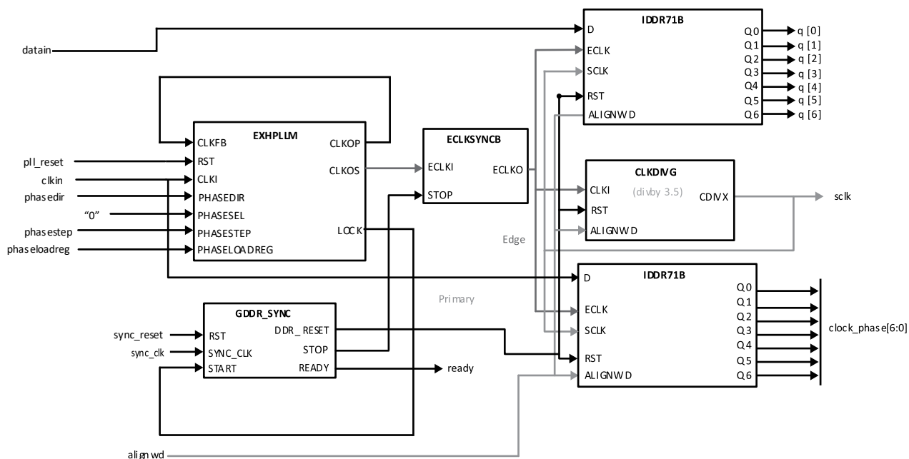
Figure 5.10. GDDR71_RX.ECLK Interface (DELAYF and BW_ALIGN Not Enabled)
