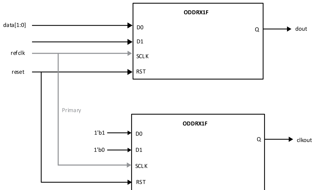
Figure 5.18. GDDR1_TX.SCLK.Aligned Interface
