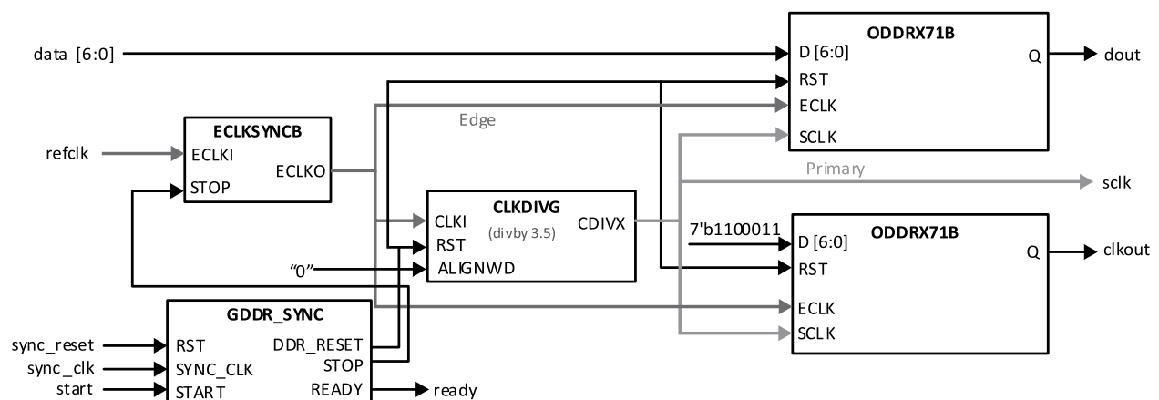
Figure 5.26. GDDR71_TX.ECLK Interface
