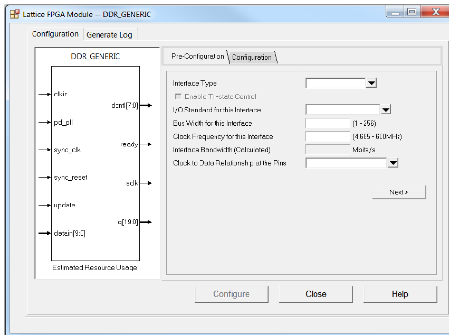
Figure 6.3. DDR_Generic Pre-Configuration Tab
