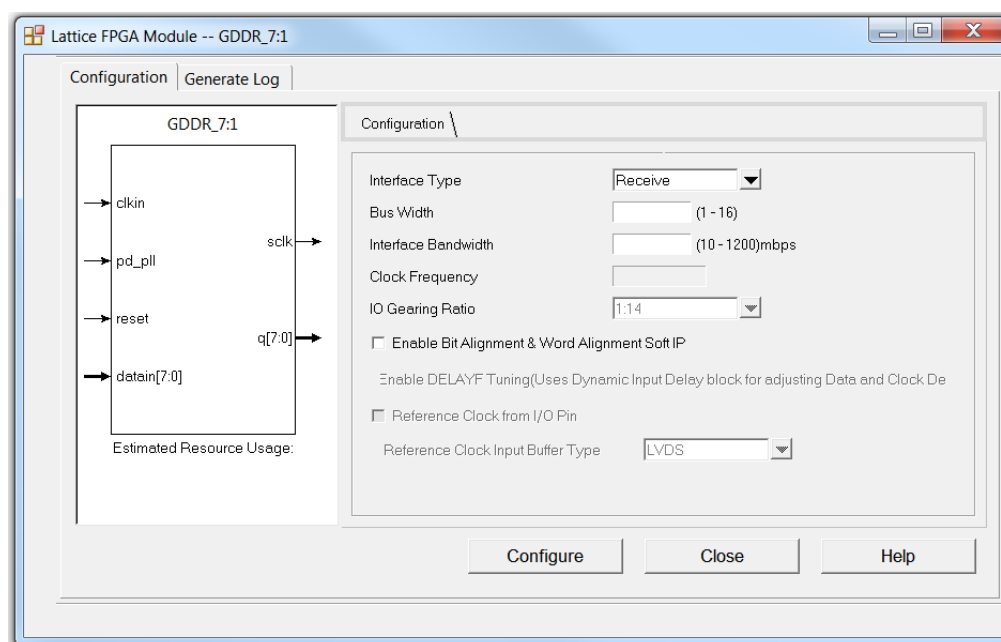
Figure 6.6. GDDR_7:1 LVDS Configuration Tab
