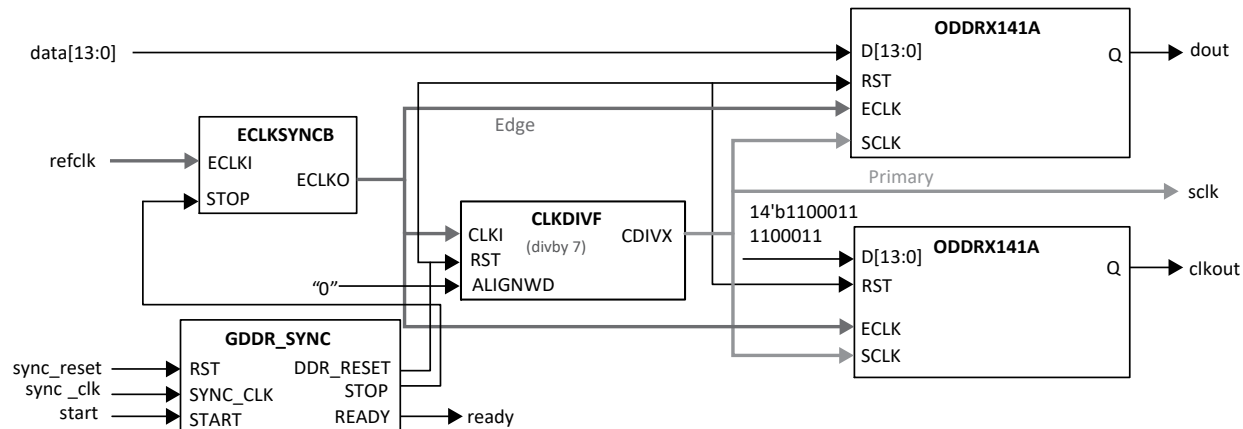
Figure 5.27. GDDR141_TX.ECLK Interface
