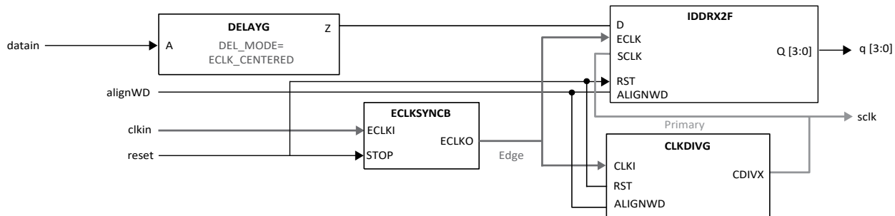
Figure 5.5. GDDR2_RX.ECLK.Centered Interface (Static Delay)
