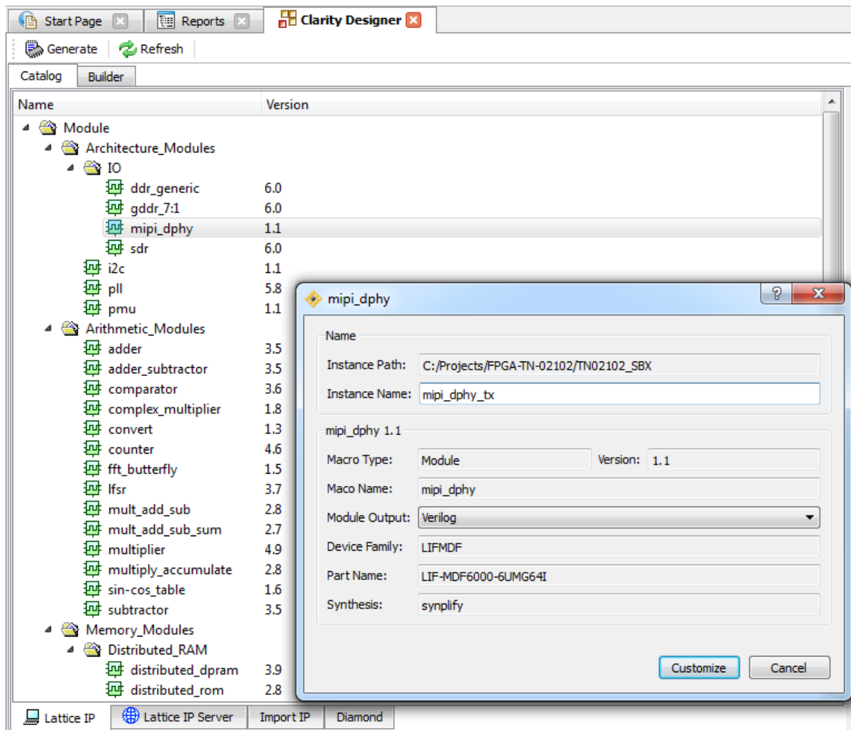
Figure 6.7. MIPI D-PHY Selected in Clarity Designer Main Window
