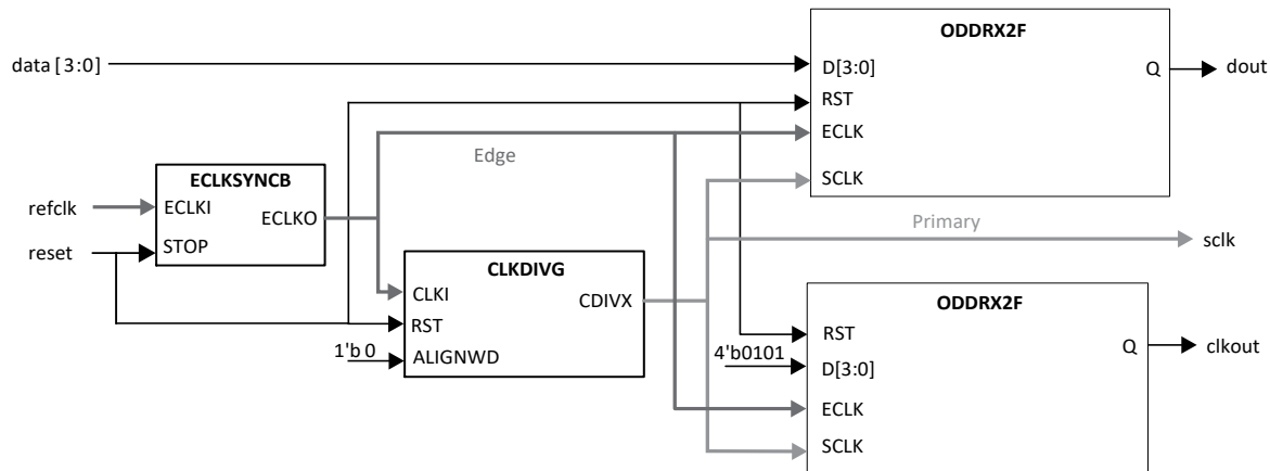
Figure 5.22. GDDR2_TX.ECLK.Aligned Interface
