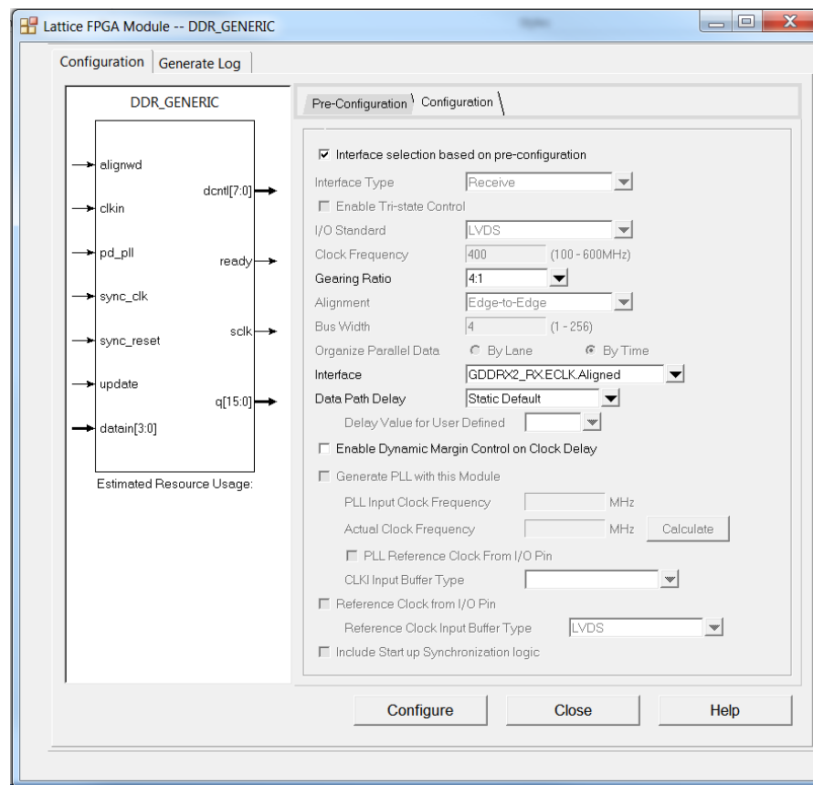
Figure 6.4. DDR_Generic Configuration Tab
