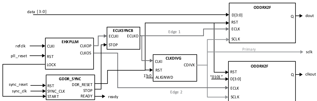
Figure 5.24. GDDR2_TX.ECLK.Centered Interface
