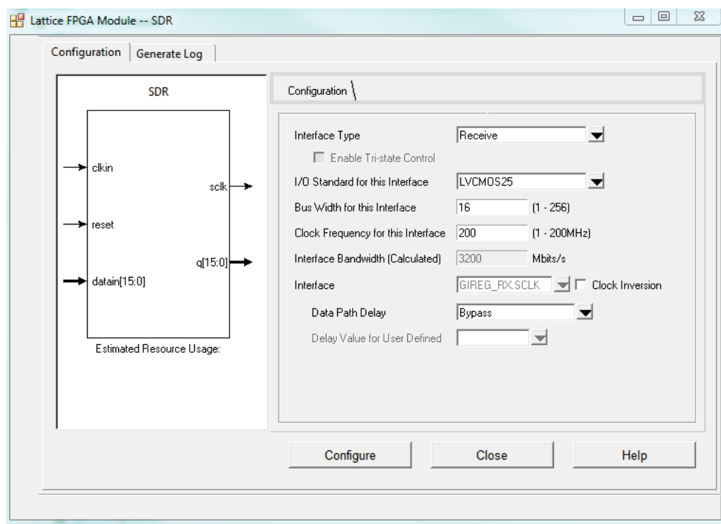
Figure 6.10. SDR Configuration Tab
