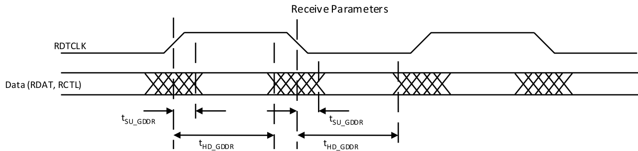
Figure 6.12. RX Aligned Interface Timing
