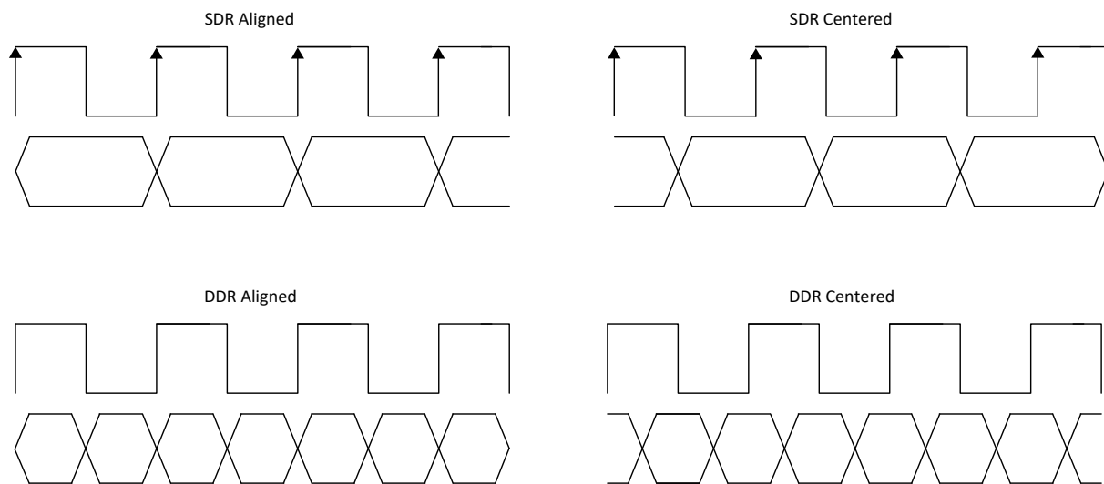
Figure 3.1. External Interface Definitions
