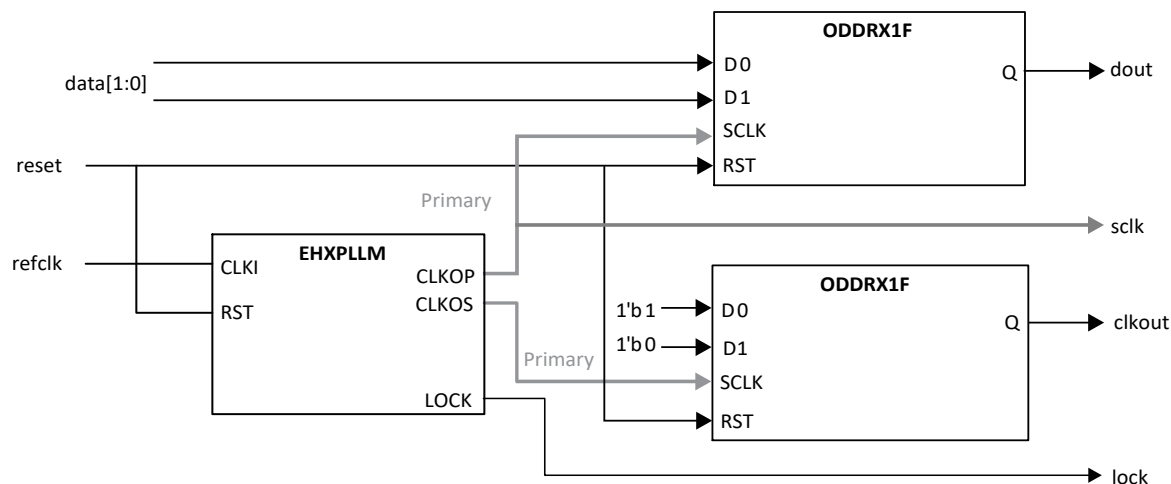
Figure 5.20. GDDR1_TX.SCLK.Centered Interface
