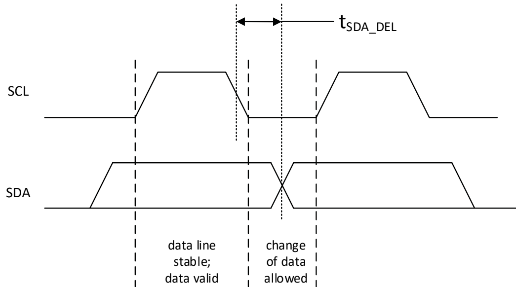
Figure 2.10. I2C Bit Transfer Timing
