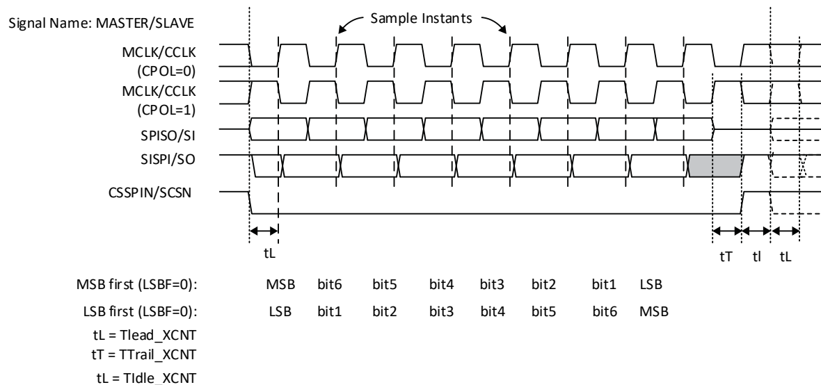
Figure 3.11. SPI Control Timing (SPICR2[CPHA]=0, SPICR1[TXEDGE]=1)
