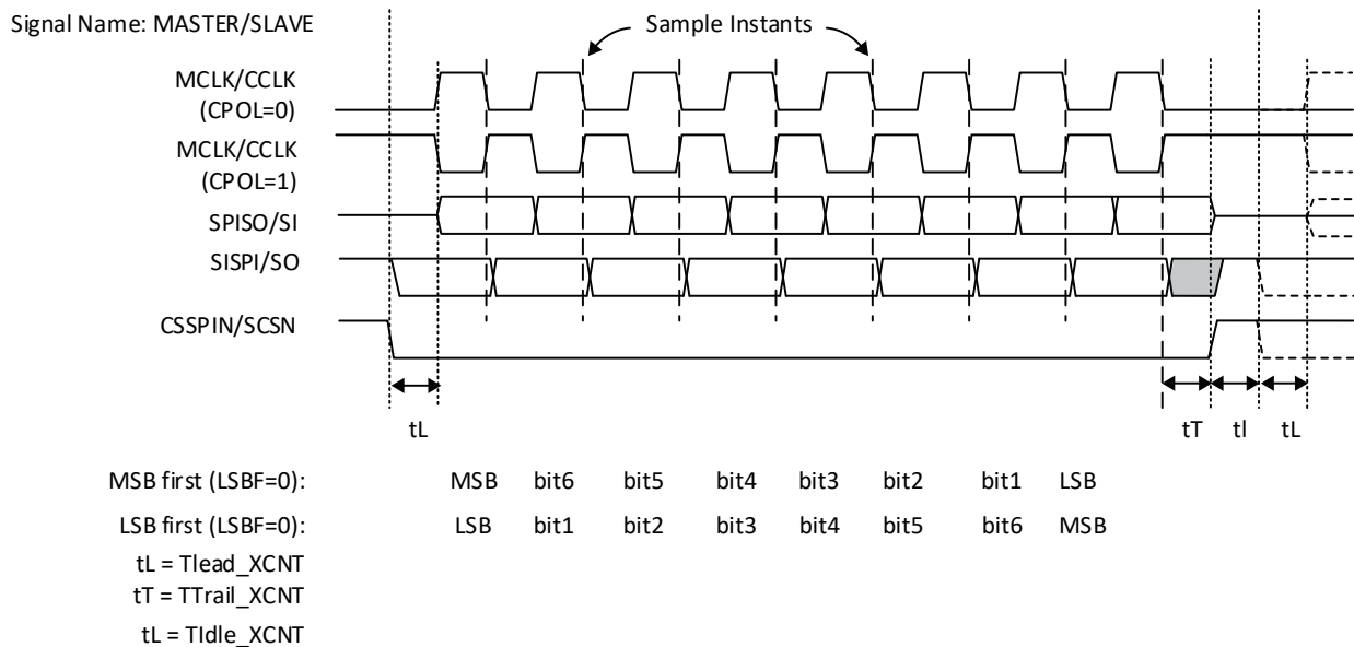
Figure 3.12. SPI Control Timing (SPICR2[CPHA]=1, SPICR1[TXEDGE]=1)
