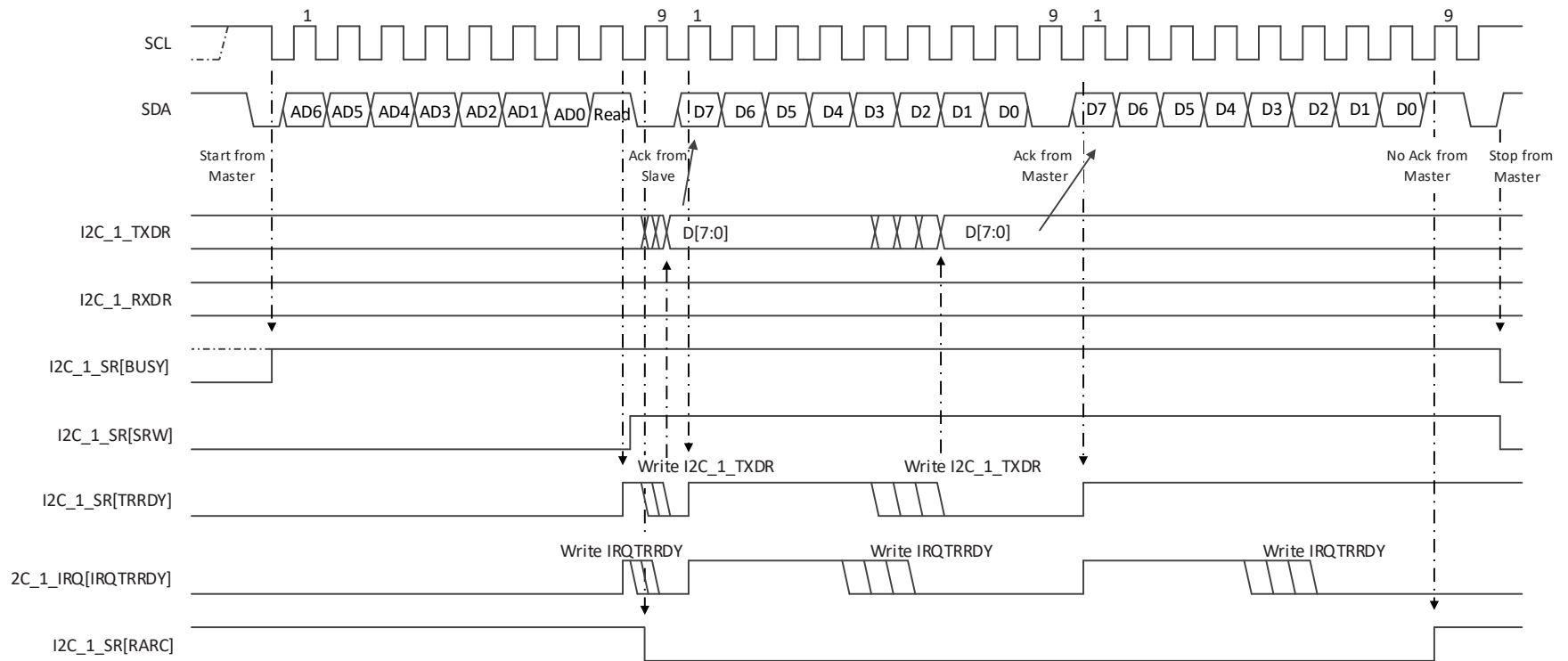
Figure 2.9. EFB Slave - I2C Read
