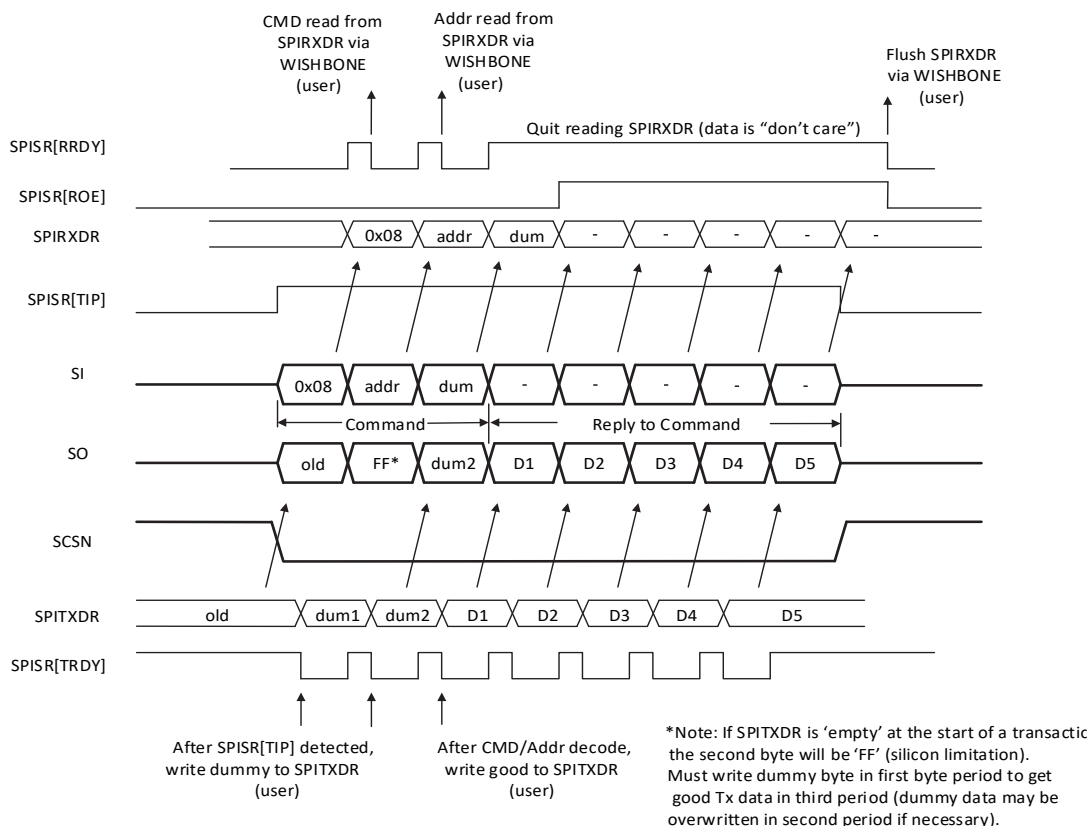
Figure 3.7. Minimally Specified SPI Transaction Example (MachXO3D as SPI Slave)
