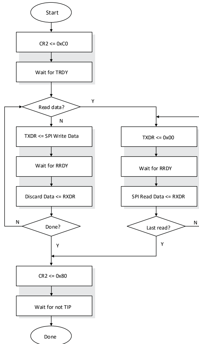
Figure 3.1. SPI Master Read/Write Example (via WISHBONE)
