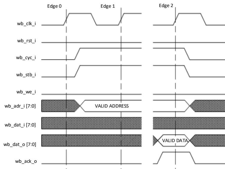
Figure 1.4. WISHBONE Bus Read Operation
