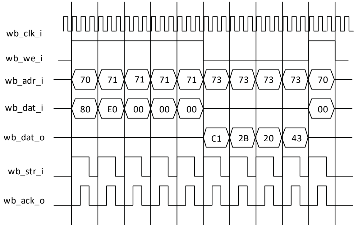
Figure 7.3. WISHBONE Read Device ID Example
