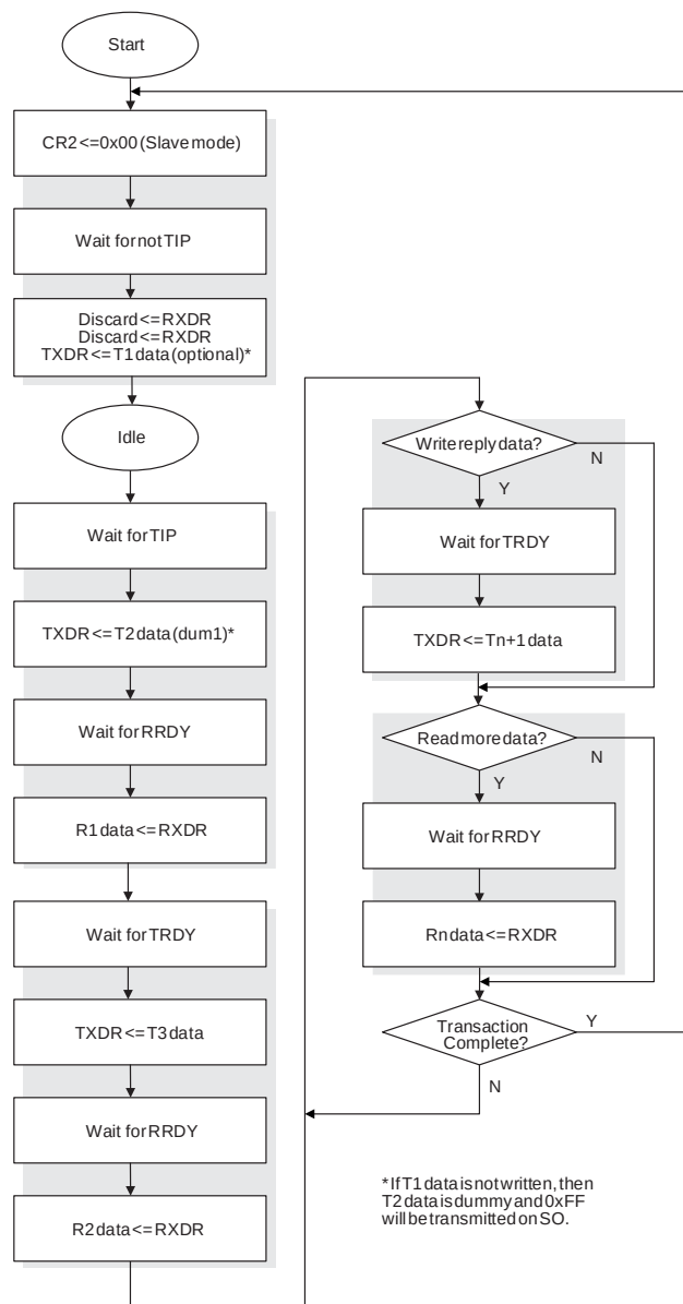
Figure 3.2. SPI Slave Read/Write Example (via WISHBONE)
