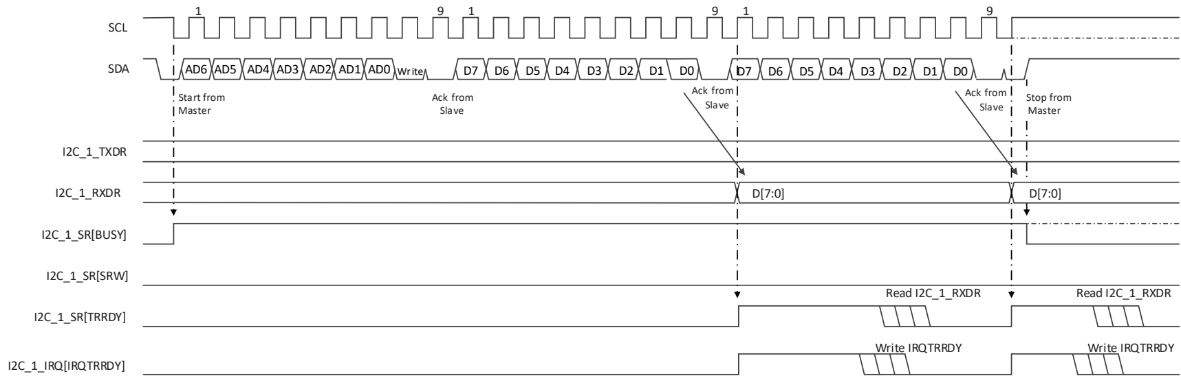
Figure 2.8. EFB Slave - I2C Write
