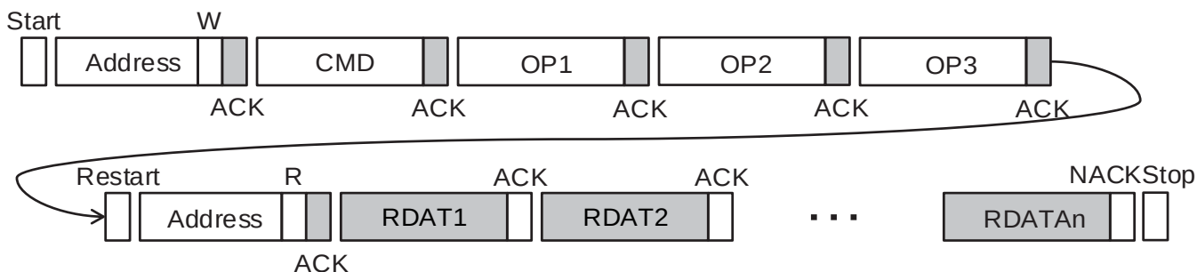
Figure 2.5. I2C Command with Read Data (for example, LSC_READ_STATUS)
