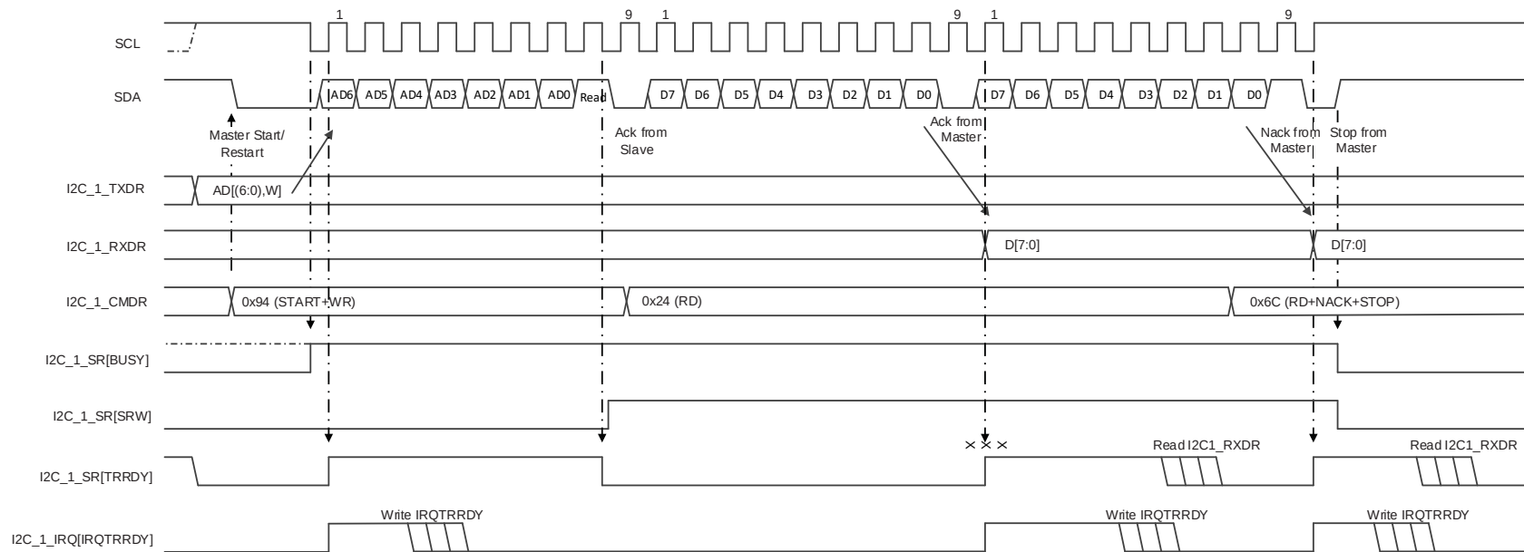
Figure 2.7. EFB Master - I2C Read
