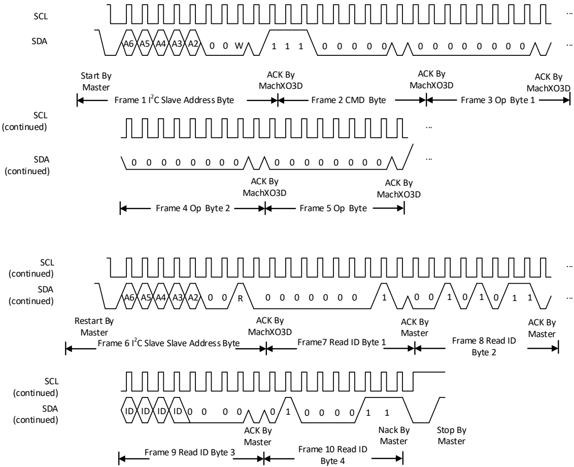
Figure 7.1. I2C Read Device ID Example
