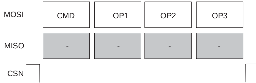
Figure 3.3. Simple SPI Command (for example, ISC_ERASE)
