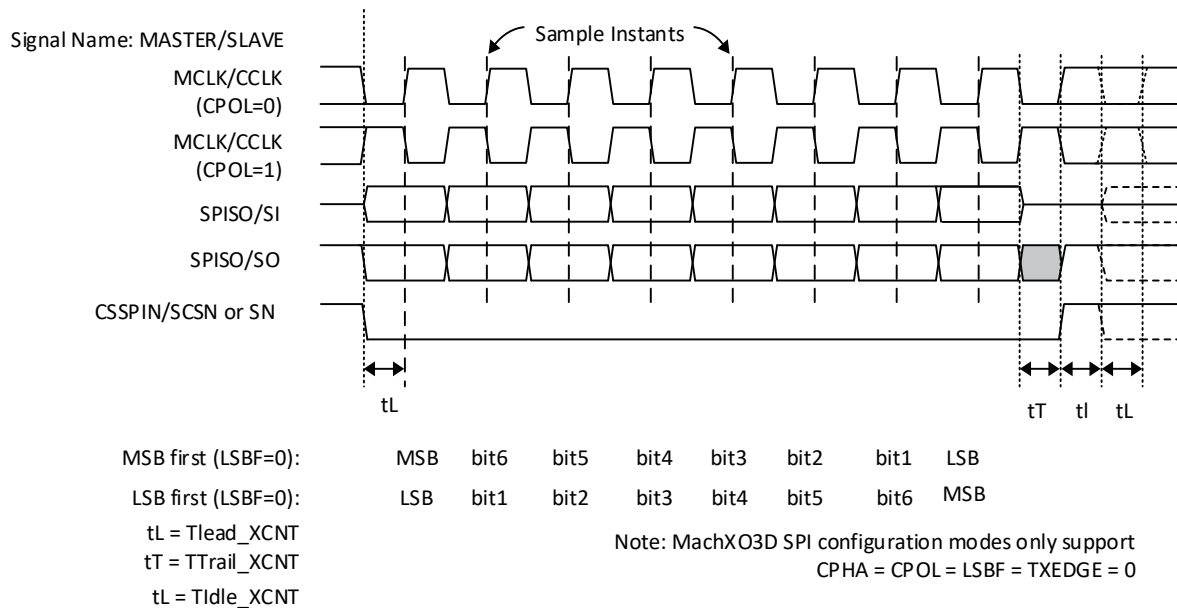
Figure 3.9. SPI Control Timing (SPICR2[CPHA]=0, SPICR1[TXEDGE]=0)
