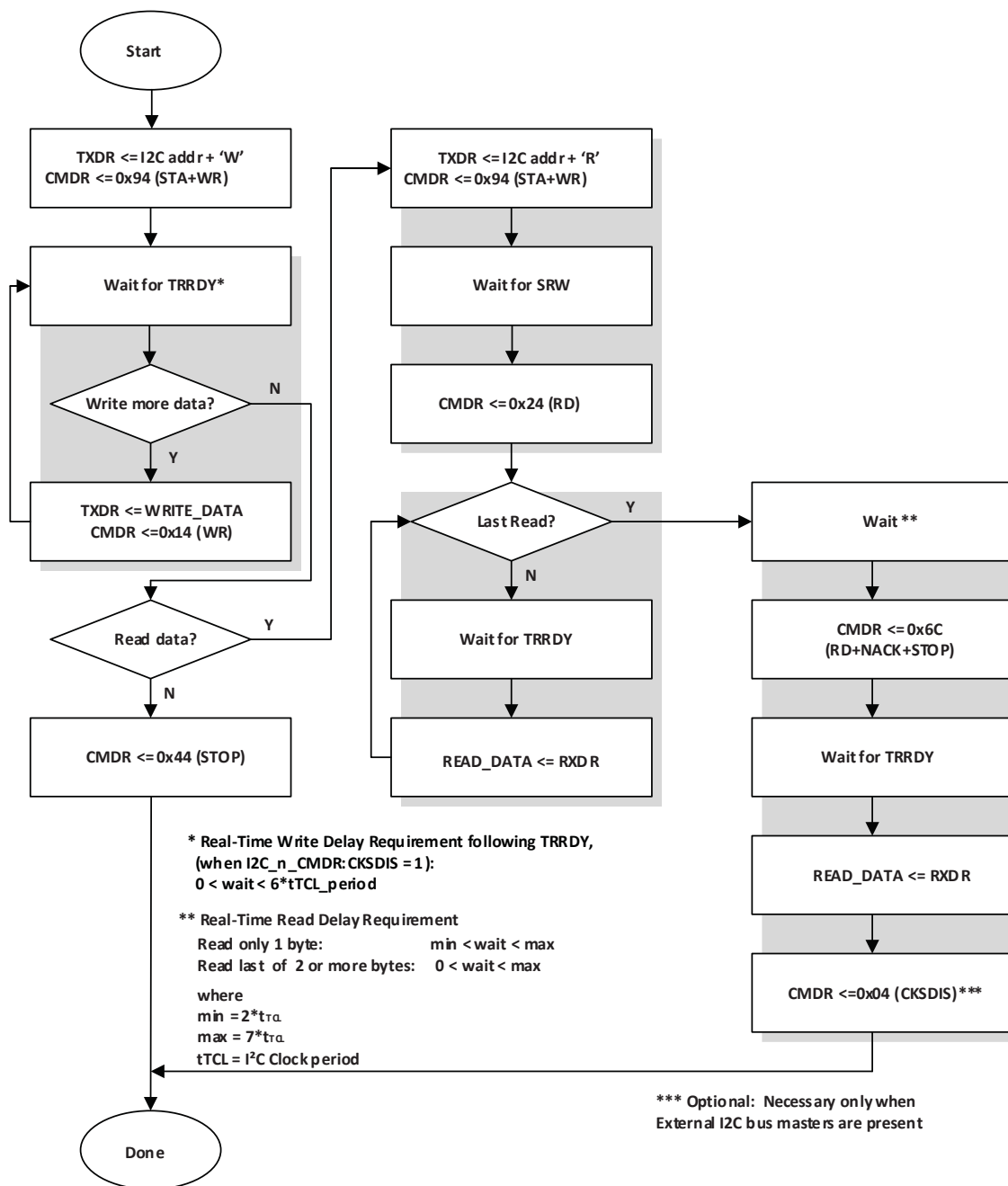
Figure 2.1. I2C Master Read/Write Example (Through WISHBONE)
