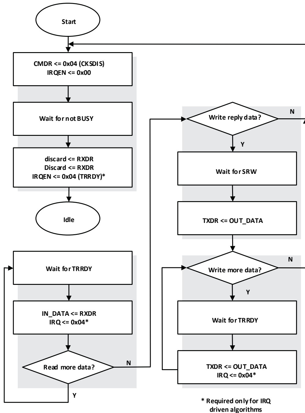
Figure 2.2. I2C Slave Read/Write Example (through WISHBONE)
