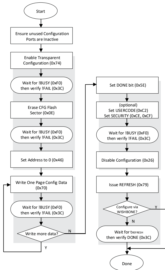
Figure 6.1. Basic Configuration UFM Program Example
