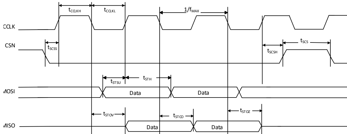
Figure 3.8. Slave SPI Configuration Timing
