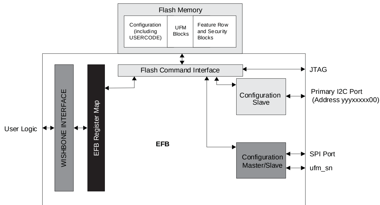
Figure 5.1. Interfaces to the Flash Memory Sectors
