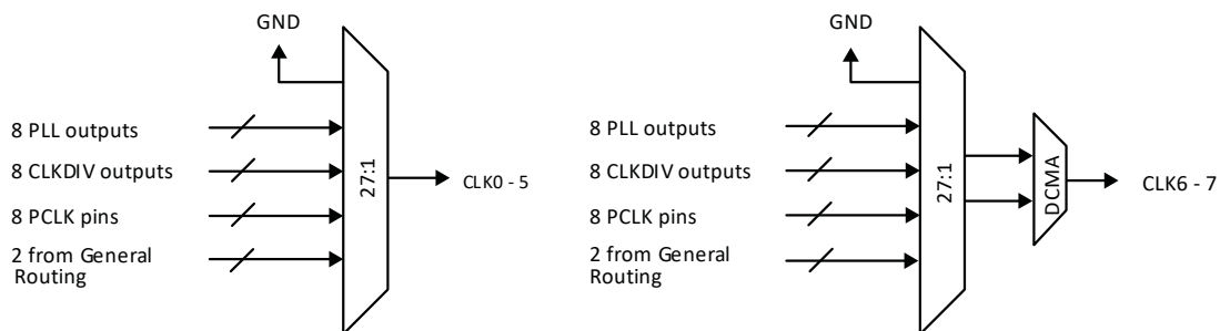
Figure A.2. MachXO3D Primary Clock Muxes
