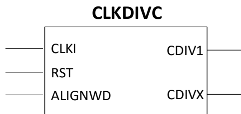
Figure 9.2. CLKDIVC Primitive Symbol
