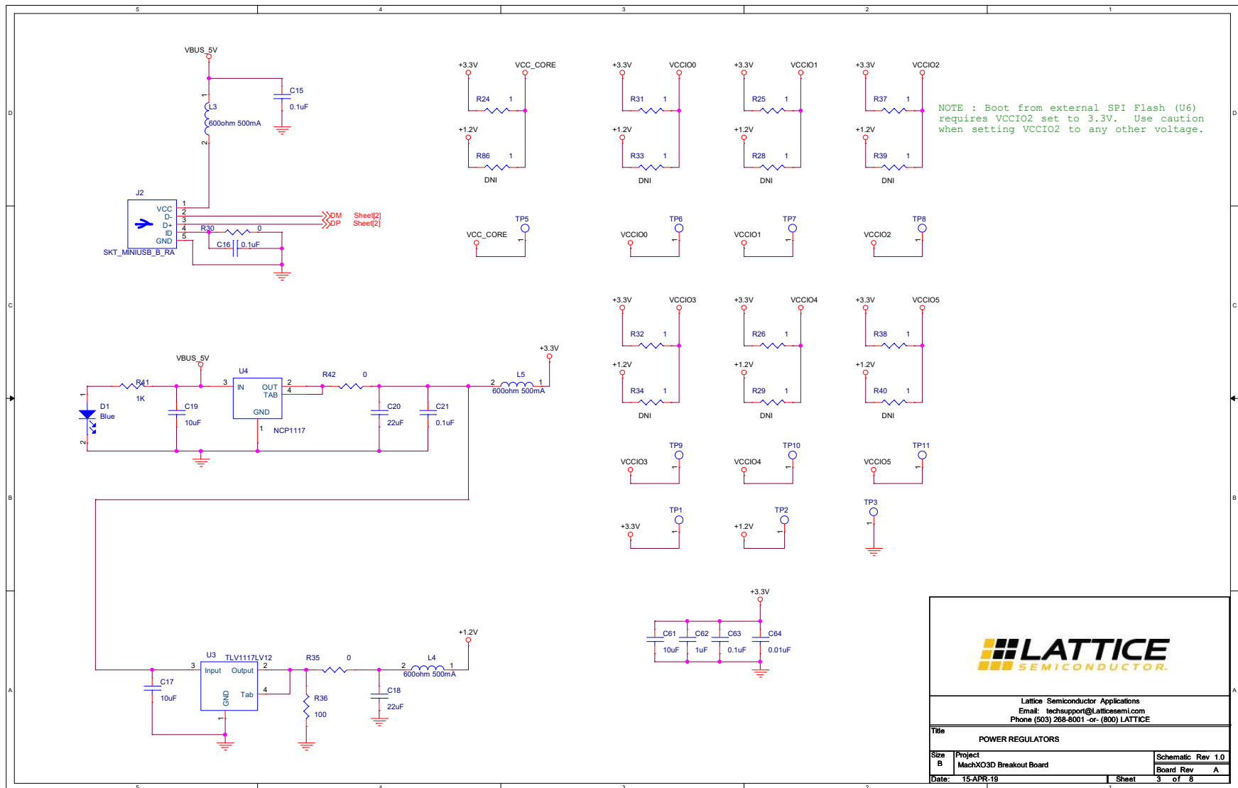
Figure A.3. Power Regulators
