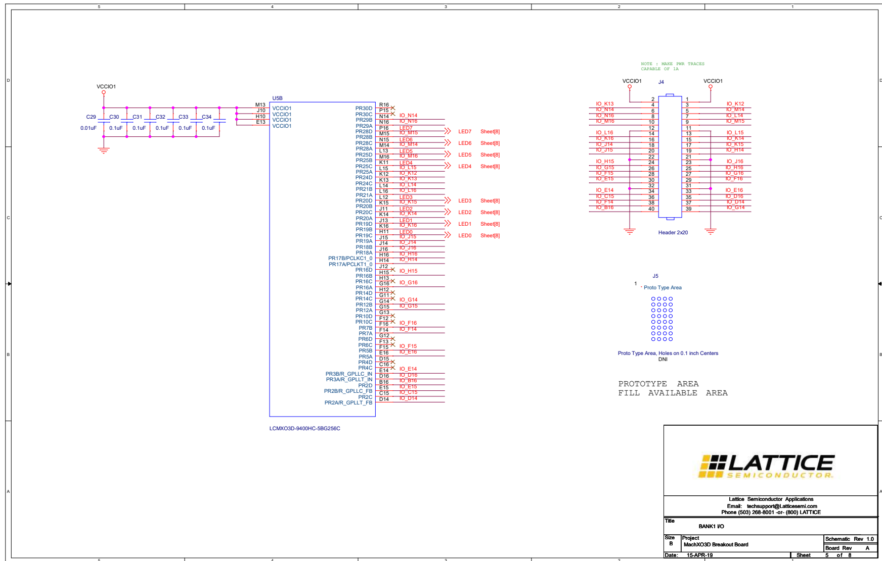
Figure A.5. Bank1 I/O
