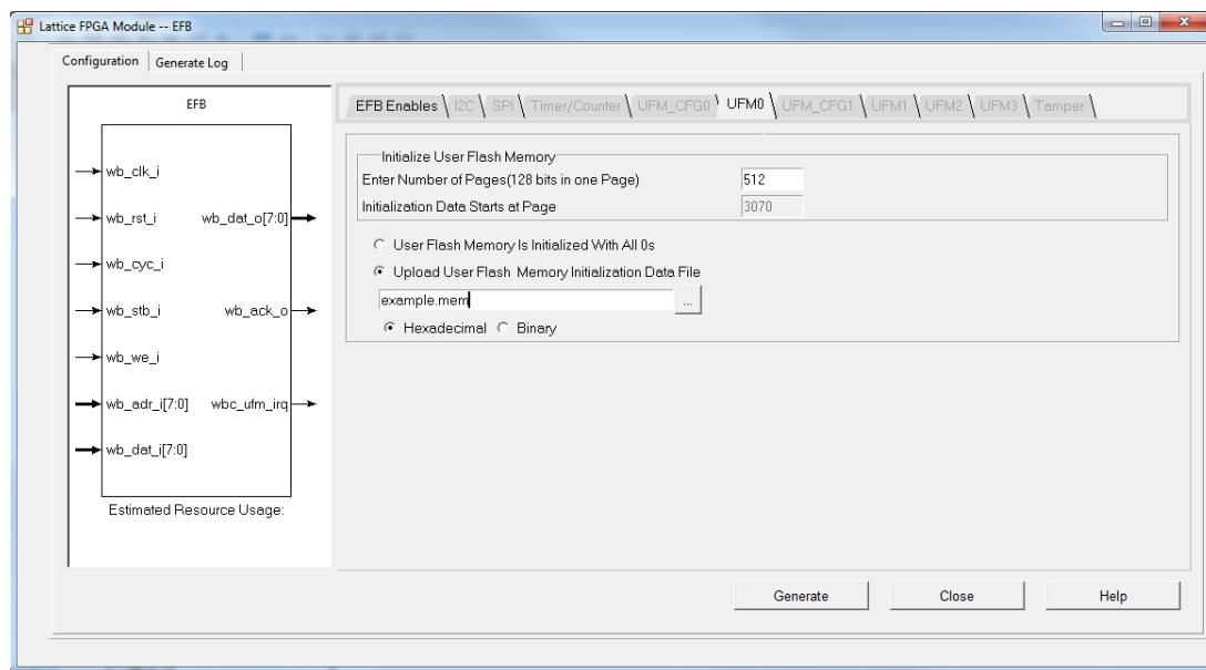
Figure 9.1. Initializing the UFM Sector with IPexpress
