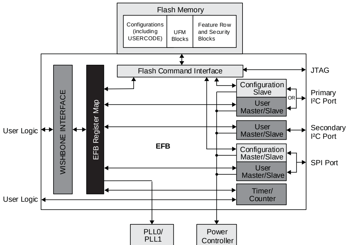
Figure 1.1. Embedded Functional Block
