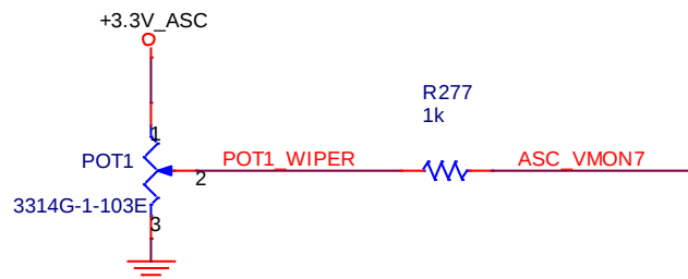
Figure 8.1. POT Circuit Design for VMON7
