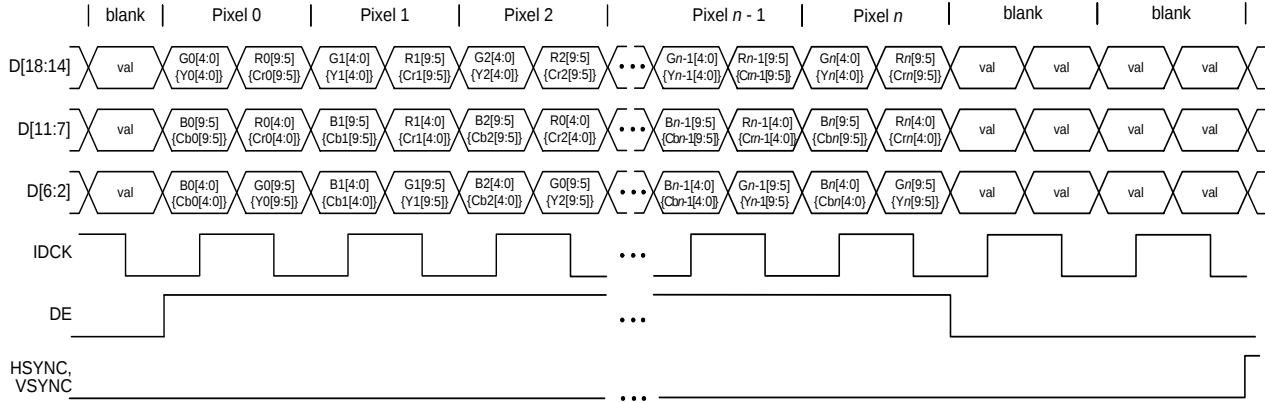
Figure 6.25. 10-Bit Color Depth 4:4:4 Dual Edge Timing
