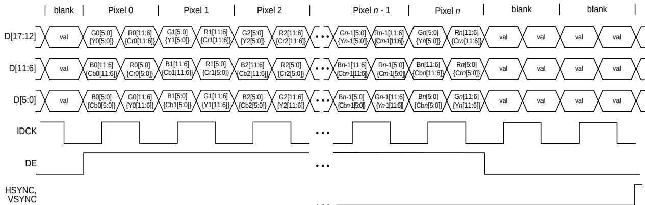
Figure 6.26. 12-Bit Color Depth 4:4:4 Dual Edge Timing
