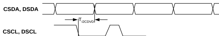
Figure 4.15. I²C Data Valid Delay (Driving Read Cycle Data)
