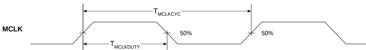
Figure 4.13. MCLK Timings
