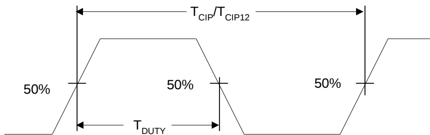
Figure 4.2. IDCK Clock Duty Cycle
