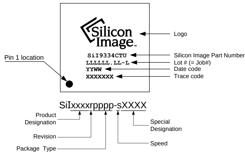
Figure 8.2. Marking Diagram
