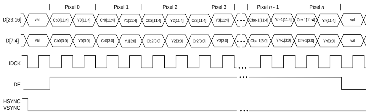
Figure 6.20. 12-Bit Color Depth YC Mux 4:2:2 Timing
