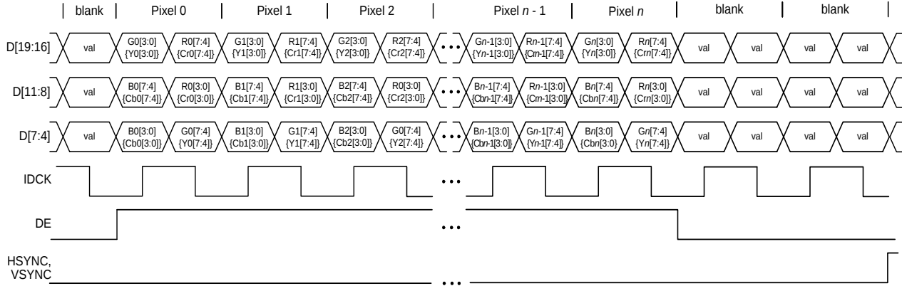
Figure 6.24. 8-Bit Color Depth 4:4:4 Dual Edge Timing
