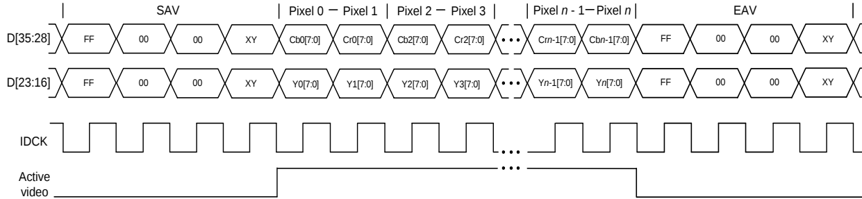
Figure 6.15. 8-Bit Color Depth YC 4:2:2 Embedded Sync Timing
