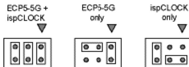
Figure 6.3. J50 Settings
