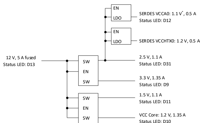
Figure 4.1. Power Distribution Scheme**
