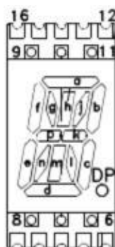
Figure 8.2. 14-Segment Display
