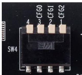
Figure 6.1. SW4
