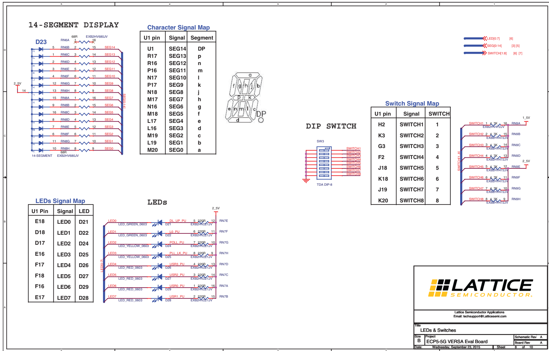
Figure A.8. LEDs and Switches
