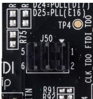
Figure 6.2. J50
