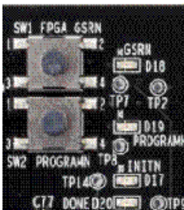
Figure 6.4. ECP5-5G Status LEDs and Push-button Controls
