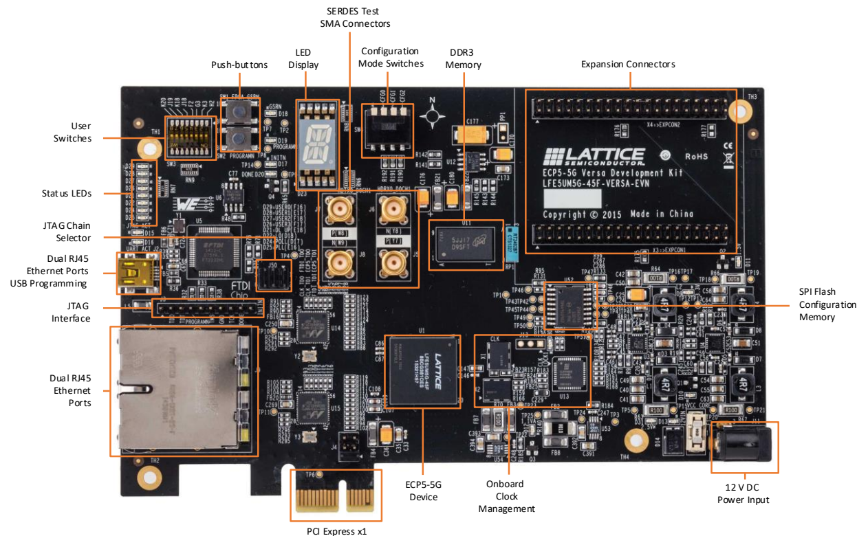
Figure 1.1. ECP5-5G Versa Development Board, Top Side
