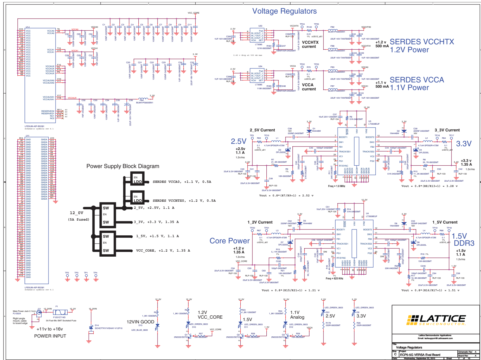
Figure A.2. Voltage Regulators (Refer to ECP5 and ECP5-5G Family Data Sheet (FPGA-DS-02012) for the V_{CCA} specifications of the latest production device)
