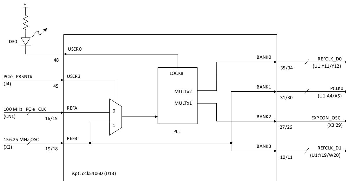
Figure 7.1. Clock Controller Scheme
