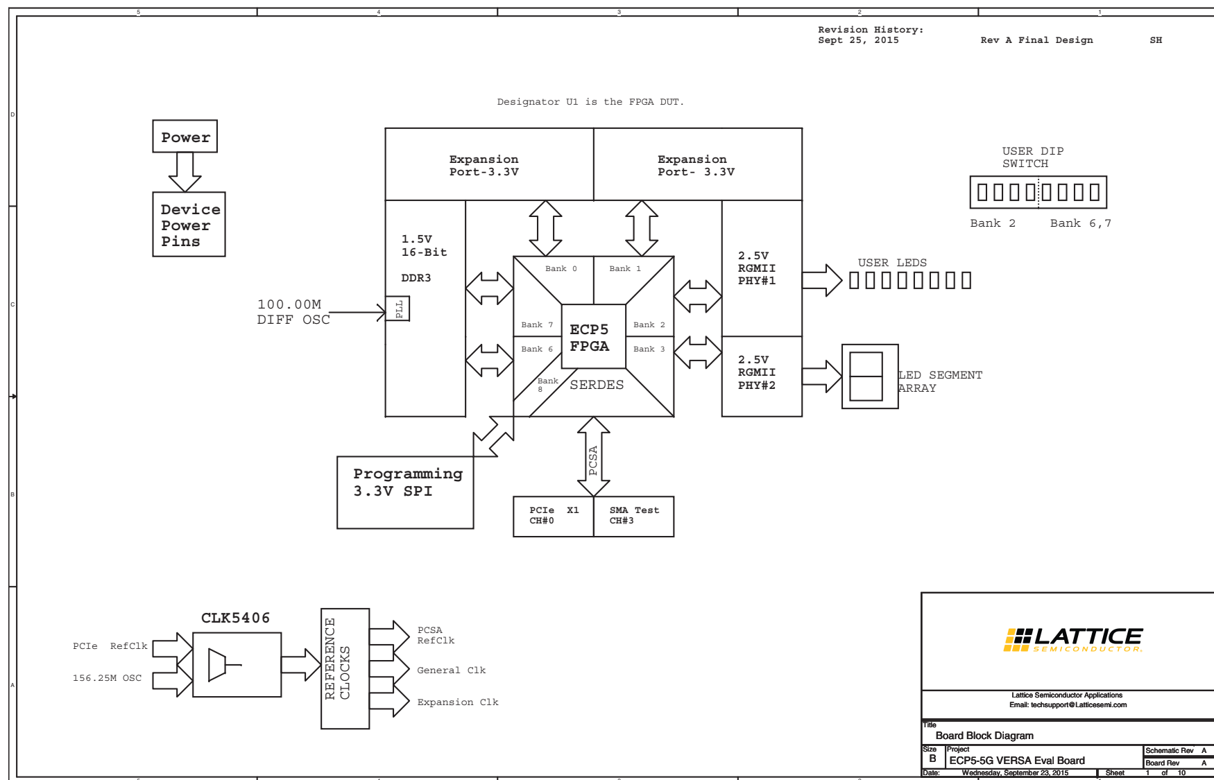
Figure A.1. Board Block Design
