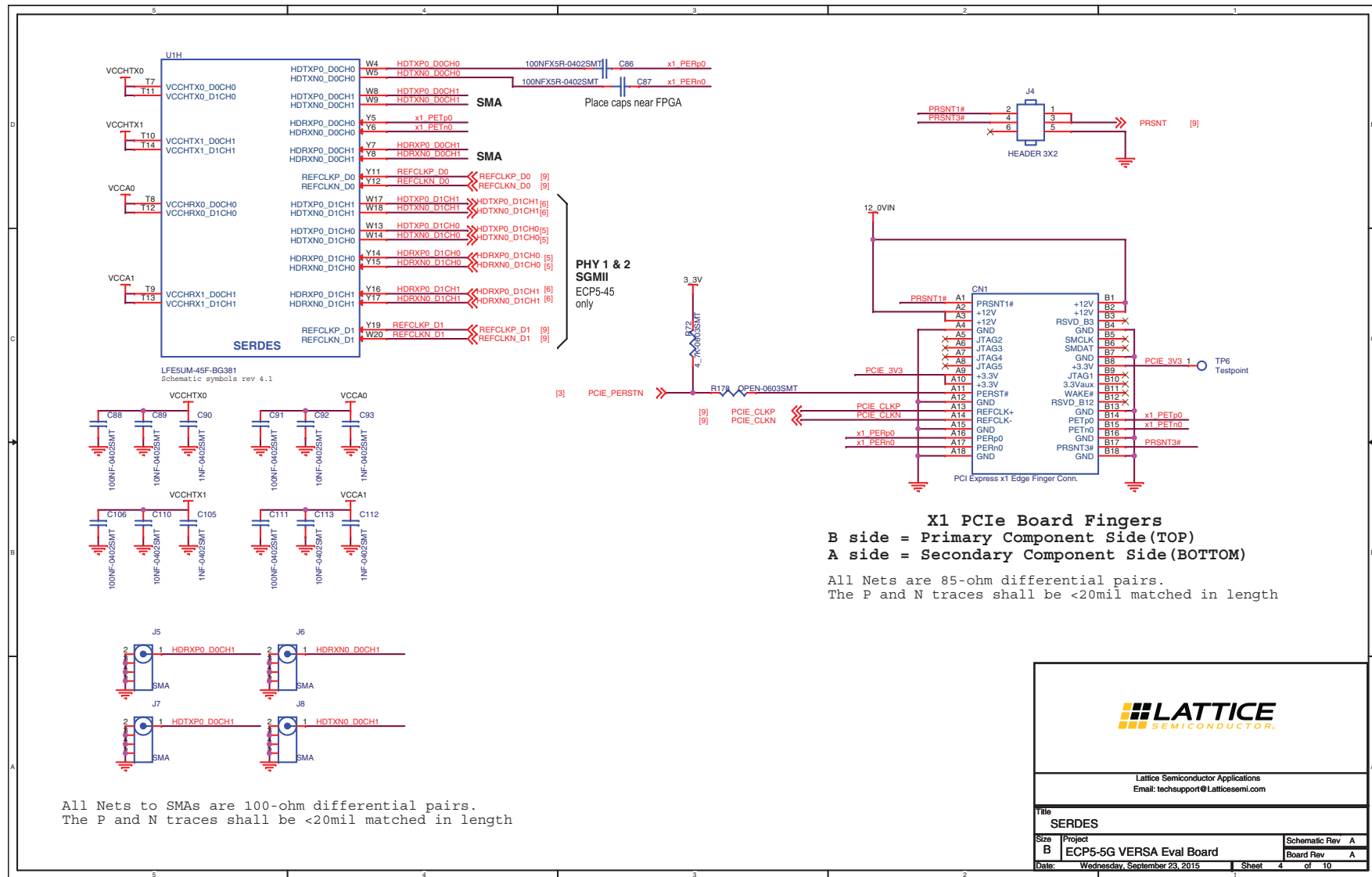
Figure A.4. SERDES
