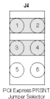
Figure 7.2. PCI Express PRSNT Control Connection
