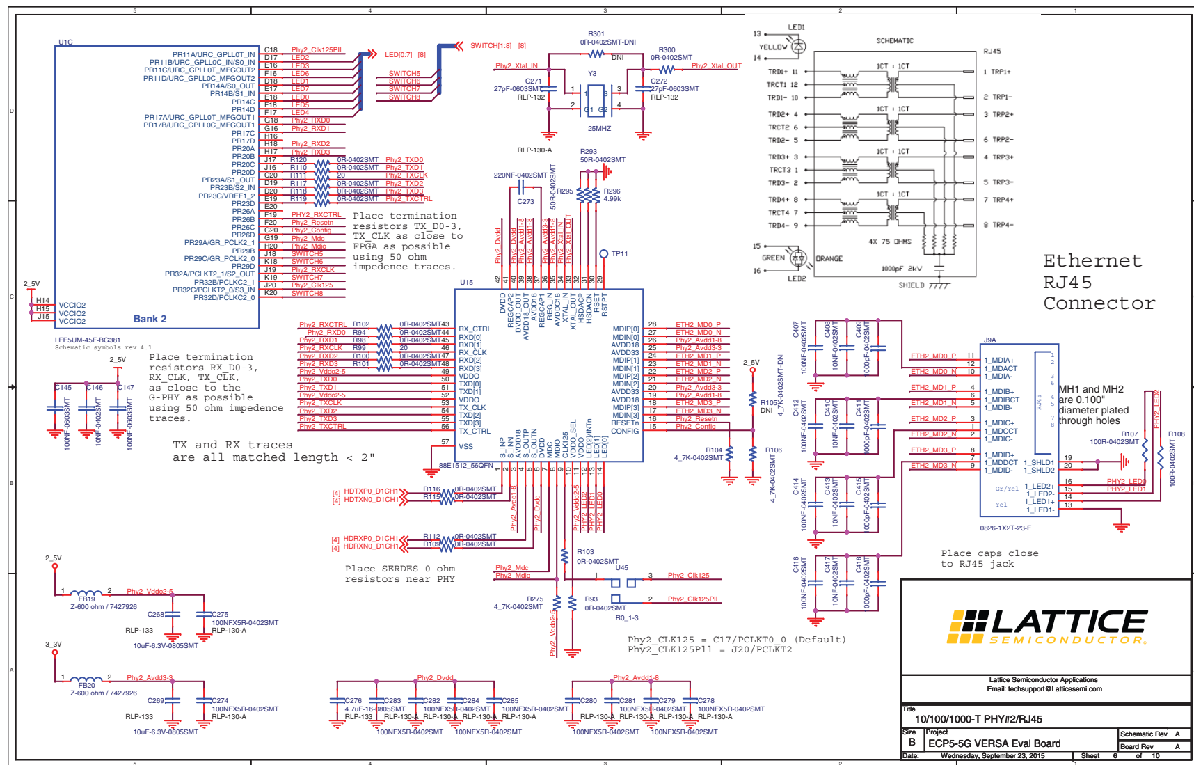
Figure A.6. 10/100/1000-T PHY #2/RJ45
