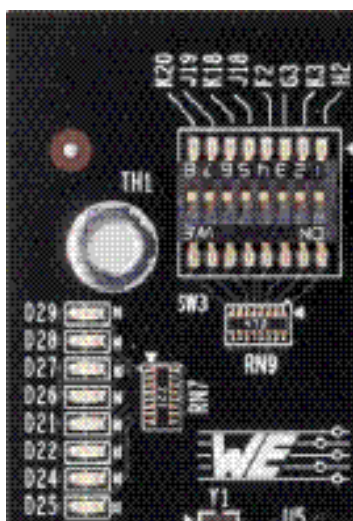
Figure 8.1. ECP5-5G Versa Development Board LEDs and Switches
