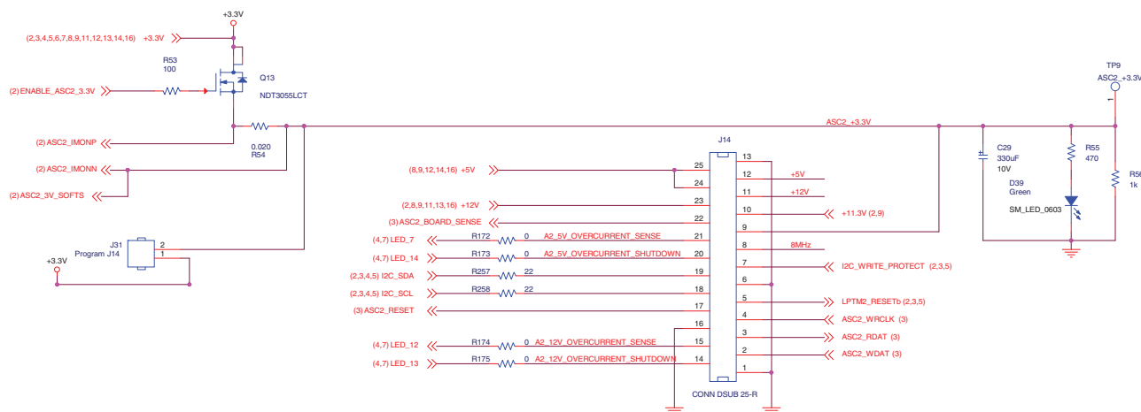
Figure 10. ASC0 IMON1 Monitors ASC2 Current and Supports Hot Swap Circuits
