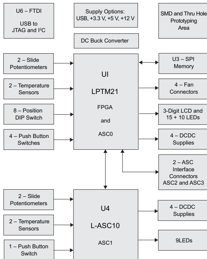
Figure 7. Platform Manager 2 Evaluation Board – Block Diagram
