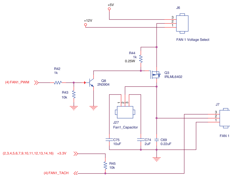
Figure 12. Fan 1 PWM Control Circuit
