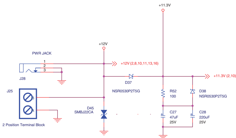
Figure 16. Fault Log Hold-Up Circuit for 12V
