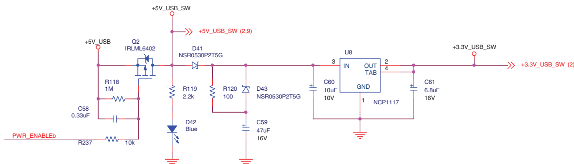
Figure 15. Fault Log Hold-Up Circuit for 5 V
