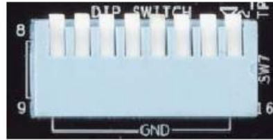
Figure 5.2. ECP5 Configuration Pin (CFG Pins)
