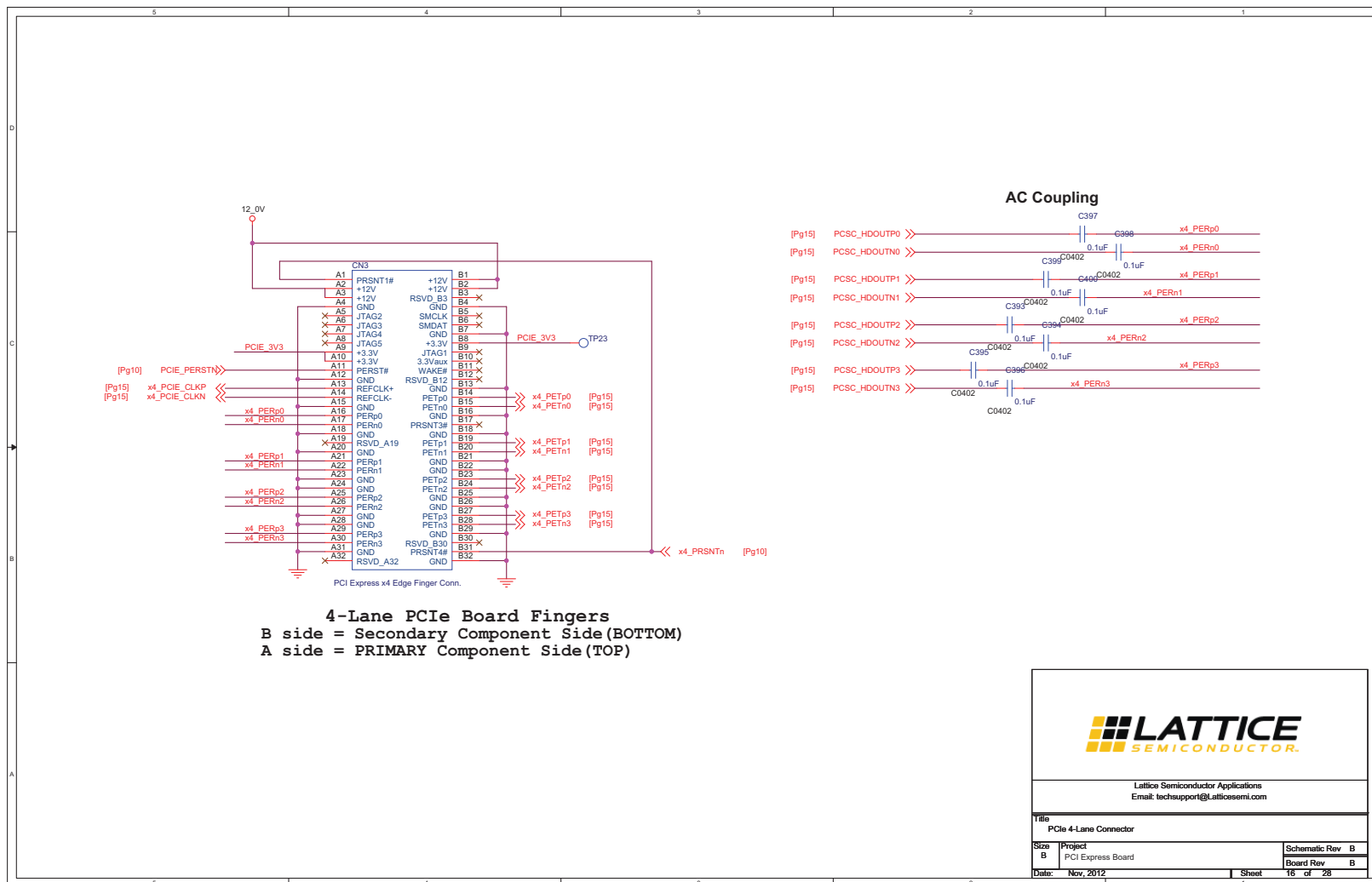
Figure B.15. PCIe 4-Lane Connector
