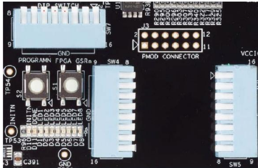
Figure 6.1. ECP5 PCI Express Board and LEDs and Switches
