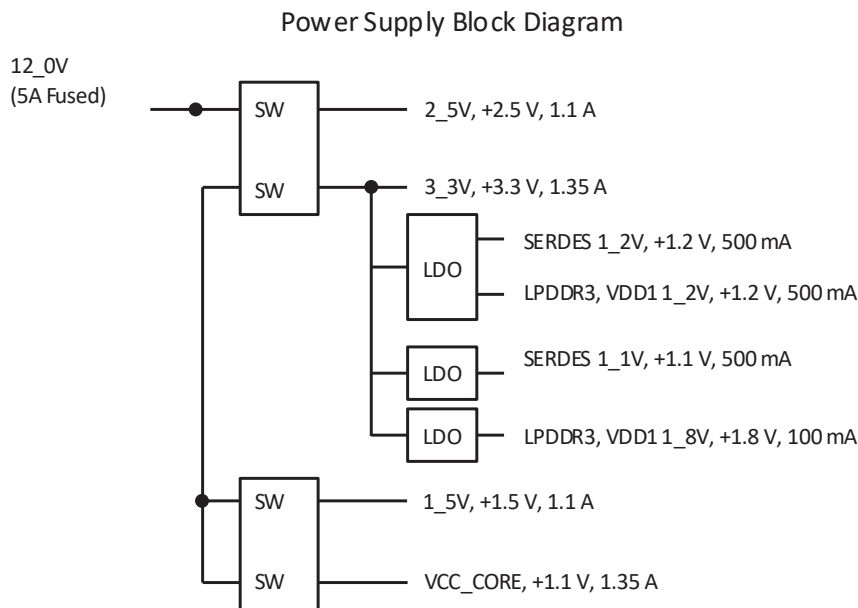
Figure 4.1. Power Distribution Scheme
