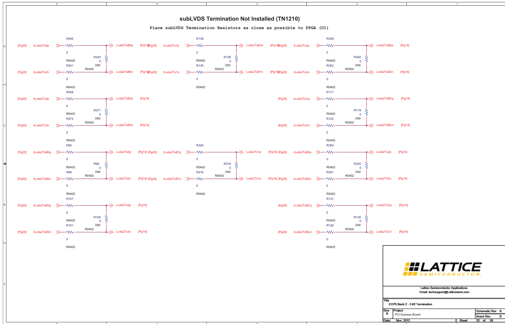
Figure B.21. ECP5 Bank 2 to Bank 3 #2 Termination
