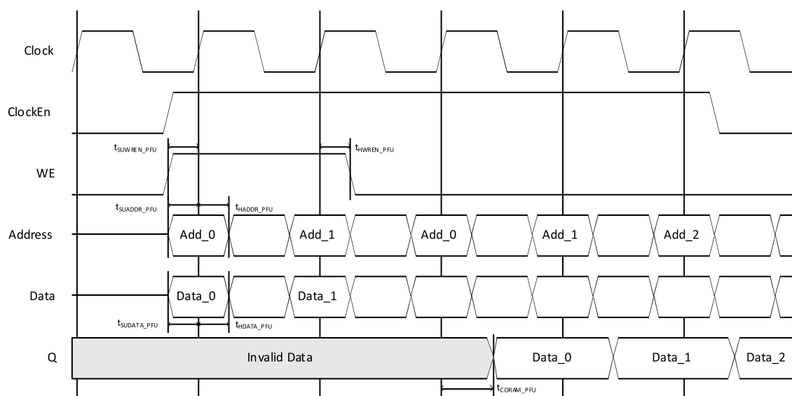
Figure 7.4. PFU-Based Distributed Single Port RAM Timing Waveform – Without Output Registers
