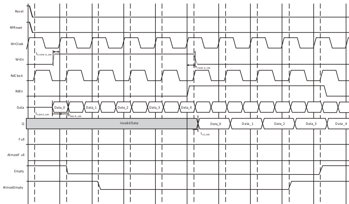
Figure 7.1. FIFO_DC Without Output Registers (Non-Pipelined)
