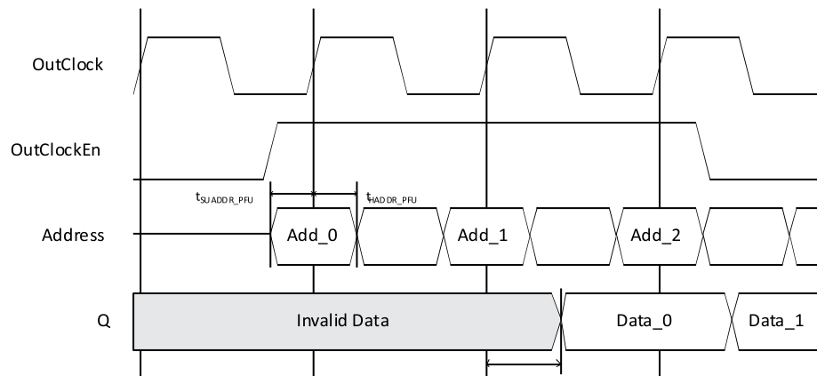
Figure 7.11. PFU-Based ROM Timing Waveform – With Output Registers
