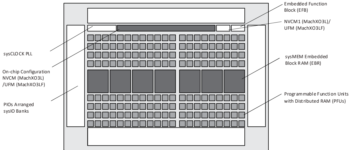
Figure 2.1. Top View of the MachXO3L/LF-1300 Device
