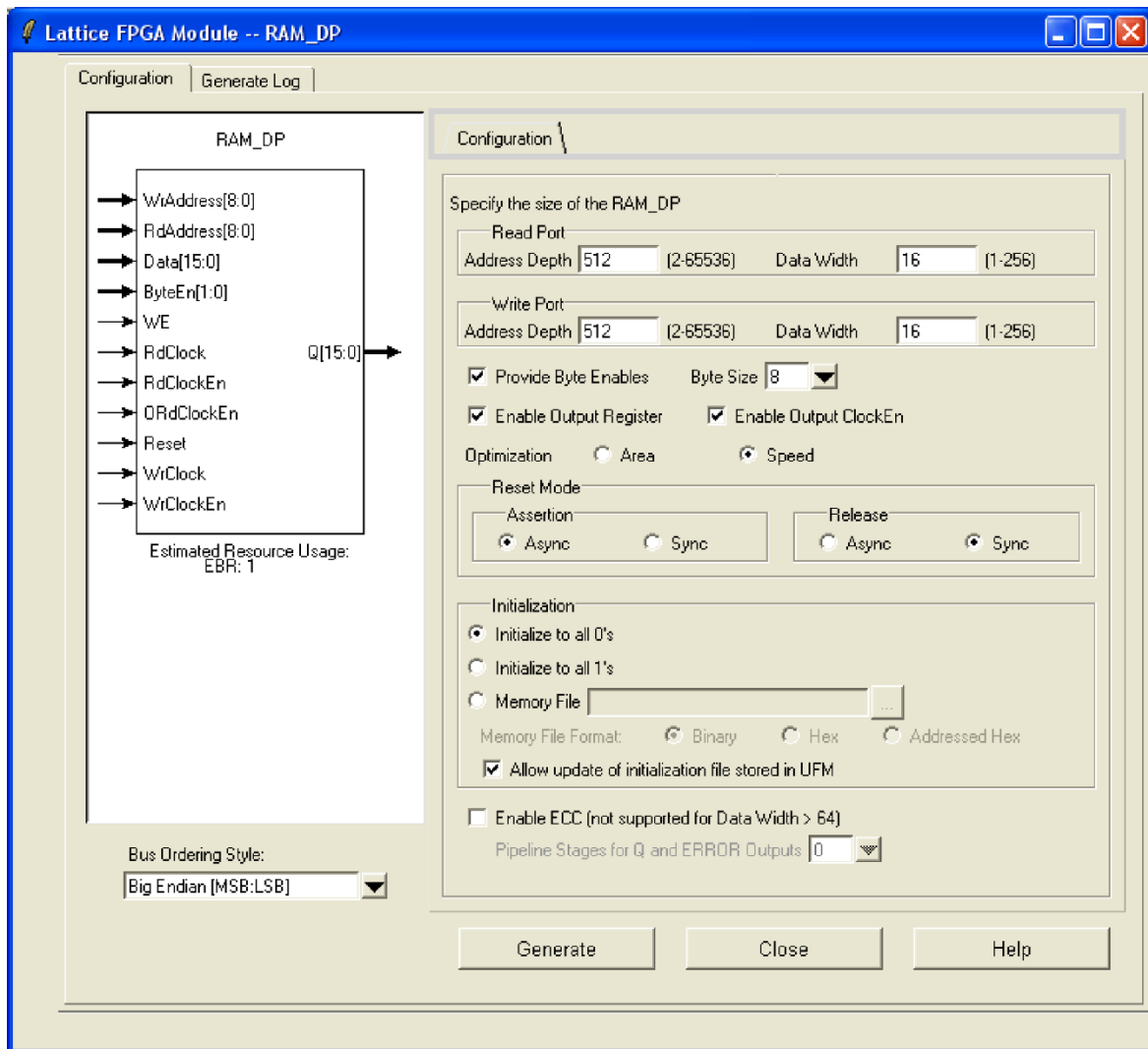
Figure 3.4 . Example Generating Pseudo Dual Port RAM (RAM_DP) Module Customization (MachXO3LF)
