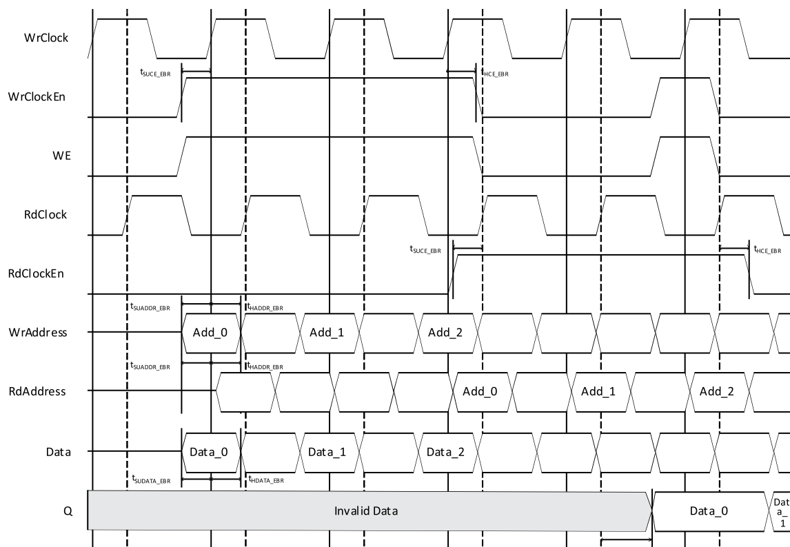
Figure 7.8. PFU-Based Distributed Dual Port RAM Timing Waveform – With Output Registers
