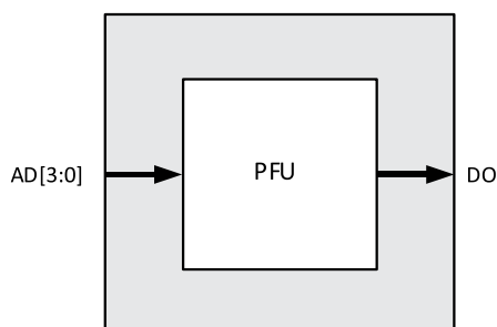
Figure 8.7. Distributed_ROM Primitive (ROM16X1A)
