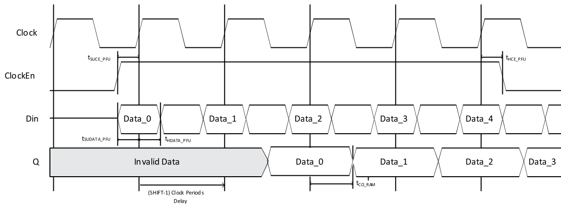
Figure 7.13. RAM-Based Shift Register Timing Waveform – Without Output Registers (Shift = 2)
