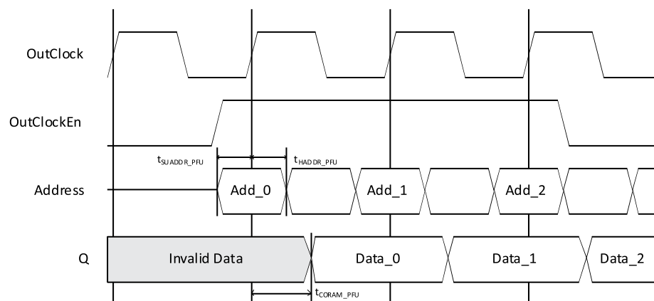
Figure 7.10. PFU-Based ROM Timing Waveform – Without Output Registers
