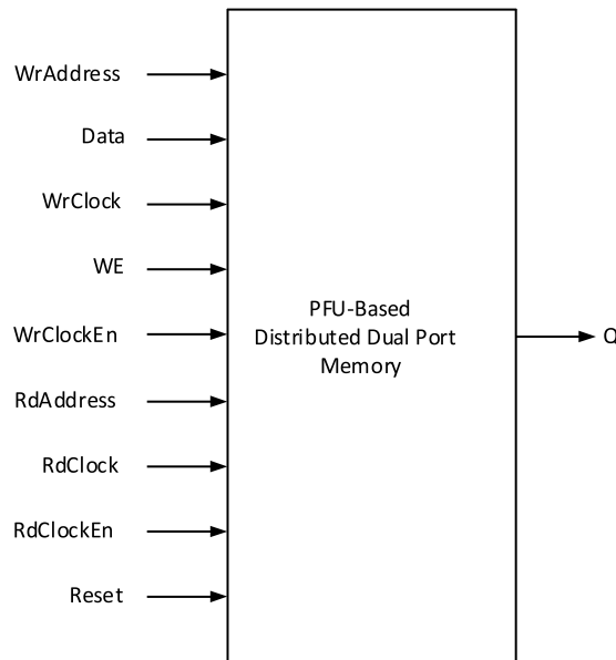
Figure 7.6. Distributed Dual Port RAM Module Generated by IPexpress
