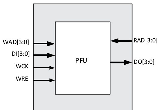
Figure 8.6. Distributed_DPRAM Primitive (DPR16X4C)
