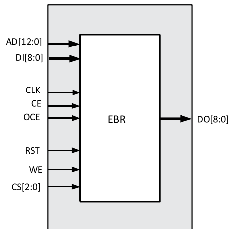
Figure 8.1. Single Port RAM (SP8KC)
