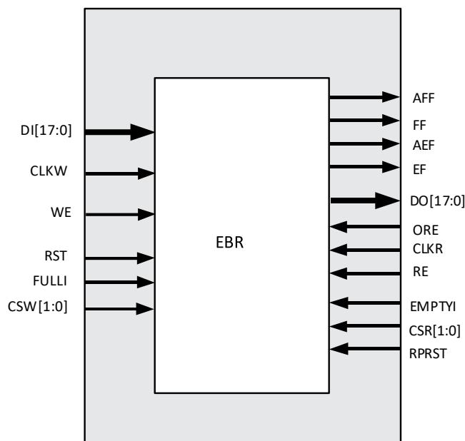
Figure 8.4. FIFO_DC Primitive (FIFO8KB)
