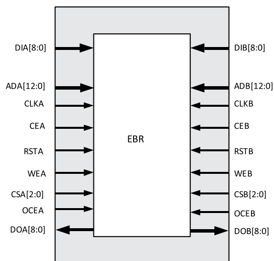
Figure 8.2. True Dual-Port RAM (DP8KC)
