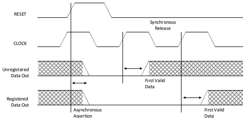
Figure 3.5. Asynchronous Reset with Synchronous Release
