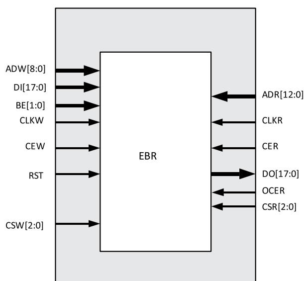
Figure 8.3. Pseudo Dual-Port RAM (PDPW8KC)
