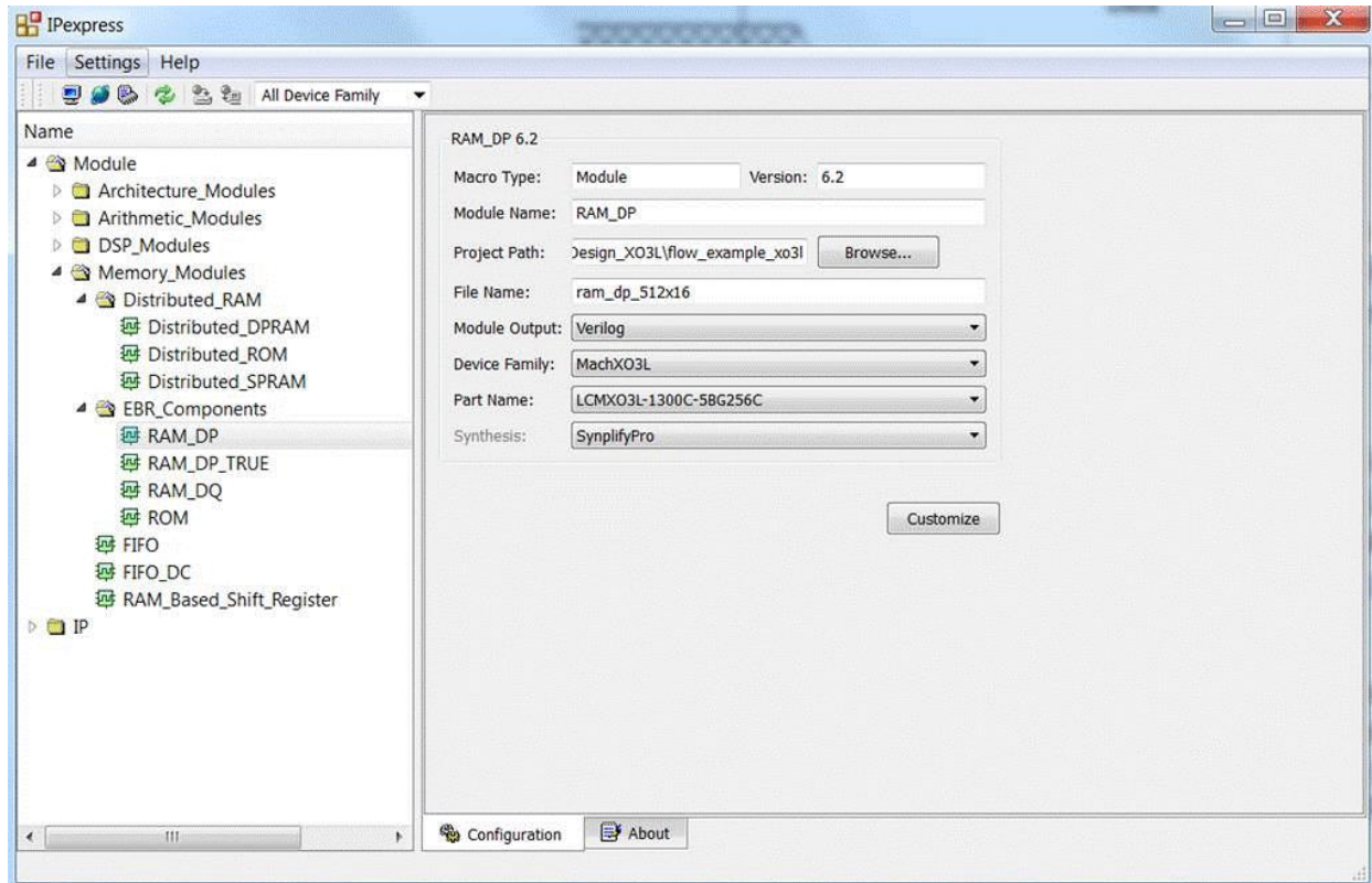
Figure 3.2. Example Generating Pseudo Dual Port RAM (RAM_DP) Using IPexpress
