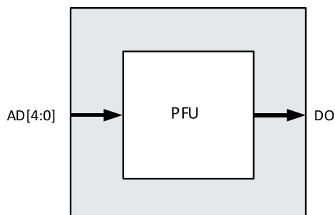
Figure 8.8. Distributed_ROM Primitive (ROM32X1A)
