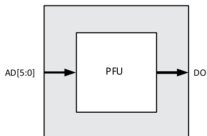
Figure 8.9. Distributed_ROM Primitive (ROM64X1A)
