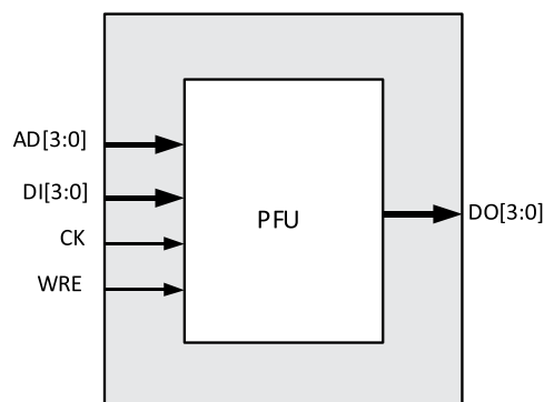
Figure 8.5. Distributed_SPRAM Primitive (SPR16X4C)
