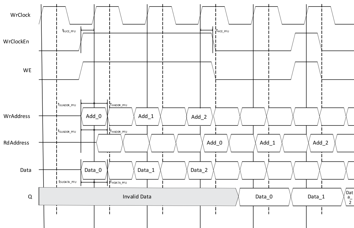
Figure 7.7. PFU-Based Distributed Dual Port RAM Timing Waveform – Without Output Registers
