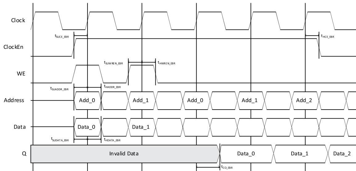
Figure 4.2. Single Port RAM Timing Waveform – NORMAL Mode, Without Output Registers
