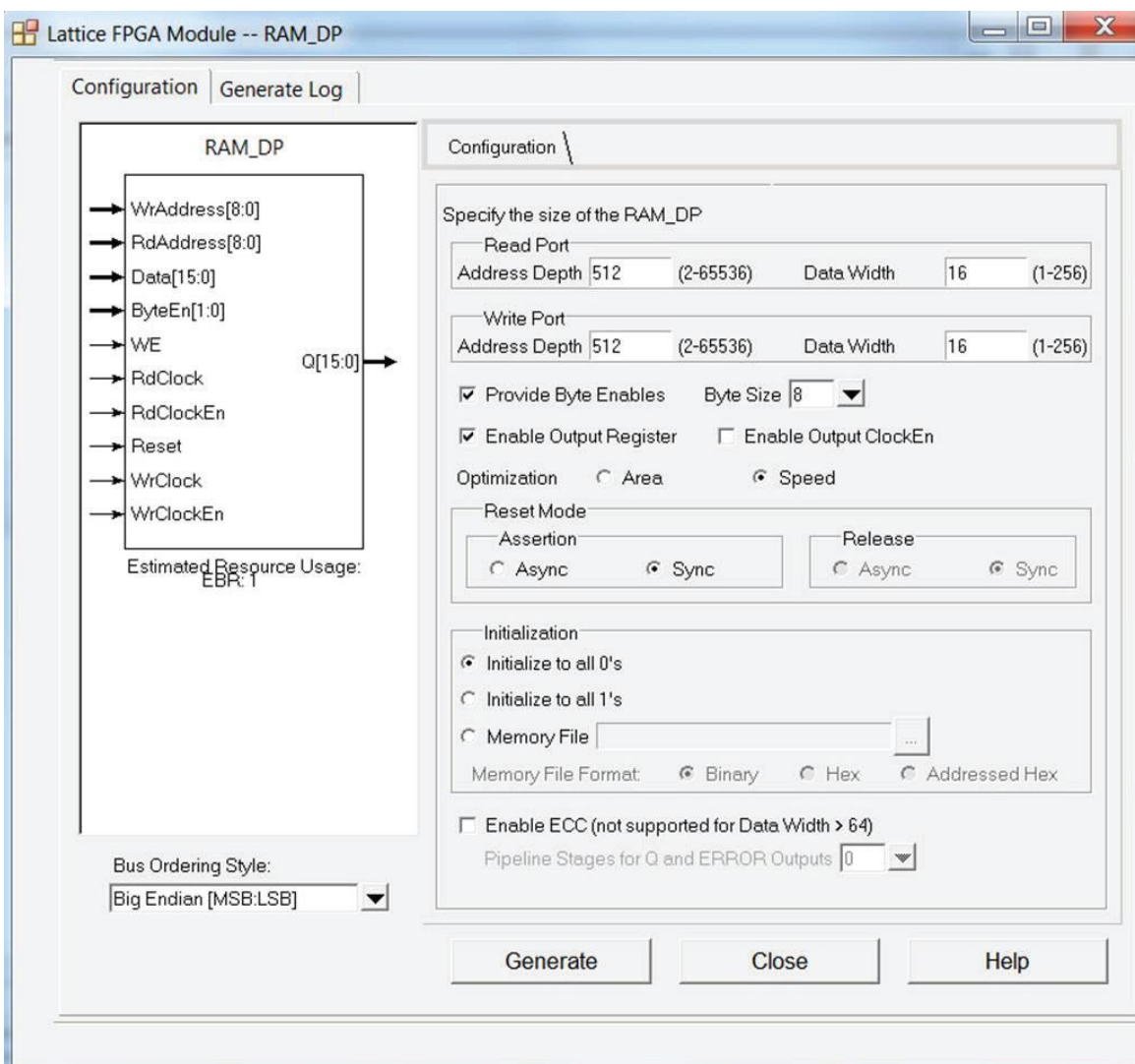
Figure 3.3. Example Generating Pseudo Dual Port RAM (RAM_DP) Module Customization (MachXO3L)
