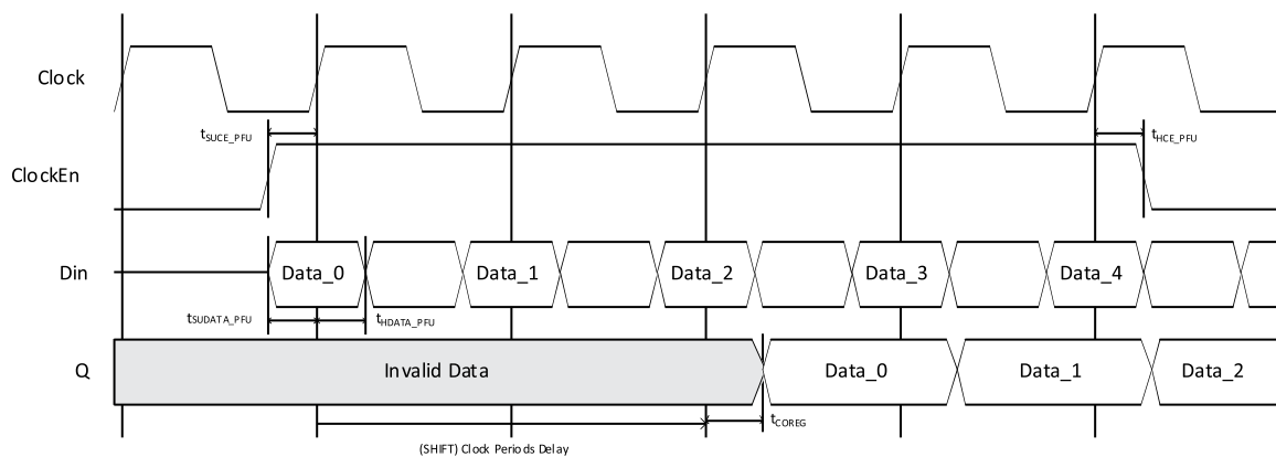
Figure 7.14. RAM-Based Shift Register Timing Waveform – With Output Registers (Shift = 2)
