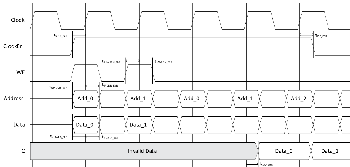
Figure 4.3. Single Port RAM Timing Waveform – NORMAL Mode, With Output Registers
