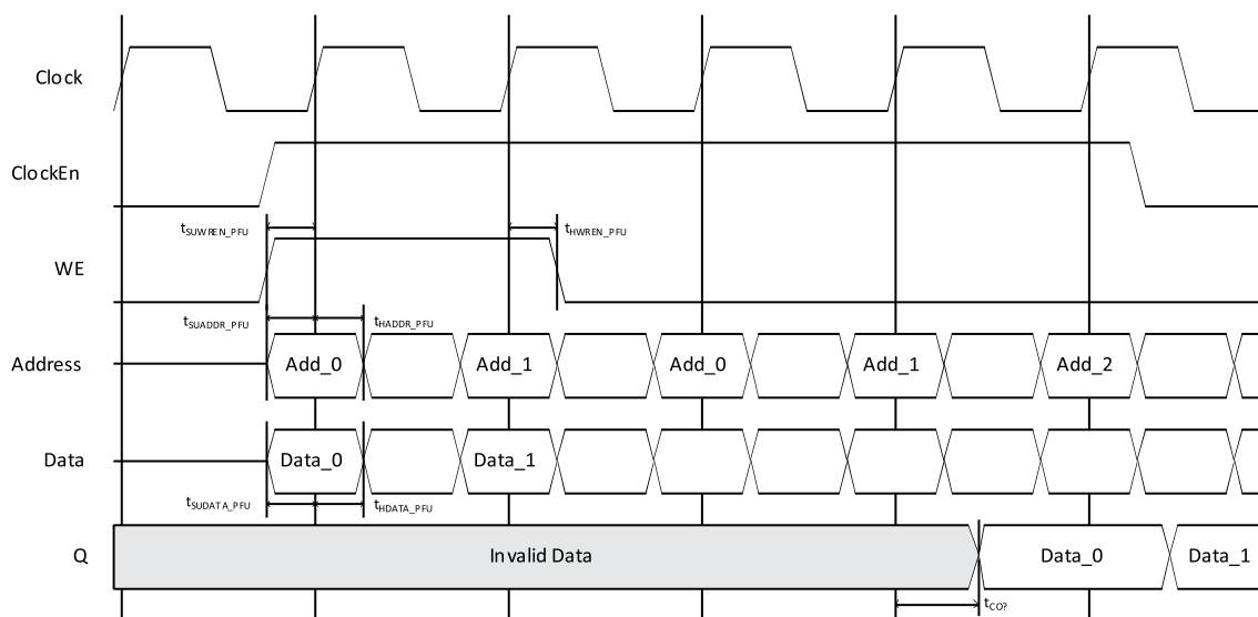
Figure 7.5. PFU- Based Distributed Single Port RAM Timing Waveform – With Output Registers
