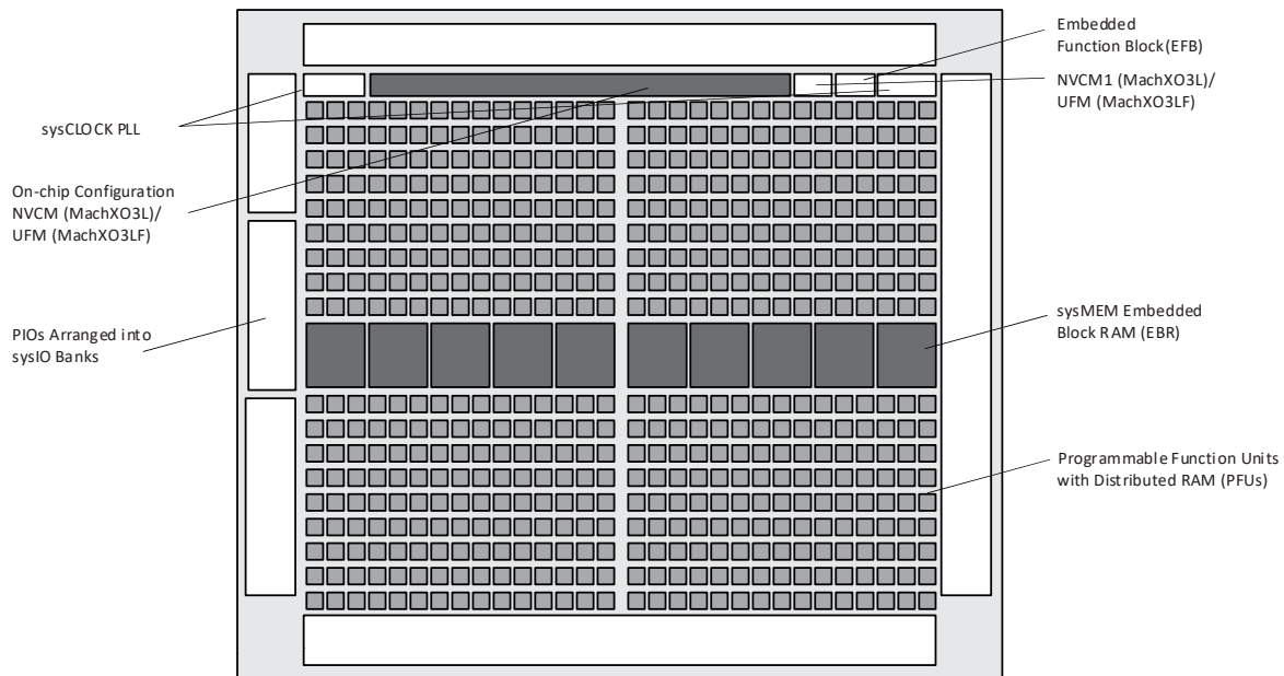
Figure 2.2. Top View of the MachXO3L/LF-4300 Device
