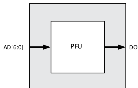
Figure 8.10. Distributed_ROM Primitive (ROM128X1A)
