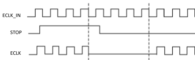
Figure 15.2. ECLKSYNC Functional Waveform
