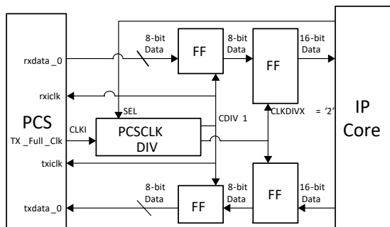
Figure 9.3. PCSCLKDIV Example Usage
