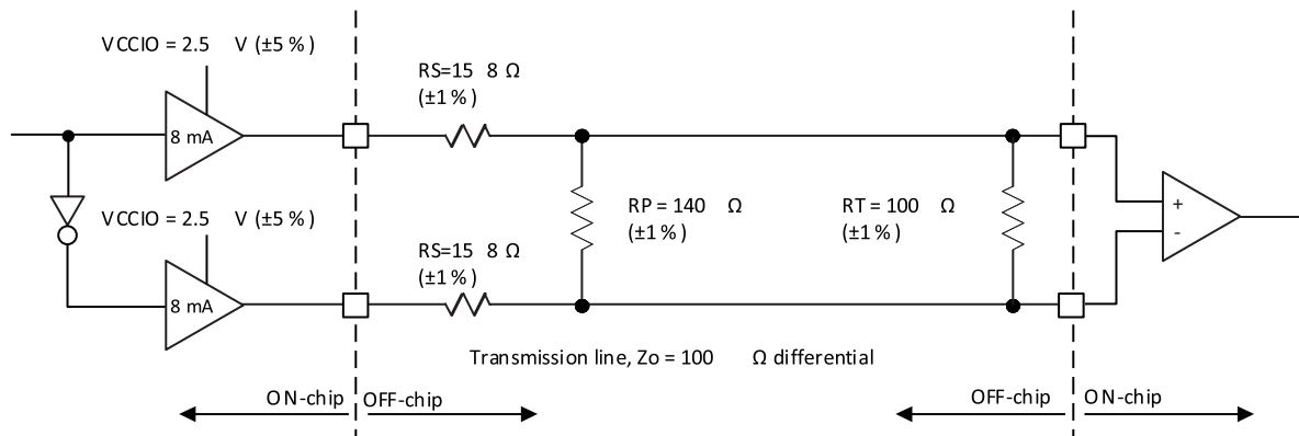
Figure 4.1. LVDS25E Output Termination Example
