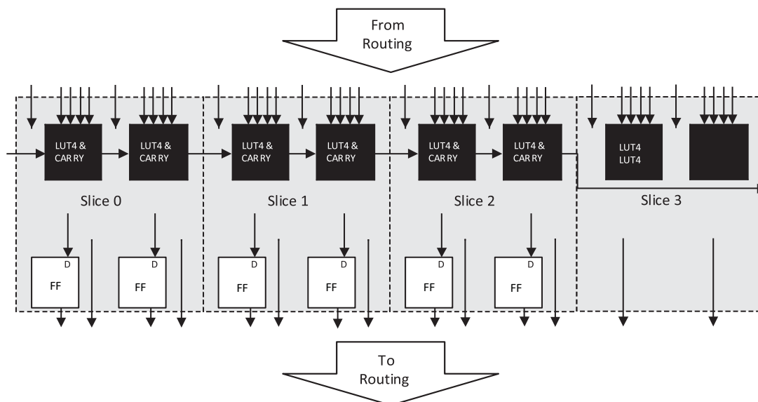
Figure 3.2. PFU Diagram
