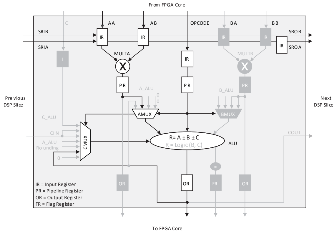
Figure 3.26. MAC DSP Element
