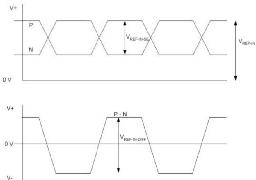
Figure 4.13. SERDES External Reference Clock Waveforms
