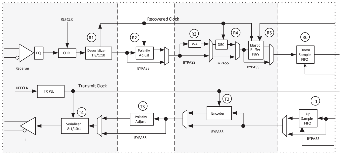
Figure 4.12. Transmitter and Receiver Latency Block Diagram
