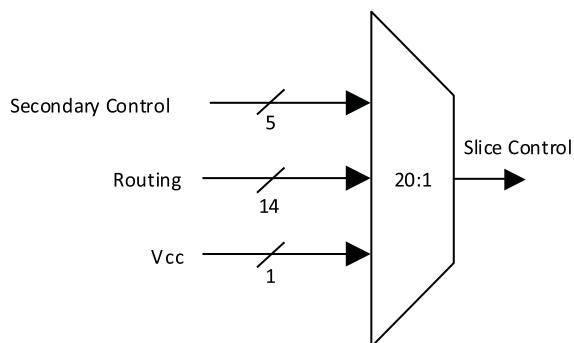
Figure 3.17. Slice 0 through Slice 2 Control Selection
