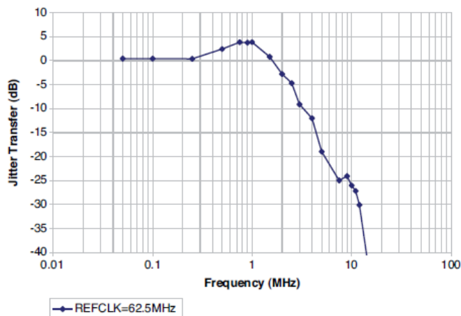
Figure 4.17. Jitter Transfer – 622 Mbps
