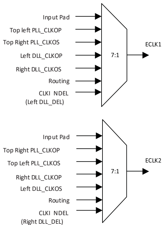
Figure 3.20. Sources of Edge Clock (Top Edge)
