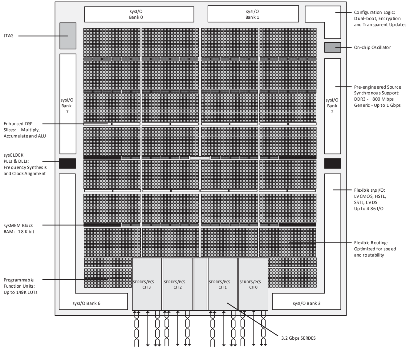
Figure 3.1. Simplified Block Diagram, LA-LatticeECP3-35 Device (Top Level)
