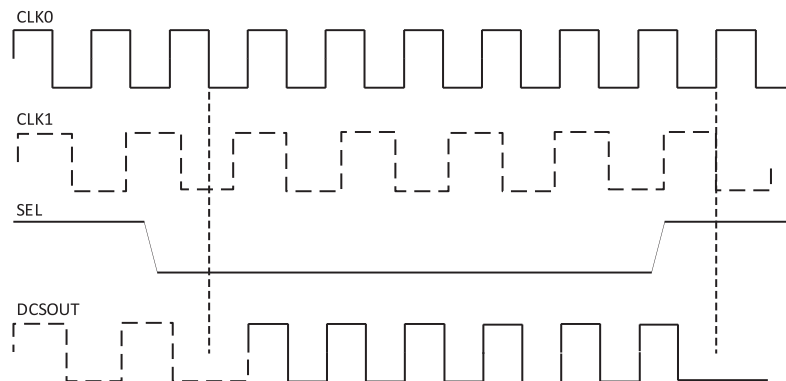
Figure 3.12. DCS Waveforms
