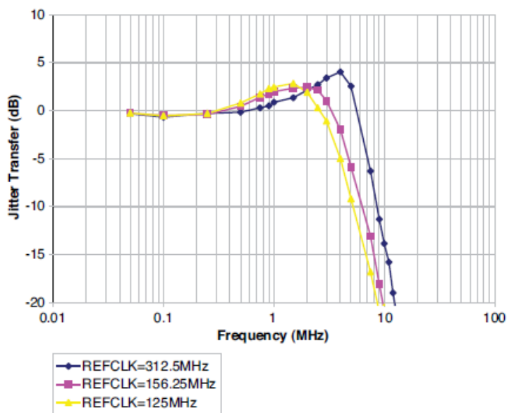
Figure 4.14. Jitter Transfer – 3.125 Gbps
