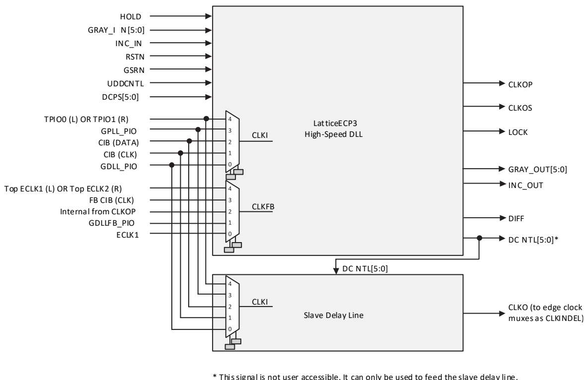
Figure 3.6. Top-Level Block Diagram, High-Speed DLL and Slave Delay Line
