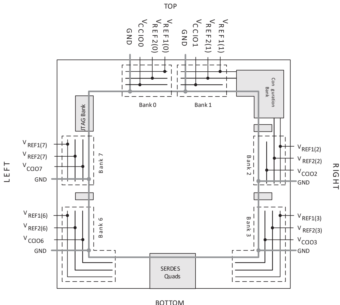
Figure 3.37. LA-LatticeECP3 Banks
