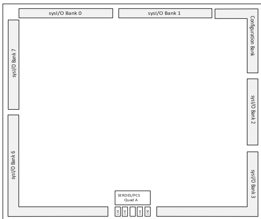
Figure 3.39. SERDES/PCS Quads (LA-LatticeECP3-35)
