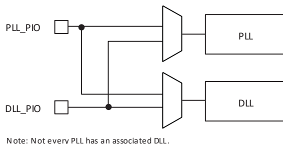
Figure 3.7. Sharing of PIO Pins by PLLs and DLLs in LA-LatticeECP3 Devices
