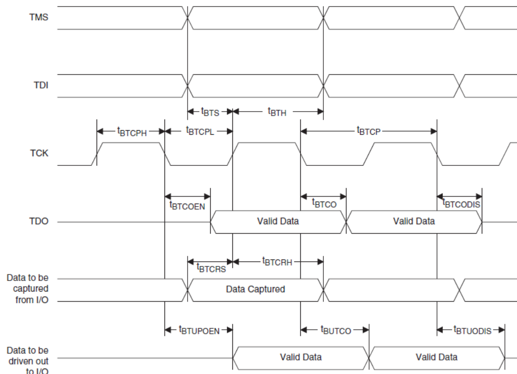
Figure 4.29. JTAG Port Timing Waveforms
