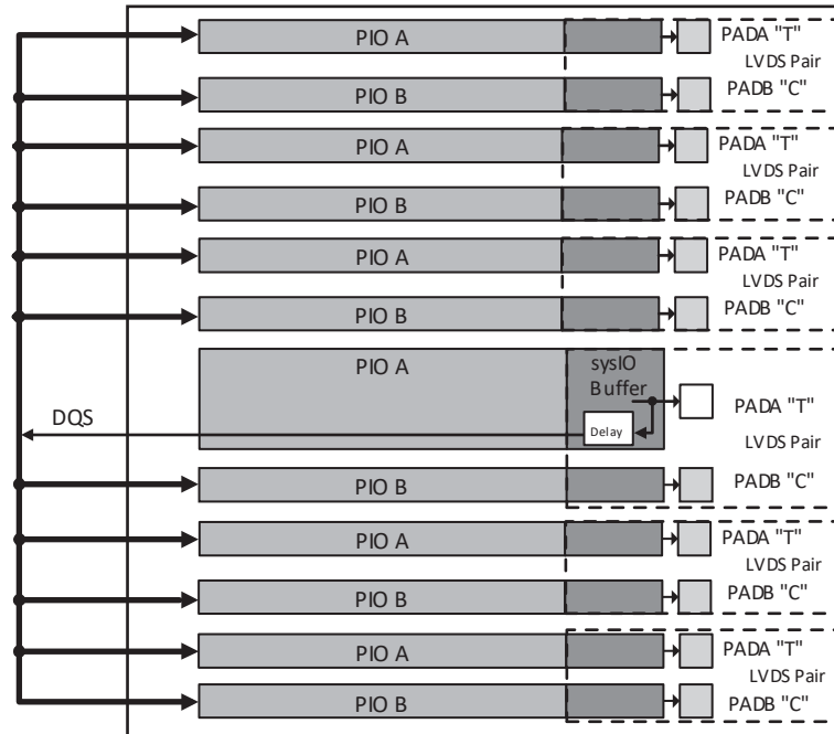
Figure 3.34. DQS Grouping on the Left, Right and Top Edges
