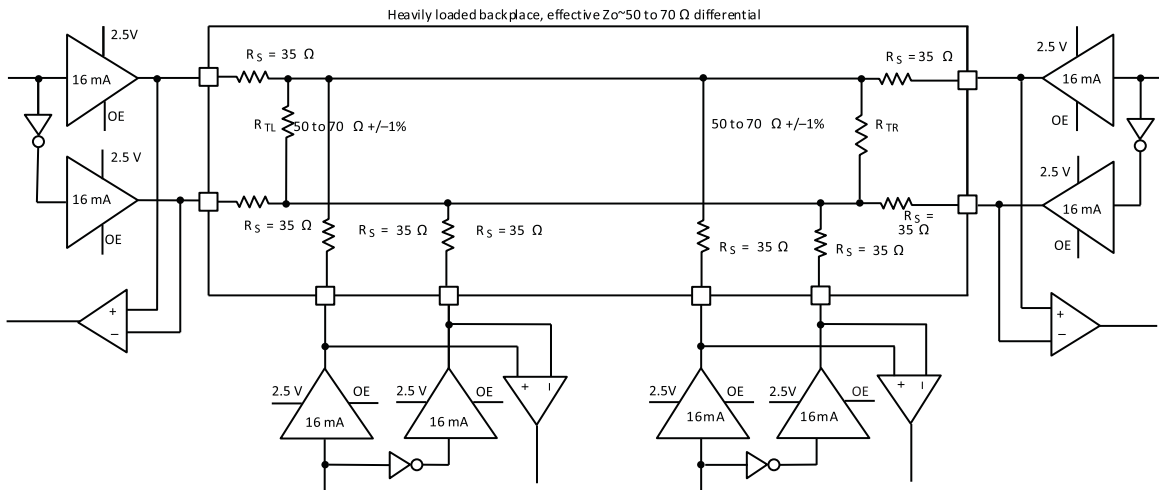
Figure 4.5. MLVDS25 (Multipoint Low Voltage Differential Signaling)
