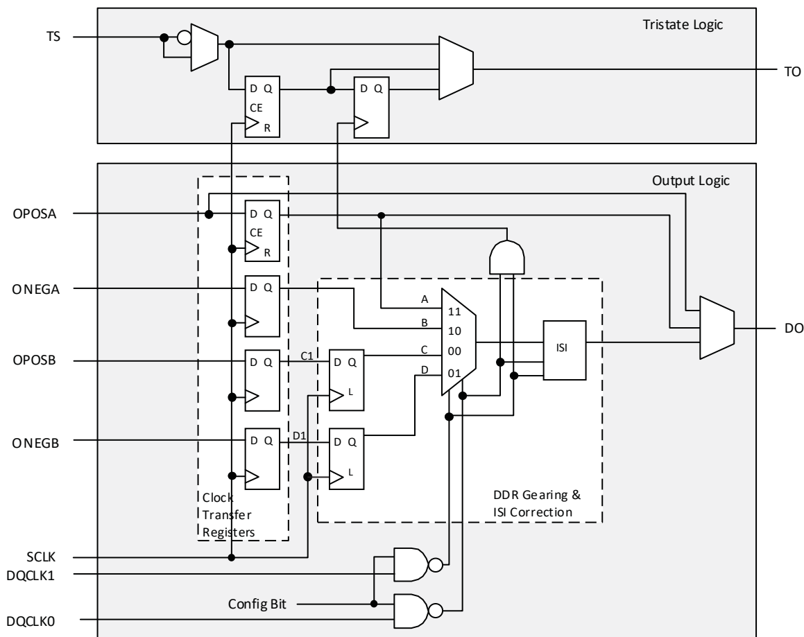
Figure 3.33. Output and Tristate Block for Left and Right Edges
