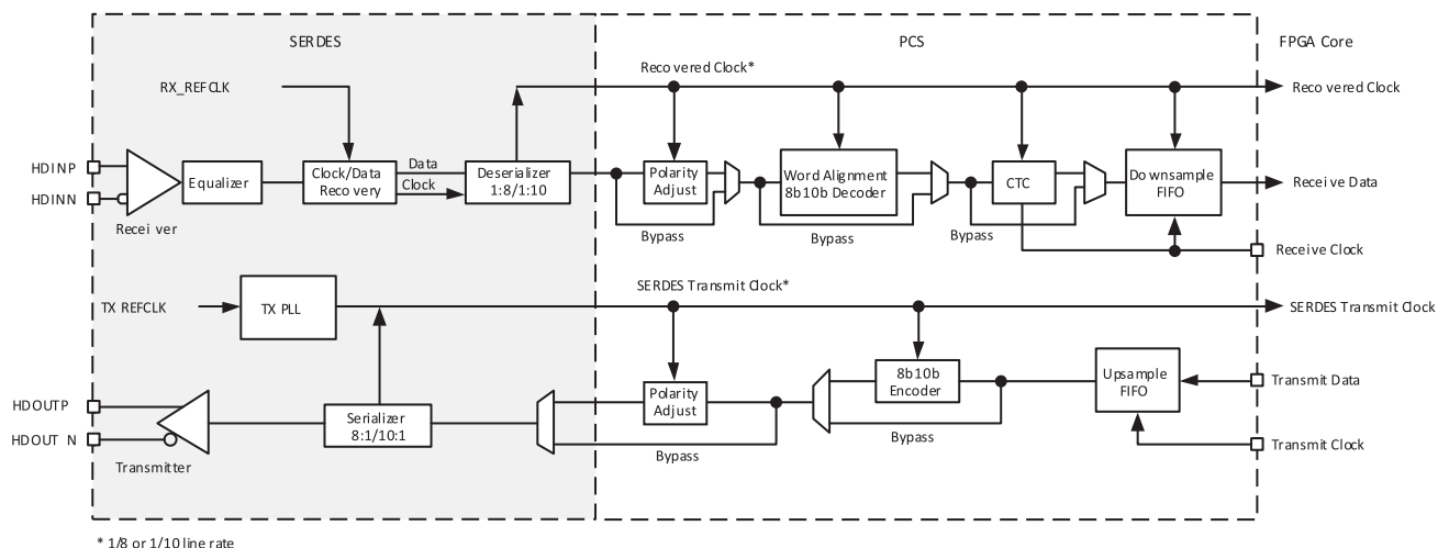
Figure 3.40. Simplified Channel Block Diagram for SERDES/PCS Block
