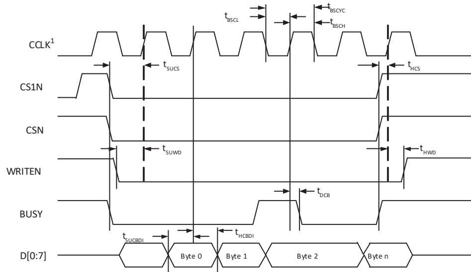
Figure 4.21. sysCONFIG Parallel Port Write Cycle
