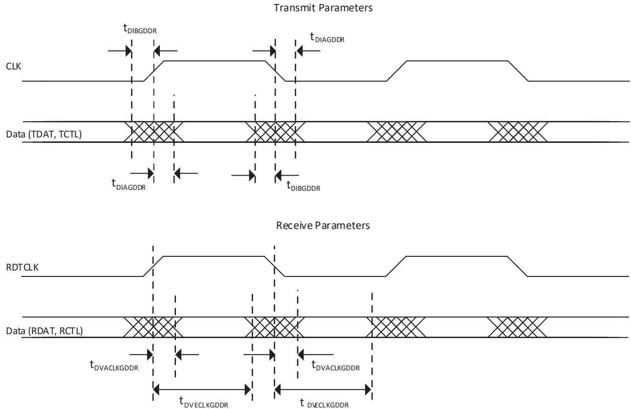
Figure 4.6. Generic DDR1/DDR2 (With Clock and Data Edges Aligned)
