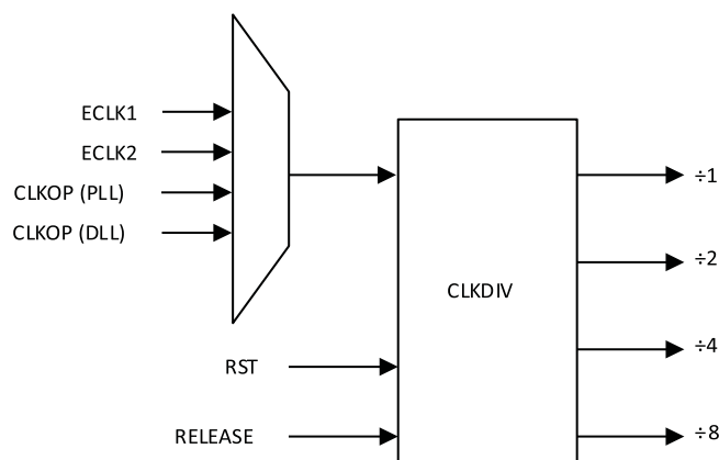
Figure 3.8. Clock Divider Connections
