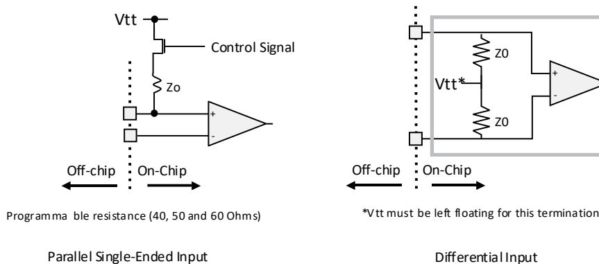
Figure 3.38. On-Chip Termination
