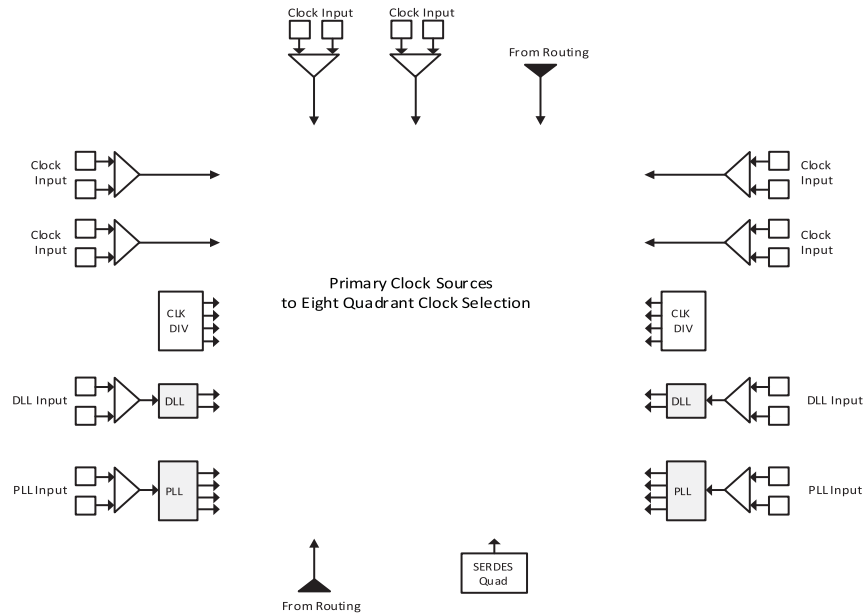
Figure 3.9. Primary Clock Sources for LA-LatticeECP3-17
