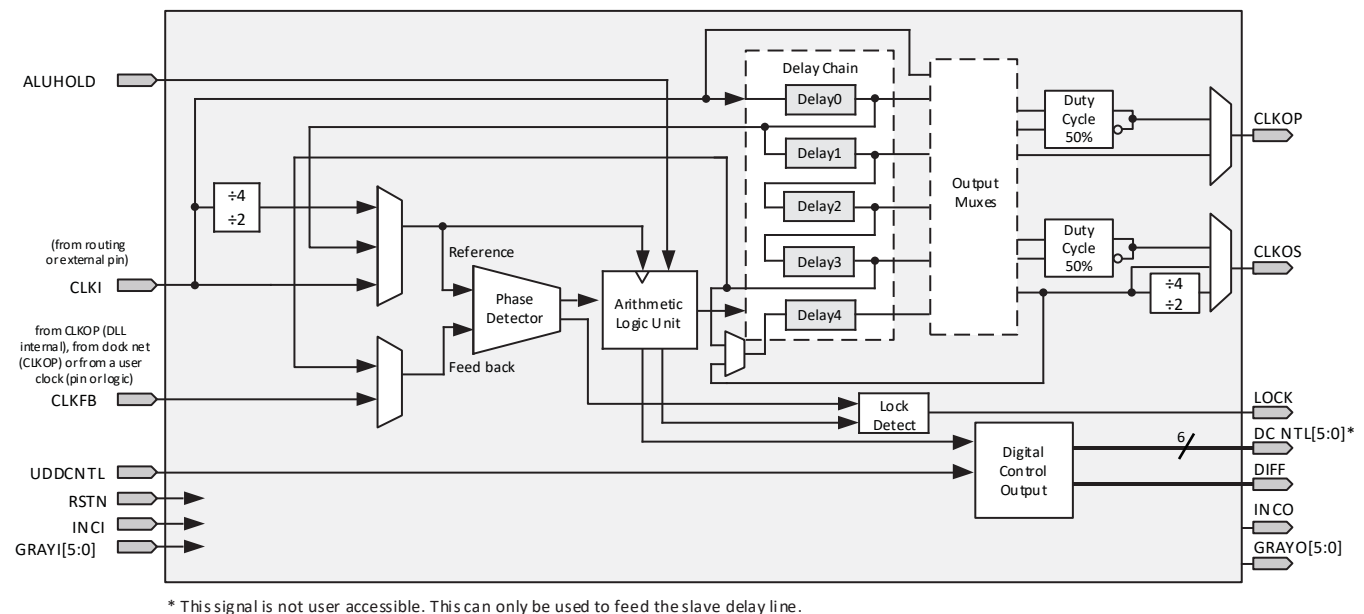
Figure 3.5. Delay Locked Loop Diagram (DLL)
