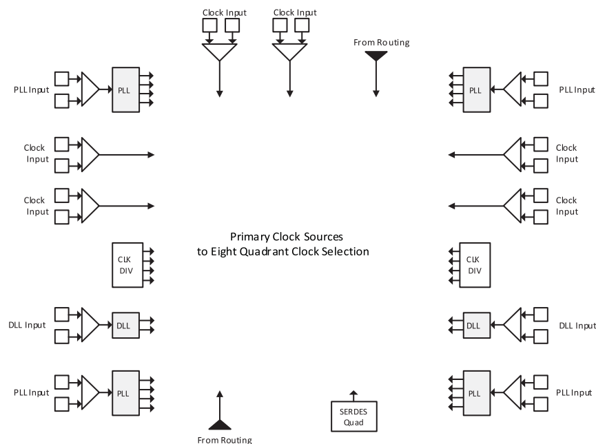
Figure 3.10. Primary Clock Sources for LA-LatticeECP3-35
