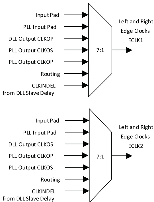
Figure 3.19. Sources of Edge Clock (Left and Right Edges)
