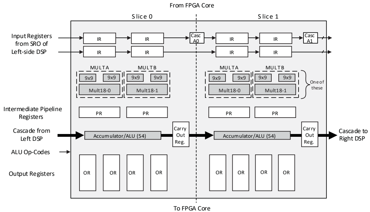
Figure 3.23. Simplified sysDSP Slice Block Diagram
