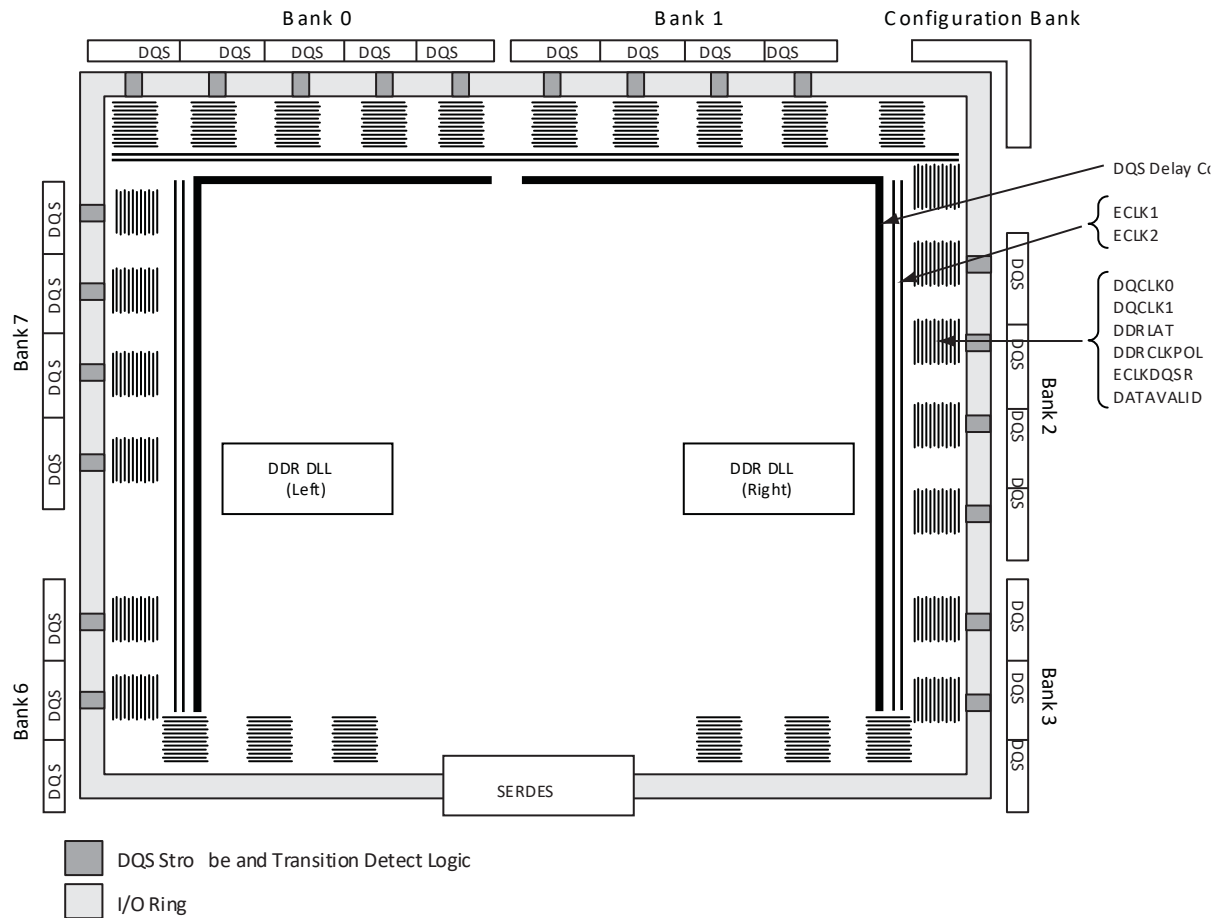
Figure 3.35. Edge Clock, DLL Calibration and DQS Local Bus Distribution
