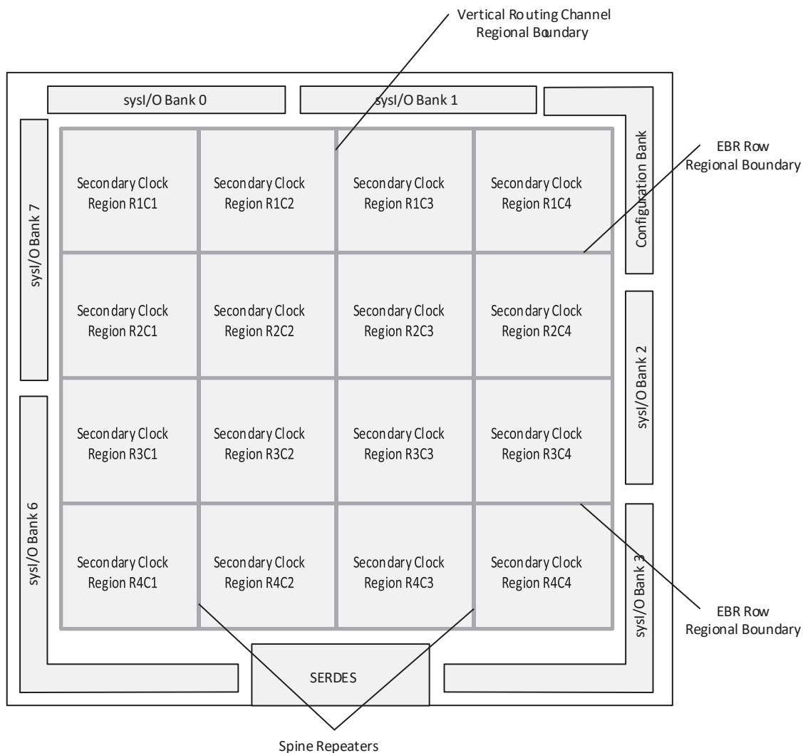
Figure 3.14. LA-LatticeECP3-17 and LA-LatticeECP3-35 Secondary Clock Regions
