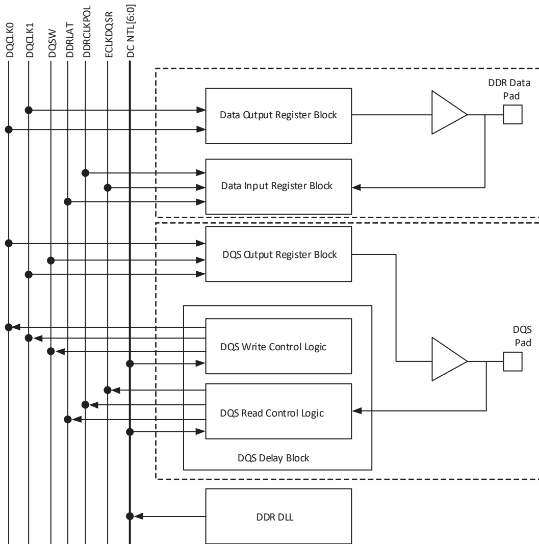
Figure 3.36. DQS Local Bus
