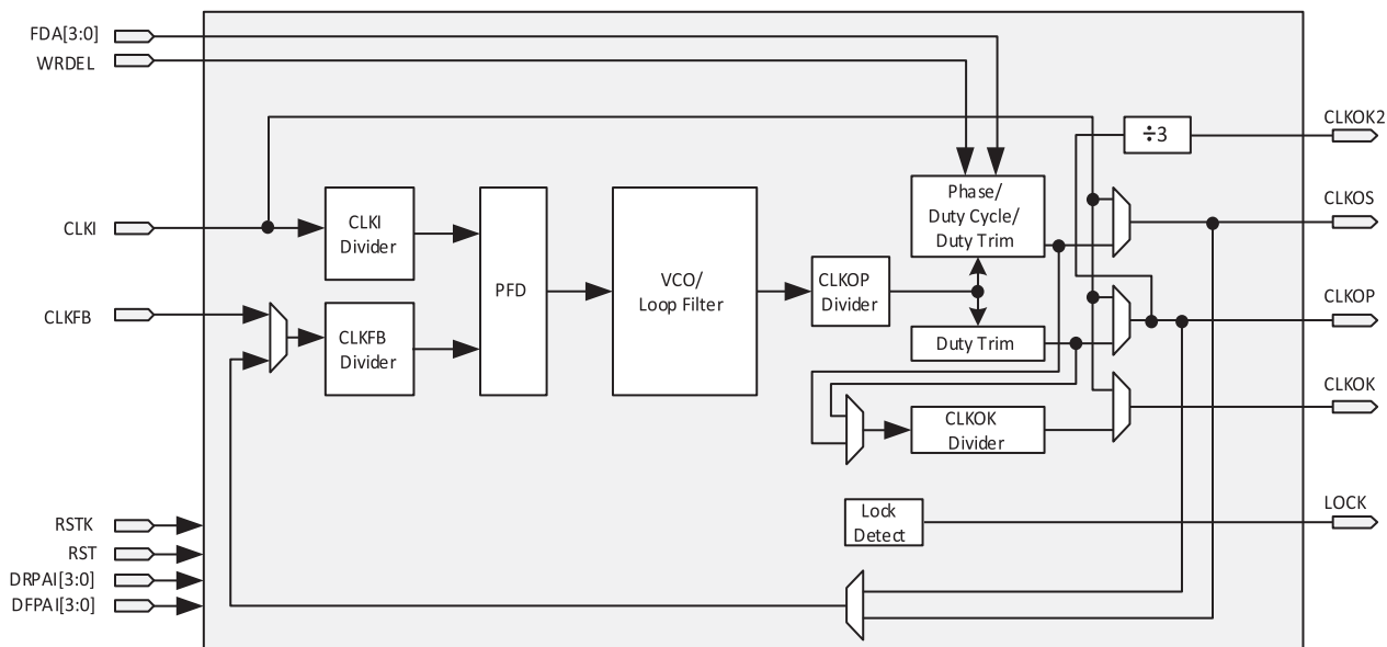
Figure 3.4. General Purpose PLL Diagram
