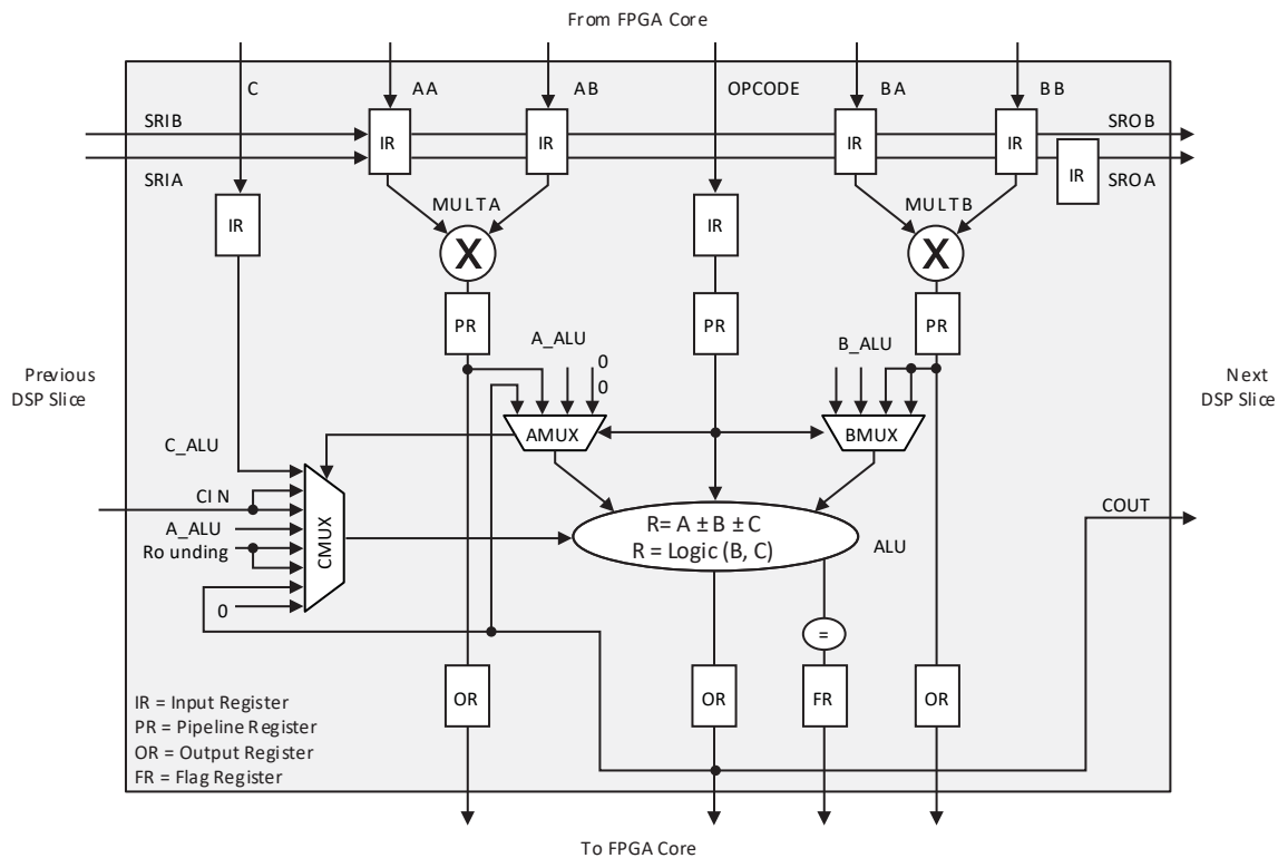
Figure 3.23. Simplified sysDSP Slice Block Diagram
