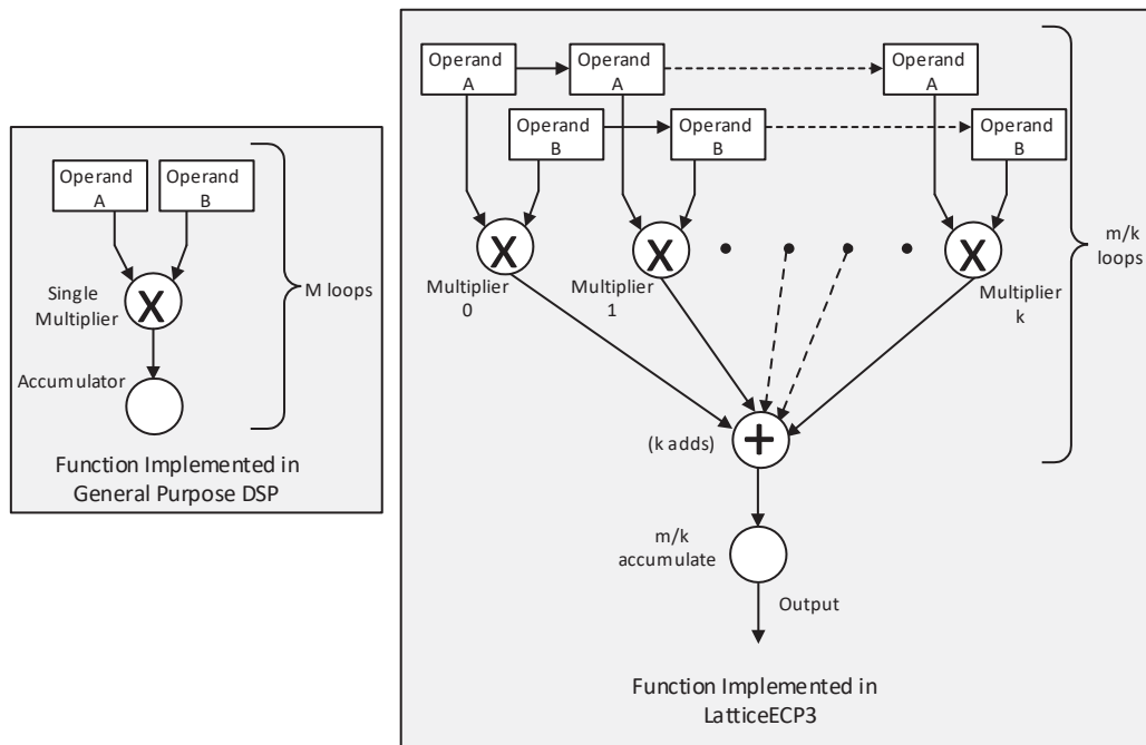
Figure 3.22. Comparison of General DSP and LA-LatticeECP3 Approaches
