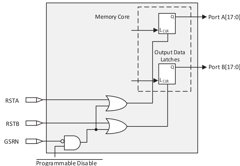
Figure 3.21. Memory Core Reset
