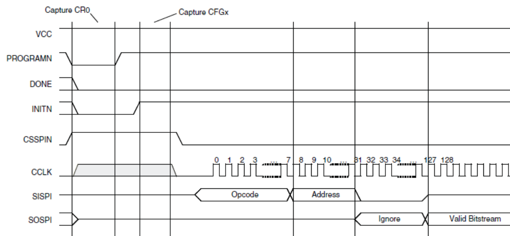
Figure 4.28. Master SPI Configuration Waveforms
