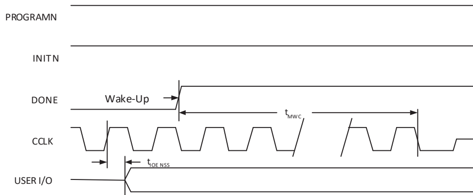
Figure 4.27. Wake-Up Timing
