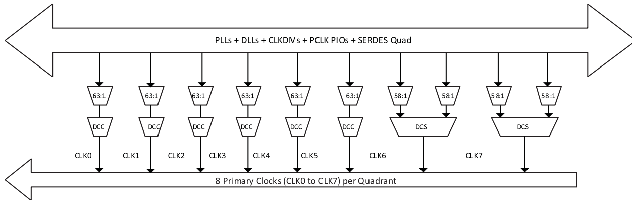
Figure 3.11. Per Quadrant Primary Clock Selection
