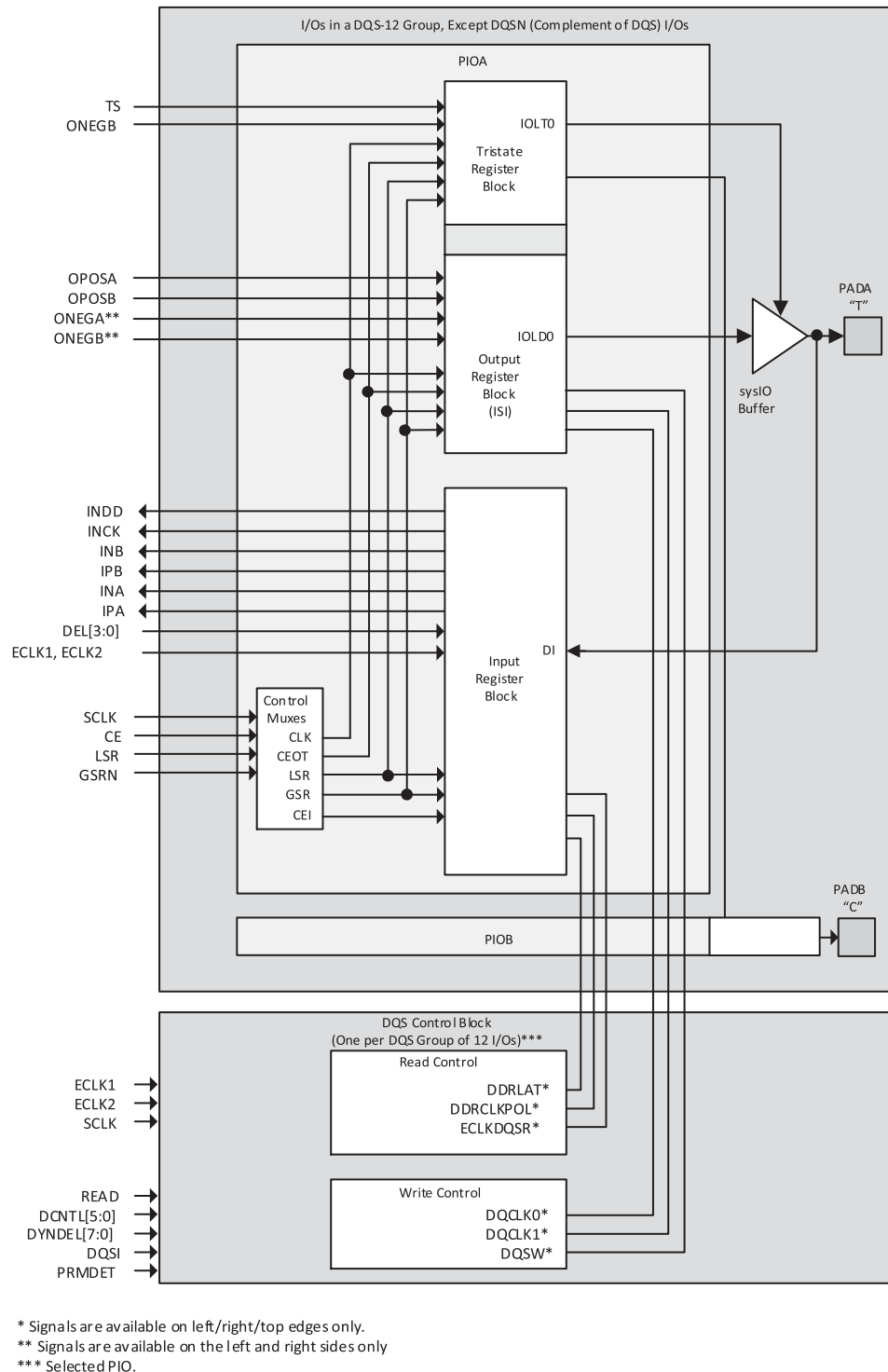
Figure 3.31. PIC Diagram
