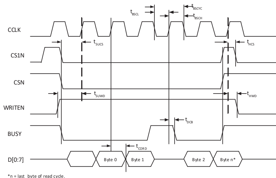
Figure 4.20. sysCONFIG Parallel Port Read Cycle
