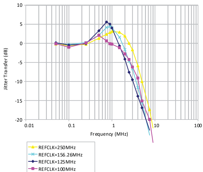
Figure 4.15. Jitter Transfer – 2.5 Gbps
