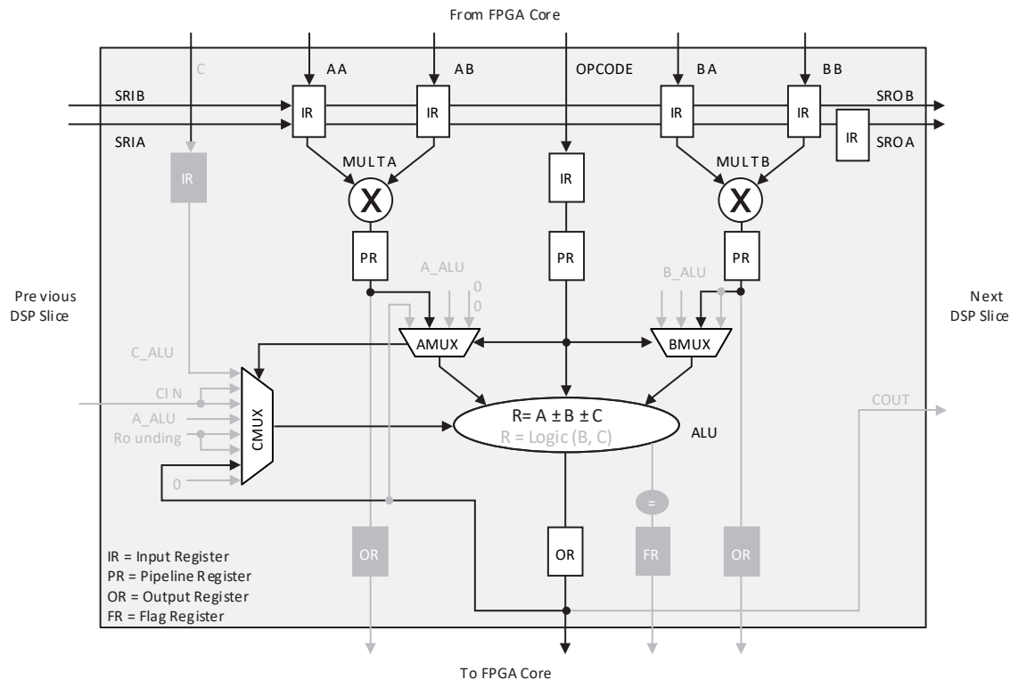
Figure 3.27. MMAC sysDSP Element
