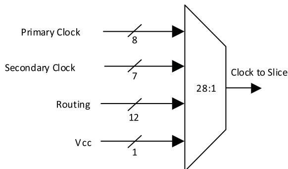
Figure 3.16. Slice 0 through Slice 2 Clock Selection
