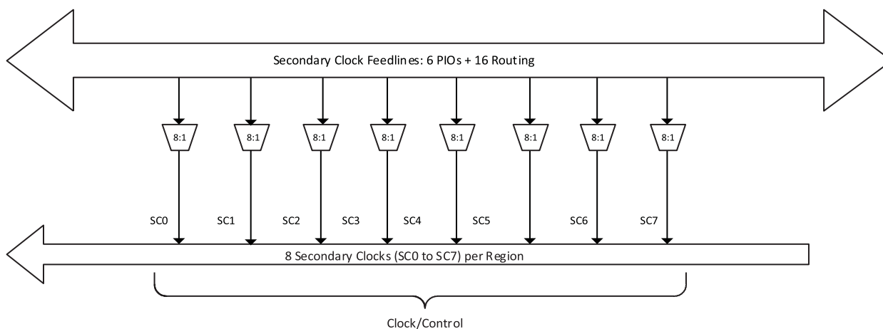
Figure 3.15. Per Region Secondary Clock Selection
