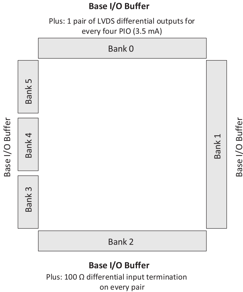
Figure 4.2. MachXO3L/LF-1300, MachXO3L/LF-2100, MachXO3L/LF-4300, MachXO3L/LF-6900, and MachXO3L/LF-9400 I/O Banking Arrangement
