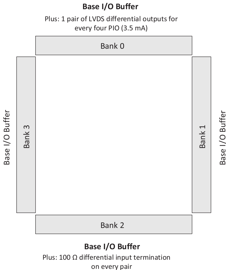
Figure 4.1. MachXO3L/LF-640 and MachXO3L/LF-1300 I/O Banking Arrangement
