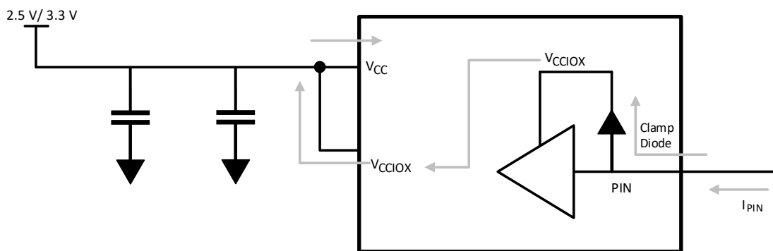
Figure D.1. Potential Current Path for Powered Down FPGA with Driven Input
