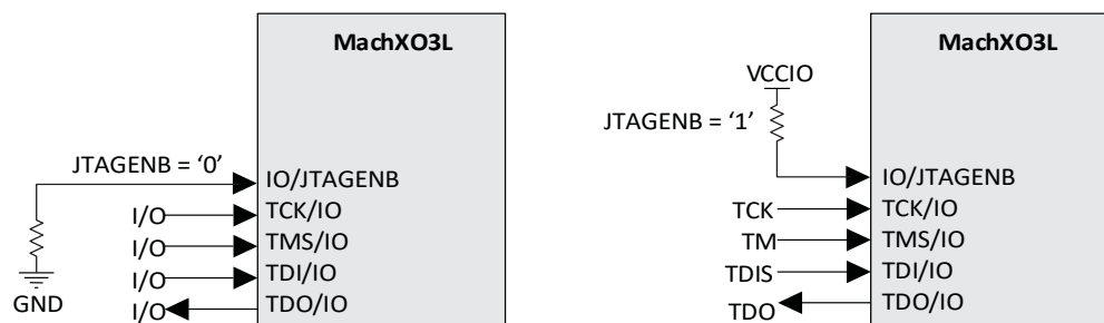
Figure 4.9. JTAG Port Behavior with JTAG_PORT = DISABLE
