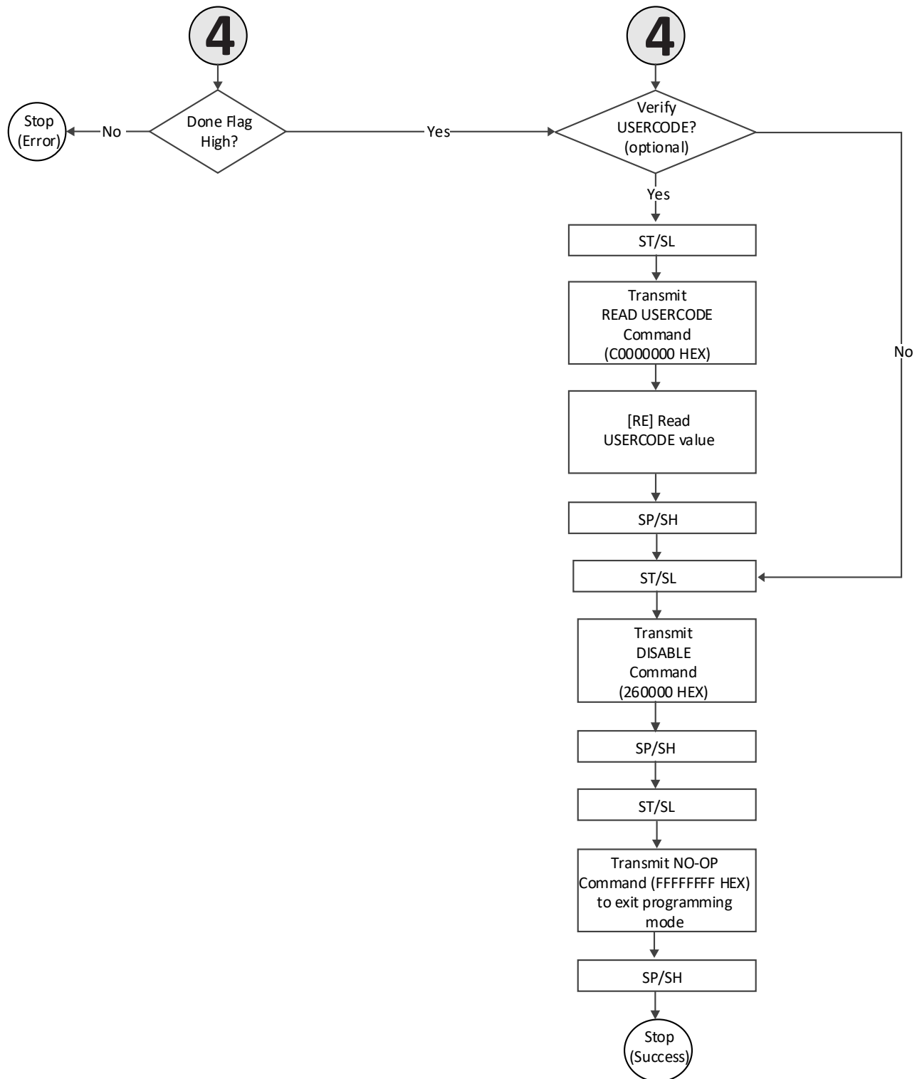
Figure 8.3. MachXO3 Slave SPI/I²C SRAM Configuration Flow
