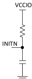
Figure 5.1. RC Delay
