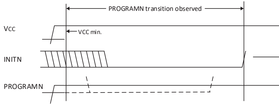
Figure 4.5. Period PROGRAMN is Always Observed
