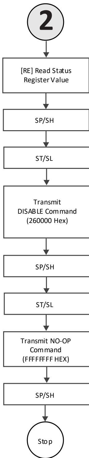
Figure 8.6. Slave SPI/I²C SRAM Read Status Register Flow
