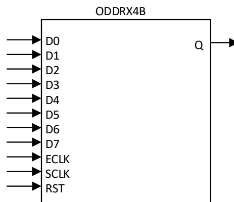
Figure 8.7. ODDRX4B Symbol
