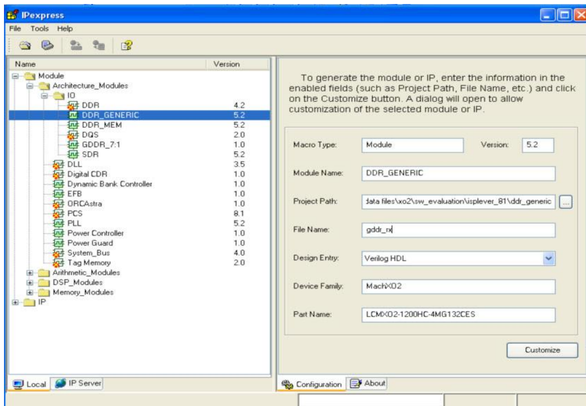
Figure 6.3. DDR_Generic Interface Selection at the IPexpress Main Window
