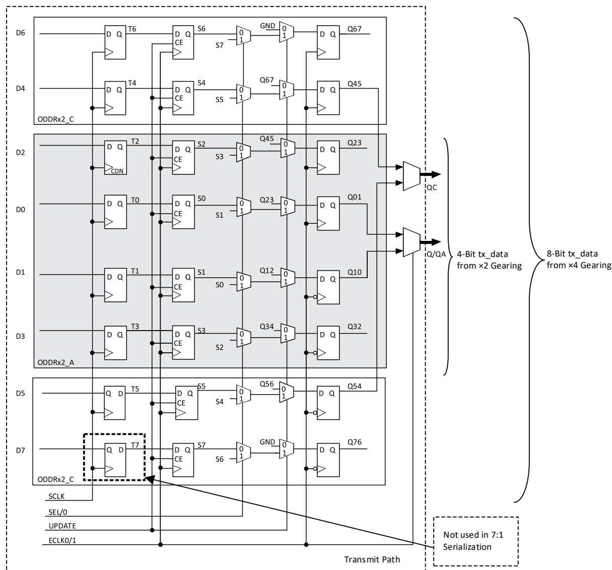
Figure 2.2. Video PIO Cell for \times 2/\times 4 and 7:1 Applications in MachXO3L/LF
