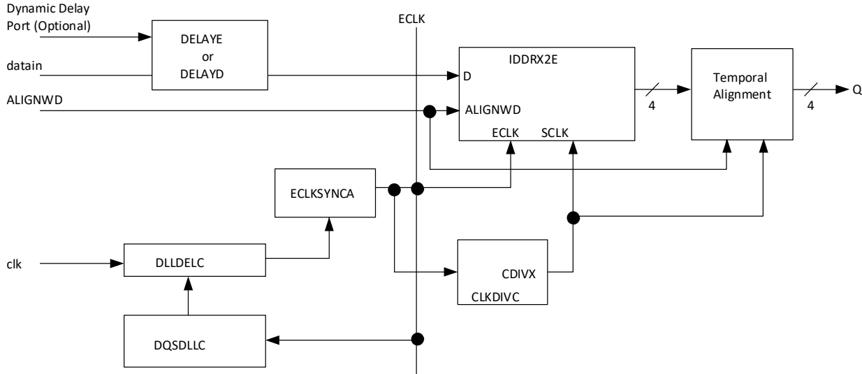
Figure 5.4. GDDR2_RX.ECLK.Aligned Interface
