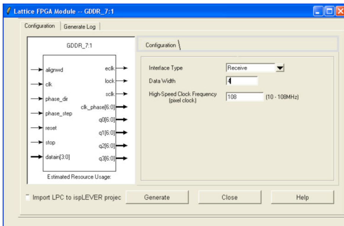
Figure 6.7. Configuration Tab of GDDR_71
