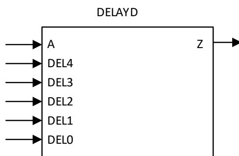
Figure 8.11. DELAYD Symbol
