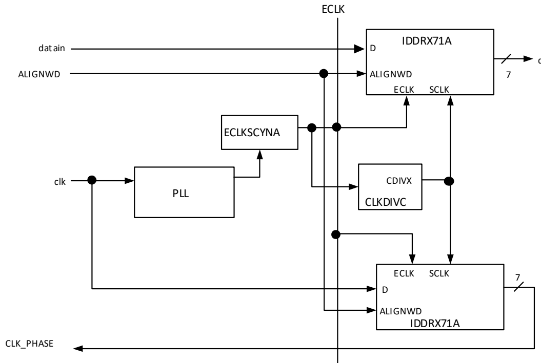
Figure 5.8. GDDR71_RX.ECLK.7:1 Interface
