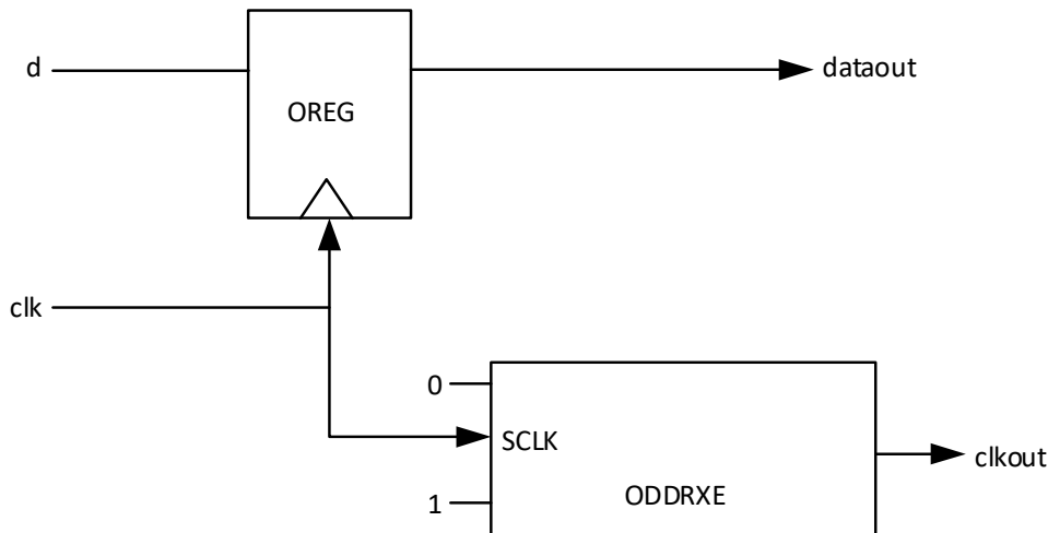
Figure 5.9. GOREG_TX.SCLK Interface
