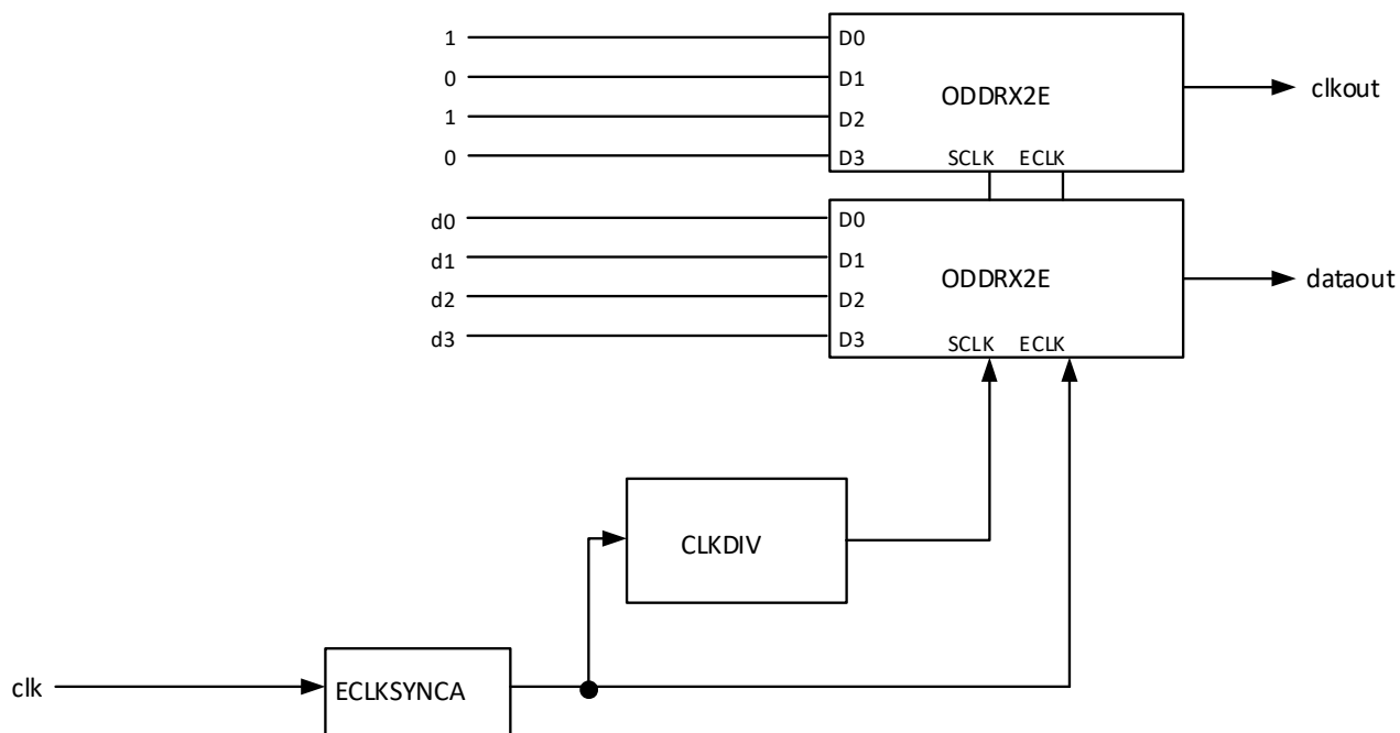
Figure 5.12. GDDR2_TX.ECLK.Aligned Interface
