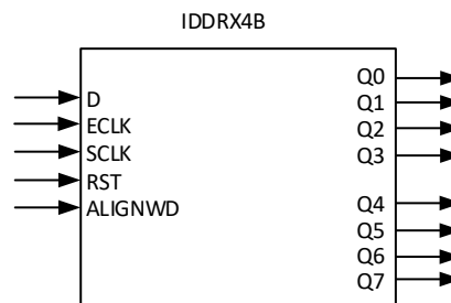
Figure 8.3. IDDRX4B Symbol
