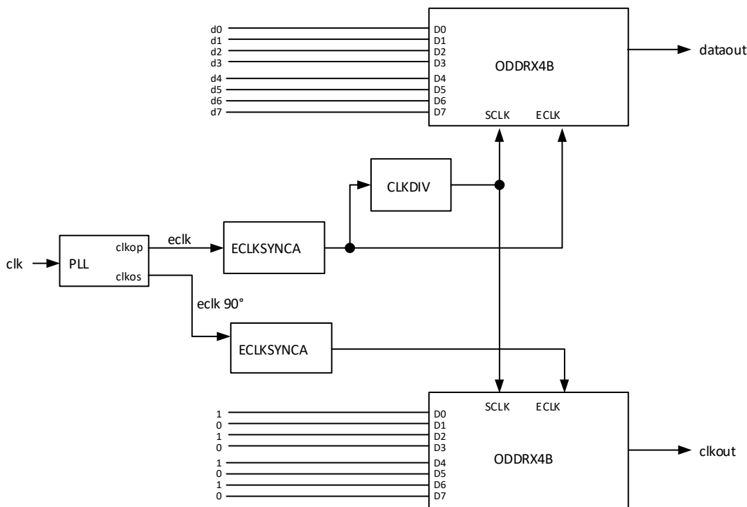
Figure 5.15. GDDR4_TX.ECLK.Centered Interface
