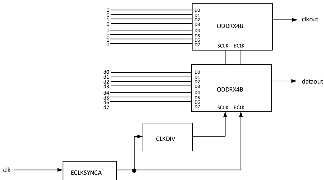
Figure 5.14. GDDR4_TX.ECLK.Aligned Interface
