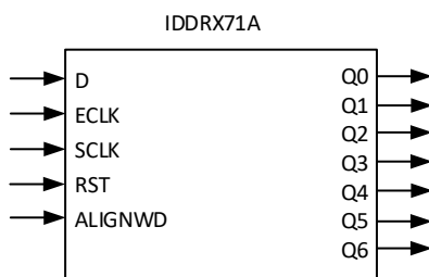
Figure 8.4. IDDRX71A Symbol
