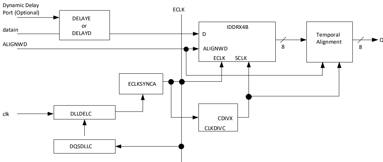
Figure 5.6. GDDR4_RX.ECLK.Aligned Interface
