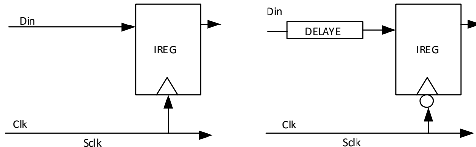
Figure 5.1. GIREG_RX Interface
