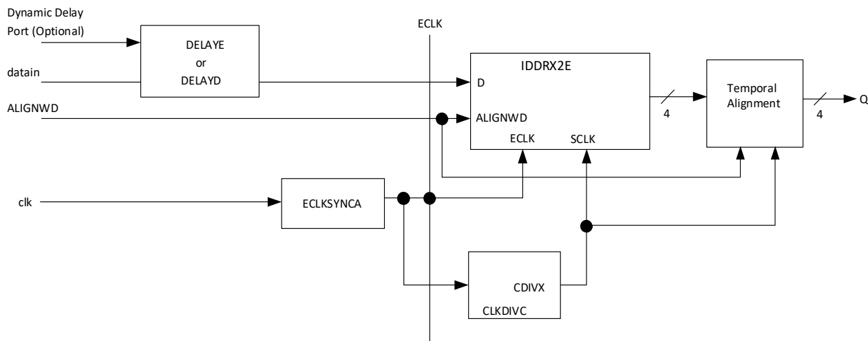
Figure 5.5. GDDR2_RX.ECLK.Centered Interface
