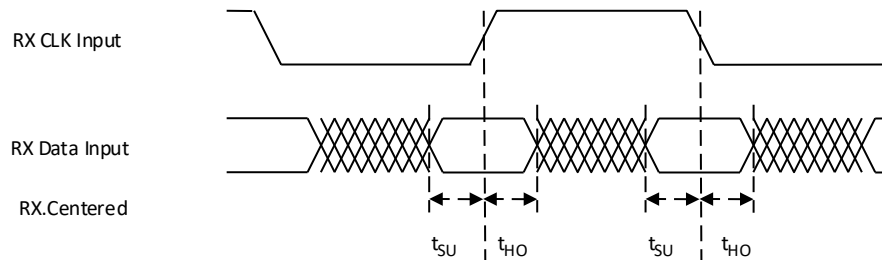
Figure 7.3. Receiver RX.CLK.Centered Waveforms
