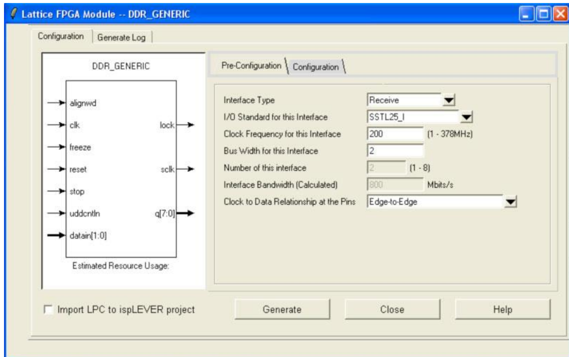
Figure 6.4. Pre-Configuration Tab of the DDR_Generic Interfaces
