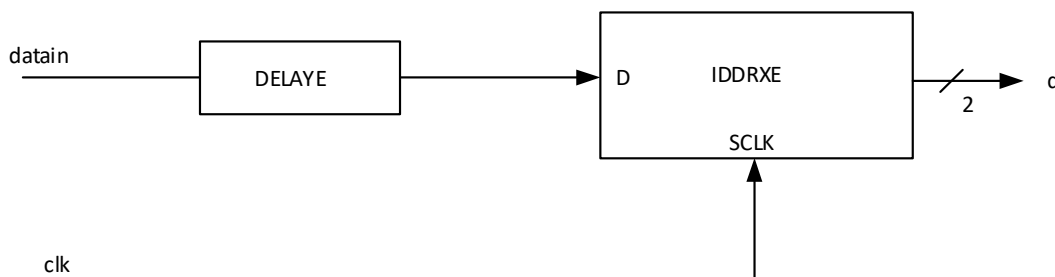
Figure 5.3. GDDR1_RX.SCLK.Centered
