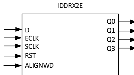
Figure 8.2. IDDRX2E Symbol
