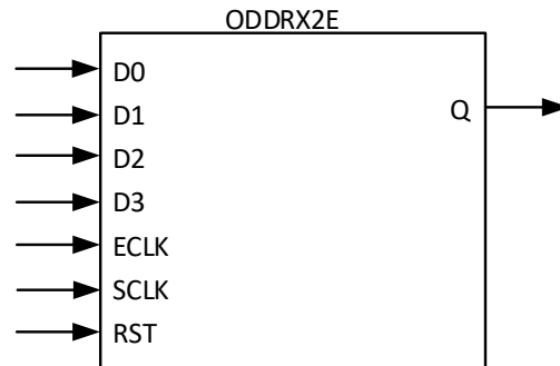
Figure 8.6. ODDRX2E Symbol
