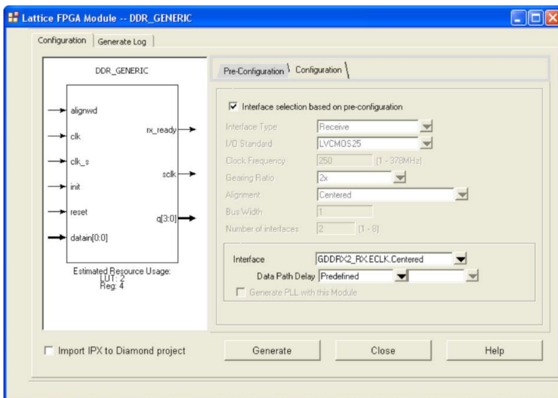
Figure 6.5. Configuration Tab of the DDR_Generic Modules
