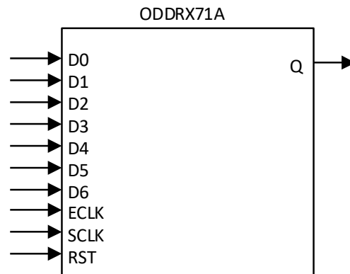
Figure 8.8. ODDRX71A Symbol
