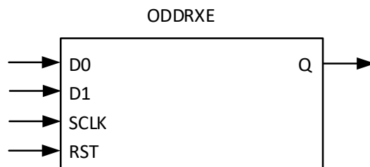
Figure 8.5. ODDRXE Symbol
