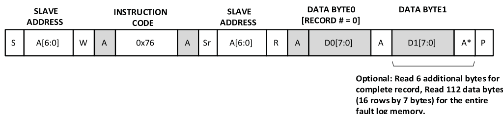
Figure 7.39. READ_ALL_FAULT_EEPROM - I 2 C Instruction Format
