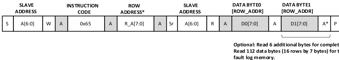
Figure 7.32. READ_USER_TAG_EEPROM - I 2 C Instruction Format
