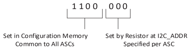
Figure 7.2. I 2 C Slave Address Construction
