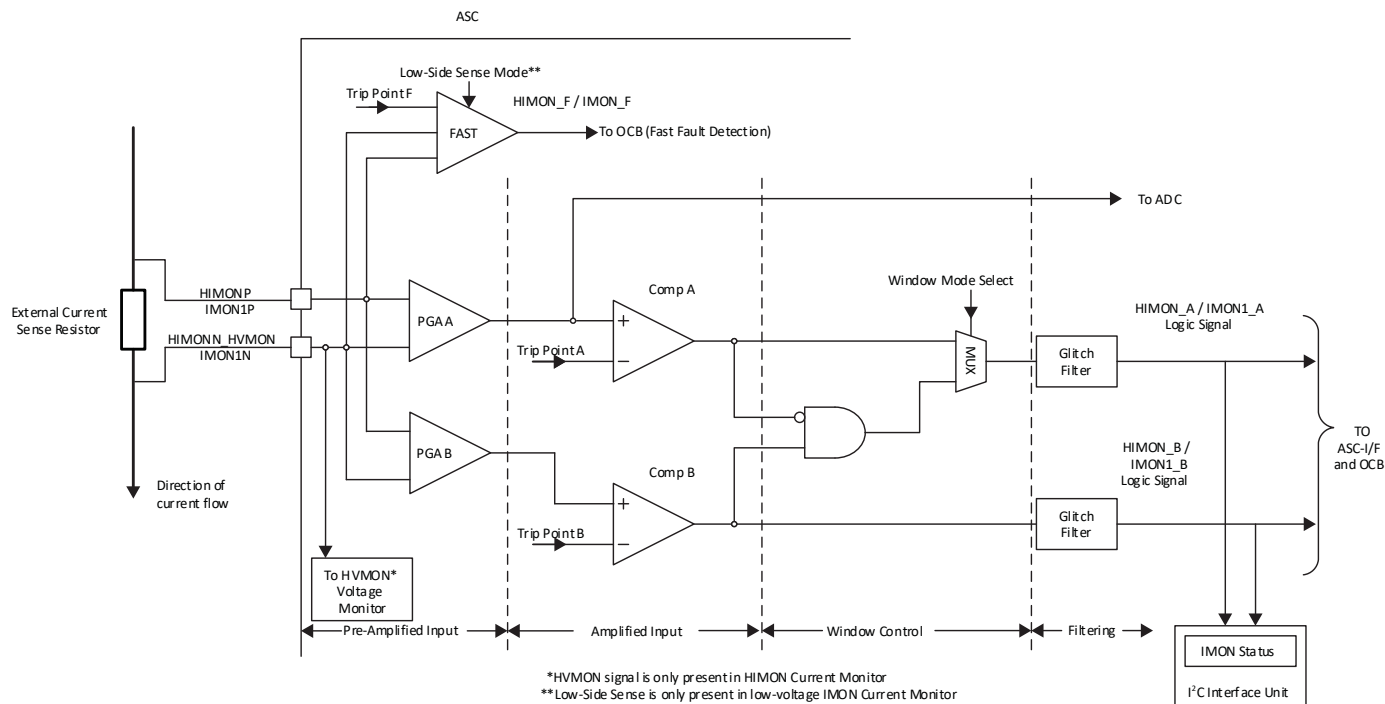
Figure 6.4. ASC Current Monitor
