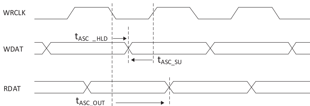
Figure 5.2. ASC Interface (ASC-I/F) Timing Diagram
