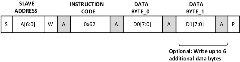
Figure 7.29. WRITE_USER_TAG_REG - I²C Instruction Format
