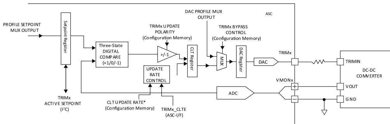
Figure 6.23. Digital Closed Loop Trim Operation
