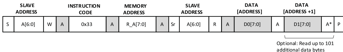
Figure 7.15. READ_CFG_REG - I 2 C Instruction Format
