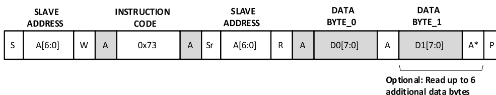
Figure 7.35. READ_FAULT_VOLATILE_REG - I 2 C Instruction Format
