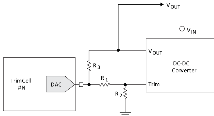
Figure 6.21. TrimCell Driving a Typical DC-DC Converter
