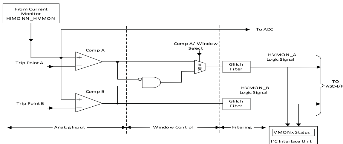
Figure 6.5. HVMON Monitor Circuit
