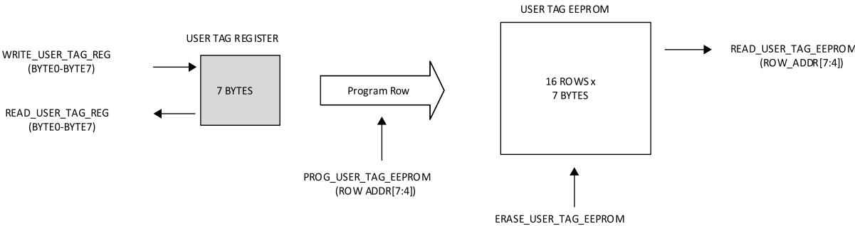
Figure 7.27. User Tag Memory Architecture with I²C Instruction Access
