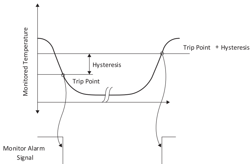
Figure 6.9. Monitor Alarm Signal Behavior - Overtemperature (OT) Setting
