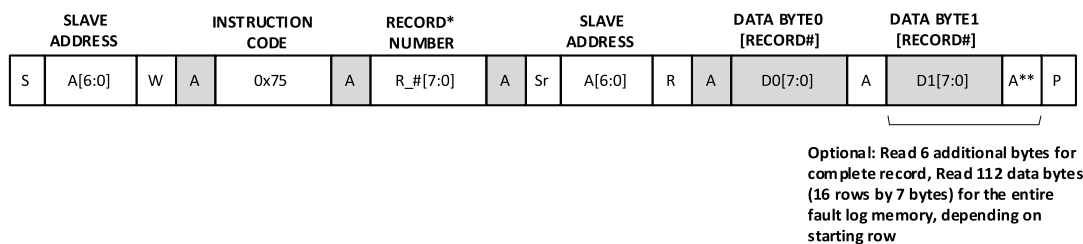
Figure 7.38. READ_FAULT_RECORD_EEPROM - I 2 C Instruction Format
