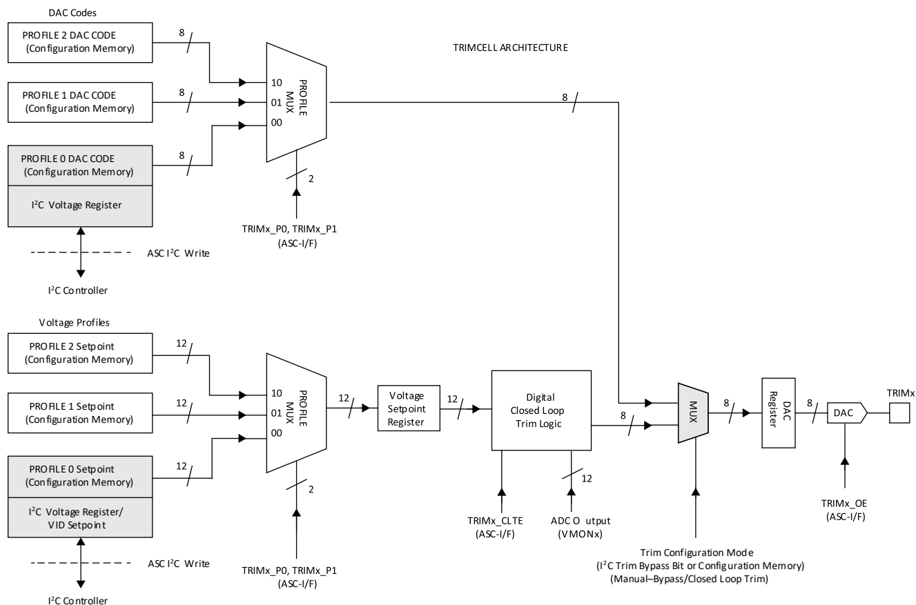
Figure 6.22. TrimCell Architecture
