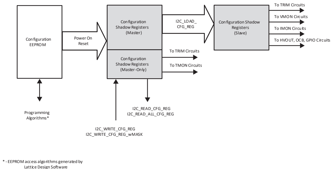
Figure 7.11. Configuration Memory Architecture
