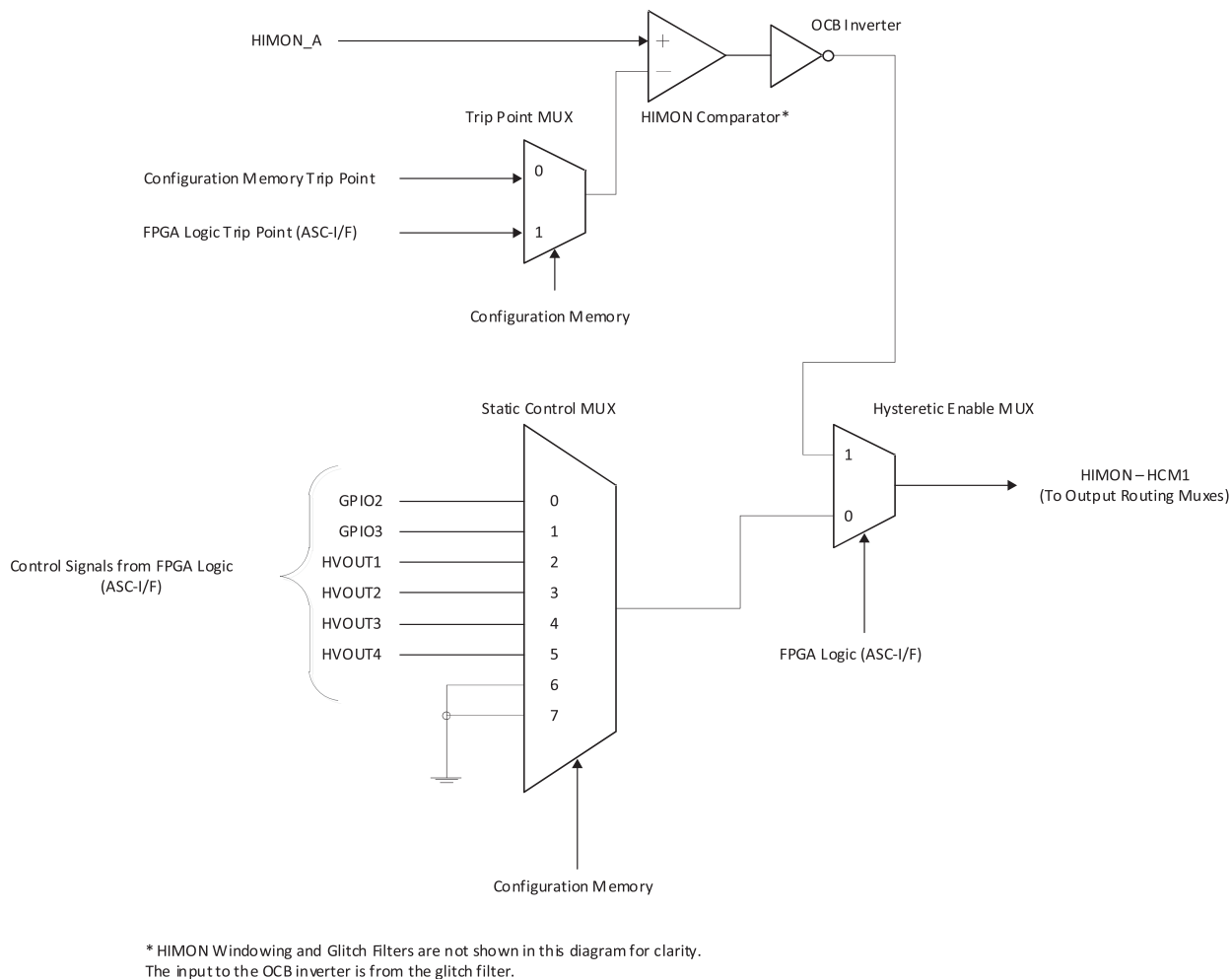
Figure 6.15. OCB HIMON HCM1 Block Diagram
