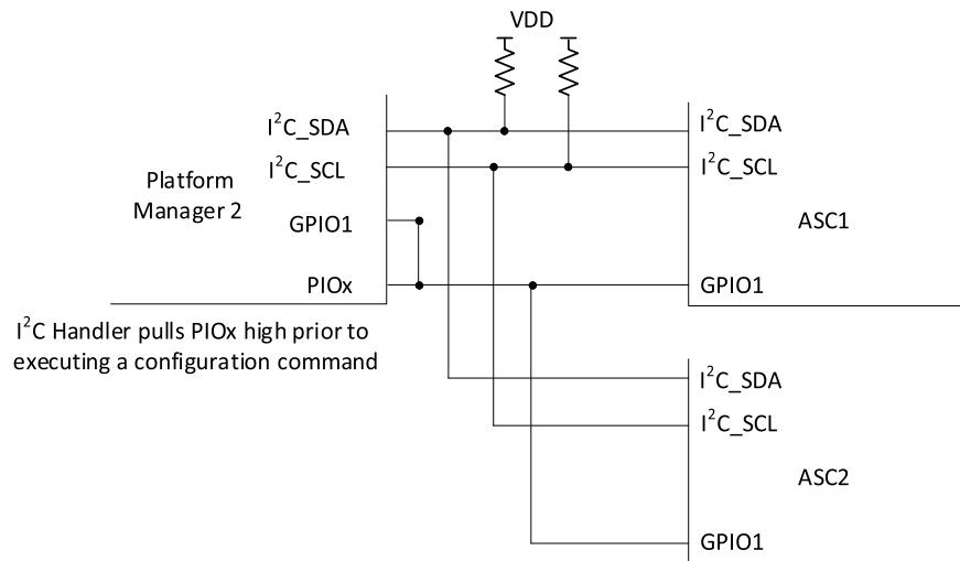
Figure 7.40. I 2 C Write Protect by GPIO1
