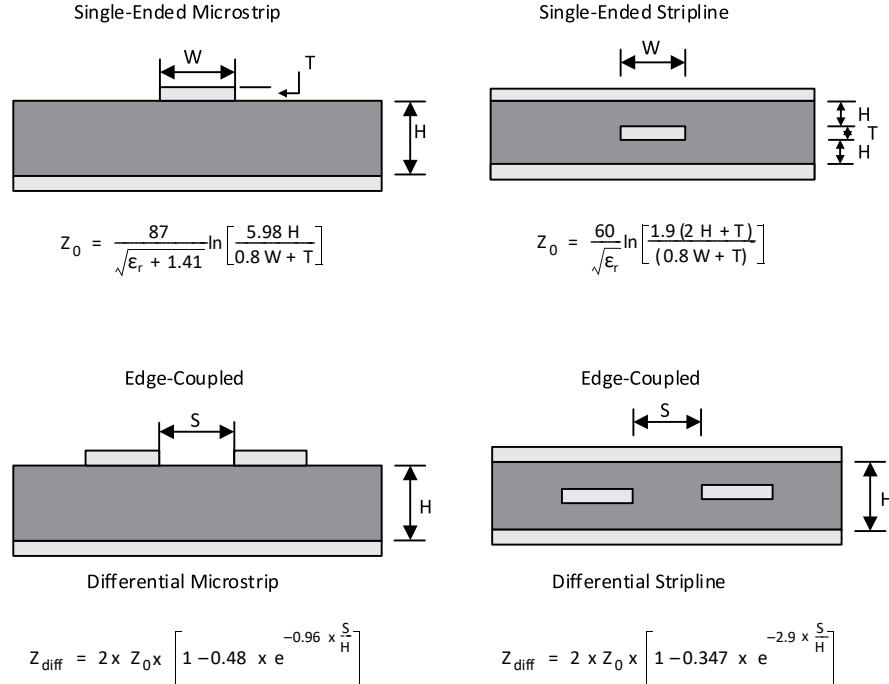
Figure 7.1. Controlled Impedance Transmission Lines
