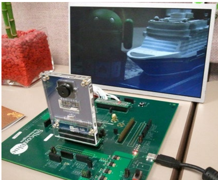
Figure 11.3. 5-Megapixel CMOS Camera to LVDS Display on iCEman40 Evaluation Board
