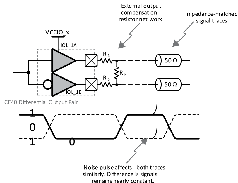
Figure 2.1. Differential Output Pair
