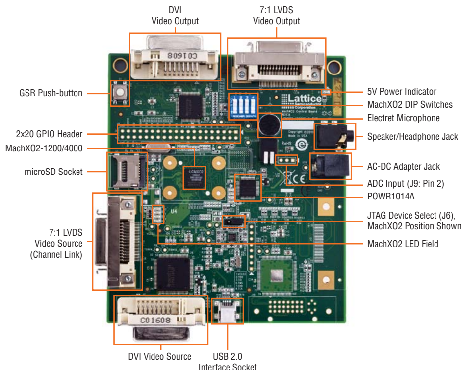
Figure 1. MachXO2-1200HC Control Evaluation Board, Top Side
