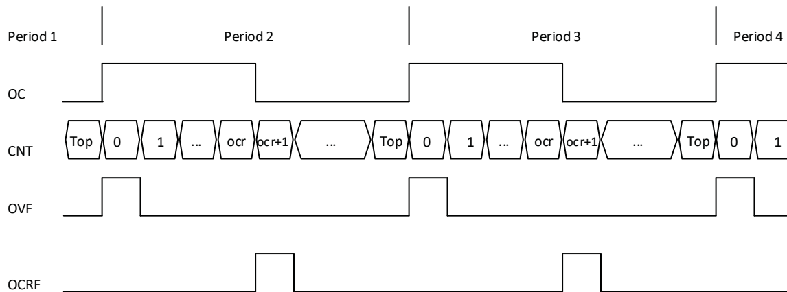
Figure 6.3. PWM Waveform Generation
