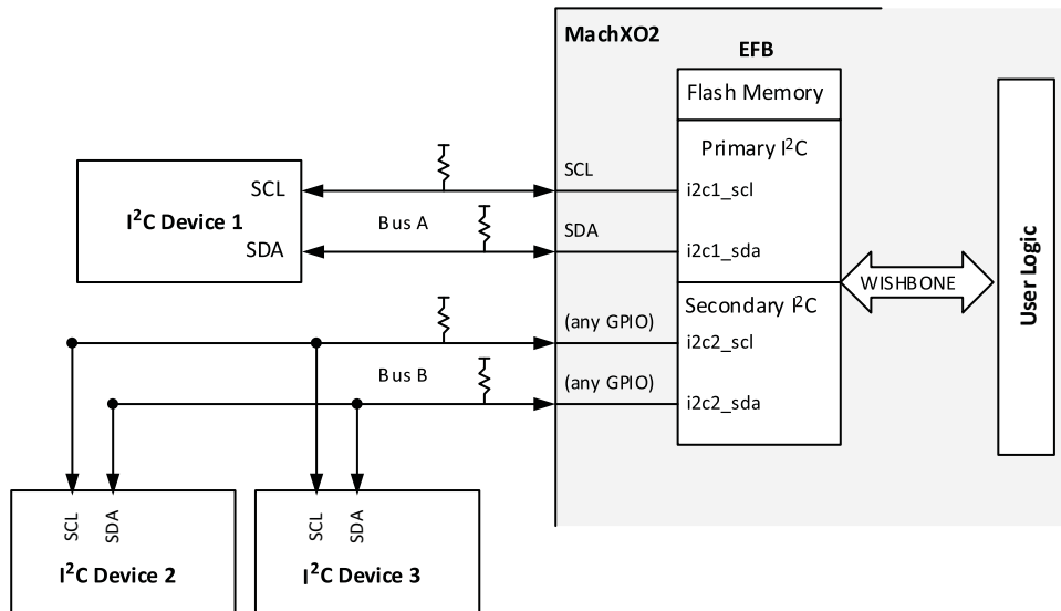
Figure 4.5. I 2 C Circuit
