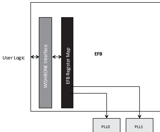
Figure 11.1. EFB Interface to Dynamic PLL
