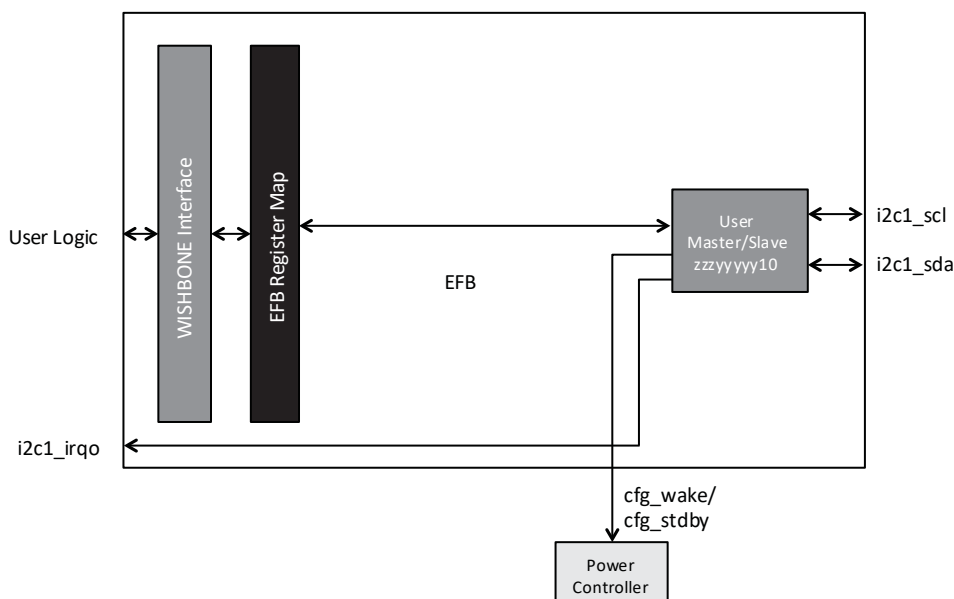
Figure 4.3. I 2 C Secondary Block Diagram
