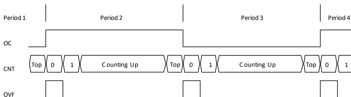
Figure 6.2. Timer/Counter Output Waveform
