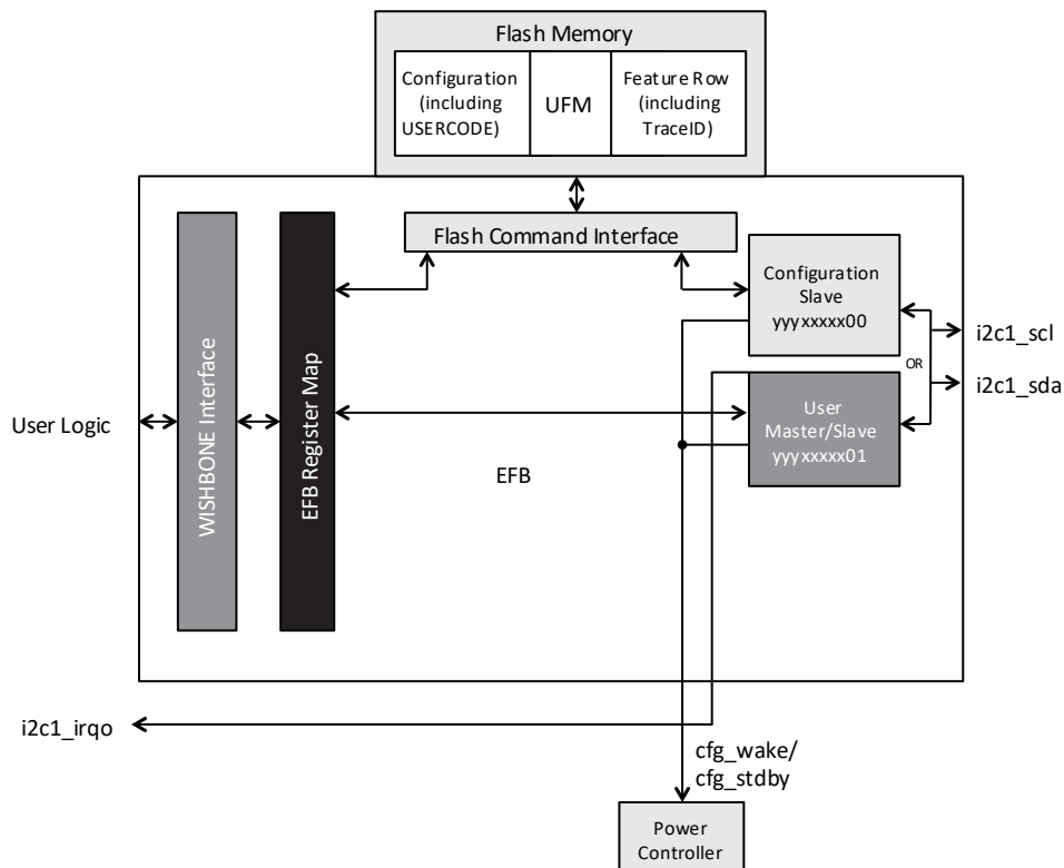
Figure 4.2. I 2 C Primary Block Diagram
