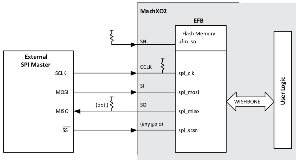
Figure 5.3. External Master SPI Device Accessing the Slave MachXO2 User SPI
