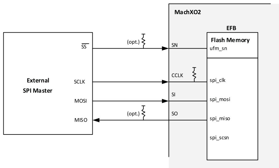
Figure 5.5. External Master SPI Device Accessing the MachXO2 Configuration Logic
