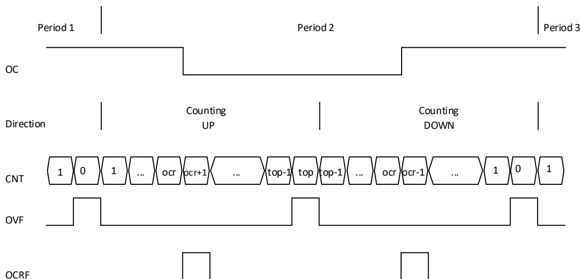
Figure 6.4. Phase and Frequency Correct PWM Waveform Generation
