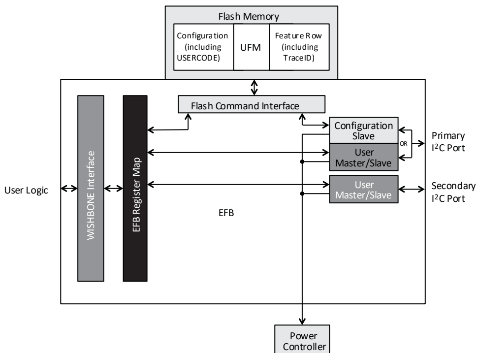
Figure 4.1. I 2 C Block Diagram
