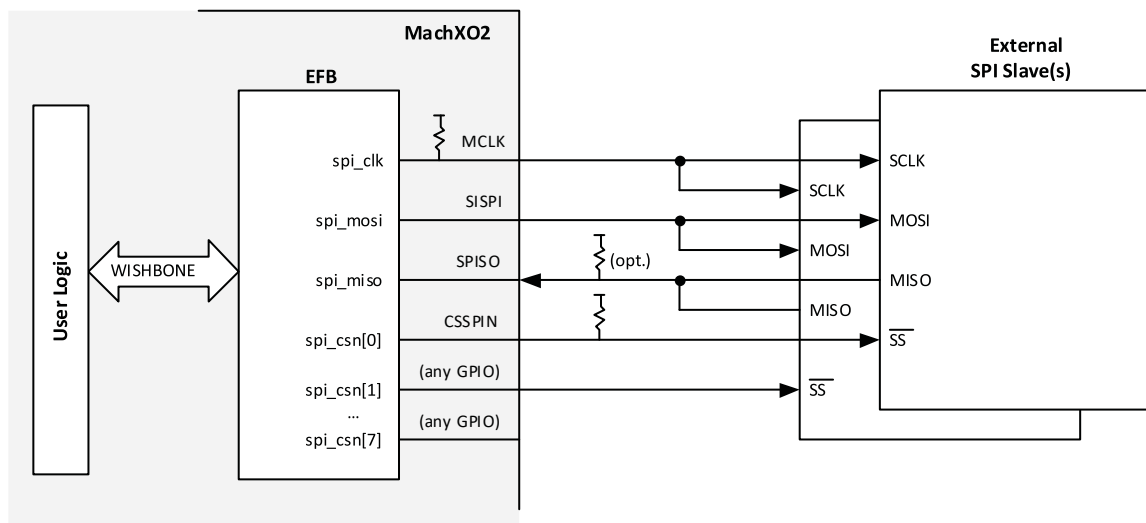
Figure 5.4. MachXO2 User SPI Master Accessing One or Multiple External Slave SPI Devices
