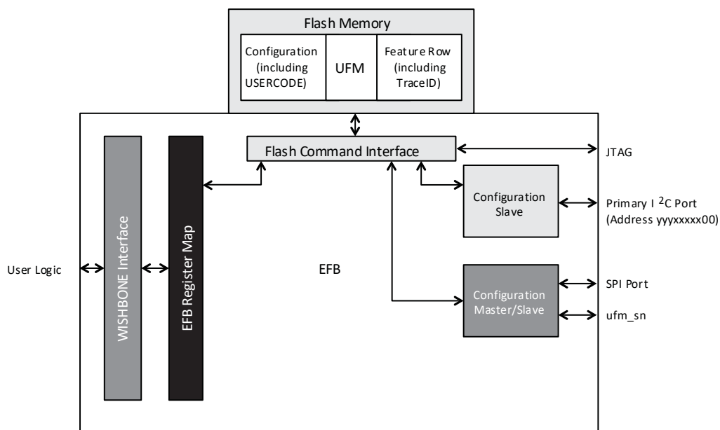
Figure 7.1. Flash Memory (UFM/Configuration) Block Diagram
