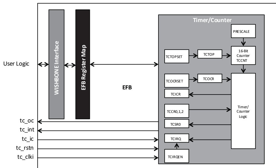
Figure 6.1. Timer/Counter Block Diagram
