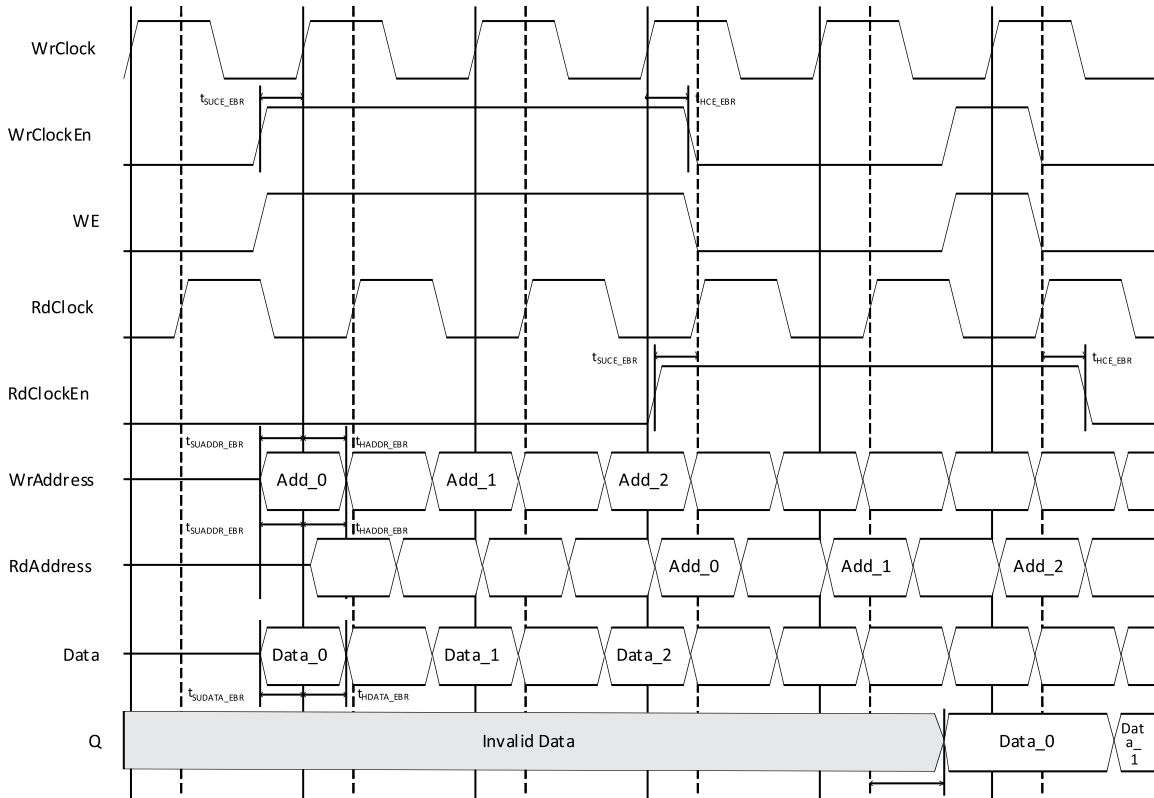
Figure 6.8. PFU-Based Distributed Dual Port RAM Timing Waveform – With Output Registers
