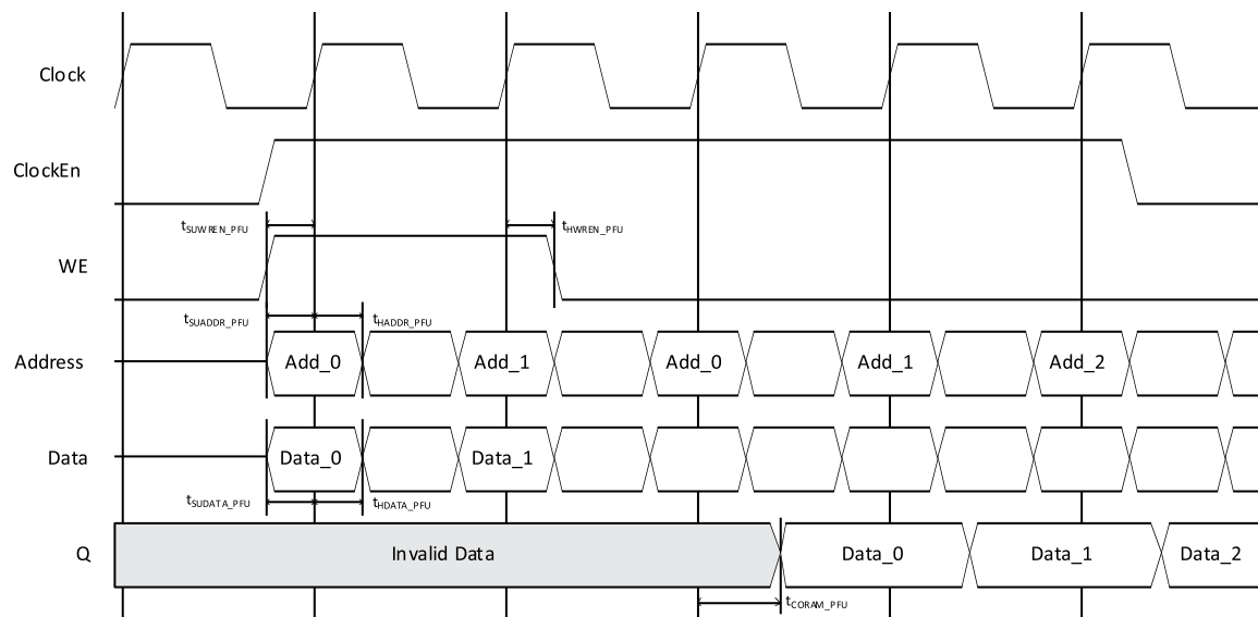
Figure 6.4. PFU-Based Distributed Single Port RAM Timing Waveform – Without Output Registers
