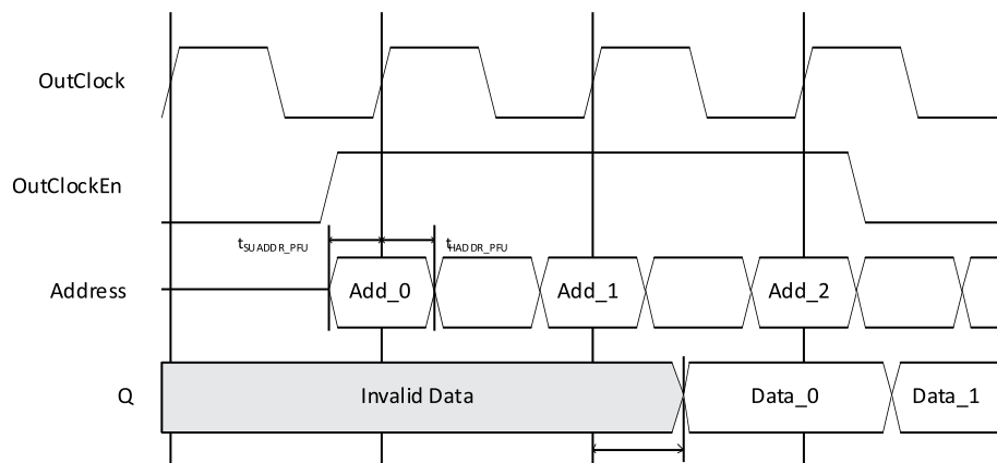
Figure 6.11. PFU-Based ROM Timing Waveform – With Output Registers
