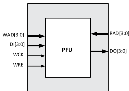
Figure 7.6. Distributed DPRAM Primitive (DPR16X4C)
