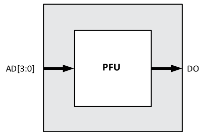
Figure 7.7. Distributed_ROM Primitive (ROM16X1A)
