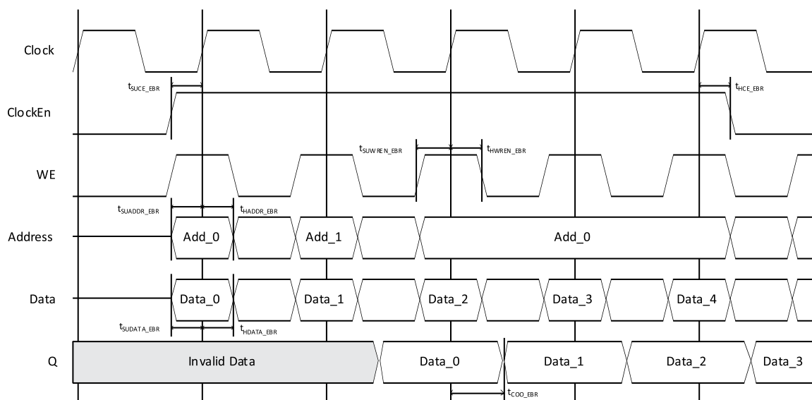
Figure 3.7. Single Port RAM Timing Waveform – WRITE THROUGH Mode, With Output Registers
