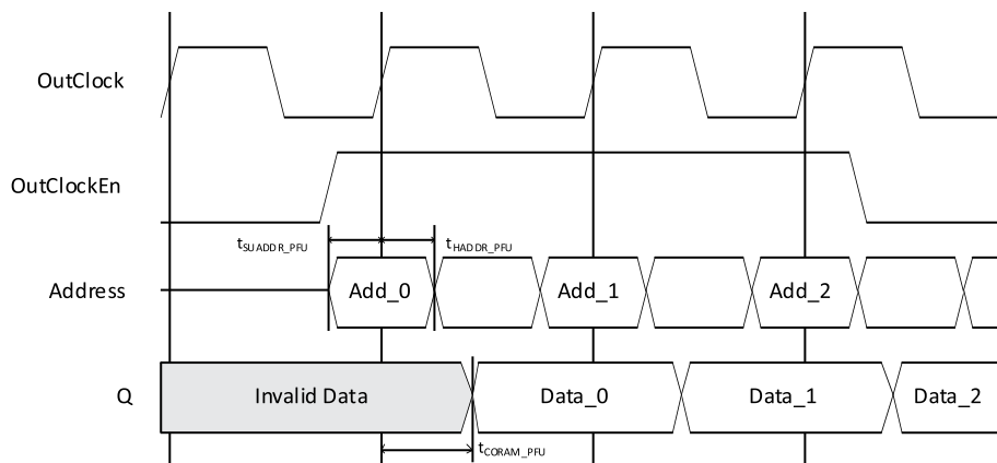
Figure 6.10. PFU-Based ROM Timing Waveform – Without Output Registers
