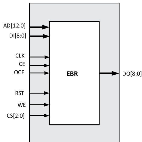
Figure 7.1. Single Port RAM (SP8KC)
