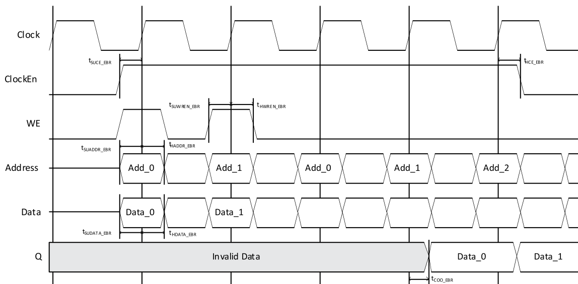
Figure 3.3. Single Port RAM Timing Waveform – NORMAL Mode, With Output Registers
