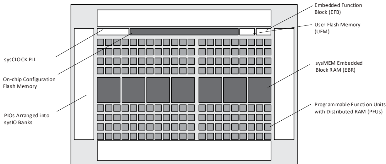
Figure 1.1. Top View of the MachXO2-1200 Device
