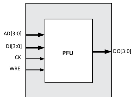
Figure 7.5. Distributed_SPRAM Primitive (SPR16X4C)
