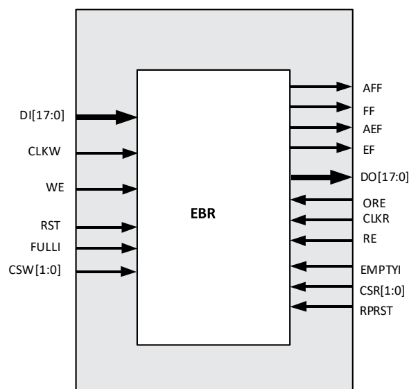
Figure 7.4. FIFO_DC Primitive (FIFO8KB)
