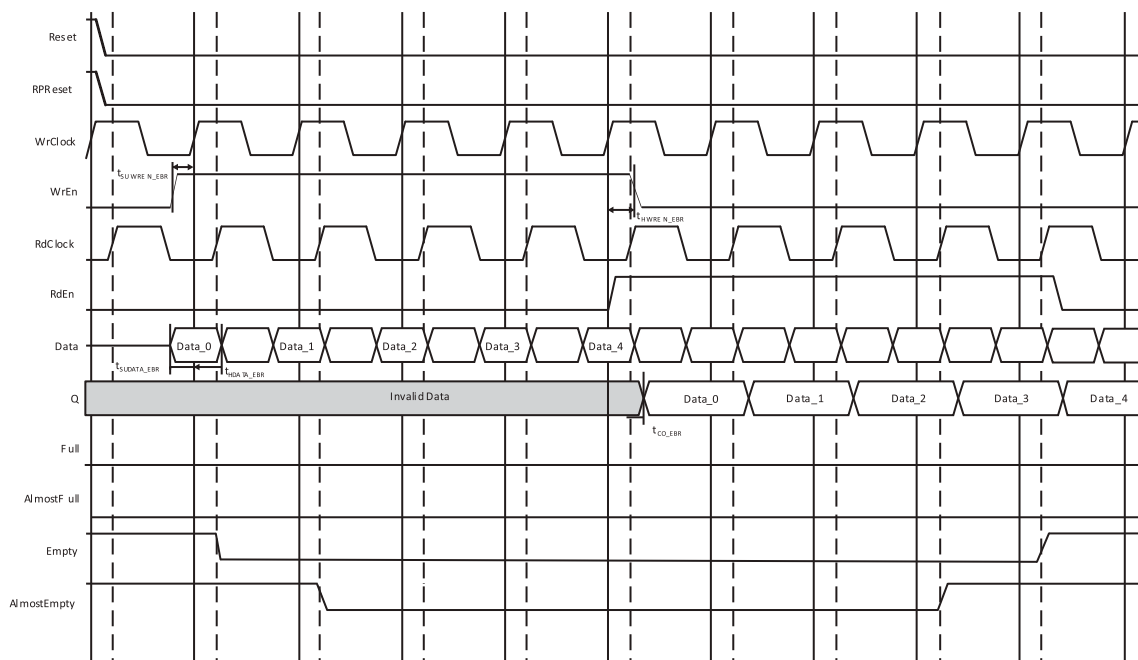
Figure 6.1. FIFO_DC Without Output Registers (Non-Pipelined)
