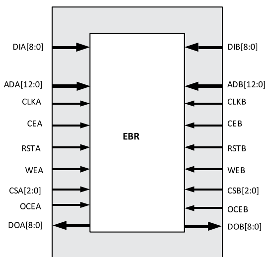
Figure 7.2. True Dual-Port RAM (DP8KC)
