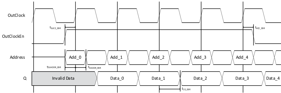
Figure 3.19. ROM Timing Waveform – Without Output Registers
