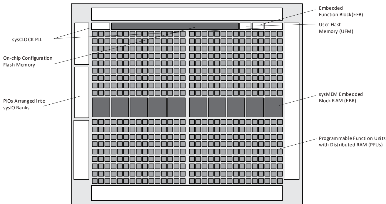
Figure 1.2. Top View of the MachXO2-4000 Device
