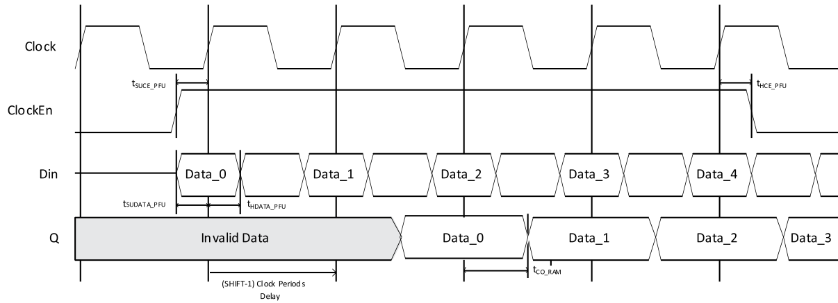
Figure 6.13. RAM-Based Shift Register Timing Waveform – Without Output Registers (Shift = 2)
