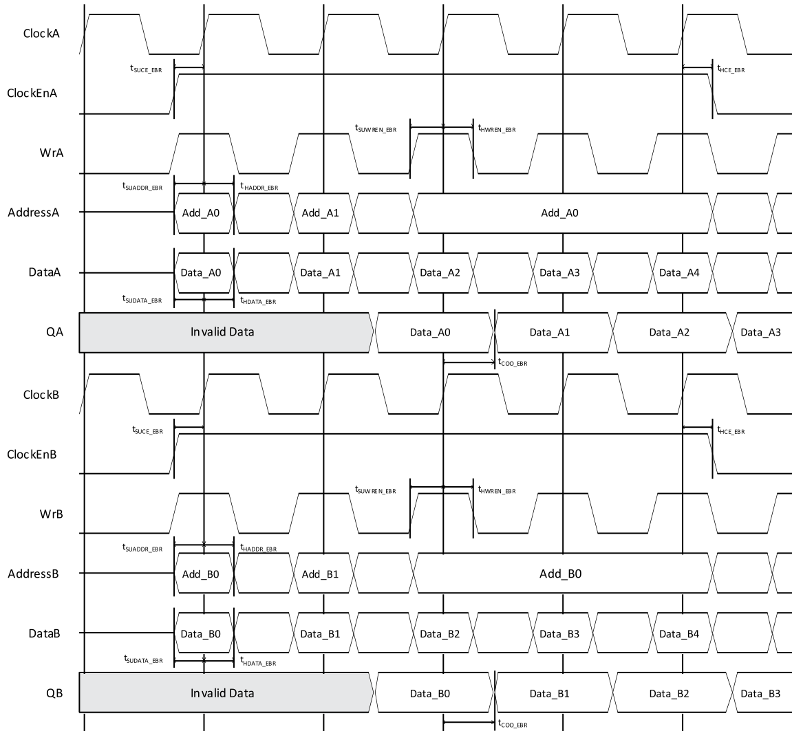
Figure 3.14. True Dual Port RAM Timing Waveform – WRITE THROUGH Mode, with Output Registers
