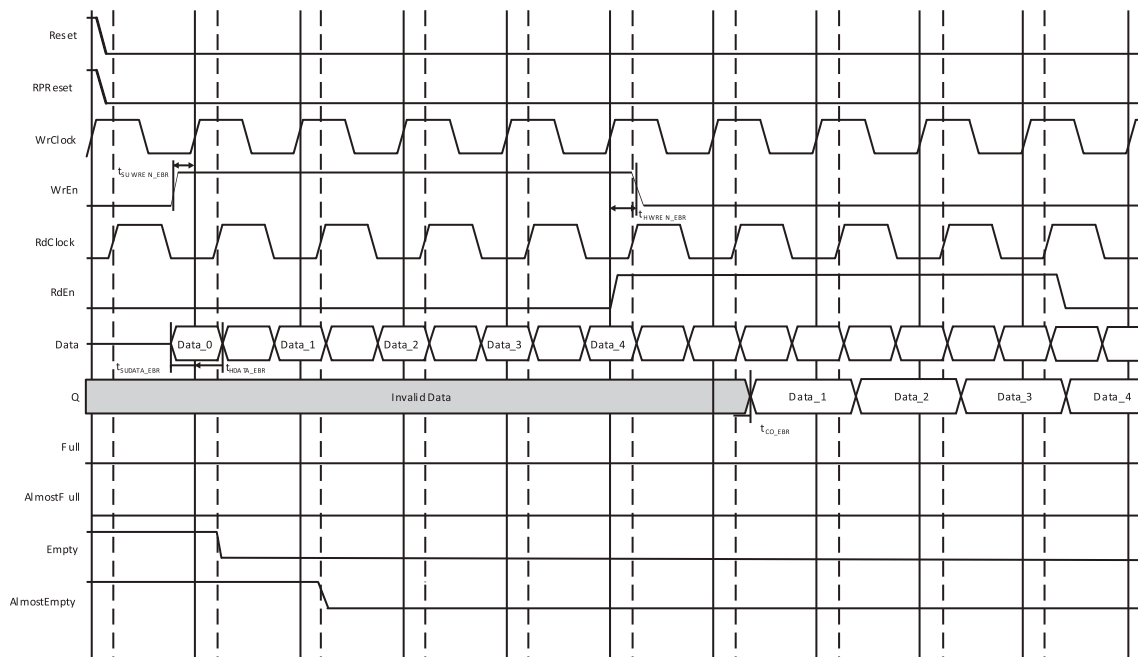
Figure 6.2. FIFO_DC With Output Registers (Pipelined)
