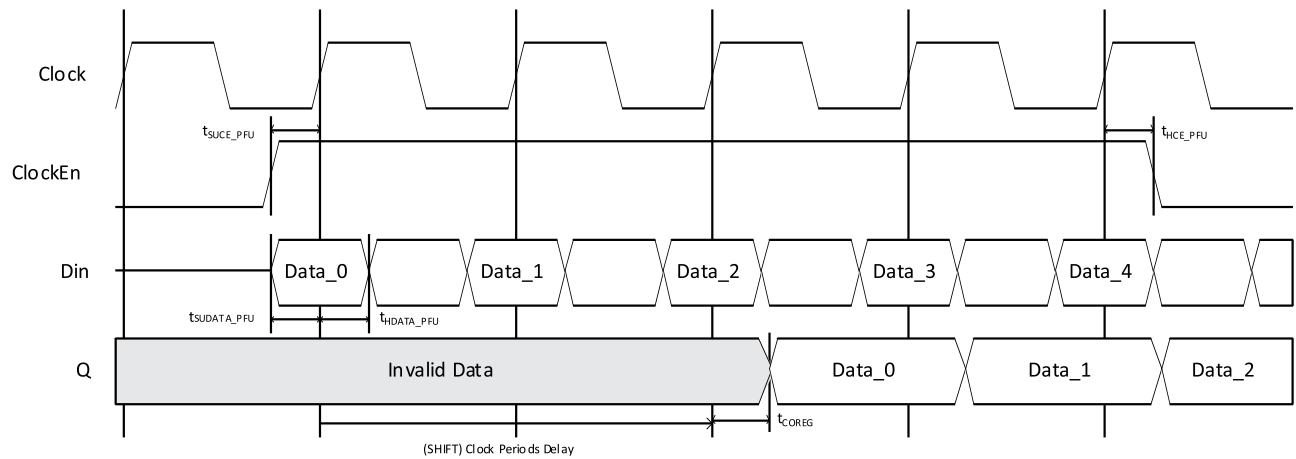
Figure 6.14. RAM-Based Shift Register Timing Waveform – With Output Registers (Shift = 2)
