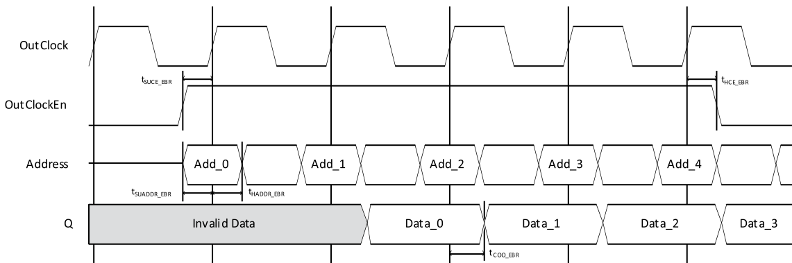
Figure 3.20. ROM Timing Waveform – With Output Registers
