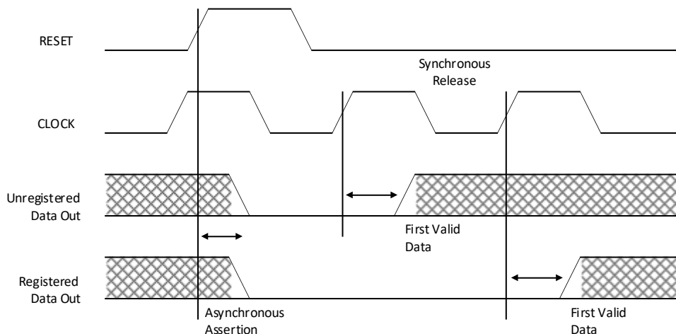
Figure 2.4. Asynchronous Reset with Synchronous Release
