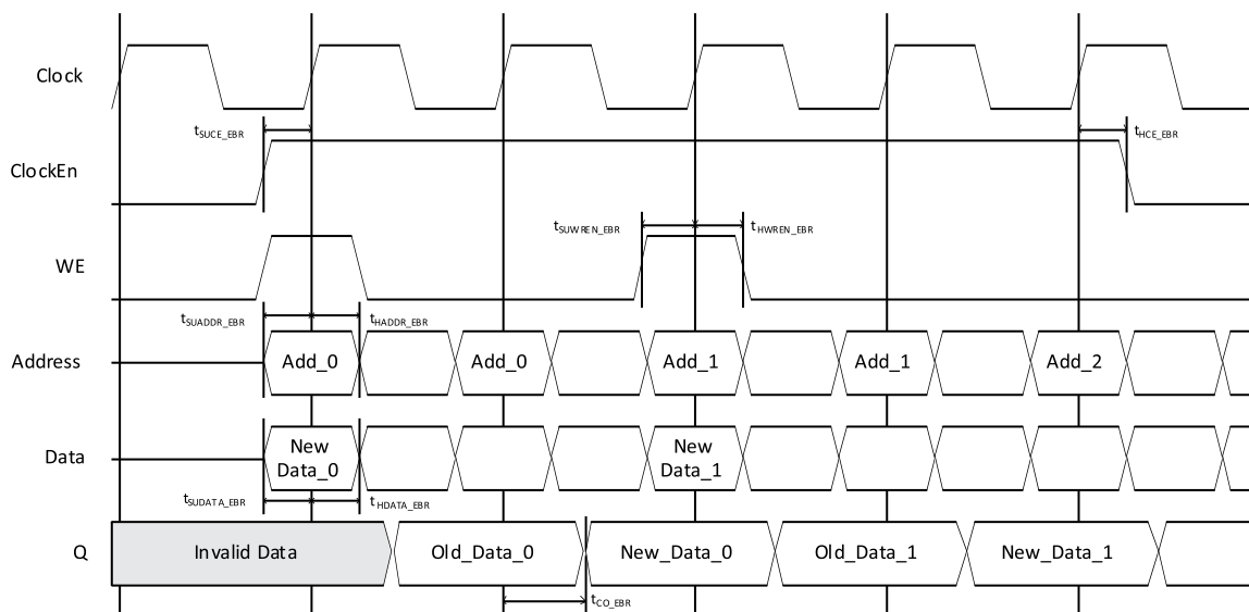
Figure 3.4. Single Port RAM Timing Waveform – READ BEFORE WRITE Mode, Without Output Registers
