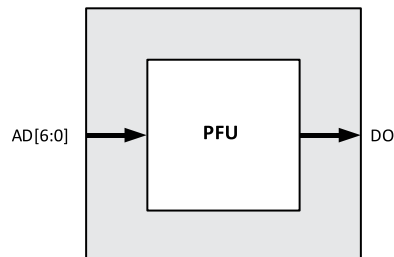
Figure 7.10. Distributed_ROM Primitive (ROM128X1A)
