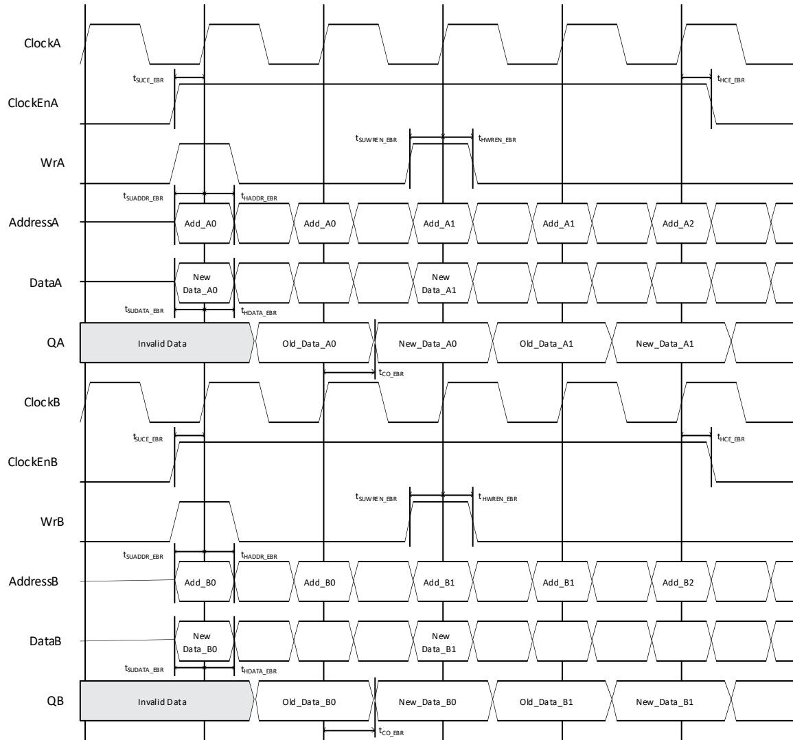
Figure 3.11. True Dual Port RAM Timing Waveform – READ BEFORE WRITE Mode, without Output Registers
