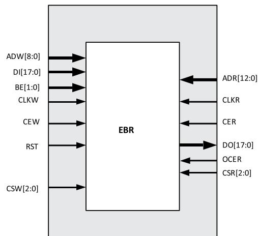
Figure 7.3. Pseudo Dual-Port RAM (PDPW8KC)
