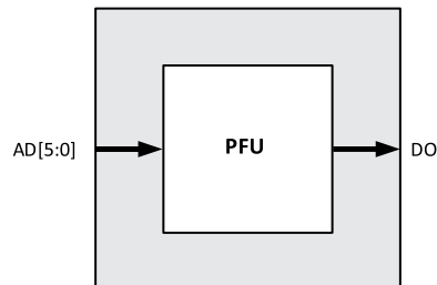
Figure 7.9. Distributed_ROM Primitive (ROM64X1A)
