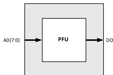
Figure 7.11. Distributed_ROM Primitive (ROM256X1A)
