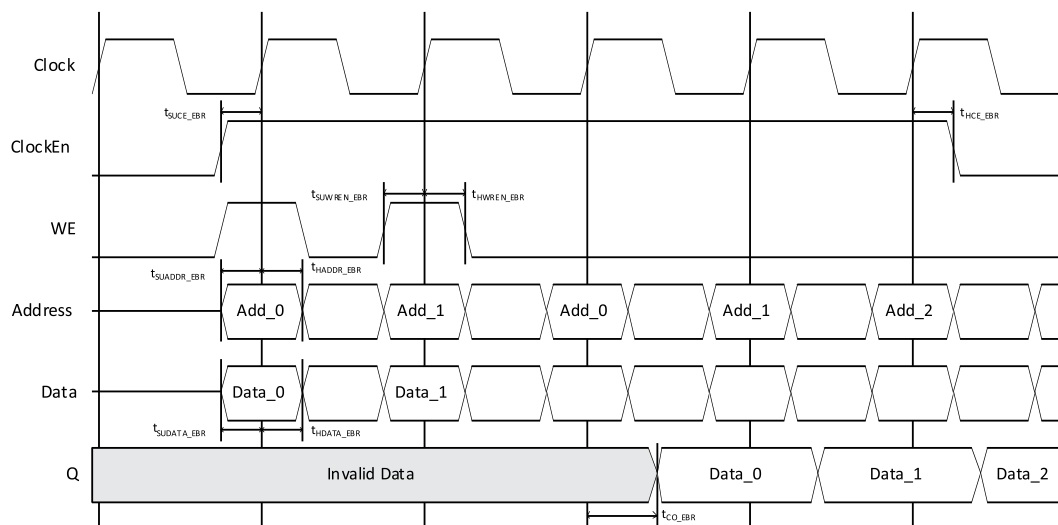
Figure 3.2. Single Port RAM Timing Waveform – NORMAL Mode, Without Output Registers
