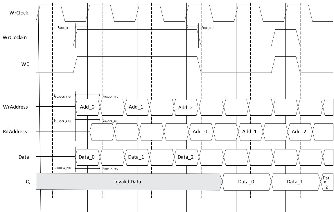
Figure 6.7. PFU-Based Distributed Dual Port RAM Timing Waveform – Without Output Registers
