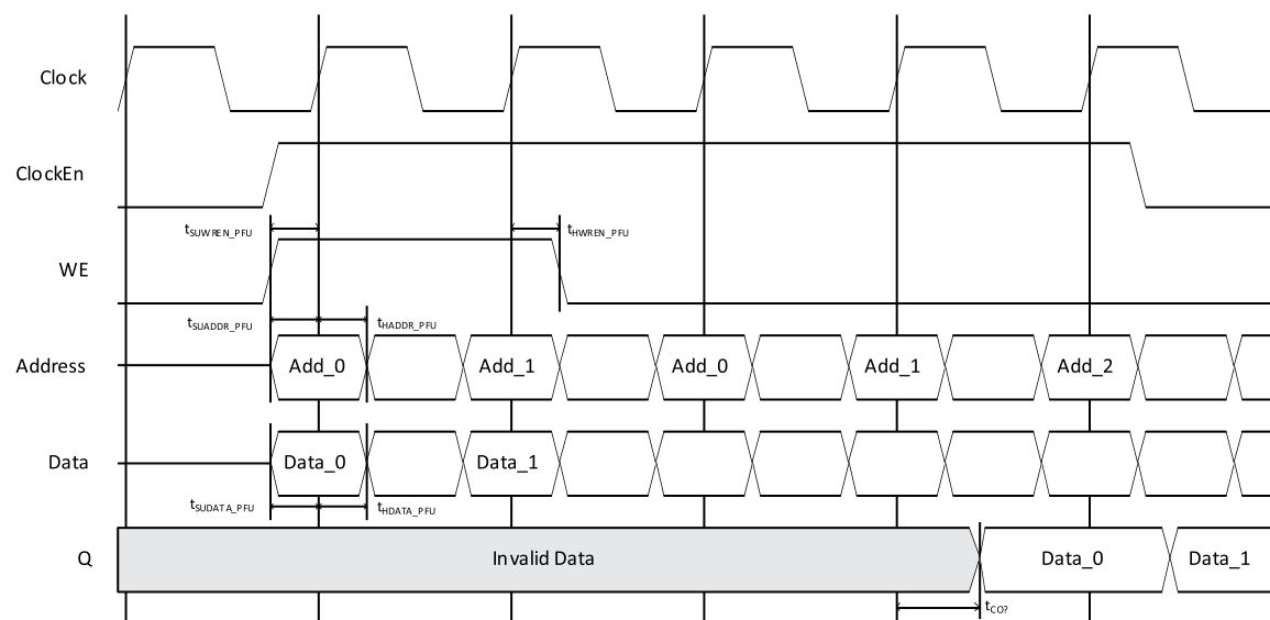
Figure 6.5. PFU- Based Distributed Single Port RAM Timing Waveform – With Output Registers
