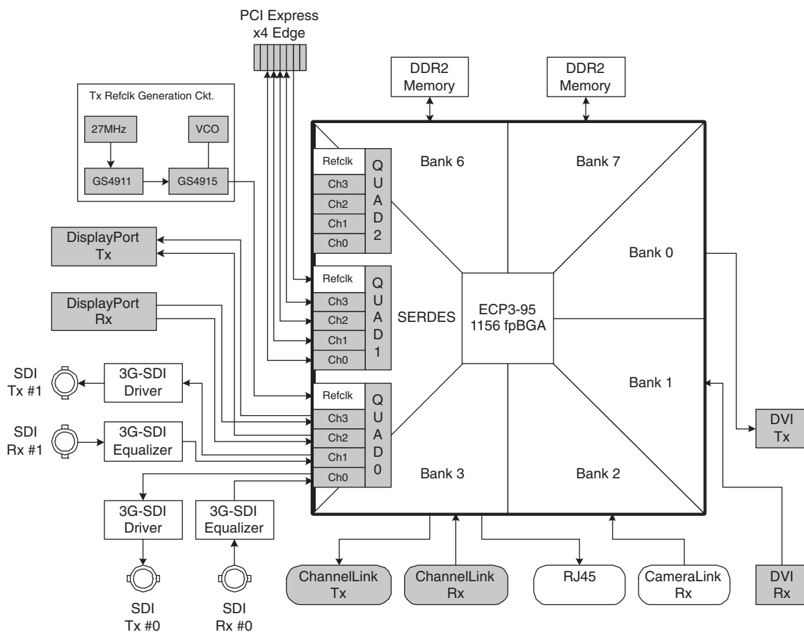
Figure 2. LatticeECP3 Video Protocol Board – Revision B Functional Partition
