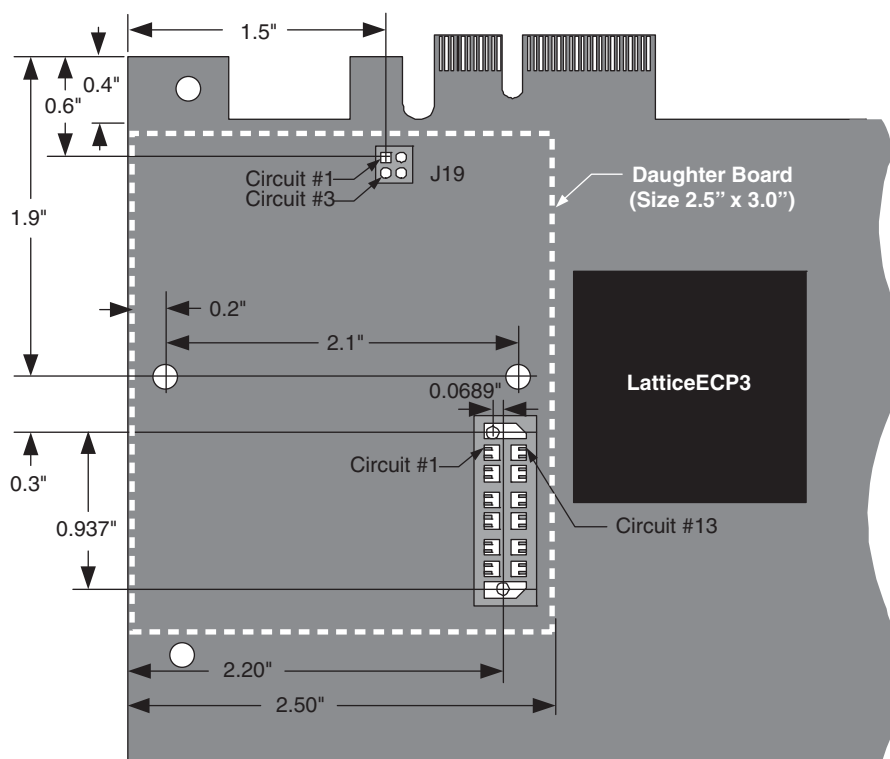
Figure 8. Mechanical Drawing of the Daughter Board Connection
