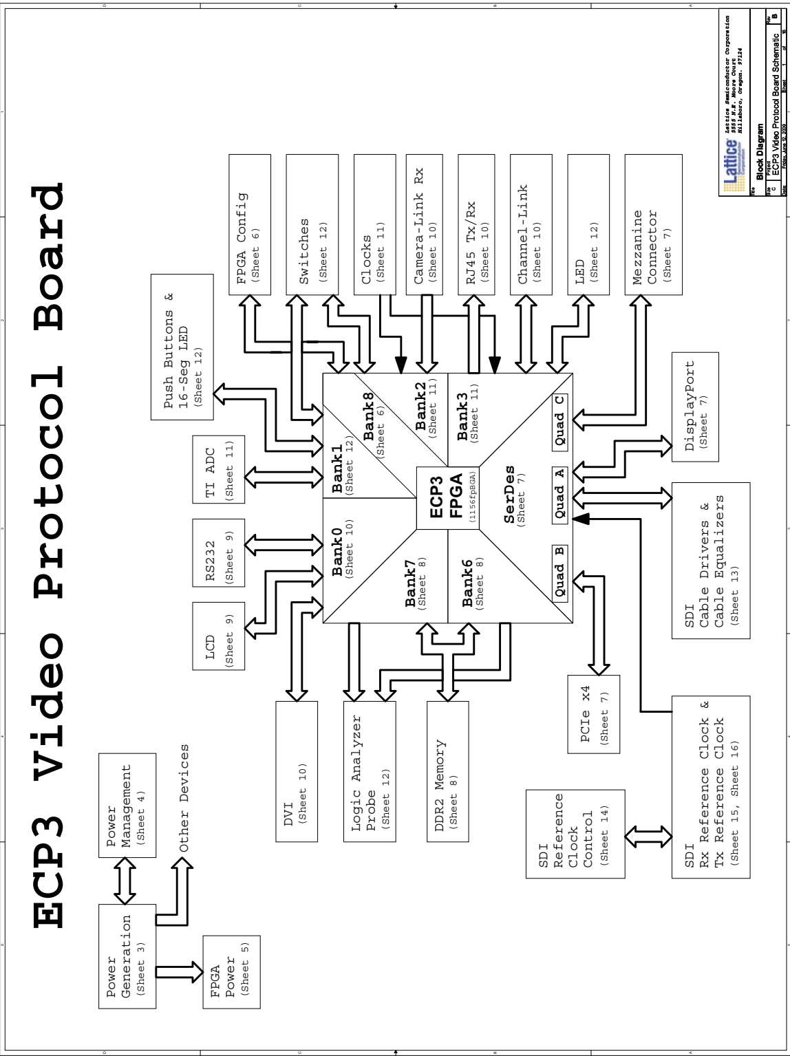
Figure 10. Block Diagram
