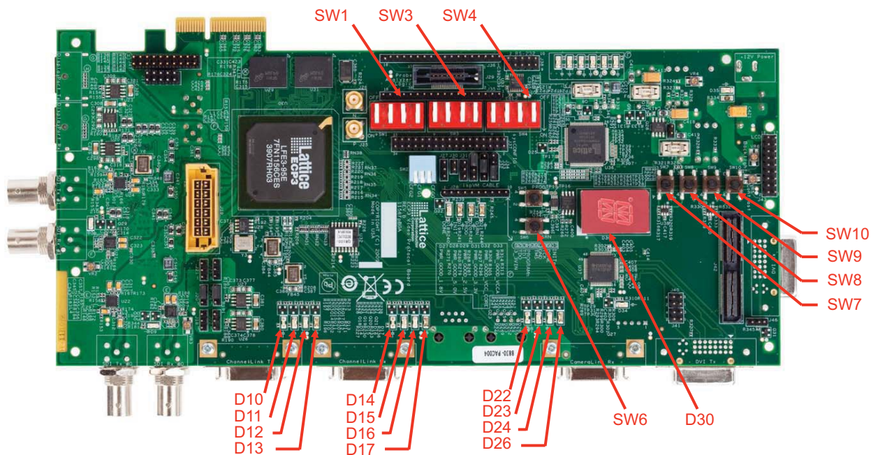
Figure 9. Locations of Switches and LEDs
