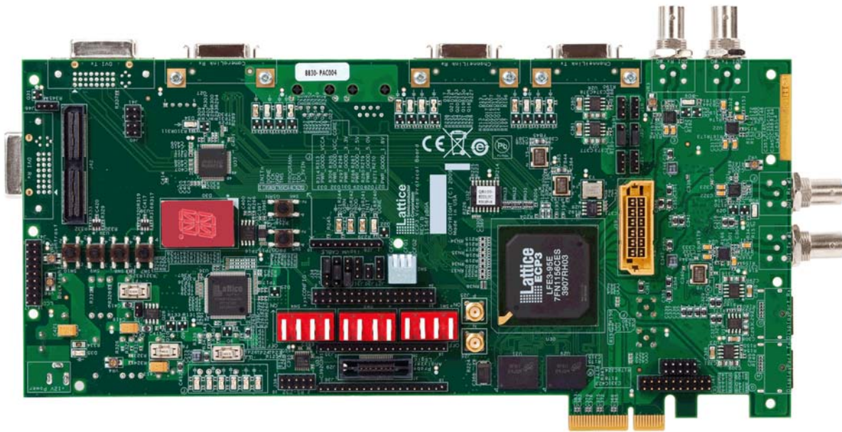
Figure 1. LatticeECP3 Video Protocol Board – Revision B
