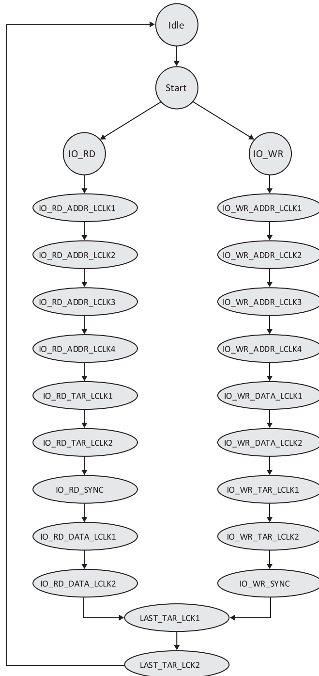
Figure 3.2. State Machine for the LPC Peripheral Module
