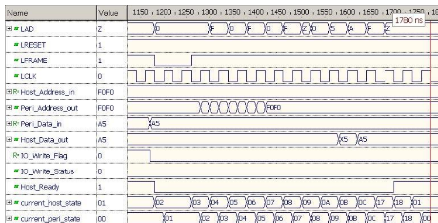
Figure 4.2. LPC Host Read Cycle
