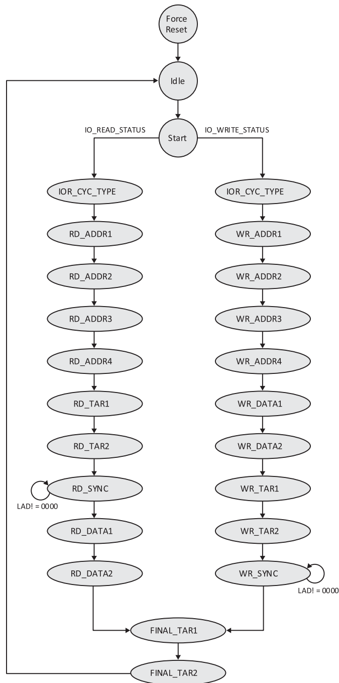
Figure 3.1. State Machine for the LPC Host Module
