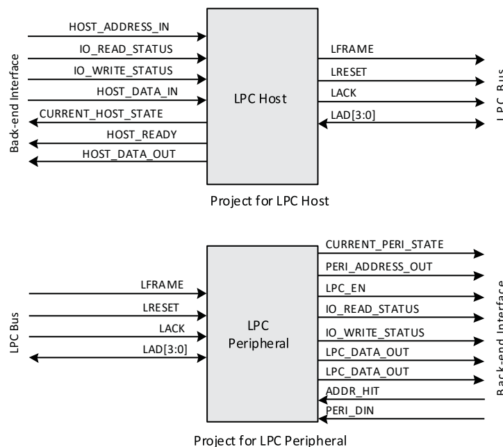
Figure 2.1. Reference Design Block Diagram
