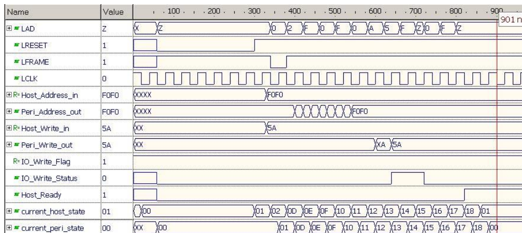
Figure 4.1. LPC Host Write Cycle
