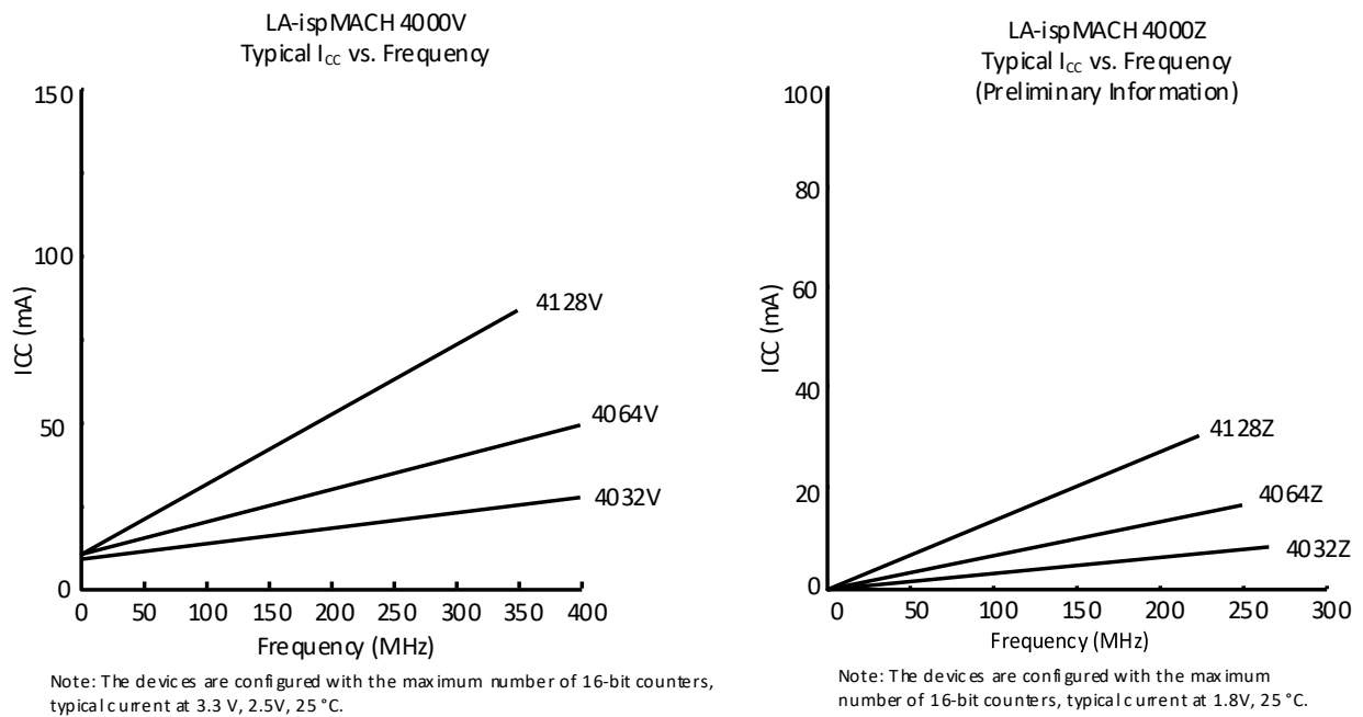
Figure 30.1. Power Consumption
