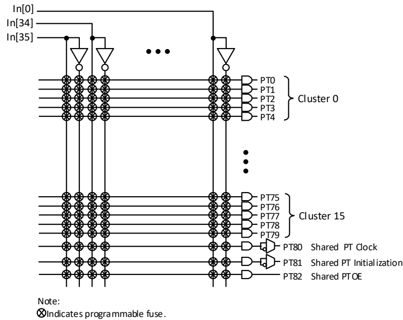
Figure 4.2. AND Array
