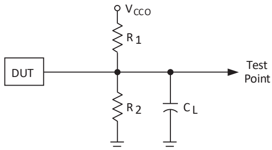
Figure 32.1. Output Test Load, LVTTTL and LVC MOS Standards
