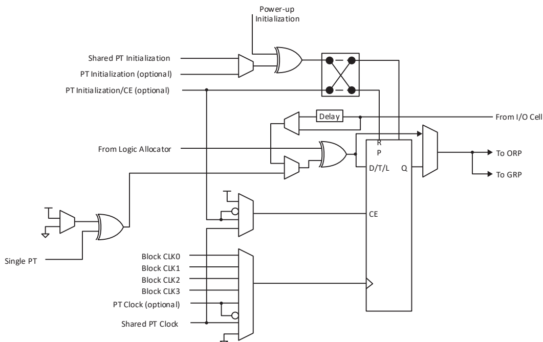
Figure 4.4. Macrocell
