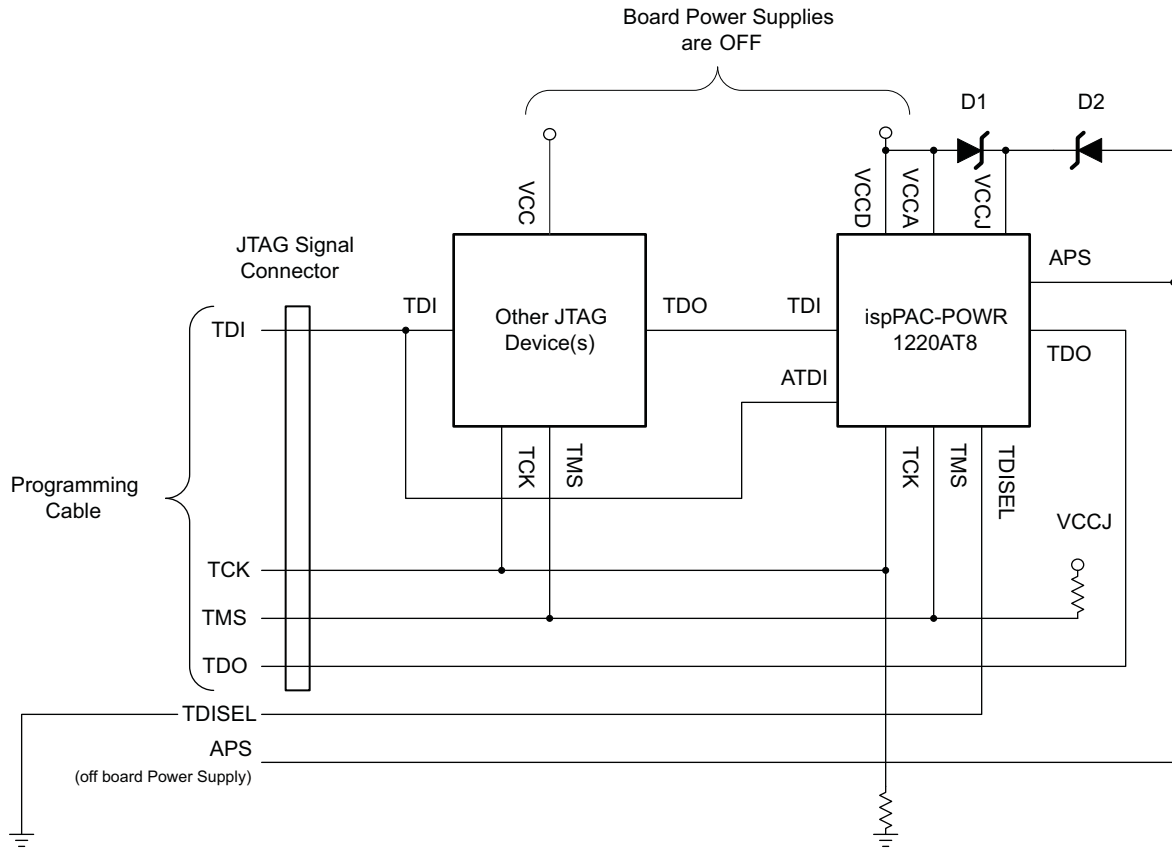
Figure 36. ispPAC-POWR1220AT8 Alternate Configuration Diagram
