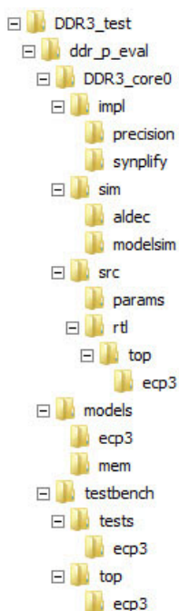
Figure 4-3. LatticeECP3 DDR3 Core Directory Structure
