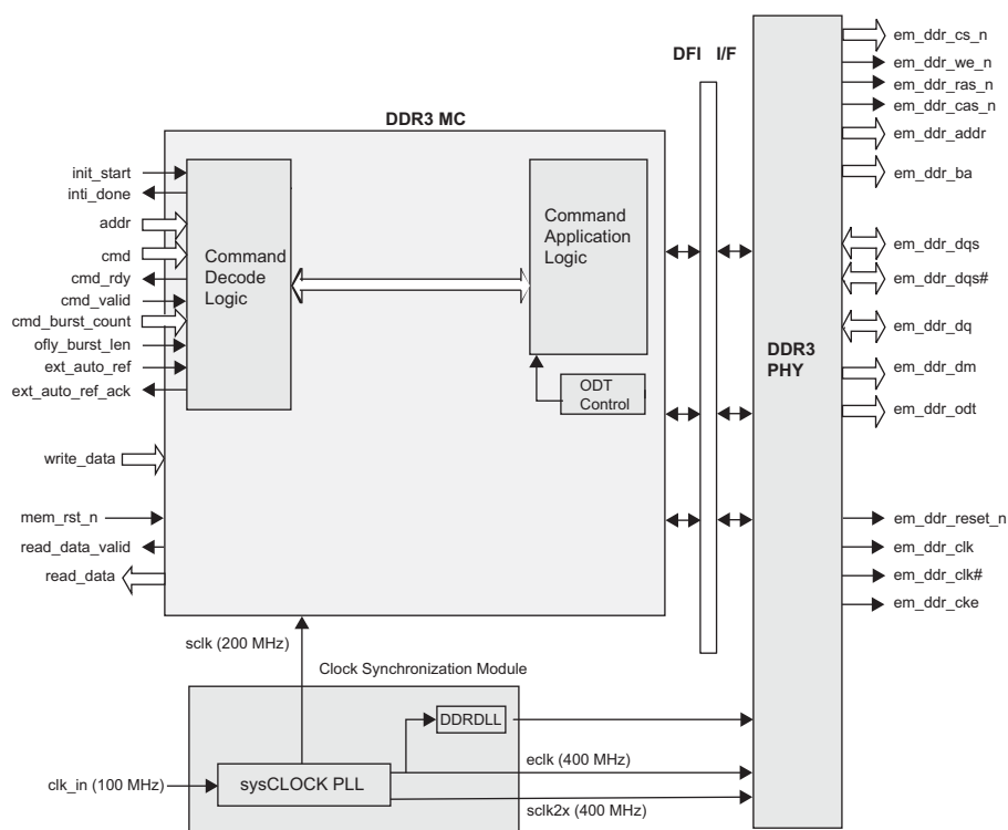
Figure 2-1. DDR3 SDRAM Controller Block Diagram
